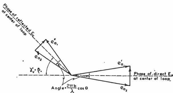
Fig. 7—Vector diagram for voltages in horizontal-loop elements due to vertically polarized downcoming wave as in Fig. 5.
