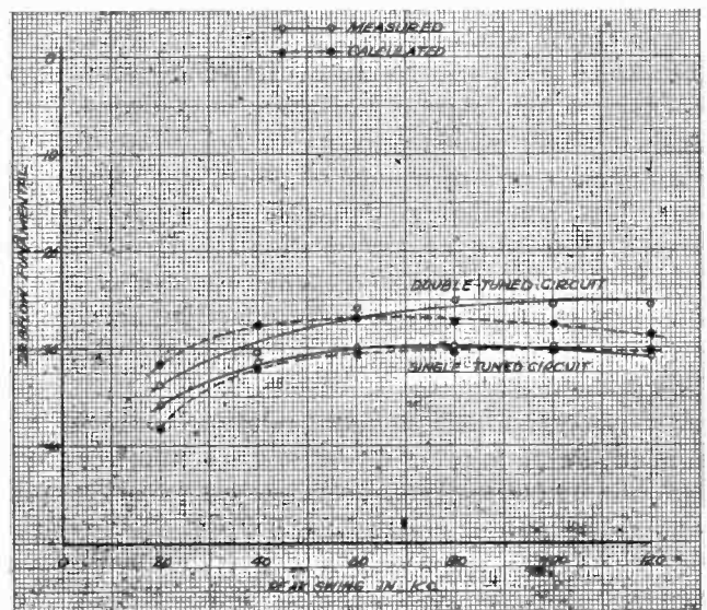
Fig. 23—Root-mean-square third- and fifth-harmonic distortion as a function of peak frequency swing for single- and double-tuned circuits. Double-tuned circuit critically coupled. F_o = 2800 cycles per second. BW = 50 kilocycles at 1700 kilocycles.
