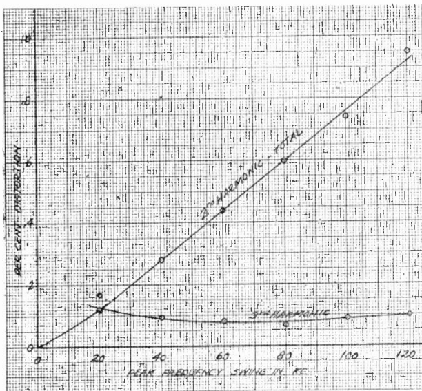
Fig. 10—System distortion as a function of frequency swing. f_m = 2800 cycles per second without tuned circuits.
