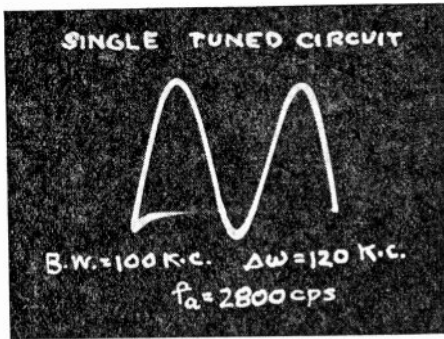
Fig. 16—The effect of doubling the bandwidth for the same parameters as in Fig. 15(a).
