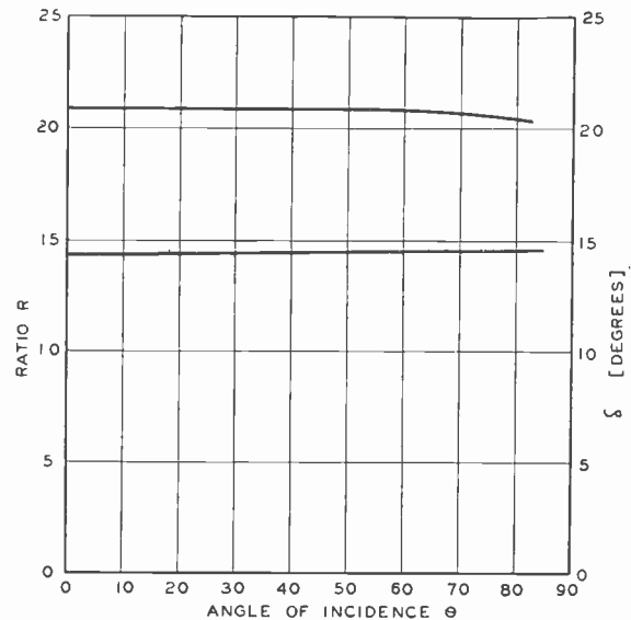
Fig. 17—Variation of loop-versus-antenna voltage ratio R and phase \delta as a function of angle of incidence for example number 2. k = 8 \delta = 5 \times 10^{-14} electromagnetic unit h_0 = \lambda/36 b = \lambda/55 \lambda = 550 meters
