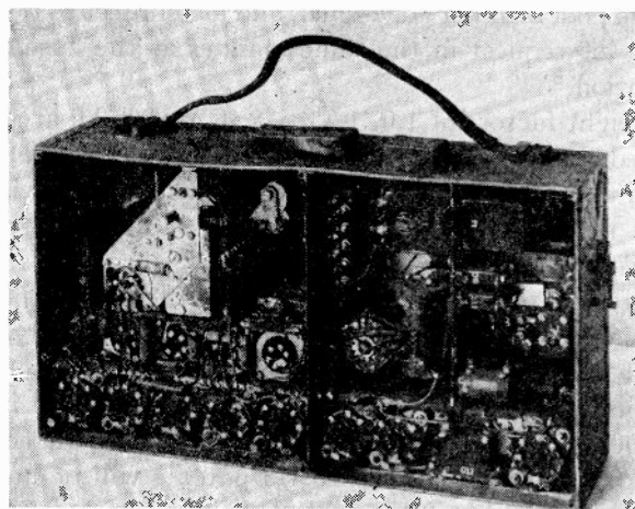
Fig. 2—Radio set constructed before the war for temperate climates. This set was sent to New Guinea after several years service in the Middle East. Results of a few months exposure to tropical climate can be seen.
