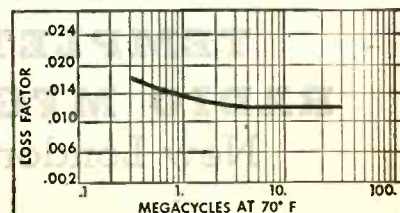
Based on Power Factor Measurements made by Boonton Radio Corp. on a standard Mykroy stock.
