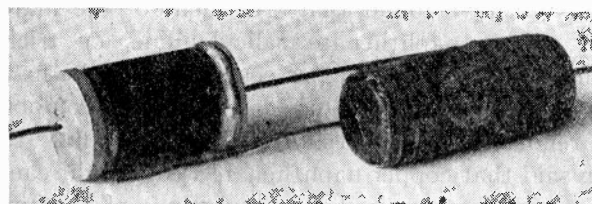
Fig. 6—Wax-moulded paper capacitor with mould on the label. The new glass-cased type is shown for comparison.
