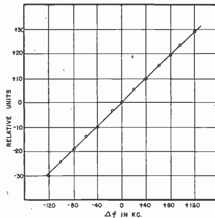
Fig. 8—Receiver detector characteristic.
