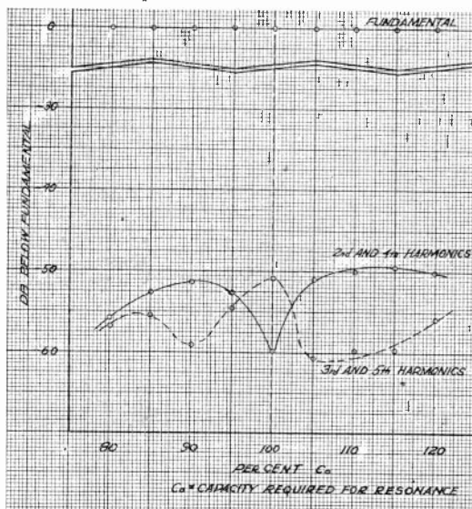
Fig. 14—Experimental determination of distortion as a function of tuning capacitance. Single-tuned circuit. BW=50 kilocycles at 1700 kilocycles. Peak frequency swing = 120 kilocycles. F_a=2800 cycles per second.
