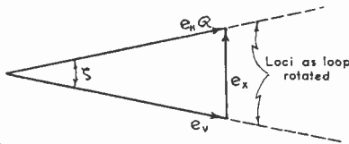
Fig. 13—Vector diagram showing residual voltage e_x resulting when neutralization is incomplete.
