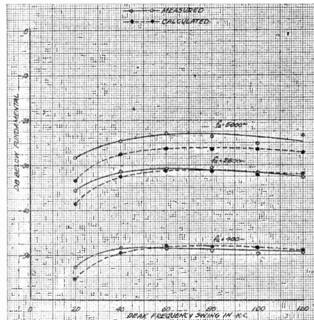
Fig. 12—Third-harmonic distortion as a function of frequency swing. Single-tuned circuit. BW = 50 kilocycles at 1700 kilocycles.
