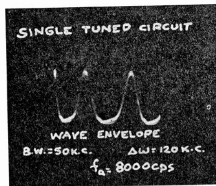
Fig. 19—Carrier envelope for conditions given on oscillogram.
