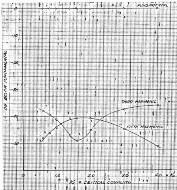
Fig. 24—Harmonic distortion as a function of coupling. Double-tuned circuit. For critical coupling. BW=125 kilocycles, F_a=2800 cycles per second. Peak frequency swing = 120 kilocycles.
