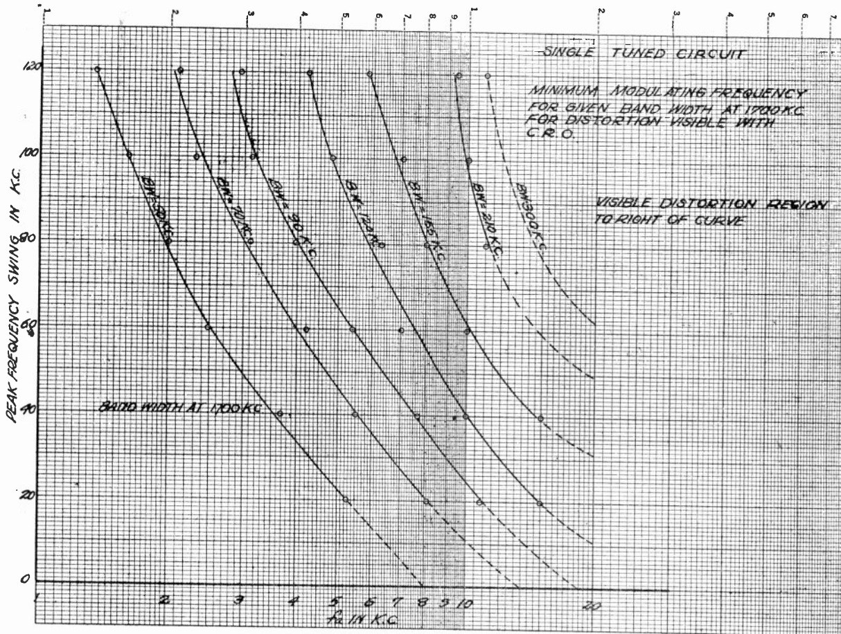
Fig. 20—Single-tuned circuit. Minimum modulating frequency for given bandwidth at 1700 kilocycles for distortion visible with cathode-ray oscilloscope.
