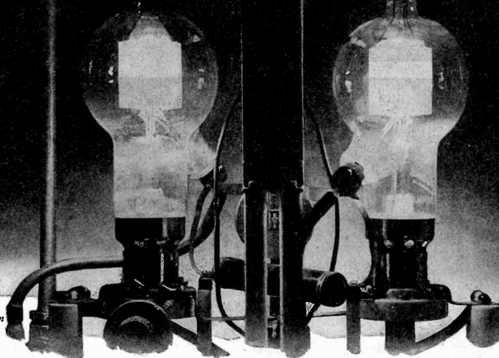
Eimac 1000T tubes in an amplifier stage of W6XAO transmitter, Hollywood
