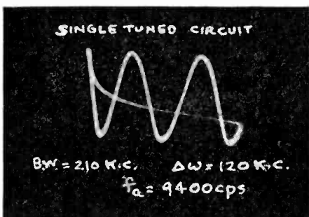
Fig. 21—Wave forms used as criteria for curves of minimum modulating frequency for given bandwidth at 1700 kilocycles for distortion visible with cathode-ray oscilloscope.
