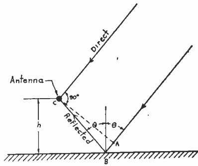
Fig. 4—Geometrical arrangement of wave paths for downcoming wave.
