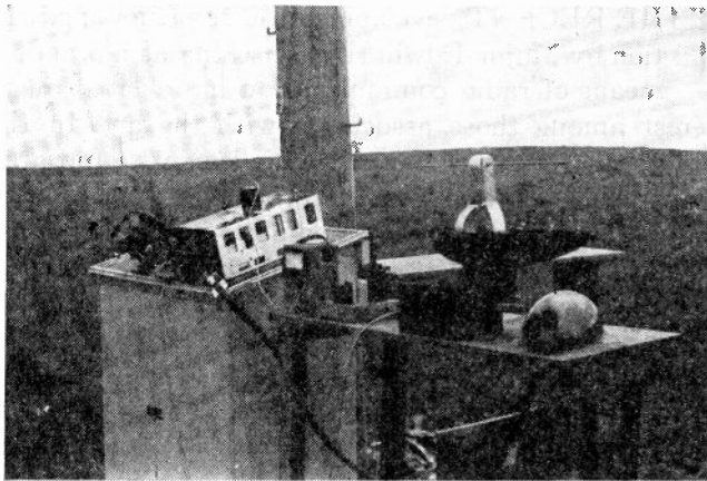
Fig. 22—Compensating antenna mounted on airborne-type direction finder for trial demonstration. Coupling amplifier is in small box in front of loop assembly. Receiver and output meter at left.
