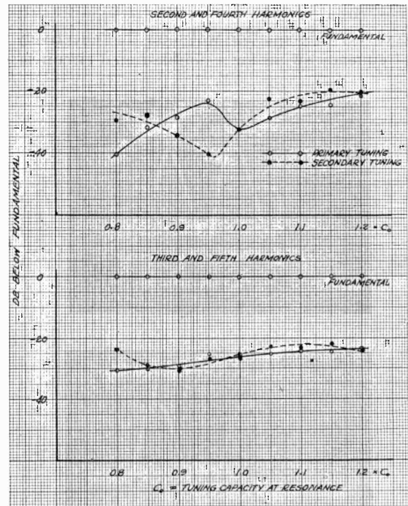
Fig. 25—Experimental determination of distortion as a function of primary and secondary tuning capacitance for a double-tuned circuit, critically coupled. BW=50 at 1700 kilocycles. F_a=2800 cycles per second. Peak frequency swing = 120 kilocycles.
