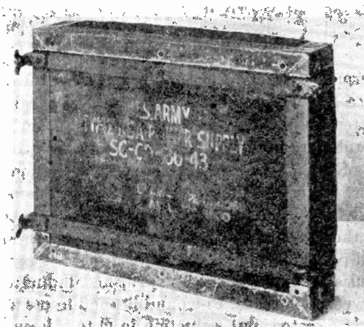
Fig. 3—Carrying-case lid constructed with casein-bonded plywood treated in any way. The damage seen took place after one month in the static-humidity-test atmosphere set out in the report.
