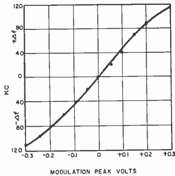
Fig. 6—Frequency-modulation signal-generator calibration.
