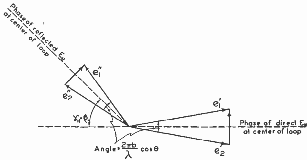
Fig. 9—Vector diagram for voltages in loop due to horizontally polarized downcoming wave as in Fig. 8.
