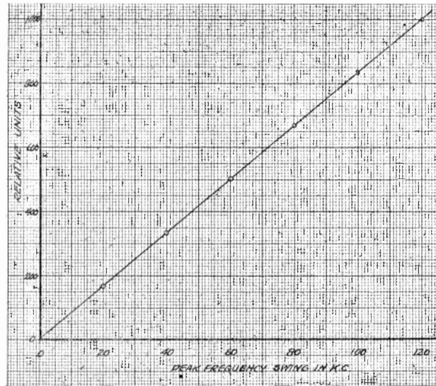
Fig. 11—Experimental determination of variation of fundamental with frequency swing. f_m = 2800 cycles per second. Single-tuned circuit, critically coupled, BW = 50 kilocycles. Bandwidth at 1700 kilocycles.
