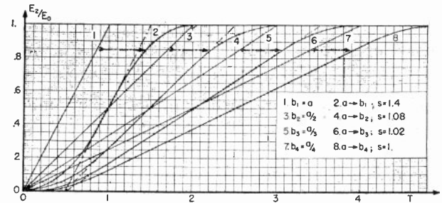
Fig. 20—Transient response of cascades of two different stages, each of which gives, alone, a straight transition to a unit-step input.
