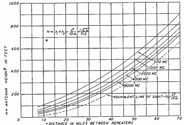
Fig. 9—Antenna heights to provide equivalent of free-space propagation.
