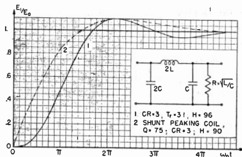
Fig. 13—Transient response to a unit step of current, of a capacitance-terminated filter.
