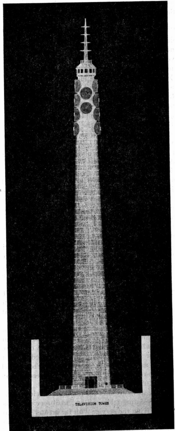
Fig. 17—Recommended design of television tower. It provides: 1. Rigid mounting of antennas at any height and pointed in any direction. 2. Housing for repeaters at antenna heights to save losses in transmission lines or wave guides. 3. Means of access protected from wind, rain, ice, and snow. 4. Observation platform for visitors. 5. Cost comparable with less-desirable steel towers. 6. Mounting for broadcast antennas when required.
