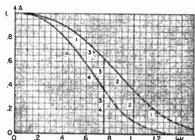
Fig. 45—Amplitude responses restricted by the width of a channel.
