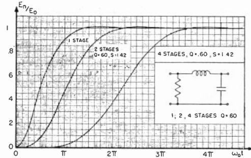
Fig. 27—Transient response of cascades of two and four stages of series-peaking coil circuits Q=0.60 to a unit step of current.
