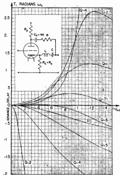
Fig. 53—Time-delay response of phase-corrector stage.
