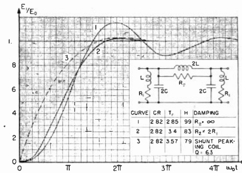
Fig. 12—Transient response to a unit step of current, of improved filter with two separate capacitances.
