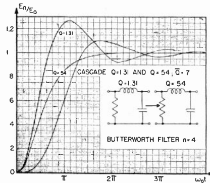
Fig. 32—Transient response of cascade n=4 of Butterworth system to a unit step of current.
