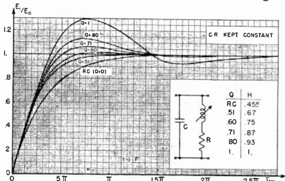
Fig. 9—Transient response to a unit step of current for equal gain, shunt-peaking coil circuit.
