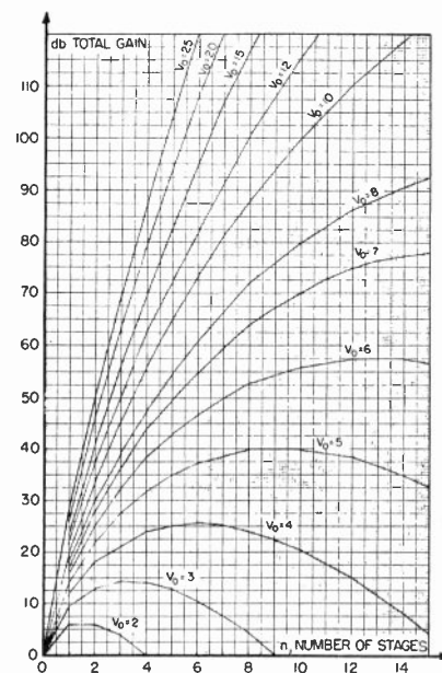
Fig. 36—Gain of amplifier cascades designed for equal over-all transition time, as a function of the number of stages.
