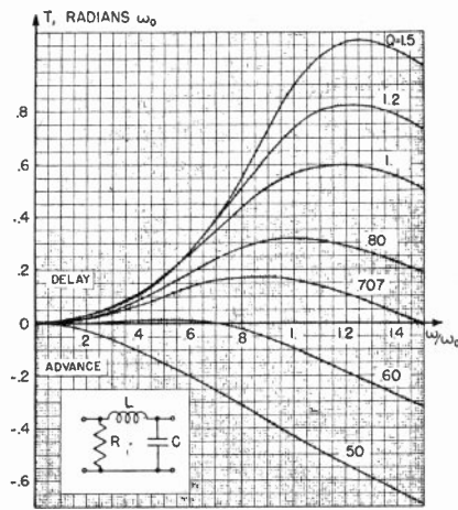
Fig. 3—Time-delay response of series-peaking coil circuit.
