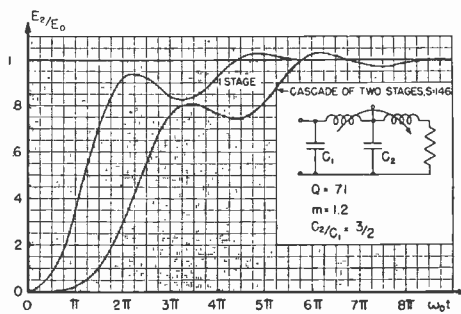
Fig. 34—Deterioration of transient response in a cascade of unsuitable stages.
