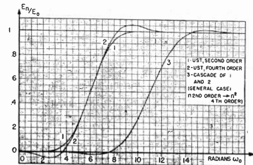
Fig. 43—Second- and fourth-order uniform-stretch transitions cascaded.
