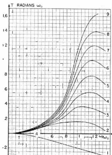
Fig. 31—Time-delay response of cascades according to Butterworth system.
