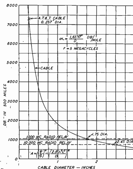
Fig. 12—Cable and radio-relay systems amplification required in 500 miles.
