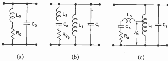
Fig. 60—The sucker circuit, the carrier-frequency analogue to the shunt-peaking coil circuit.
