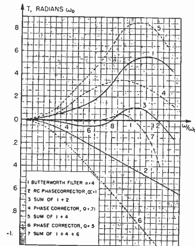
Fig. 56—Time-delay response of Butterworth filter n=4 with phase correction.
