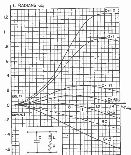
Fig. 7—Time-delay response of shunt-peaking coil circuit.
