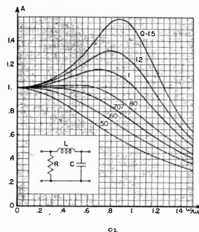
Fig. 2—Amplitude response of series-peaking coil circuit.
