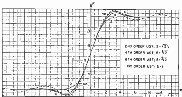
Fig. 42—Uniform-stretch transitions, fourth, sixth, and \infty orders.
