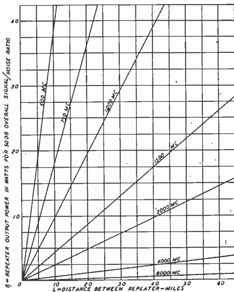
Fig. 8—Power output required from repeaters. P_T = (2.8 \times 10^3 \lambda^3 L^2 NP_p) / D^4 .
