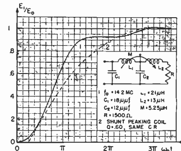
Fig. 15—Transient response to a unit step of current, of a filter with an m -derived terminating section.
