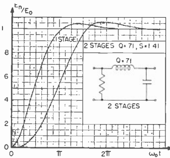
Fig. 28—Transient response of a cascade of two stages with series-peaking coil circuits Q=0.71 to a unit step of current.
