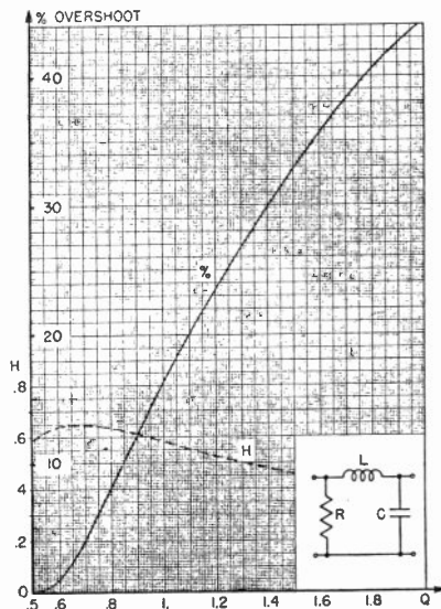
Fig. 4—Overshoot and figure of merit of series-peaking coil circuit.
