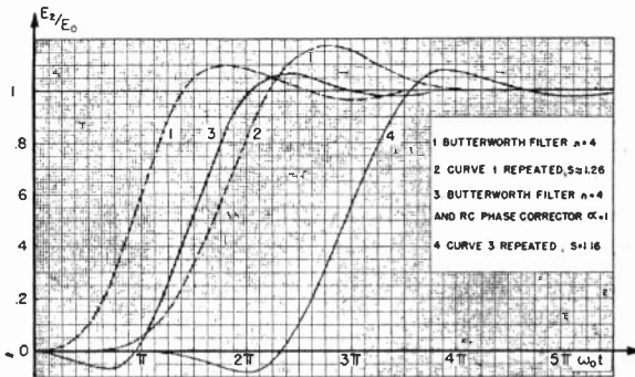
Fig. 57—Transient response of Butterworth filter n=4 with phase correction.
