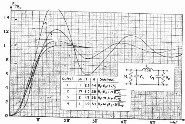
Fig. 10—Transient response to a unit step of current, of filter with two separate capacitances.
