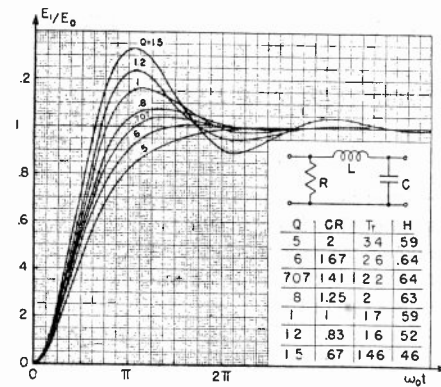
Fig. 1—Transient response of series-peaking coil circuit to a unit step of current.
