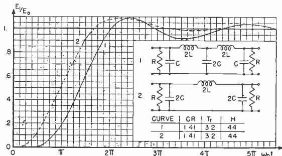
Fig. 11—Transient response to a unit step of current, of filter with three separate capacitances.
