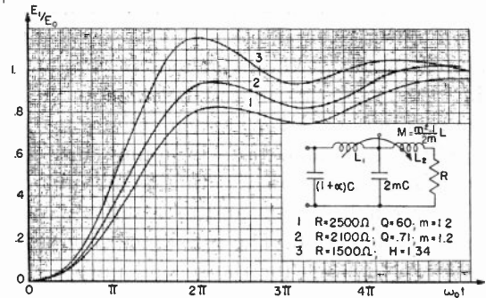
Fig. 14—Transient response to a unit step of current, of a filter with an m -derived terminating section.
