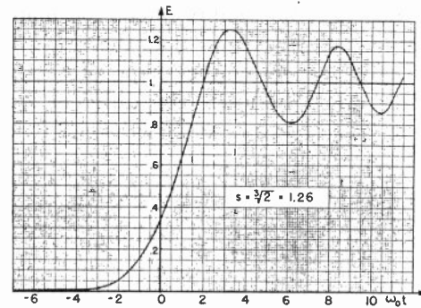
Fig. 41—Uniform-stretch transition, third order.
