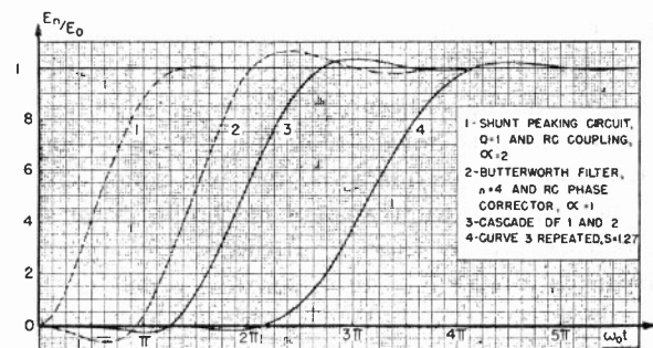
Fig. 58—Transient response of cascade of curve 3, Fig. 57, and curve 1, Fig. 52.
