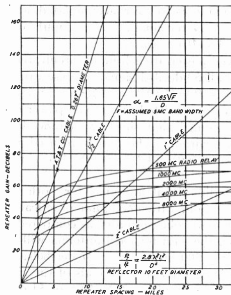
Fig. 11—Cable and radio-relay systems, gain per repeater required for various repeater spacings.
