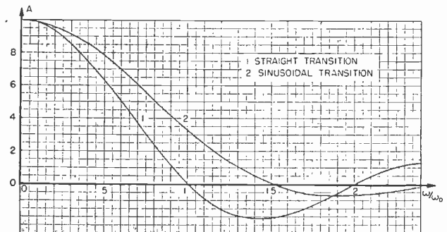
Fig. 21—Amplitude response corresponding to a straight, and to a sinusoidal, transition.
