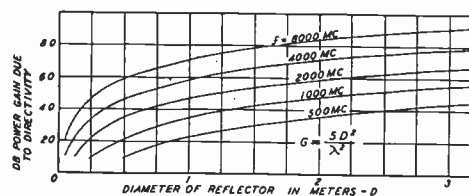
Fig. 5—Power gain per hop due to antenna directivity as compared with short dipoles.
