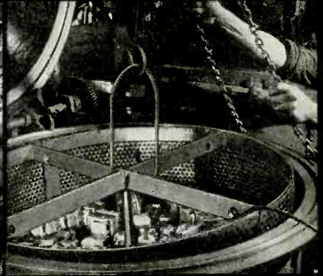
VACUUM IMPREGNATION with varnish removes moisture from coil and provides excellent turn, layer and section insulation, resulting in long trouble-free life.
