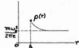
Fig. 5—Space-charge distribution, as a function of r , under critical conditions.
