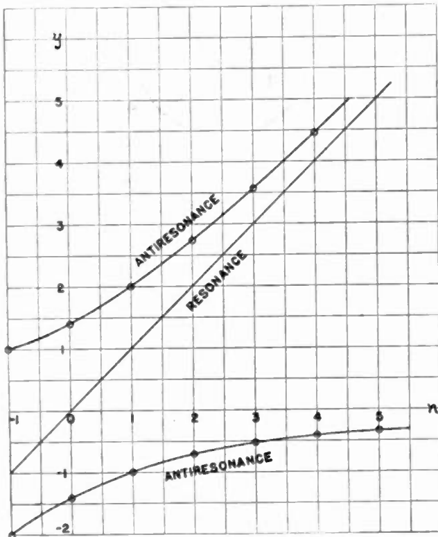
Fig. 8—Proper frequencies of oscillation corresponding to the different types indicated on Fig. 7, y = \omega/\omega_H is the ratio of frequency to Larmor's frequency, while n specifies the type of vibration.
