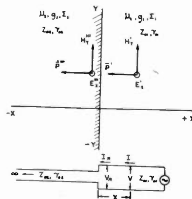
Fig. 7—Field-intensity vectors of incident and refracted waves at normal incidence and transmission-line analogue. (Vectors of reflected wave are omitted.)
