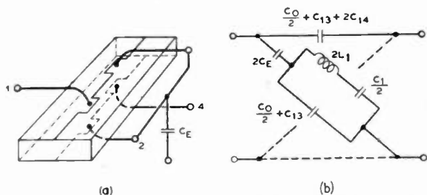
Fig. 17—Crystal connections and equivalent circuit for a flexure crystal used to obtain a phase reversal.
