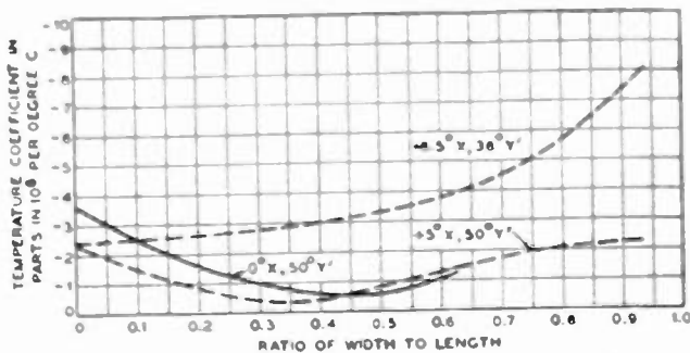
Fig. 13—Temperature coefficients of low-frequency NT flexure crystals.
