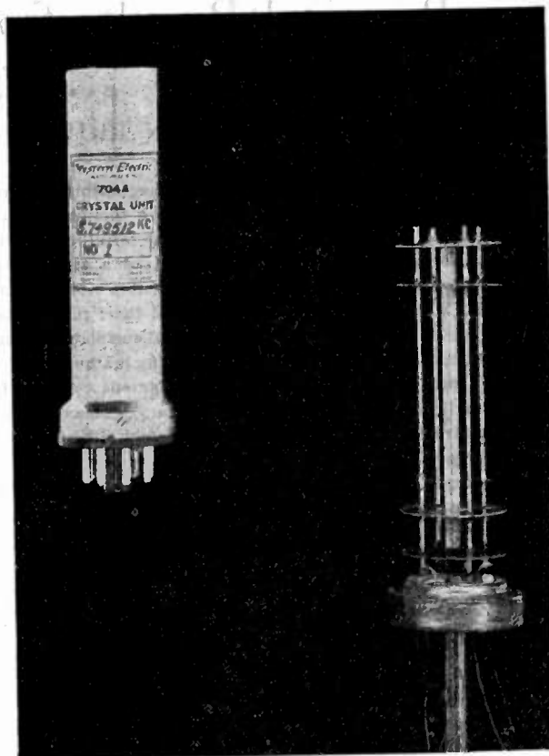
Fig. 18—Photograph of NT flexure crystal and holder.
