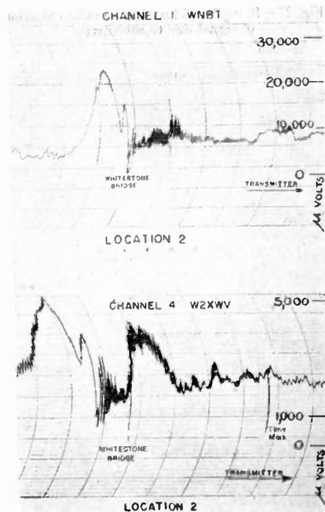
Fig. 26—Field-strength near Whitestone Bridge.
