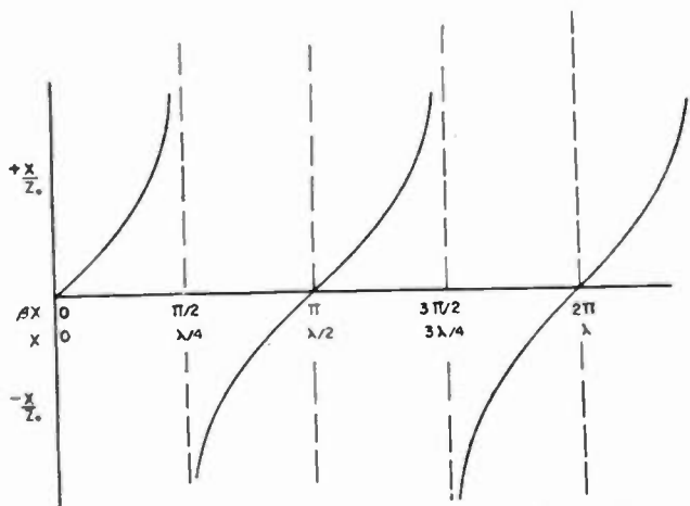
Fig. 5—Impedance ratios of short-circuited lossless line.
