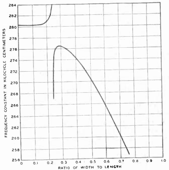
Fig. 3—Frequency constant of a +5-degree X-cut crystal as a function of the ratio of width to length.
