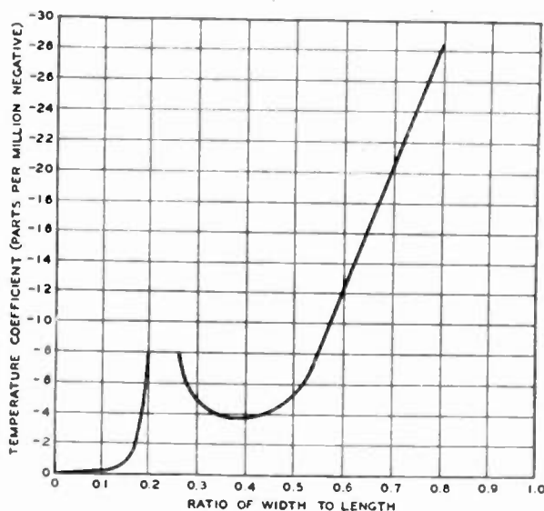
Fig. 4—Temperature coefficient of a +5-degree X-cut crystal as a function of the ratio of width to length.
