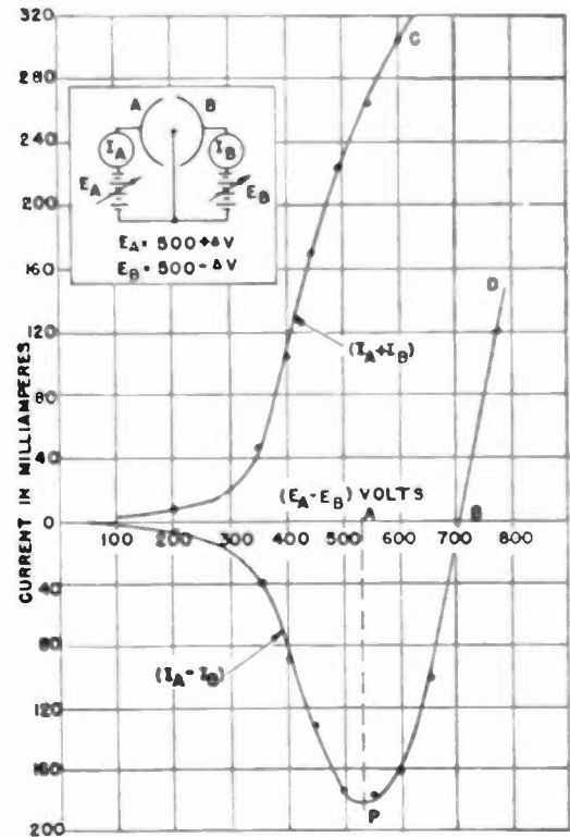
Fig. 12—Experimental results obtained by Kilgore for a split-anode magnetron ( n = 1 , 2 anodes). The interesting curve is the lower one, giving the static characteristic of I_A - I_B as a function of E_A - E_B . Notice the negative resistance corresponding to a slope downward.
