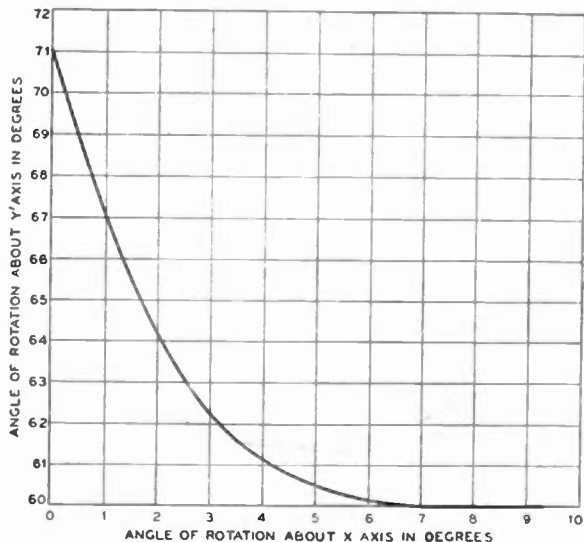
Fig. 15—Locus of angular orientations about X and Y' to produce a zero temperature coefficient for long thin NT flexure crystals.
