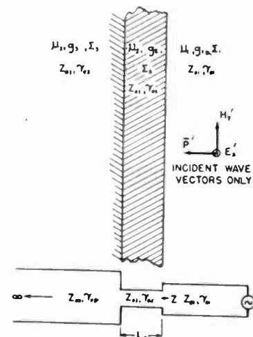
Fig. 9—Multiple-reflection and transmission-line analogue.
