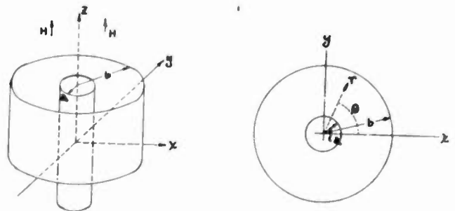
Fig. 1—Schematic representation of a magnetron.
