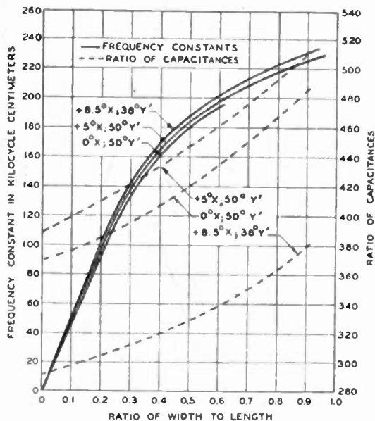
Fig. 14—Frequency constants and ratios of capacitances of low-frequency NT flexure crystals.
