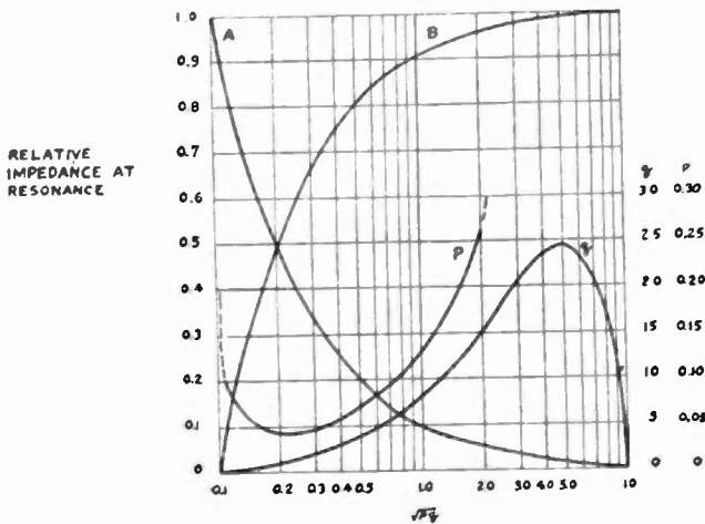
Fig. 3—Relative impedance at the two circle frequencies.
