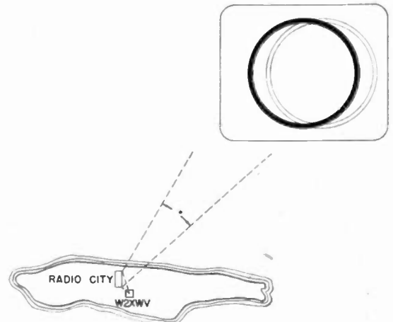
Fig. 11—Type A—fixed ghost. Narrow-angle reflection near transmitter.
