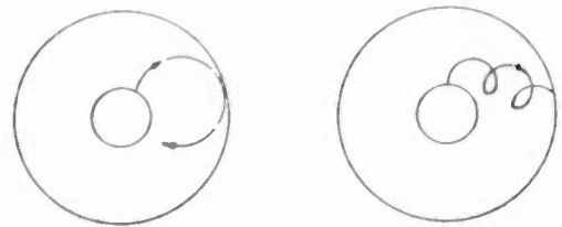
Fig. 2—Wrong electronic trajectories computed with incorrect space-charge distribution.
