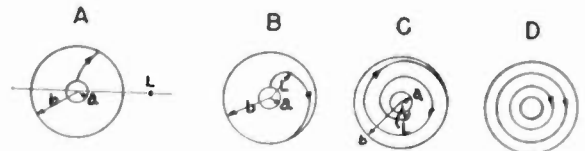
Fig. 3—Electronic trajectories for different magnetic fields
