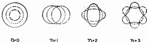
Fig. 7—Different types of possible oscillations in the space-charge distribution.
