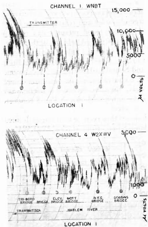
Fig. 23—Field-strength variations in Harlem River.
