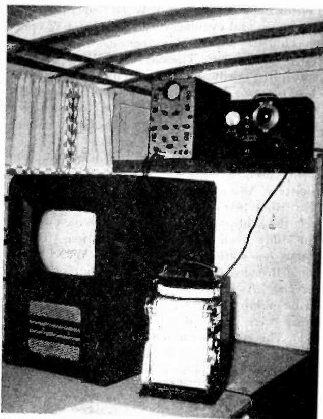
Fig. 4—Field-test recording setup.
