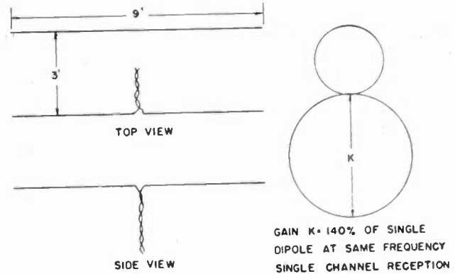
Fig. 2—Horizontal dipole and reflector.
