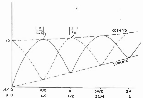
Fig. 3—Voltage and current ratios of short-circuited lines. Low attenuation.
