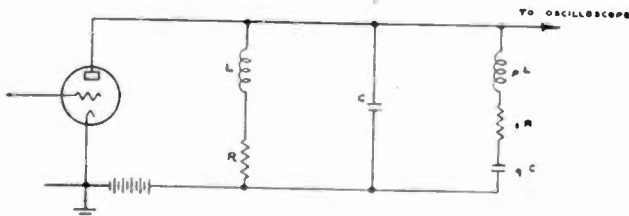
Fig. 2—Circuit for circle generation for two frequencies.
