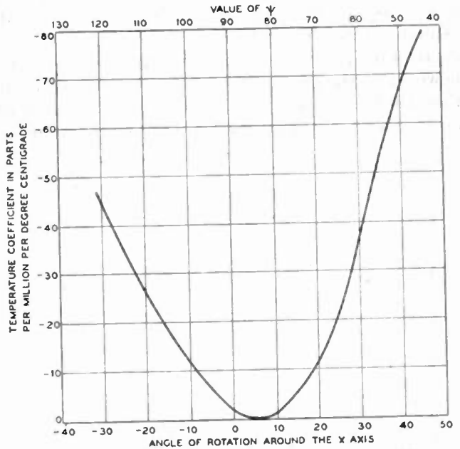
Fig. 2—Temperature coefficients of rotated X-cut bars.
