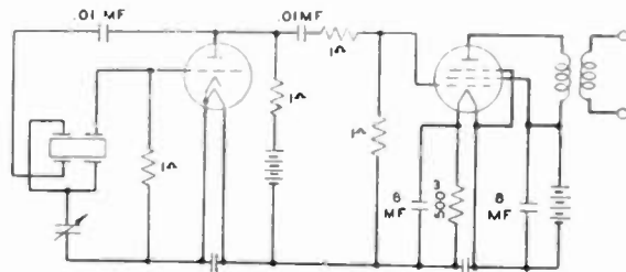
Fig. 16—Oscillator circuit for driving a low-frequency flexure crystal.
