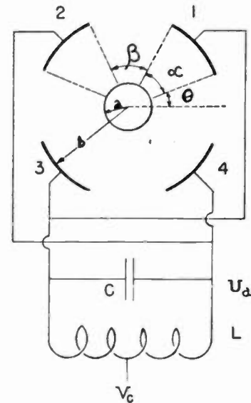
Fig. 9—Schematic representation of a split-anode magnetron connected to one single circuit ( n=2 , 4 anodes).
