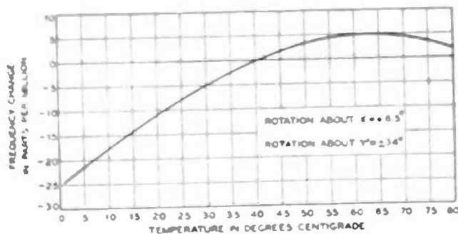
Fig. 12—Change in frequency of an MT crystal over a wide temperature range.
