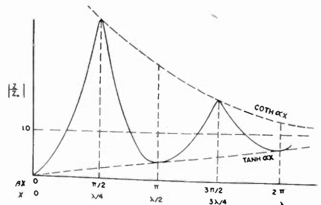
Fig. 4—Impedance ratios of short-circuited line. Normal line.
