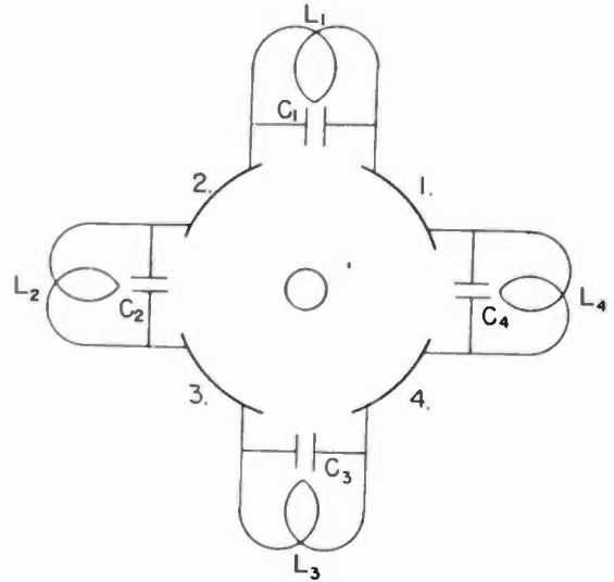
Fig. 13—Connections of a 4-anode magnetron with 4 separate circuits, instead of the conventional scheme of Fig. 9.
