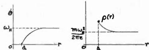
Fig. 5—Space-charge distribution, as a function of r , under critical conditions.
