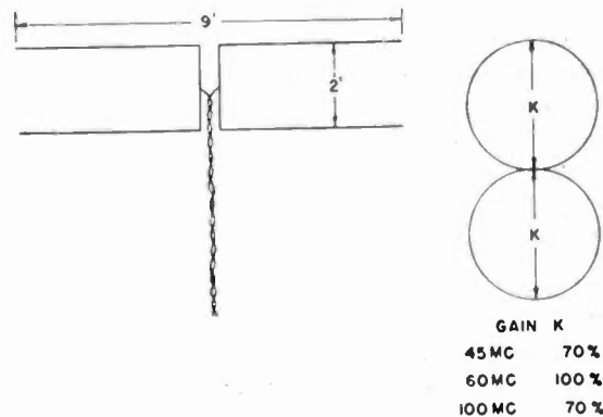
Fig. 3—Horizontal double dipole.
