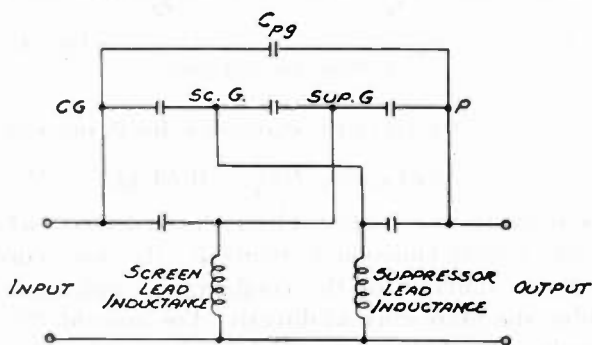
Fig. 12—Equivalent circuit of pentode.
