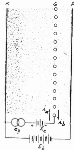
Fig. 6—Triode showing presence of electron space charge.
