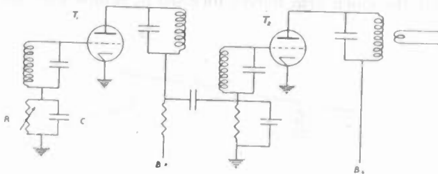
Fig. 4—The basic circuit of the Diamond-Hinmann radio-meteorograph transmitter.
