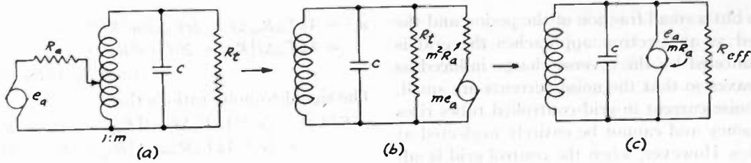
Fig. 4—Equivalent circuits of input transformer of receiver for any value of effective step-up ratio m between antenna and tube.
