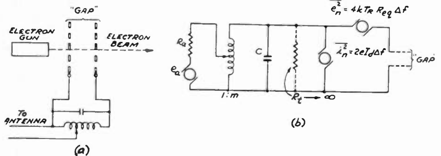
Fig. 6—A velocity-modulation type of mixer tube and its equivalent circuit. Two noise generators \overline{e_n^2} equivalent to noise at the anode and at points beyond, and the other as a current generator \overline{i_n^2} corresponding to induced noise across the input electrodes.
