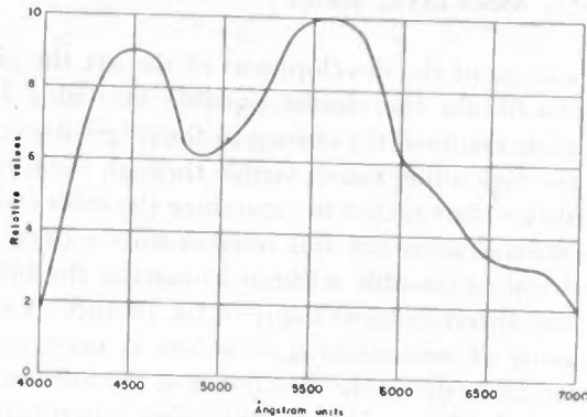
Fig. 1—Spectral characteristic of an experimental phosphor.
