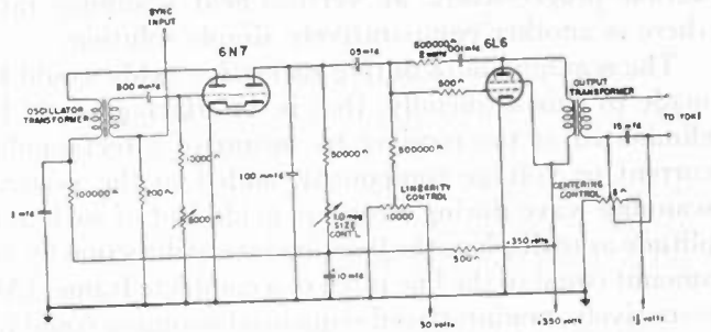
Fig. 19—High-frequency scanning circuit.
