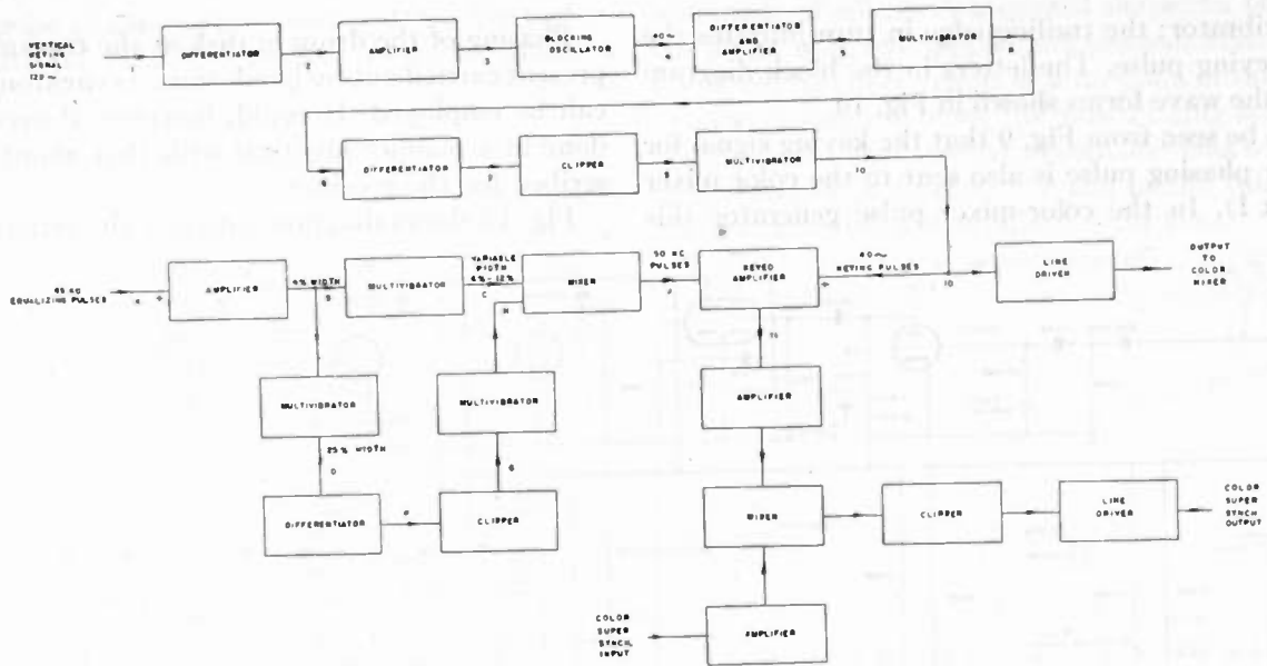
Fig. 9—Color-phasing pulse-generator block diagram.
