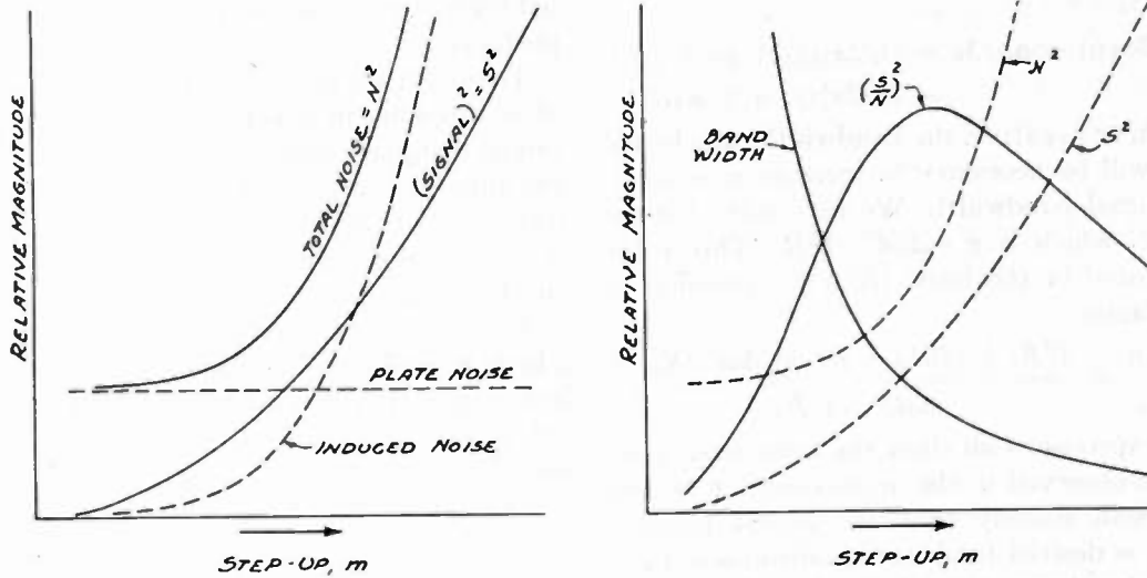
Fig. 7—Relative magnitudes of signal, noise, bandwidth, and signal-to-noise ratio for a case where input resistance is infinite. The curves are divided into two groups only to avoid confusion; the S^2 and N^2 curves are common to both groups.
