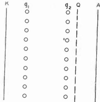
Fig. 8—Determination of amplification factor and inter-electrode capacitance in multigrad structures by use of the Q plane.
