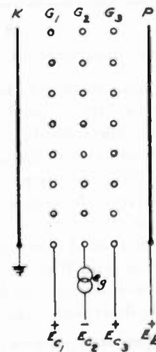
Fig. 9—Space-charge-grid tube in which effect of space charge is to lower effective input conductance and capacitance.
