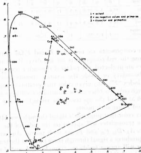
Fig. 6—Comparison of color reproduction.
