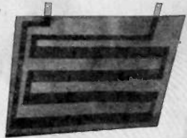
Battery heater for installation between cells to maintain 65°-70° temperature, for maximum battery efficiency.
