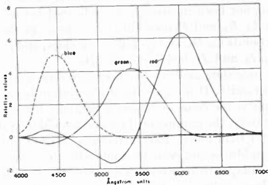
Fig. 3—Spectral characteristics at transmitter; primaries A .
