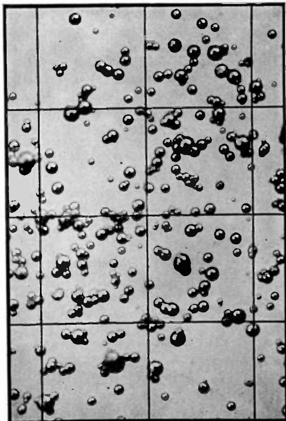
GAW Carbonyl Iron Powder "E" A superior core material for normal frequencies
