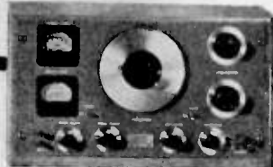
No. 205 AG Audio Signal Generator—Combines a Resistance tuned oscillator having 5 watts output and less than 1% distortion, plus Output meter, Input meter. Attenuator and an impedance matching system... all in a single unit.
