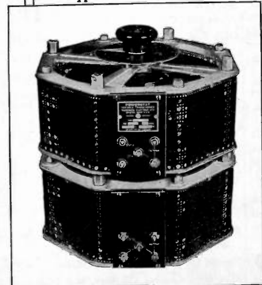
Three-Phase Powerstat
