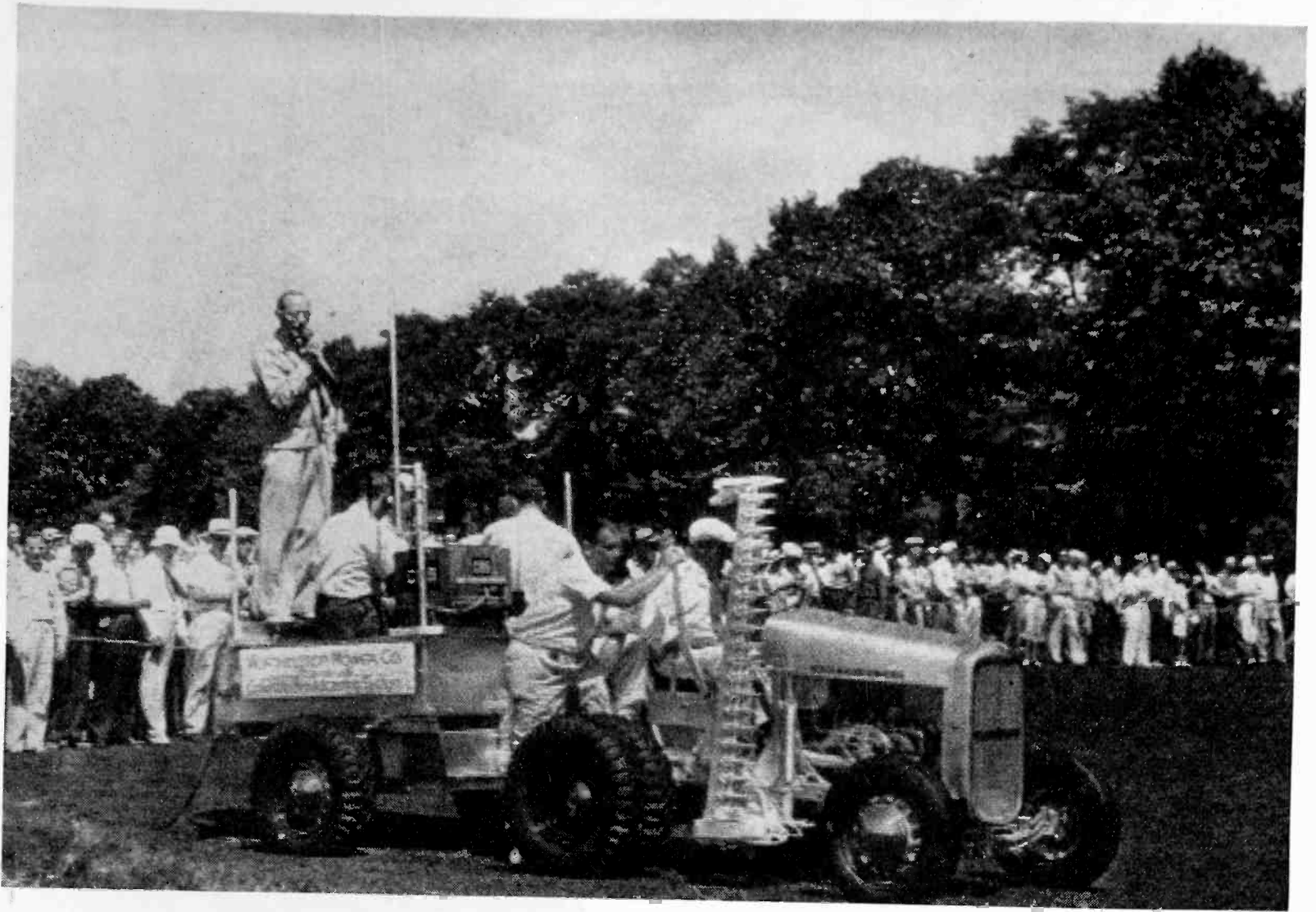
Fig. 15—Scanned picture (441 lines, 30 frames, 4.25 megacycles, \epsilon^{-x^2} aperture).
