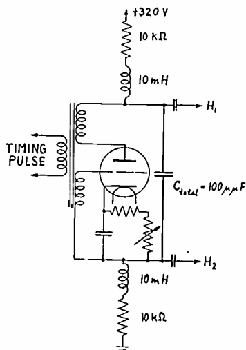
Fig. 3—Saw-tooth generator for push-pull deflection.
