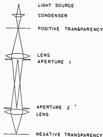
Fig. 6—Optical system.
