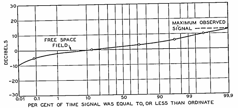
Fig. 12—Time distribution of the signal strength on 2 meters wavelength for the year 1938.
