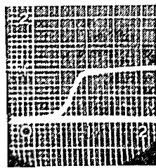
Fig. 19—Transient response of the test equipment itself; 3 divisions = 0.1 microsecond.
