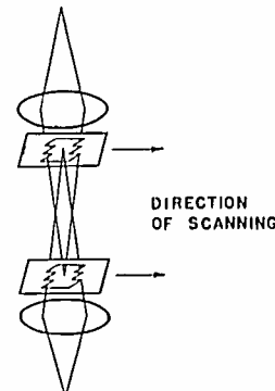
Fig. 12—Arrangement of apertures to simulate effect of frequency response and receiver spot size.
