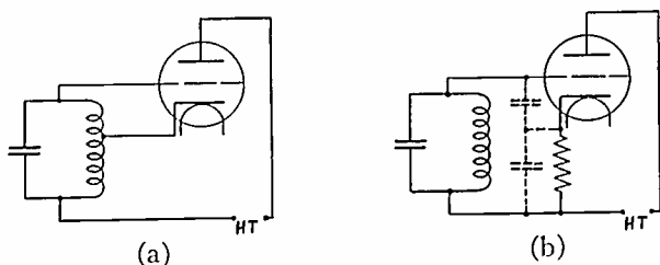
Fig. 14—(a) Cathode-coupled oscillator circuit; (b) cathode follower as oscillator circuit.
