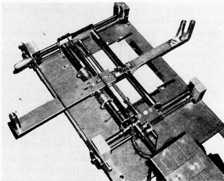
Fig. 5—Artificial television scanner partially disassembled.
