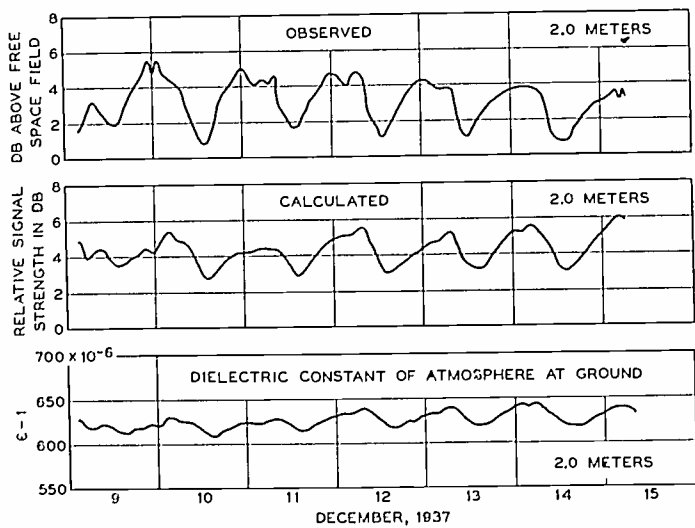
Fig. 14—There were times when a degree of correlation was observed between the signal strength and the dielectric constant of the air at Beer's Hill. The top curve shows the observed signal, the bottom curve, the dielectric constant of the air at Beer's Hill, and the middle curve shows the calculated value of field strength as explained in the text.
