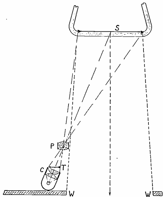
Fig. 17—Scale projection for cathode-ray tubes.
