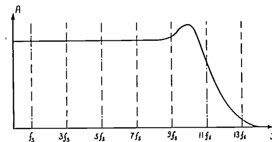
Fig. 2—Exploring harmonics of a square wave of the frequency f_s .
