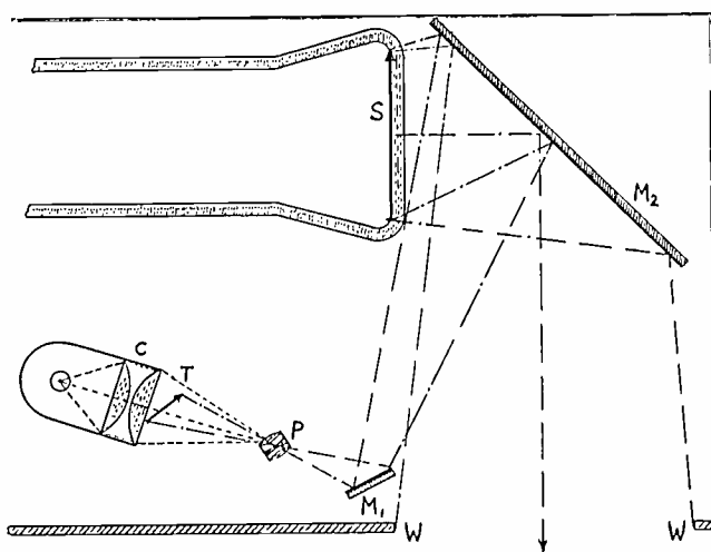
Fig. 16—Space-saving arrangement of scale projection.
