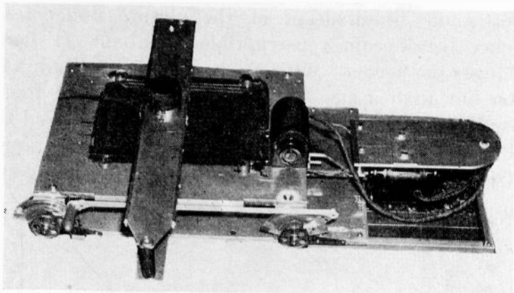
Fig. 4—Artificial television scanner.
