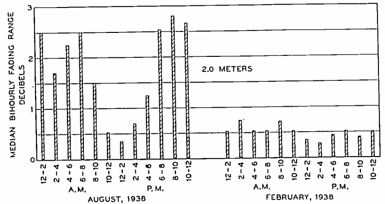
Fig. 8—Chart showing that the fading was greater during the night than during the day and was worse in summer than in winter.
