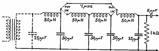
Fig. 7—Timing-pulse delay filter.
