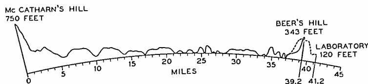
Fig. 2—Profile map of McCatharn's Hill-Beer's Hill path.
