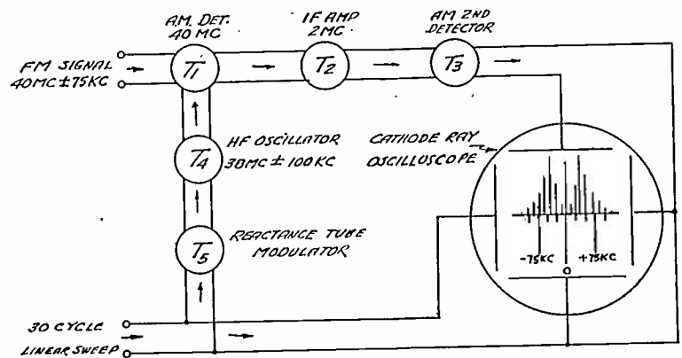
Fig. 2—Block diagram of monitoring system.
