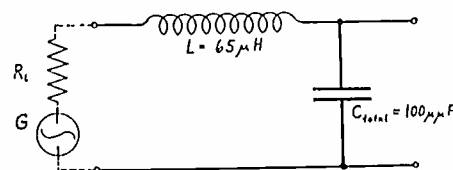
Fig. 21—Test object for time scale calibration.
