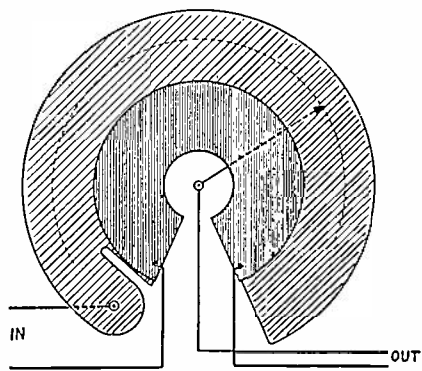
Fig. 11—Circular resistance strip as attenuator.
