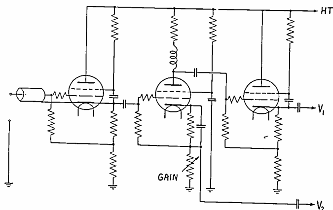
Fig. 13—Output amplifier circuit.
