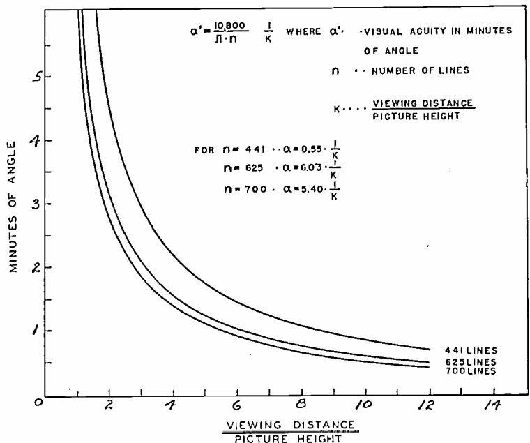
Fig. 1—Visual acuity versus ratio of viewing distance to picture height.
