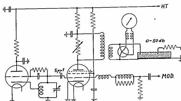
Fig. 9—Ultra-high-frequency oscillator, modulator, and attenuator.
