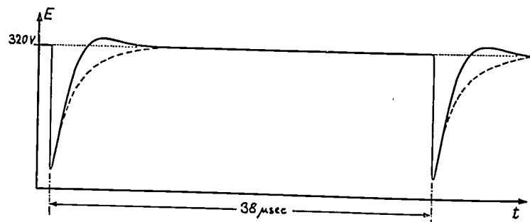
Fig. 4—Improvement of the saw-tooth shape through insertion of series inductances.
