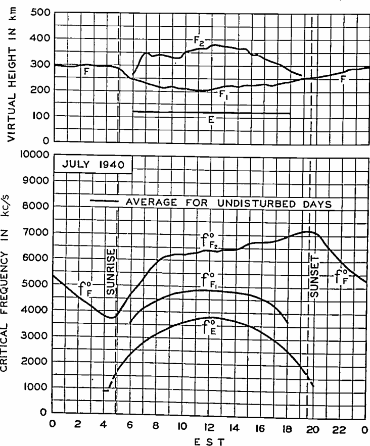
Fig. 1—Virtual heights and critical frequencies of the ionospheric layers, observed at Washington, D. C., July, 1940.
