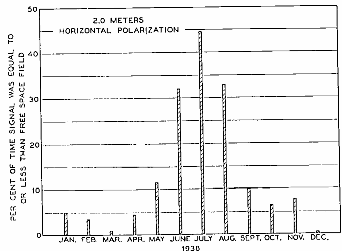
Fig. 13—Chart which shows the per cent of time that the signal was equal to or less than the free-space field for each month of 1938.
