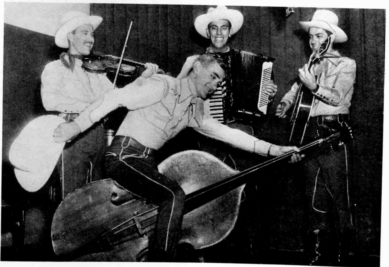
Fig. 16—Scanned picture (441 lines, 30 frames, 4.25 megacycles, \epsilon^{-x^2} aperture).
