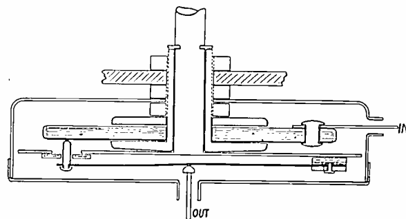
Fig. 12—Cross section through ultra-high-frequency attenuator.
