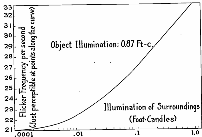
Fig. 3—Perceptible flicker frequency versus illumination of surroundings.
