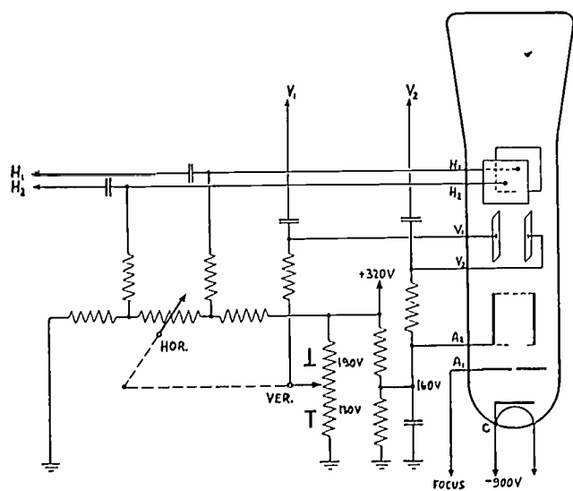
Fig. 5—Position-control circuit.
