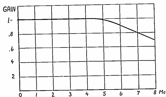
Fig. 15—Amplitude response of the output amplifier.
