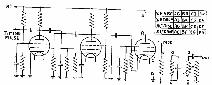
Fig. 8—Square-wave-generator circuit.
