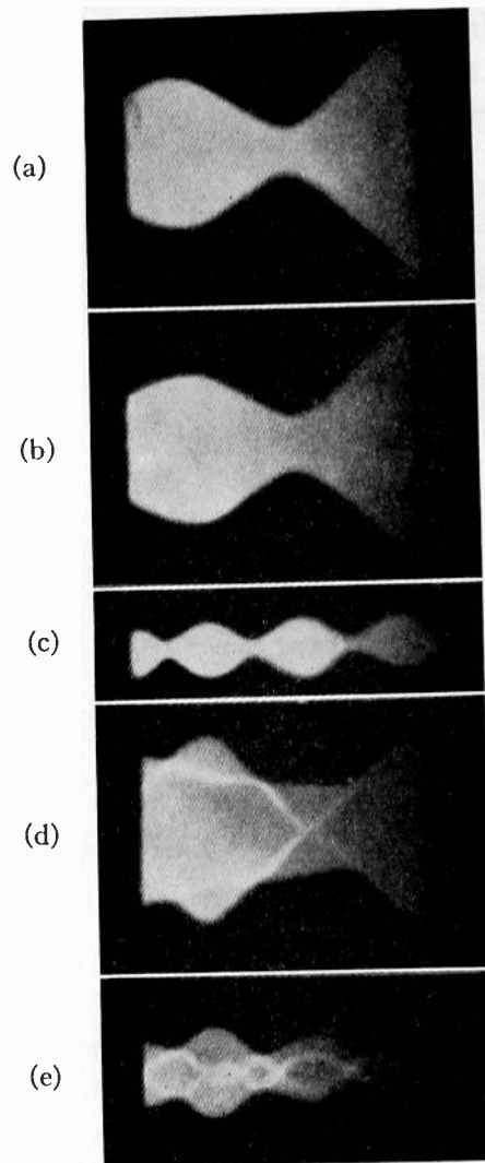
Fig. 6—(a) and (c) harmonic inversion spectra at 161 and 530 megacycles. (b) distorted spectrum with second harmonic. (d) and (e) double spectra.
