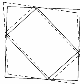
Fig. 2—Mode of motion of low-frequency shear crystals.
