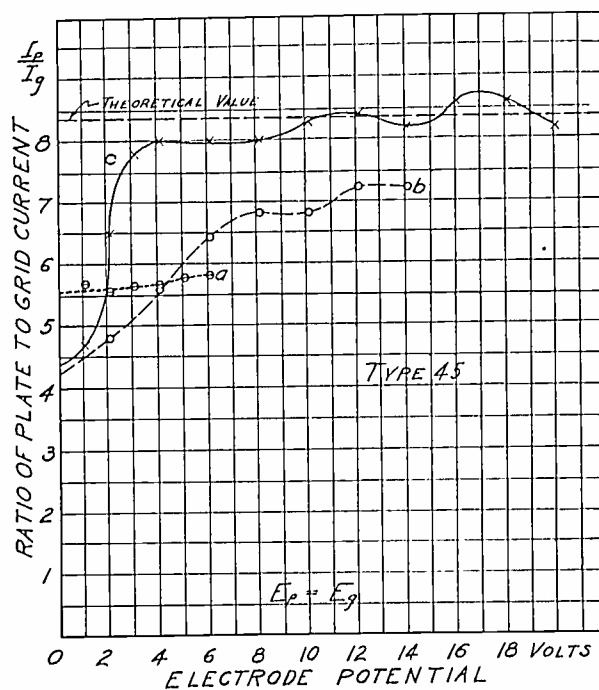
Fig. 7—Current-division factor in a 45 tube.
