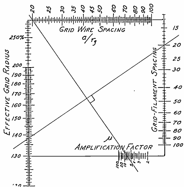
Fig. 4—Nomograph of effective grid radius.
