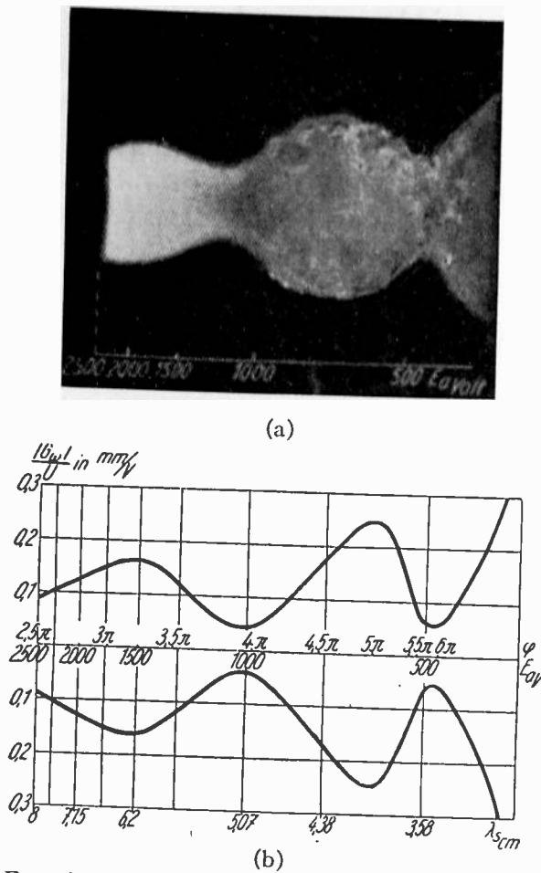
Fig. 3—Experimental and computed inversion spectrum of a harmonic ultra-high-frequency oscillation at 418 megacycles.
