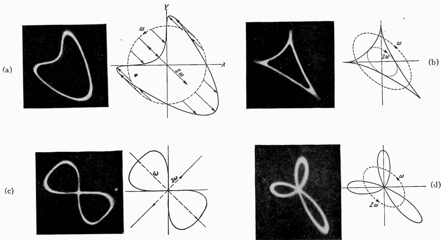
Fig. 11—Ultradynamic Lissajous figures containing the second harmonic.
