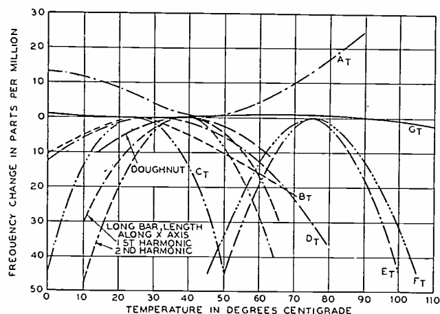
Fig. 1—Frequency-temperature relations for zero-temperature-coefficient crystals.
