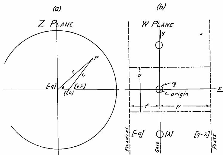
Fig. 1—Fundamental configuration of the plane triode.
