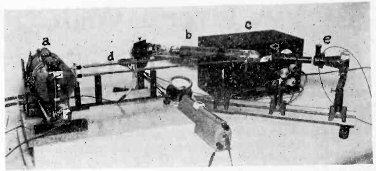
Fig. 16—Microwave oscillograph with magnetron generator. (a) Magnetron (c) Power pack (b) Microwave tube (d) Lecher wires (e) Microscope with eyepiece and camera.
