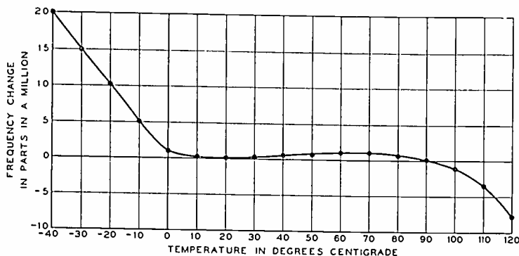
Fig. 6—Frequency-temperature curve for GT crystal.
