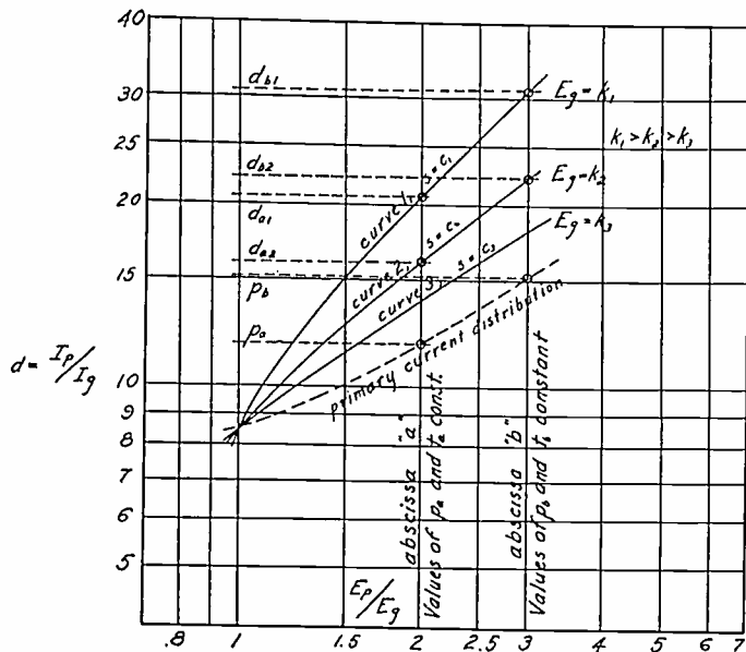
Fig. 9—Determination of primary-current distribution from current-division in the presence of secondary emission.
