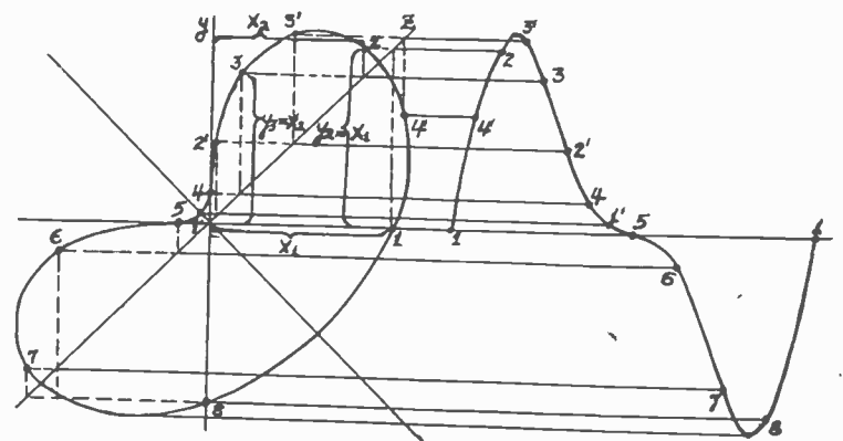
Fig. 10—Analysis of the transit-time figure of Fig. 8.
