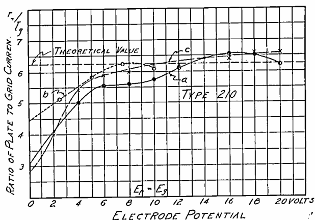
Fig. 6—Current-division factor in a 210 tube.
