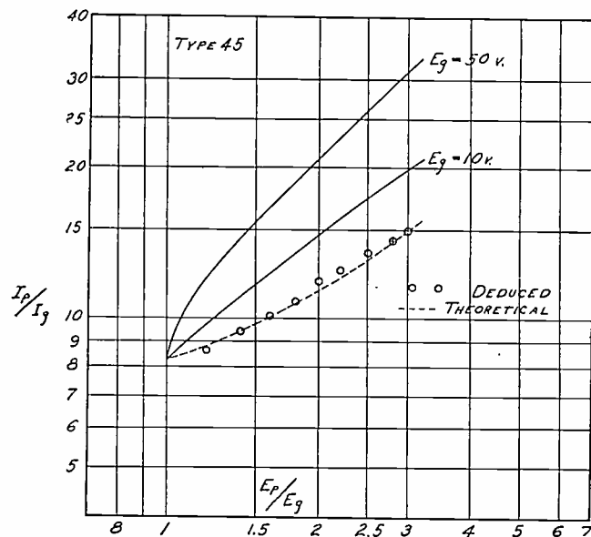
Fig. 8—Primary-current division in a 45 tube.
