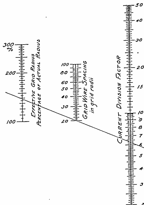
Fig. 5—Nomograph of current-division factor.
