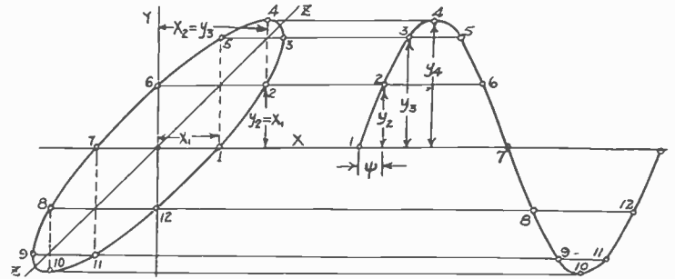
Fig. 9—Analysis of an ultradynamic ellipse.
