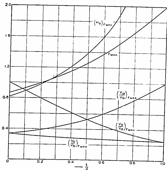
Fig. 5—Variation of the coefficient F_{max} with the ratio t/d ( t_0 be used in (15) for calculating maximum current), and of functions H_0 , V_a/V_b , V_0/V_b , V_0/V_a for the condition of maximum current.
