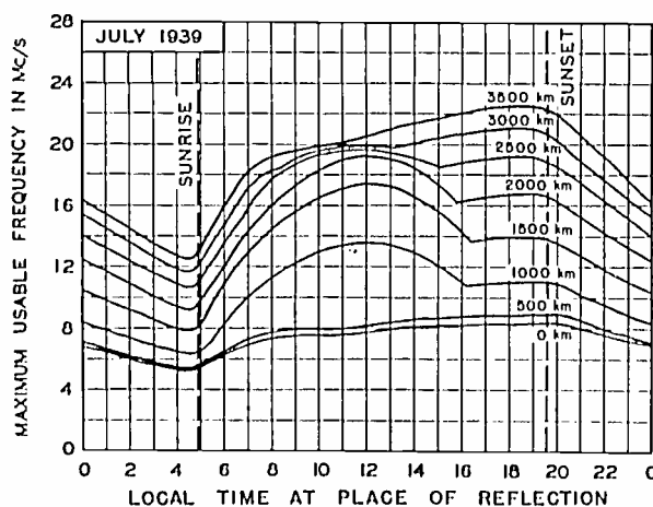
Fig. 2—Maximum usable frequencies for dependable radio transmission via the regular layers. Average for July, 1939, for undisturbed days. The values shown were considerably exceeded during irregular periods by reflections from clouds of sporadic E.
