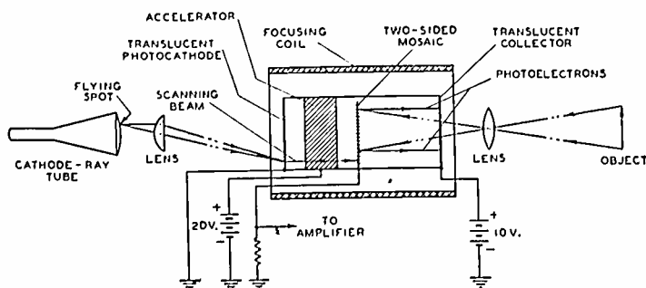
Fig. 5—Pickup tube using photoelectrons for scanning beam.
