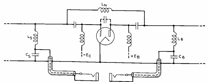
Fig. 6--Method of phase indication and tube neutralization.
