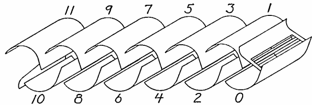
Fig. 6—Electrostatic electron multiplier.
