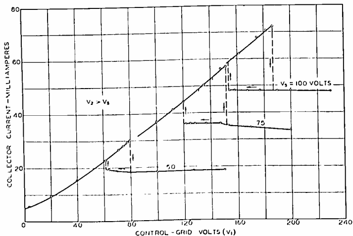
Fig. 31—Hysteresis loops in I_c versus V_1 characteristic ( H = \text{constant} ) of a short-beam tube.
