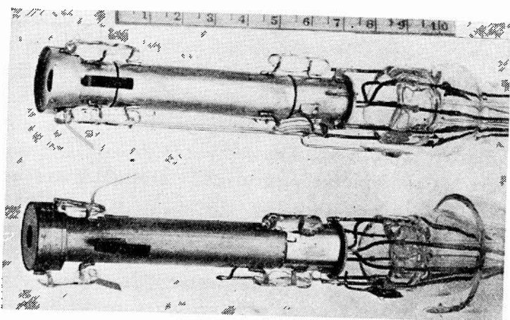
Fig. 4—Photograph of the old and new guns.
