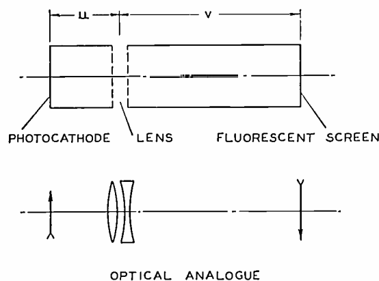
Fig. 4—Diagram of basic electrostatic-lens system.
