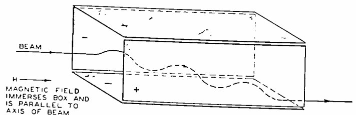
Fig. 8—Path taken by beam passing through rectangular electrostatic box.
