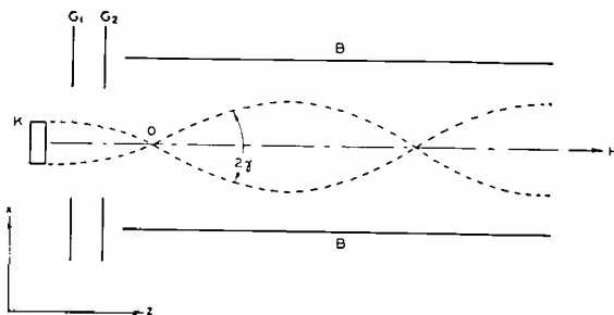
Fig. 10—Diverging beam entering the sheath electrode with a transverse velocity v_t = v_0 \sin \gamma .
