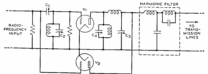
Fig. 5--Essentials of the high-efficiency circuit.
