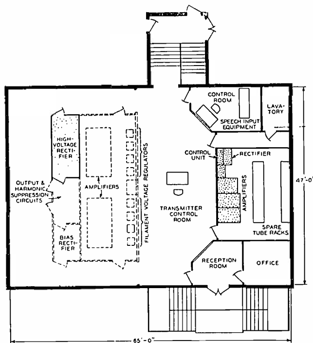
Fig. 1—First-floor plan.
