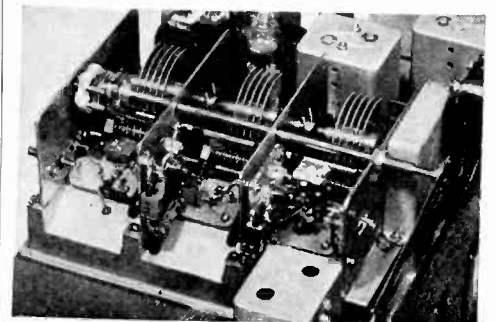
The radio-frequency tuning section of the NHU receiver
