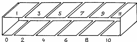
Fig. 5—Staggered multiplier with plane electrodes.
