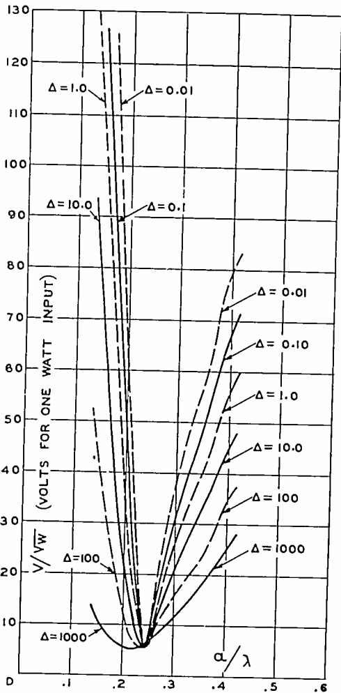
Fig. 3—Voltage on base insulator of sine-wave antenna.
