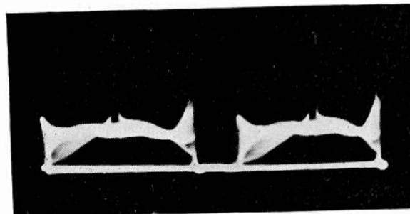
Fig. 8—Photograph of the signal as it appeared on the screen of the oscillograph tube when the oscillograph was synchronized to horizontal-line frequency. The sharp peak is the signal due to a rectangle of light on the iconoscope mosaic.
