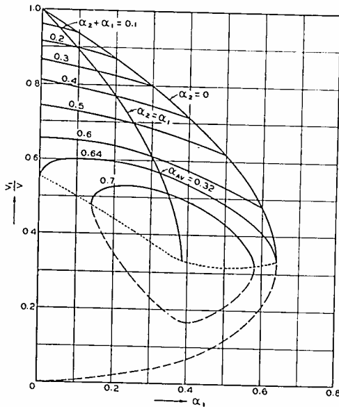
Fig. 23—Variation of space potential with current in the case of two thin beams for in-phase current modulation ( \alpha_1 = \alpha_2 = \alpha_0 ) and for 180-degree out-of-phase modulation ( \alpha_1 = \alpha_0 - \alpha_2 ).
