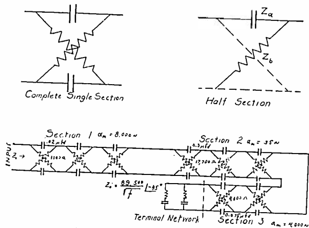
Fig. 1—45-degree network.
