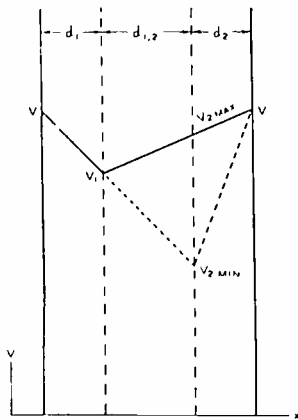
Fig. 18.—Limiting potential distributions for the case \lambda^2 = V_1/V = \text{constant} ; ( V - V_1 - V ) for I_2 = 0 , and ( V - V_1 - V_{2\text{min}} - V ) for I_1 = 0 .
