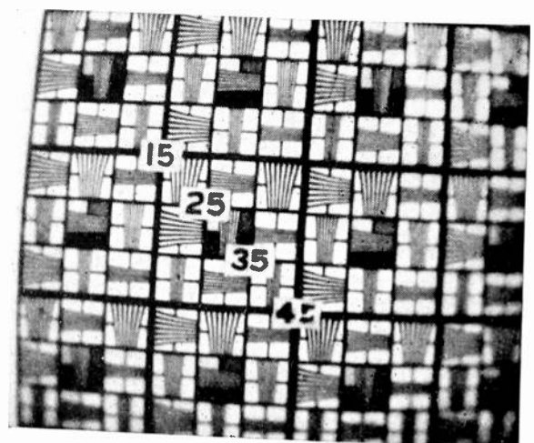
Fig. 8—Resolution pattern by magnetic-image tube.
