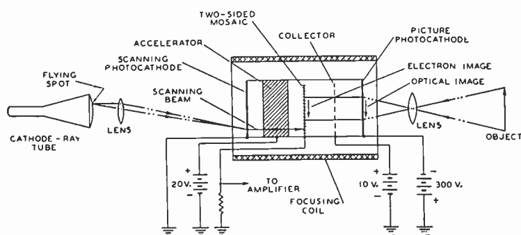
Fig. 10—Pickup tube using photoelectrons for scanning beam.
