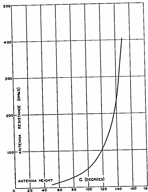
Fig. 1—Theoretical radiation-resistance curve.
