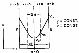
Fig. 2—Potential distribution in x, y plane for z = \text{constant} , y = \text{constant} .
