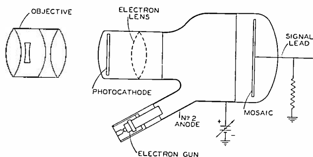
Fig. 2—Schematic diagram of image iconoscope.
