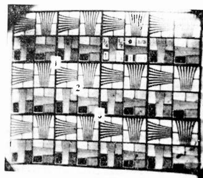
Fig. 13—Resolution pattern reproduced by electrostatic-image iconoscope.
