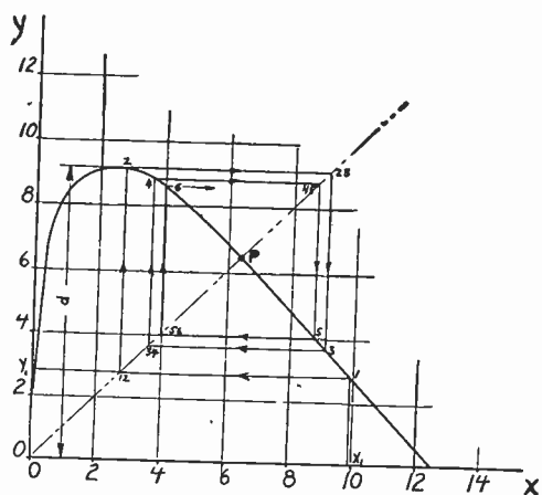
Fig. 8—Focusing curve.
