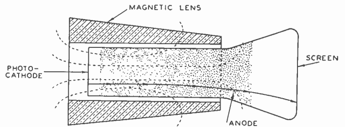
Fig. 7—Magnetic-image tube.
