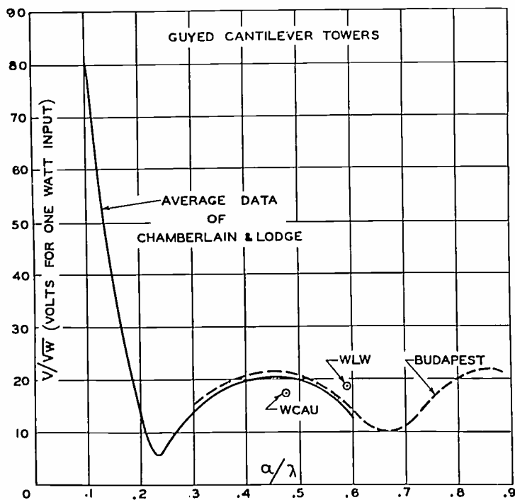
Fig. 5—Voltage on base insulator of guyed cantilever towers. The Budapest antenna is 1000 feet tall while WLW, Cincinnati, is 830 feet in height. The WCAU, Philadelphia, antenna is a guyed cantilever tower, 400 feet tall, and top-loaded with a capacitance-inductance hat.
