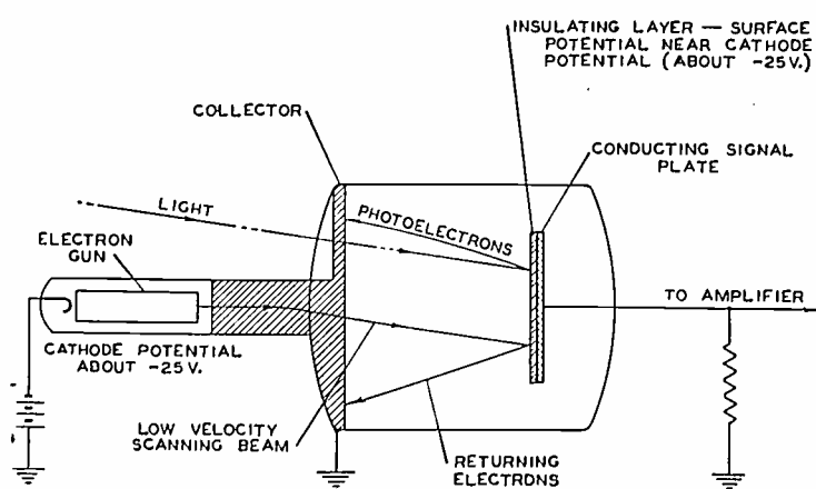
Fig. 2—Pickup tube using low-velocity electron beam for scanning.
