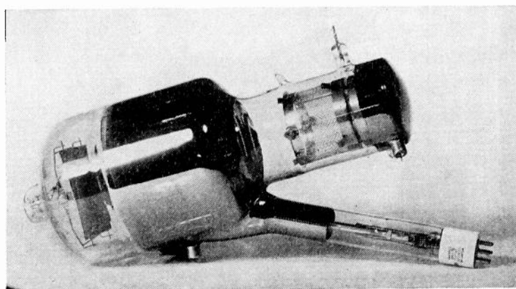
Fig. 10—Photograph of electrostatic-image iconoscope.
