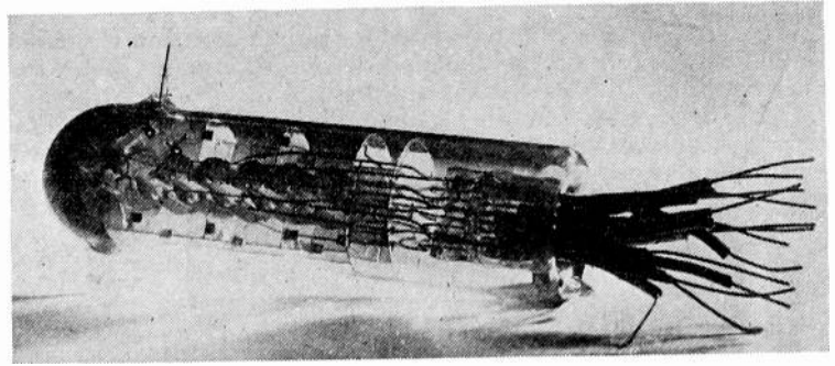
Fig. 12—Photograph of partition-type multiplier.
