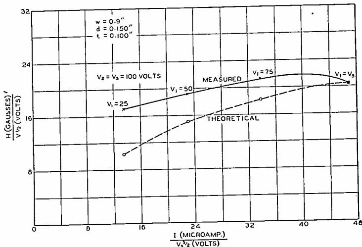
Fig. 32—Comparison between the theoretical and experimentally determined value of the minimum magnetic field.
