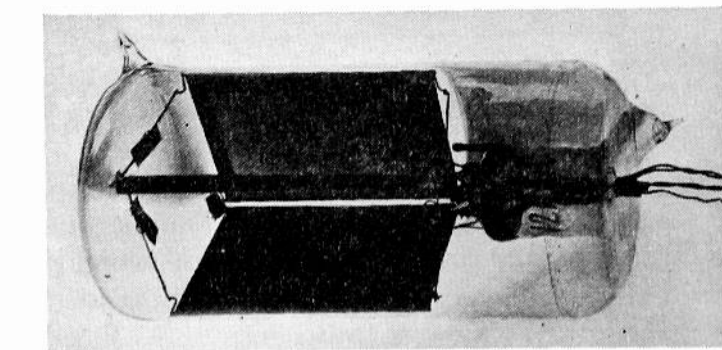
Fig. 12—Photograph of tube illustrated in Fig. 6.
