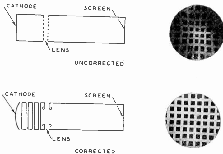
Fig. 5—Corrected and uncorrected electrostatic-lens system.
