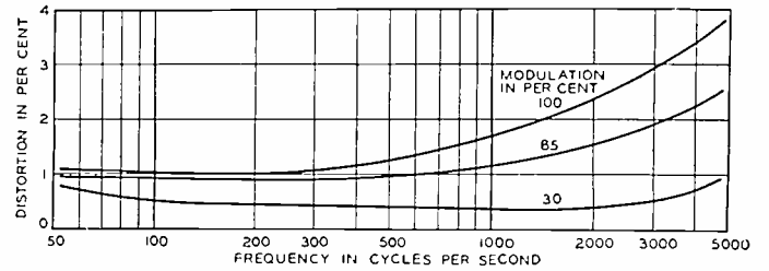
Fig. 4--Distortion measurements at 50 kilowatts.
