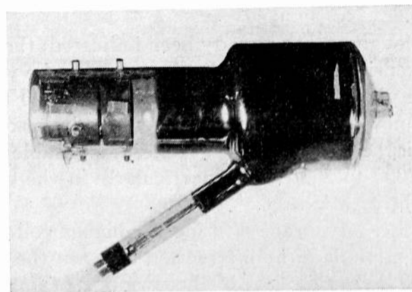
Fig. 11—Photograph of electrostatic-image iconoscope.
