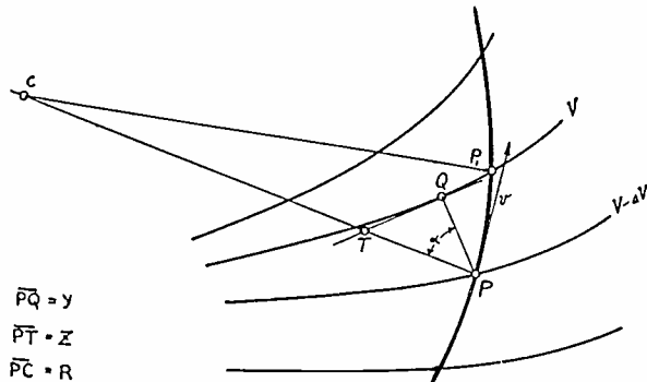
Fig. 1—The circle method.
