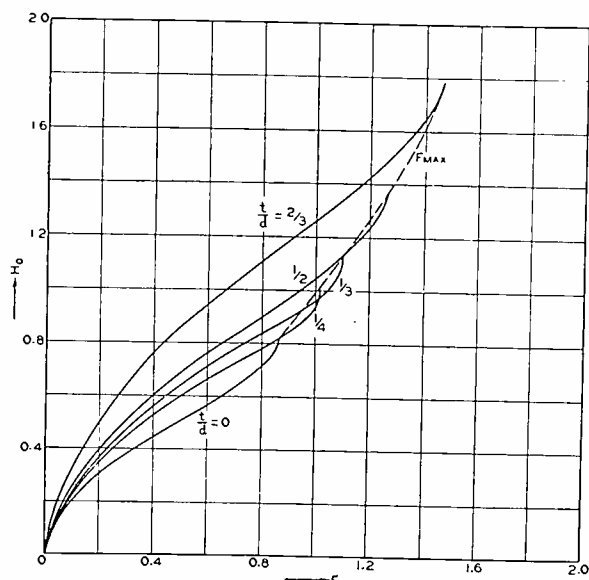
Fig. 9—Variation of the coefficient H_0 (equation (21)) with F (equation (16)) for different values of t/d .
