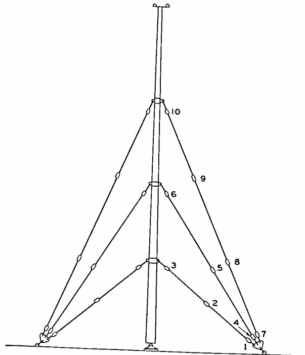
Fig. 19—Guy-insulator distribution for the tubular mast.
