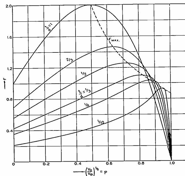
Fig. 3—Variation of function F with the ratio p = (V_0/V_a)^{1/2} for different values of the ratio of beam thickness l to the opening d of the sheath electrode.
