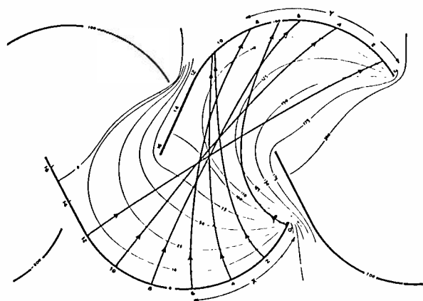
Fig. 7—Electron paths in the electrostatic multiplier.
