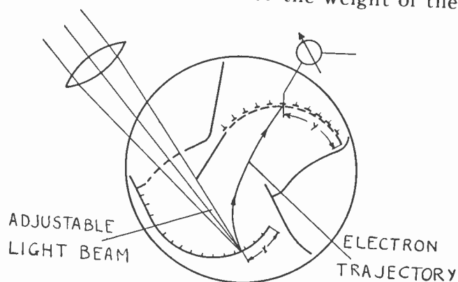
Fig. 3—Test tube.
