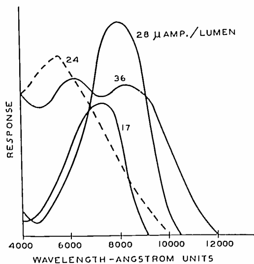
Fig. 3—Spectral response of semitransparent photocathodes.
