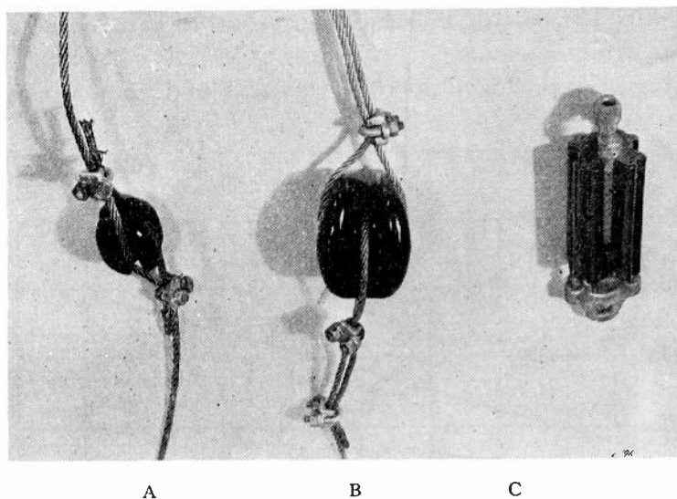
Fig. 20—Insulators suitable for sectionalizing guy wires.
