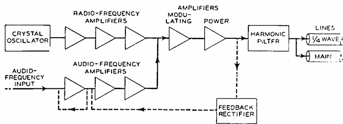
Fig. 3--Block diagram of amplifier circuits.
