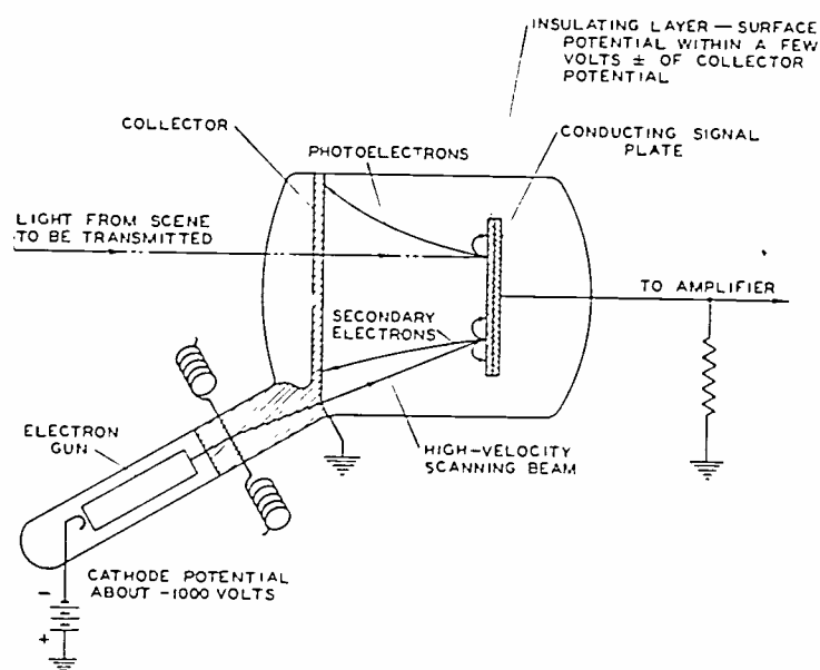
Fig. 1—Pickup tube using high-velocity electron beam for scanning.
