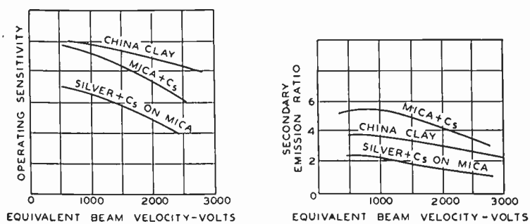
Fig. 9—Properties of various mosaics.
