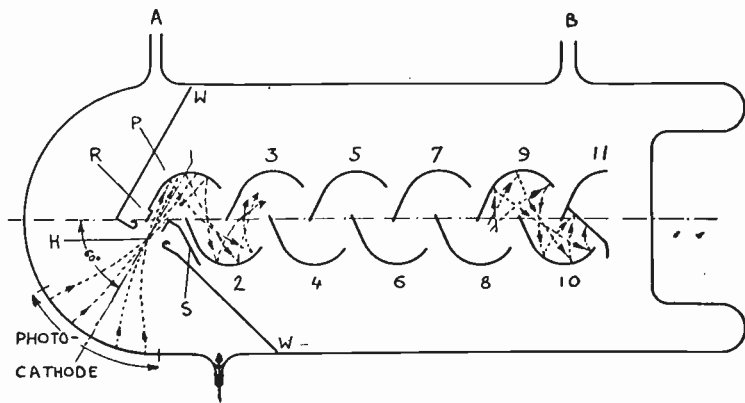
Fig. 11—Partition-type electron multiplier.
