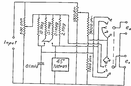
Fig. 3—Wiring diagram of amplifier tester.
