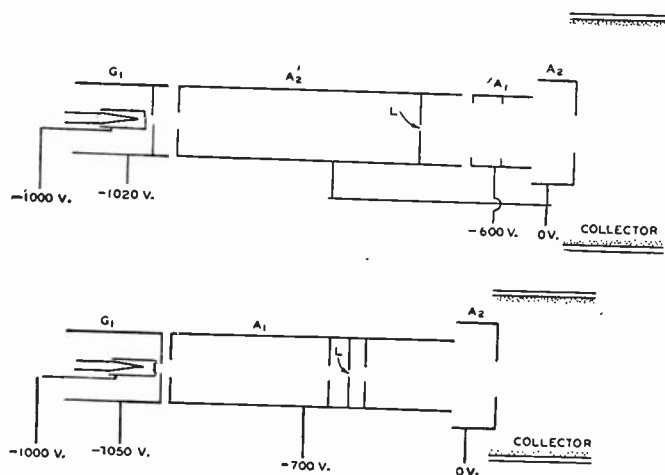
Fig. 3—Schematic drawings of the old and new guns. The older type is shown at the bottom, the newer at the top.
