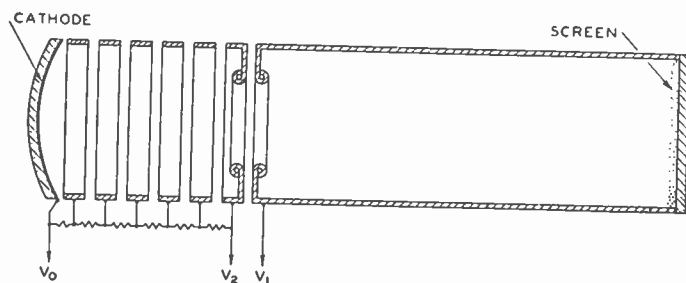
Fig. 6—Electrostatic-image tube.
