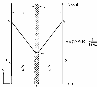
Fig. 12—Potential distribution in x, y plane for the case of a thin beam ( t/d \ll 1 ).
