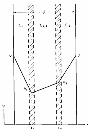
Fig. 17—Potential distribution for the case of two thin beams inside a common sheath electrode at a potential V .
