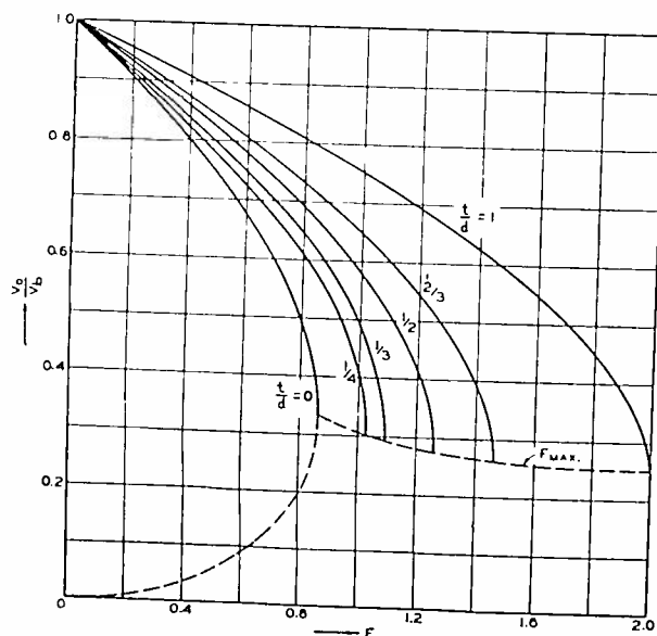
Fig. 6—The variation of the minimum space potential ( V_0 ) with the generalized current F (equation (16)) for different values of t/d .
