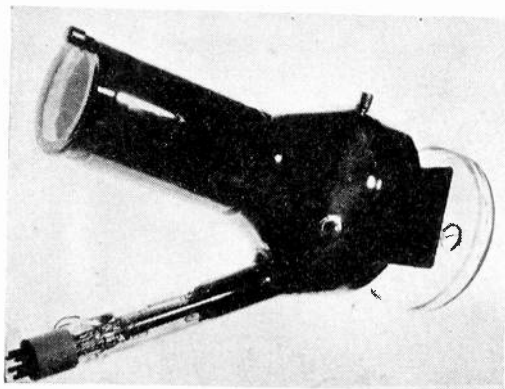
Fig. 12—Magnetic-image iconoscope.
