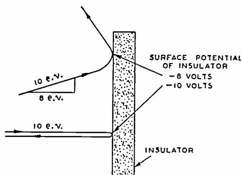
Fig. 4—Electron paths near target.
