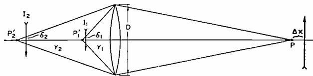
Fig. 1—Depth of focus in the object field.
