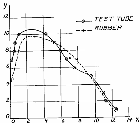
Fig. 4—Comparative focusing curves.
