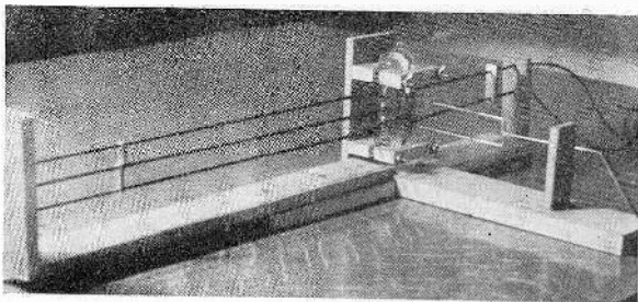
Fig. 1—Barkhausen tube and its circuit.
