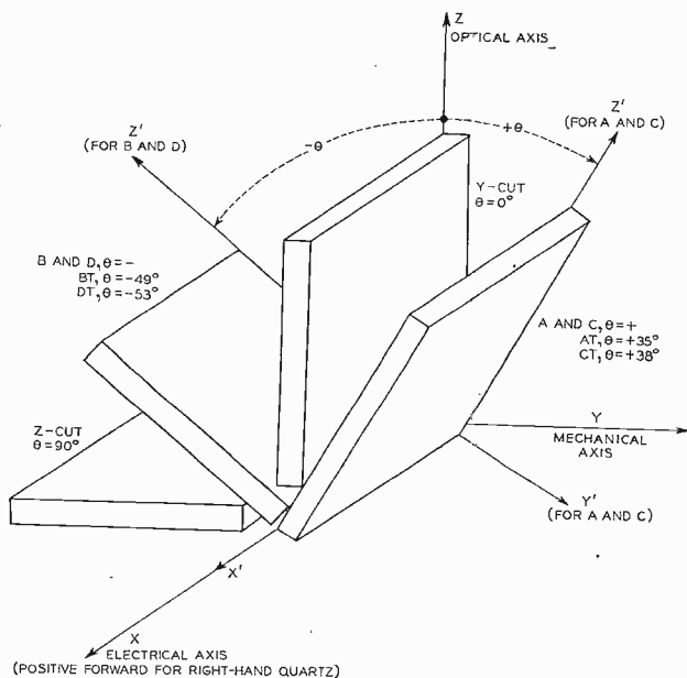
Fig. 2—The standard notation for describing the orientation of various cuts. A and B signify plates operated in the high-frequency shear mode, C and D signify low-frequency shear mode, T appended signifies zero-temperature coefficient of frequency.
