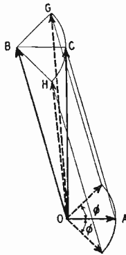
Fig. 5—Vector diagram of radio-frequency currents with frequency modulation.
