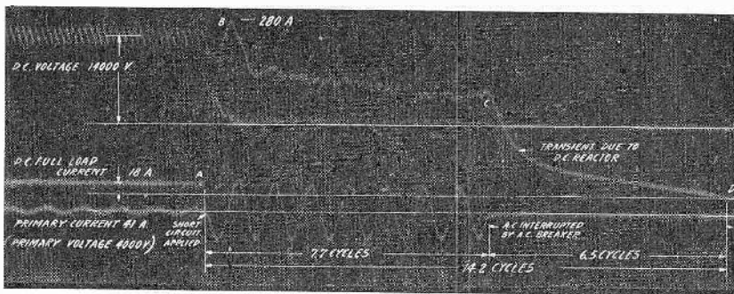
Fig. 11—Oscillographic record of interruption of a short circuit by an alternating-current circuit breaker.
