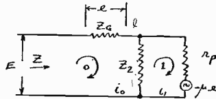
Fig. 2—Equivalent network of impedance seen from crystal.
