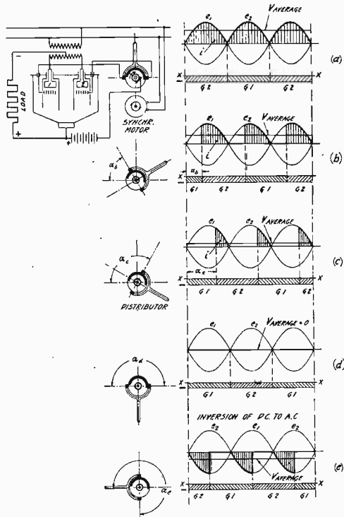
Fig. 1—Principle of operation of phase-shift control in a single-phase rectifier.
