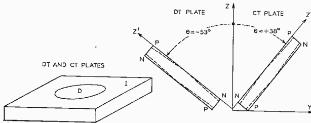
Fig. 7—An advantage of the CT and DT plates, for precision installations, is that the frequency may be finally adjusted in either direction—by grinding in regions D to decrease, and I to increase, the frequency. Further the temperature coefficient may be finally adjusted by grinding in regions P for a more positive value and N for a more negative value.
