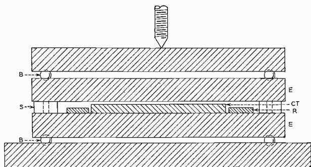
Fig. 10—The special holder for the CT plate as used in the frequency substandard. The plate is loosely retained between spaced electrodes E by a peripheral retainer R , the lower electrode being slightly convex to support the crystal nodally. The three isolantite spacers S and the steel clamping balls B are aligned to reduce warping strains in the electrodes.
