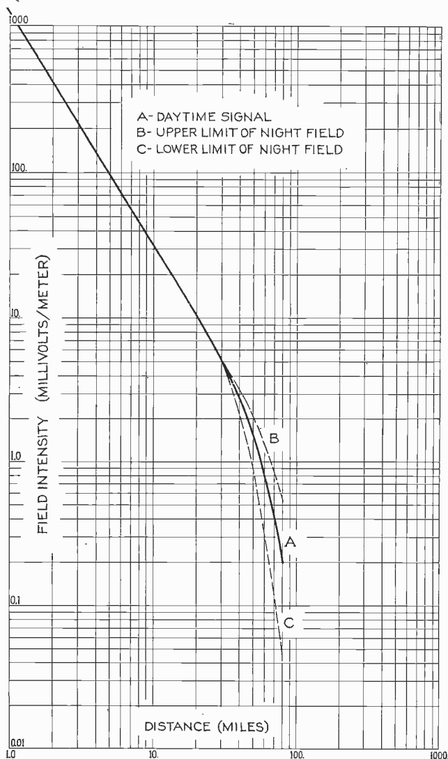
Fig. 33—Field strength along the northern radial, with the modified hat.
