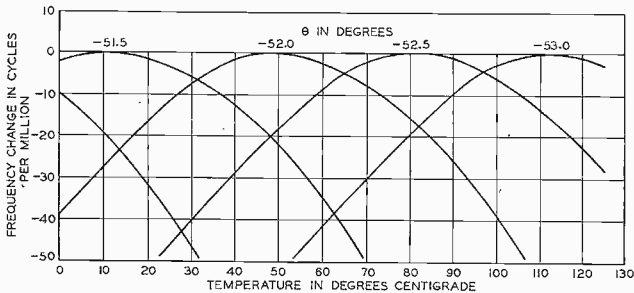
Fig. 6—The same representation for the DT plate as in Fig. 5. It is to be noted that, for the DT plate, the frequency varies less than one cycle in a million from its mean value over a range of twenty-five degrees centigrade.
