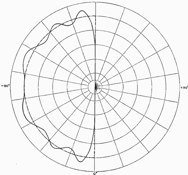
Fig. 3—Directional pattern, illustration 1.
