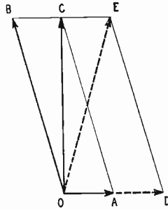
Fig. 4—Vector diagram of radio-frequency currents with amplitude modulation.
