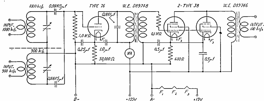
Fig. 3—Circuit arrangement of 100-kilocycle detector-amplifier.
