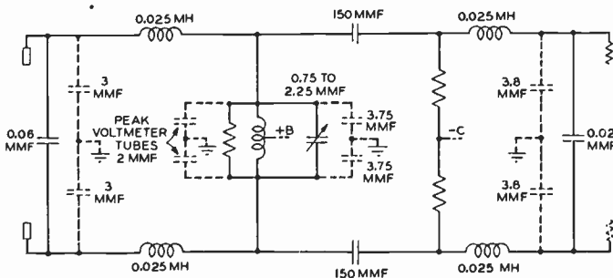
Fig. 13—Diagram of interstage circuit.
