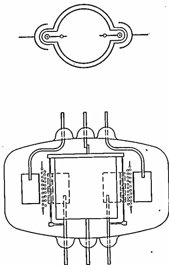
Fig. 4—Sectional view of the double pentode tube.
