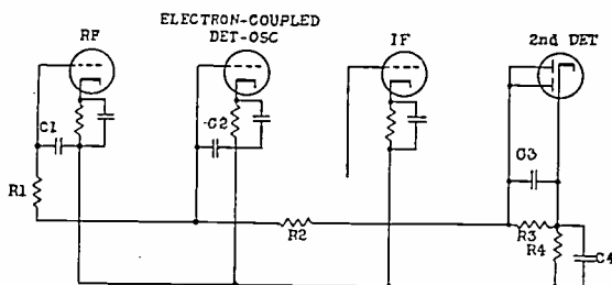
Fig. 3—Skeleton automatic volume control circuit.
