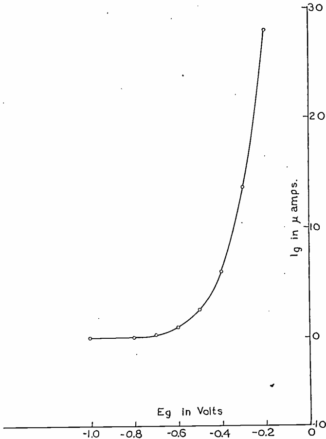
Fig. 2—Grid current vs. grid voltage curve for type 75.
