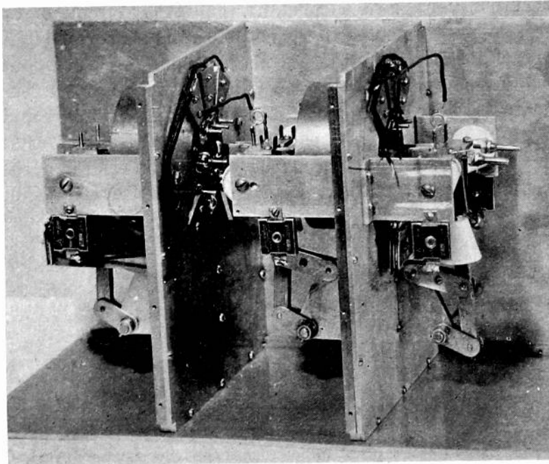
Fig. 12—An experimental two-stage one-meter amplifier using two of the earlier type push-pull pentode tubes.
