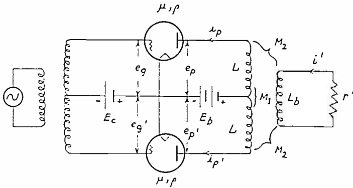
Fig. 2.— r = (L/L_b)r' ; i = \sqrt{L_b/L} i' ; c_g = -E_c + E \cos \theta ; c_g' = -E_c - E \cos \theta ; L_2 = L - M_2^2/L_b ; L_1 = L - M_1 .
