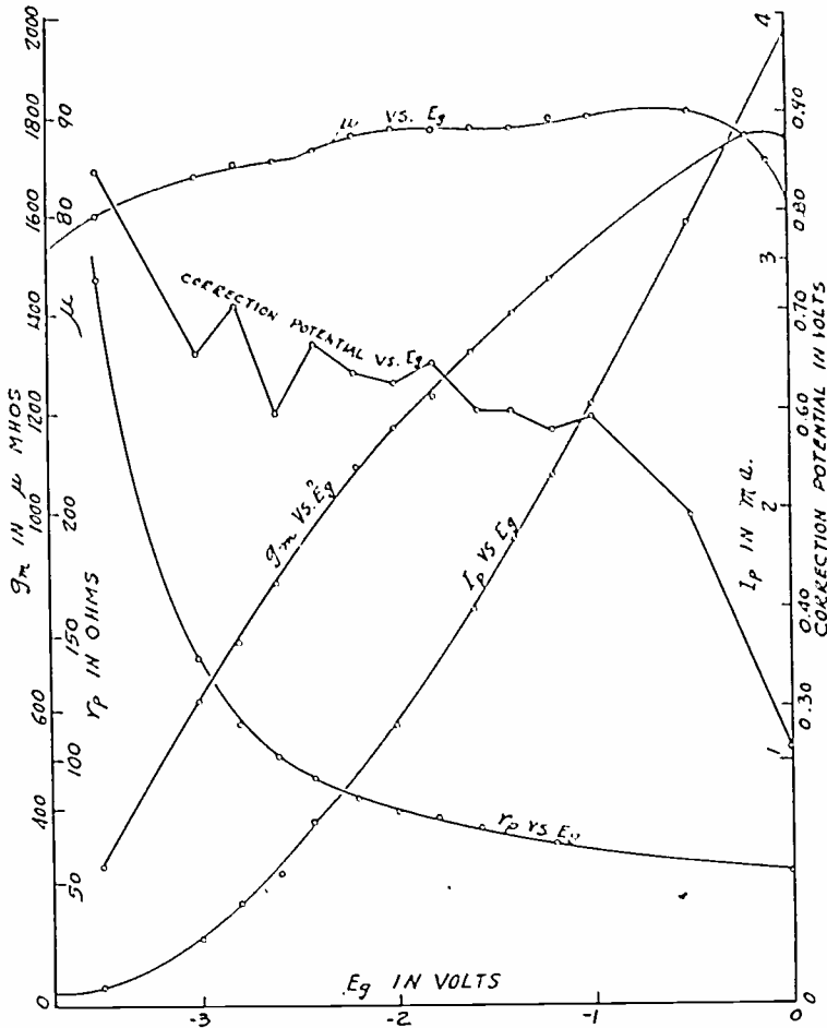
Fig. 6—Triode grid correction potential vs. grid voltage. Triode amplification factor vs. grid voltage. Triode mutual conductors vs. grid voltage. Triode plate current vs. grid voltage. Triode plate resistance vs. grid voltage. Type 75 E_h = 6.3 volts E_p = 250 volts
