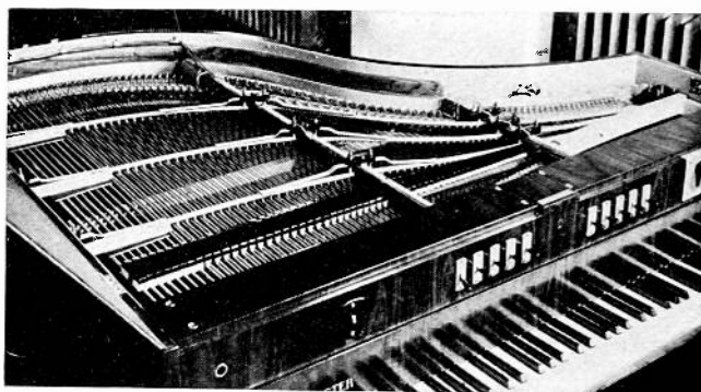
Fig. 12—Internal view of the Vierling-Forster piano.
