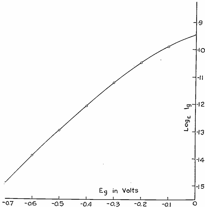
Fig. 4— \text{Log}_{10} grid current vs. grid voltage curve for type 75. E_h = 6.3 volts E_p = 250 volts
