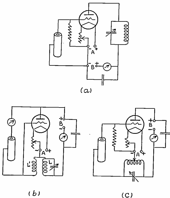
Fig. 2—Driving circuits for oscillations.
