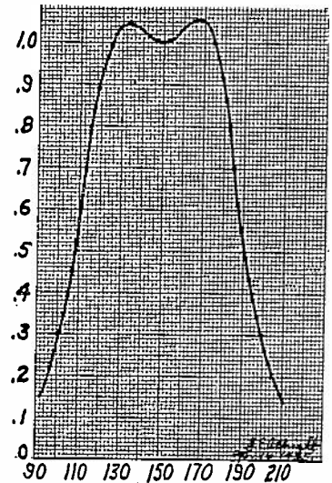
Fig. 4—Selectivity of broad amplifier.
