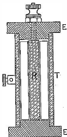
Fig. 1.—The holder for cylindrical quartz oscillator.
