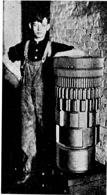
Fig. 2—Cahill magnetolectric tone generator unit comprising fundamental and seven overtones.
