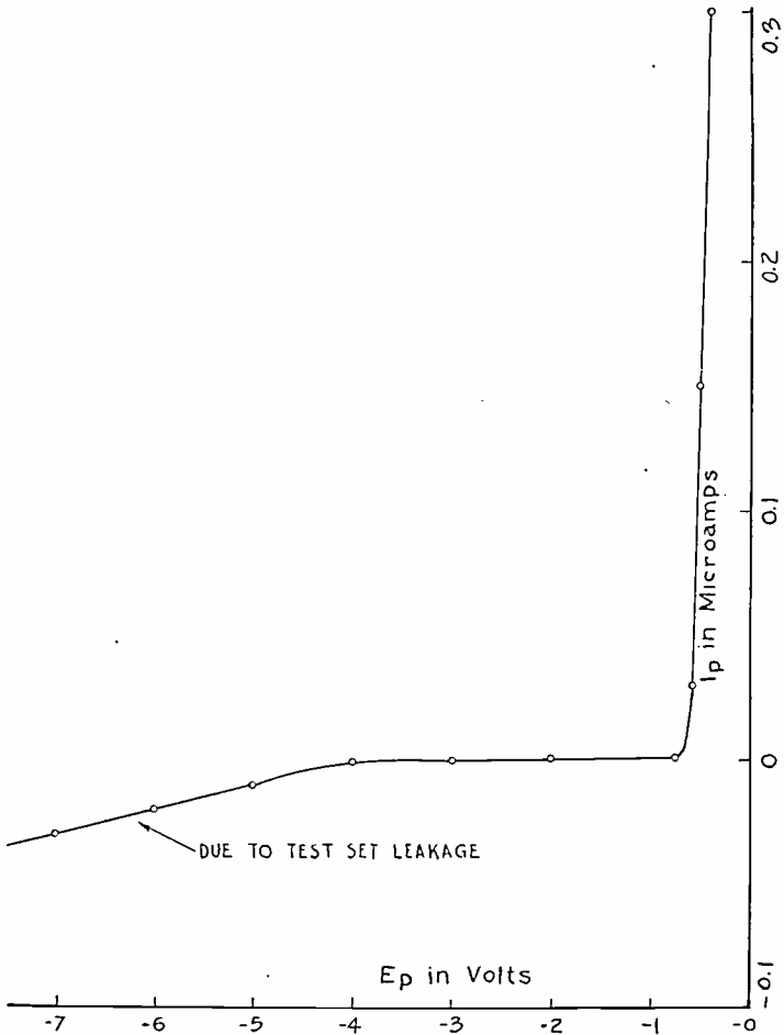
Fig. 1—Diode plate current vs. plate voltage for type 75. E_a = 6.3 volts
