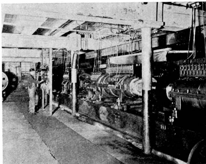
Fig. 3—Section of a generator room of the Telharmonium.
