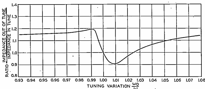
Fig. 15—Reaction Curve.
