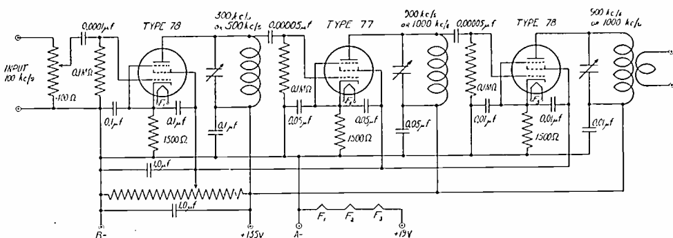
Fig. 2—Circuit arrangement of harmonic amplifiers.
