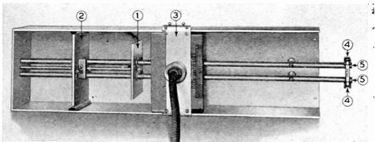
Fig. 14—Photograph of impedance measuring Lecher frame.
