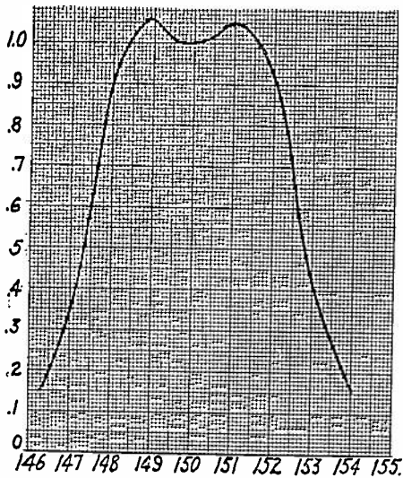
Fig. 3—Selectivity of sharp amplifier.
