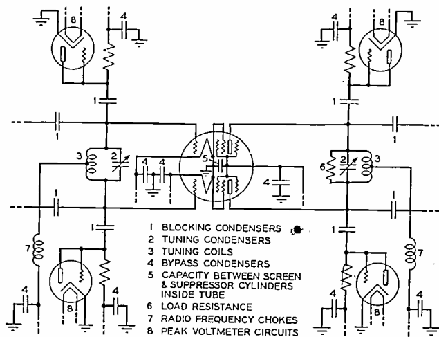
Fig. 11—Circuit diagram of single stage test amplifier.
