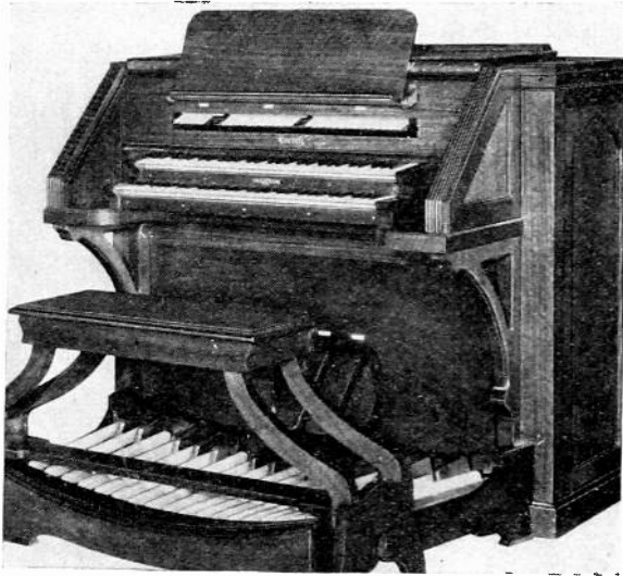
Fig. 14—Everett Orgatron Model MD-1, using wind-blown Harmonium reeds with electrostatic pickup.
