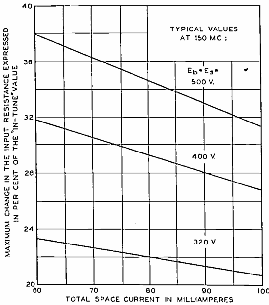
Fig. 10—The input-output reaction at 150 megacycles.
