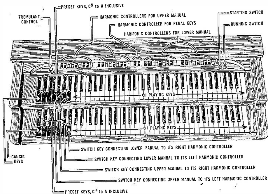
Fig. 8—Plan view of the Hammond organ console.
