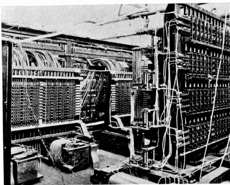
Fig. 4—Telharmonium. Close-up view of wiring.
