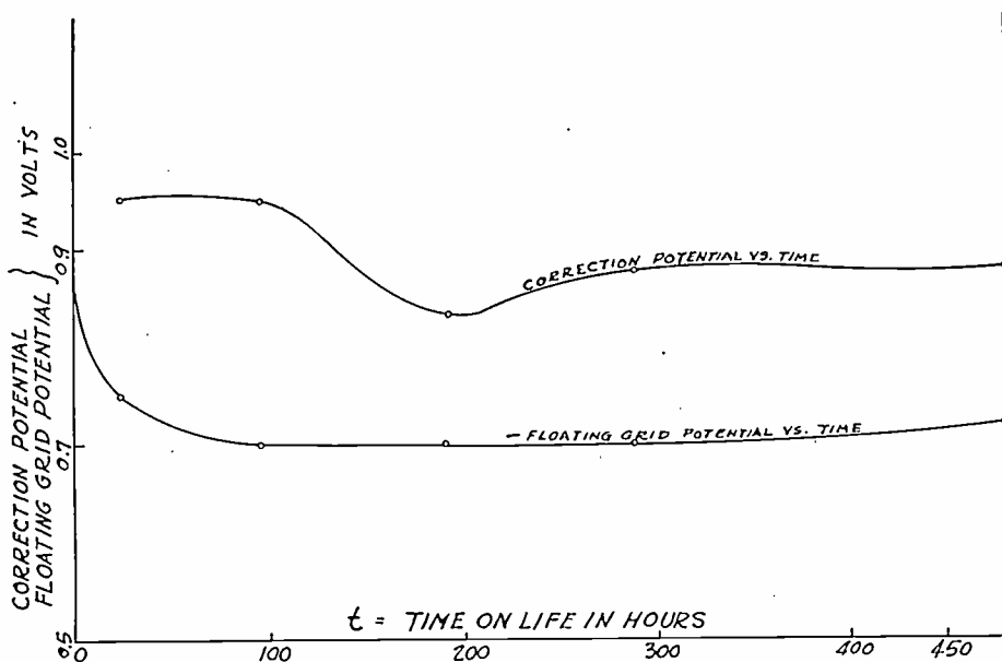
Fig. 8—Triode grid correction potential vs. time of life. Negative floating grid potential vs. time of life. Type 75 E_h = 6.3 volts E_p = 250 volts
