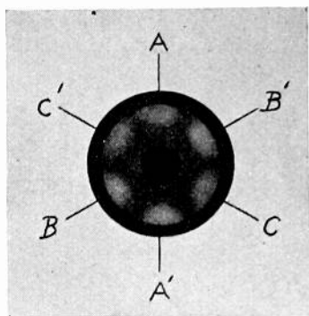
Fig. 3—Radial vibration, examined under polarized light.
