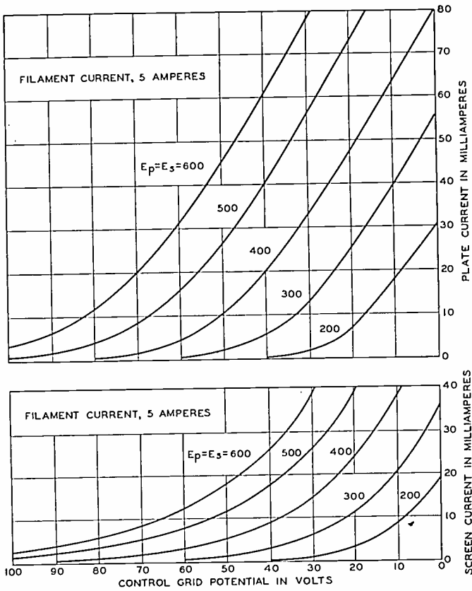
Fig. 6—Mutual characteristics of the double pentode tube.
