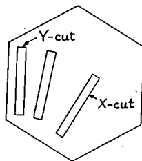
Fig. 6—Trial cutting to find the plate of zero temperature coefficient in the intermediate orientation between X- and Y-cut plates.
