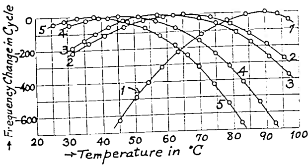
Fig. 12—Frequency temperature relation at \phi = 138^\circ . Numerals correspond to those in Table IV.
