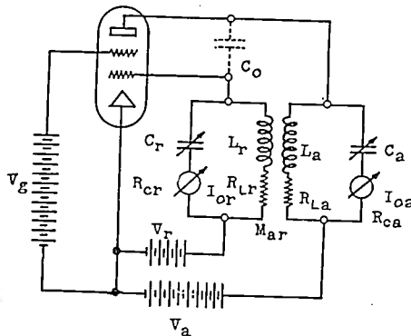
Fig. 1—Retroactive dynatron oscillator of the first kind.
