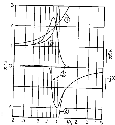
Fig. 5—Impedance characteristics of full-section filter built out of the output transformer. The scales are ratios as in Fig. 4. Curve 1 is the modulus of the transformer alone terminated in a constant resistance. Curve 2 is the resistance and reactance of an ideal filter section terminated in its iterative impedance. Curve 3 is the resistance and reactance of the actual network terminated in a constant pure resistance.
