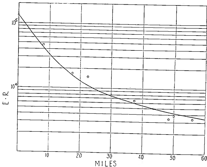
Fig. 2—WPHC, Massillon, Ohio. Transmission east. K\sqrt{P} = 130,000 , \sigma = 0.68 \times 10^{-13} , \lambda = 0.188 kilometer.
