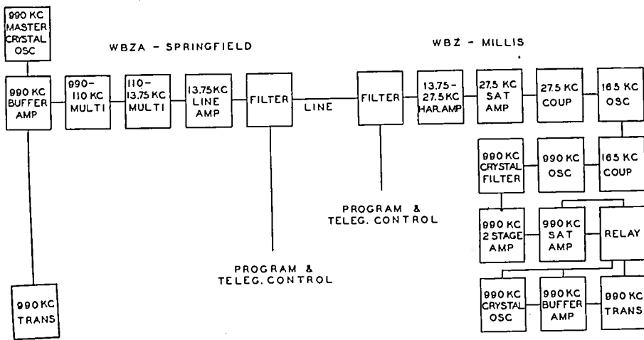
Fig. 2—Present WBZ-WBZA synchronizing system.
