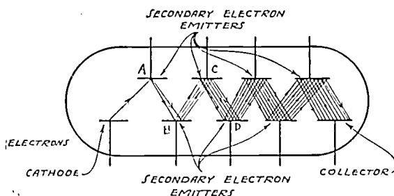
Fig. 1—Simplified secondary emission multiplier.
