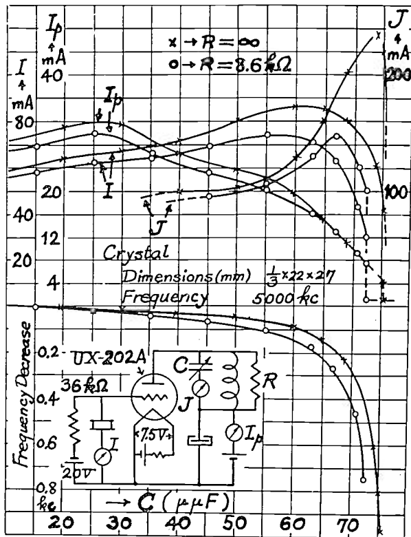
Fig. 13—Characteristics of triode crystal oscillator.
