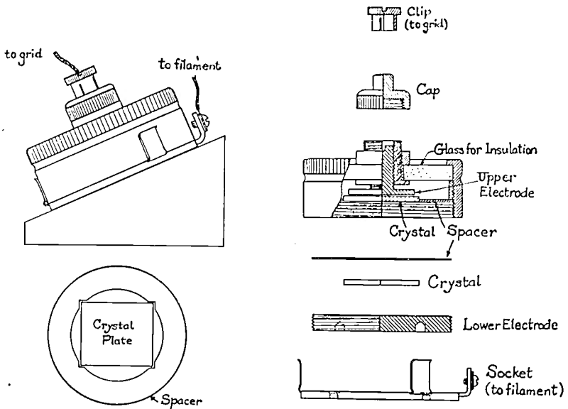
Fig. 16—Crystal holder.
