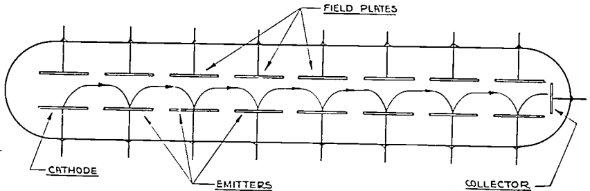
Fig. 5—Magnetic secondary emission multiplier.
