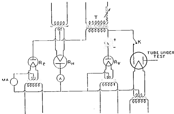
Fig. 1—Circuit for measurement of primary grid emission.
