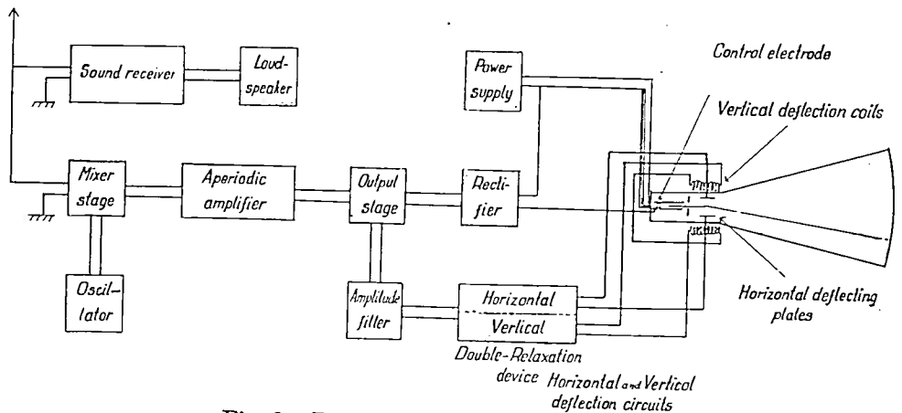
Fig. 2—Diagram of television receiver.
