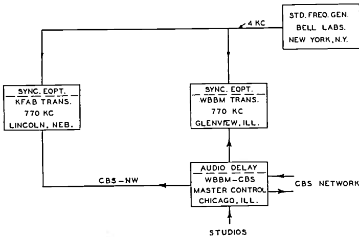
Fig. 4—WBBM-KFAB synchronizing system.
