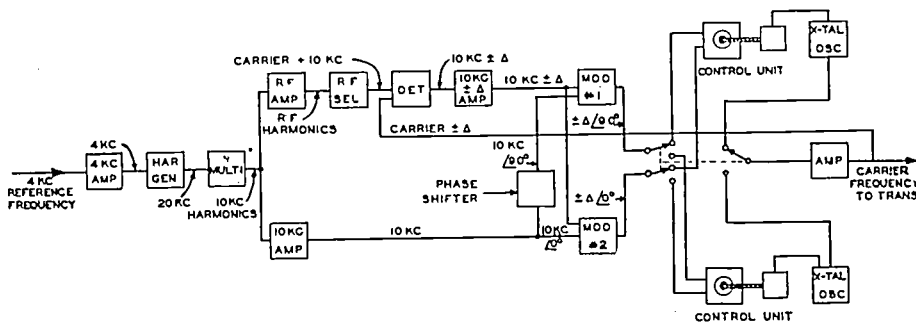
Fig. 3—Western Electric synchronizing equipment.
