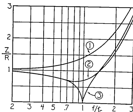
Fig. 4—Impedance characteristics of half-section filter built out of interstage transformer. The scales are reduced to ratios applicable to any particular transformer. Curve 1 is the modulus for a practical transformer without correction. Curve 2 is the actual modulus for the corrected network. Curve 3 is the characteristic of an ideal filter section terminated in its iterative impedance. (See footnote 7.)
