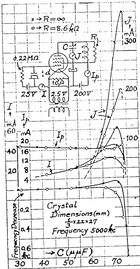
Fig. 14—Characteristics of pentode crystal oscillator.
