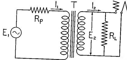
Fig. 6—Equivalent circuit of driver amplifier, showing only details necessary to the analysis given in the text.
