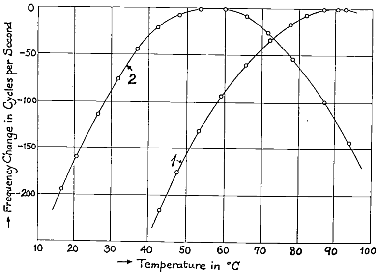
Fig. 21—Frequency temperature curve for the oscillator shown in Fig. 20.
