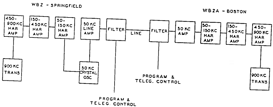
Fig. 1—Original WBZ-WBZA synchronizing system.
