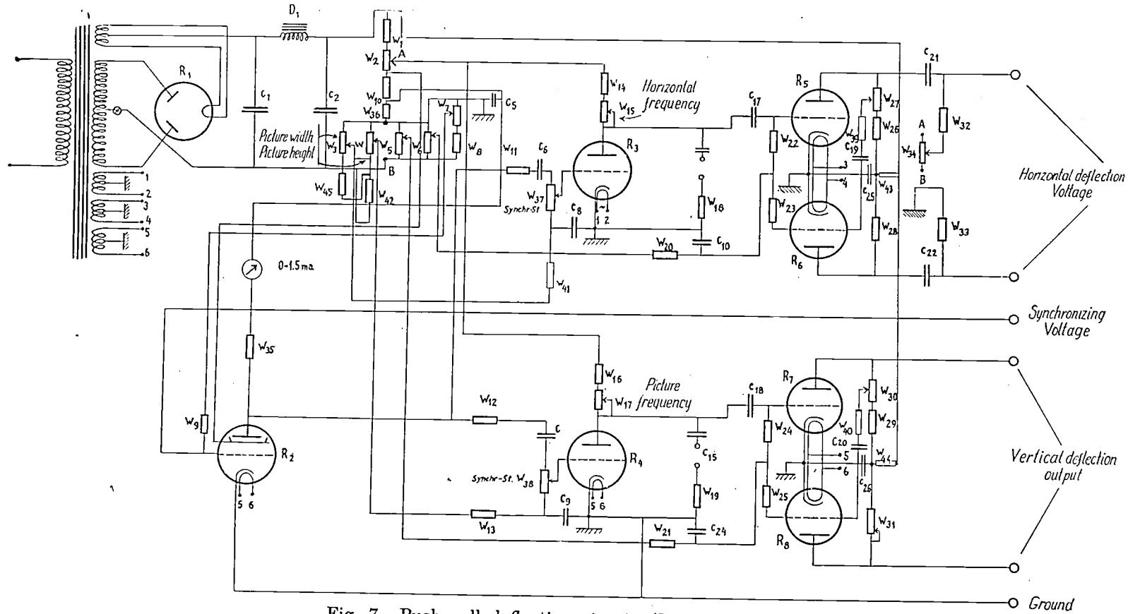
Fig. 7—Push-pull deflection circuit. (Type 1933/34.)
