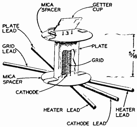
Fig. 2—Internal Structure of the triode.
