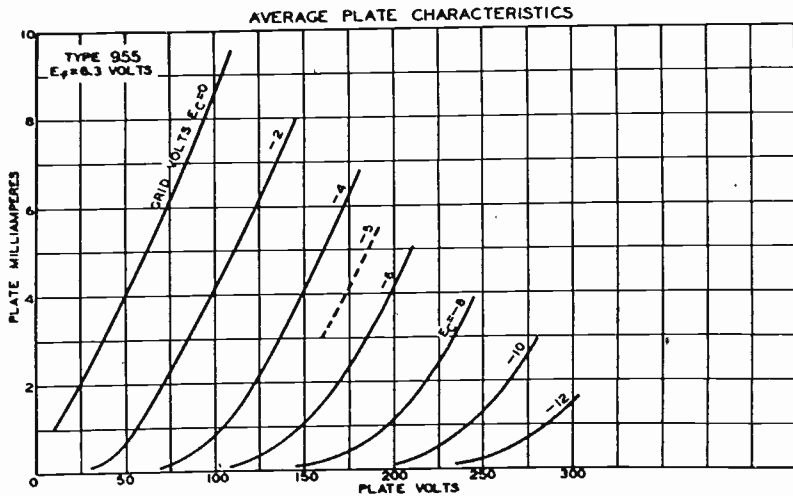
Fig. 5—A typical plate family for the triode.
