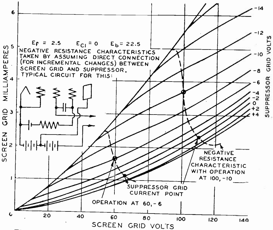
Fig. 7—Average RCA-57 used as negative transconductance tube.
