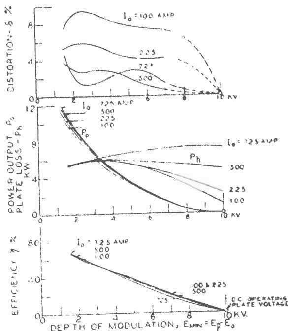
Fig. 15—Distortion as a function of modulation.
