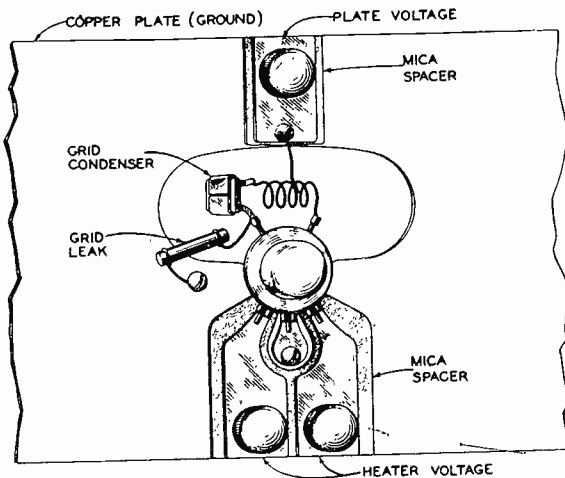
Fig. 11—A typical triode oscillator set-up.
