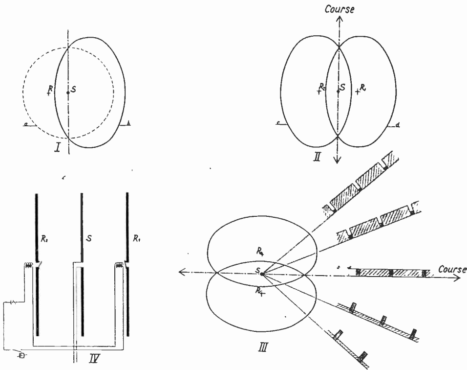
Fig. 1—Ultra-short-wave beacon.
