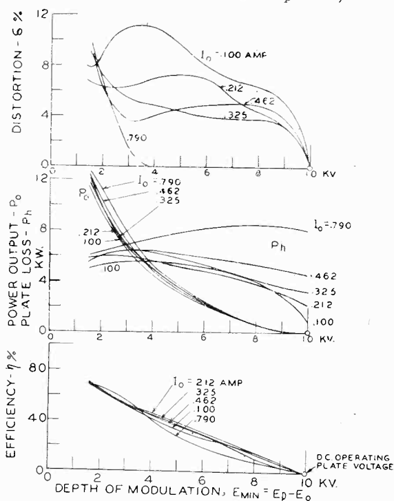
Fig. 14—Distortion as a function of modulation.
