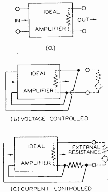
Fig. 1.—Ideal amplifier used to illustrate conception of negative resistance.
