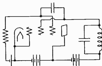
(a) VOLTAGE-CONTROLLED OSCILLATOR CIRCUIT
