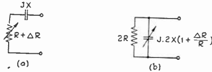
(a) and (b) are equivalent when R = X
