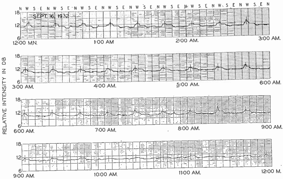
Fig. 1—Sample record of waves of interstellar origin. Record taken 12:00 midnight to 12:00 noon on September 16, 1932.
