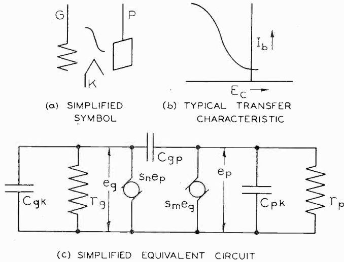
Fig. 4—Negative transconductance tube.
