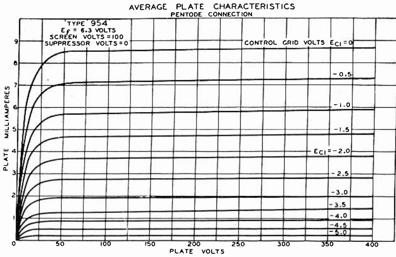
Fig. 6—A typical plate family for the pentode.
