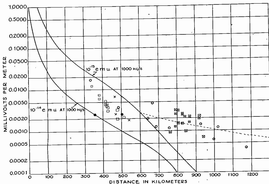
Fig. 4—Daytime field intensity measurements reduced to one kilowatt of radiated power and given as a function of distance for broadcast stations in the United States. The solid curves were taken from the Report of the United States Committee on Radio Propagation Data and are theoretical ground-wave formulas. The dotted curve represents an empirical formula for distances greater than 600 kilometers.
