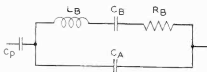
Fig. 1—Electrical representation of a piezoelectric crystal.
