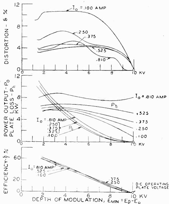
Fig. 16—Distortion as a function of modulation.
