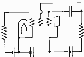
(b) CURRENT-CONTROLLED RELAXATION-OSCILLATOR CIRCUIT
