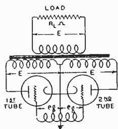
Fig. 10—Class B modulation scheme.
