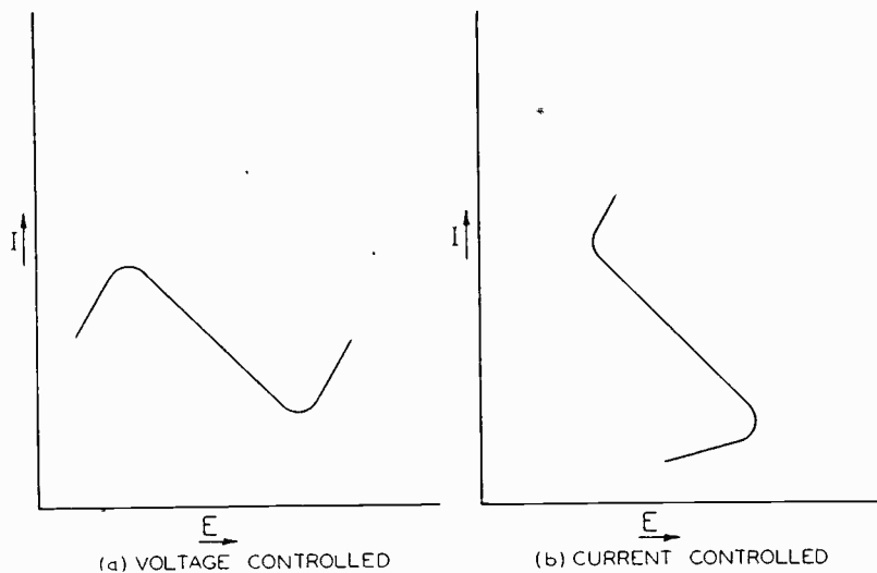
Fig. 2—Falling characteristics exhibited by negative resistance devices.
