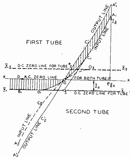
Fig. 8—Modulation characteristic for two tubes in push-pull.
