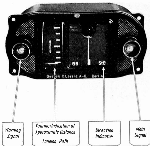
Fig. 9—Visual indicator assembly.
