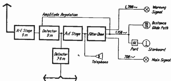
Fig. 10—Diagram of receiving circuits.
