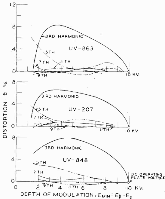
Fig. 7—Distribution of harmonic components.
