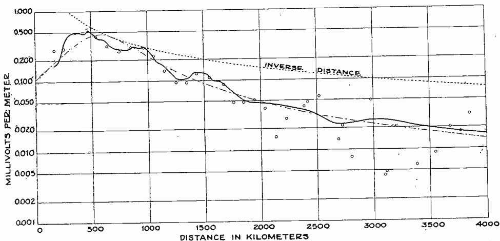
Fig. 6—Two averages of night field intensity measurements together with the graph of an empirical formula which was designed to represent the data.
