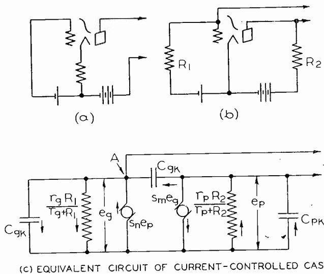
Fig. 6—Production of current controlled negative resistance.
