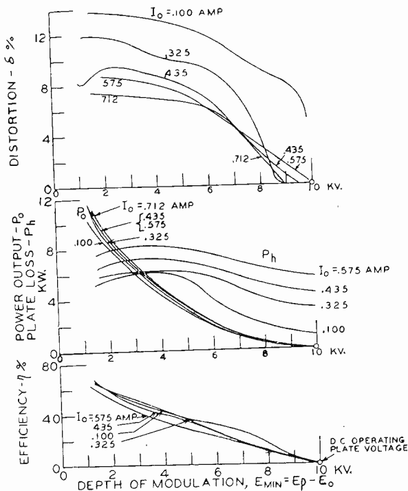
Fig. 17—Distortion as a function of modulation. WL-419A tube E_p = 10,000 volts R_L = 1680 ohms \mu = 3.6
