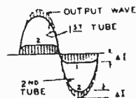
Fig. 11—Output wave.
