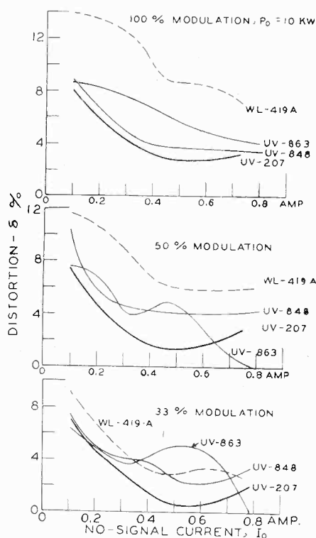
Fig. 18—Variation of distortion with no-signal current, I_o . E_p = 10,000 volts R_L = 1680 ohms
