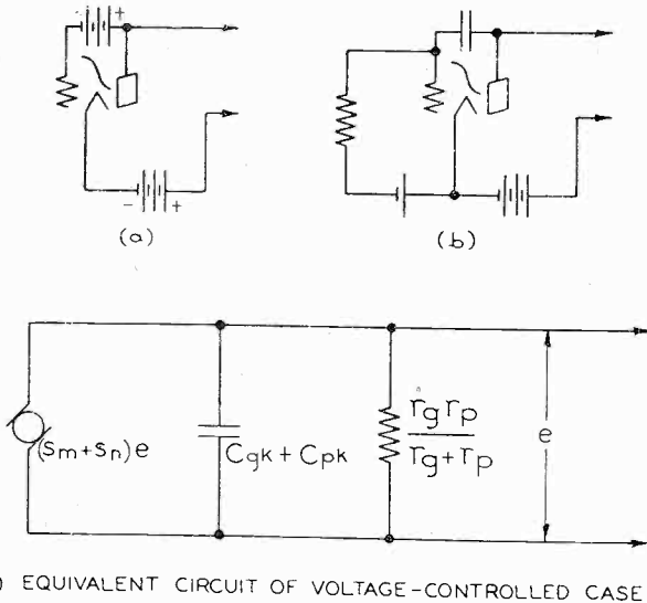
Fig. 5—Production of voltage controlled negative resistance.
