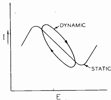
(a) VOLTAGE CONTROLLED
