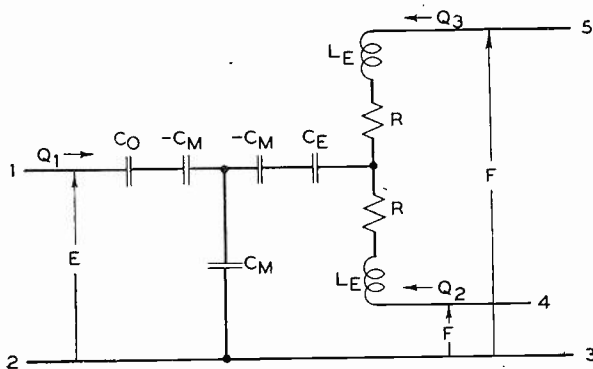
Fig. 2—Electromechanical representation of a symmetrical piezoelectric crystal.
