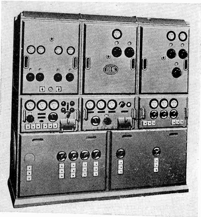
Fig. 6—Beacon transmitter.
