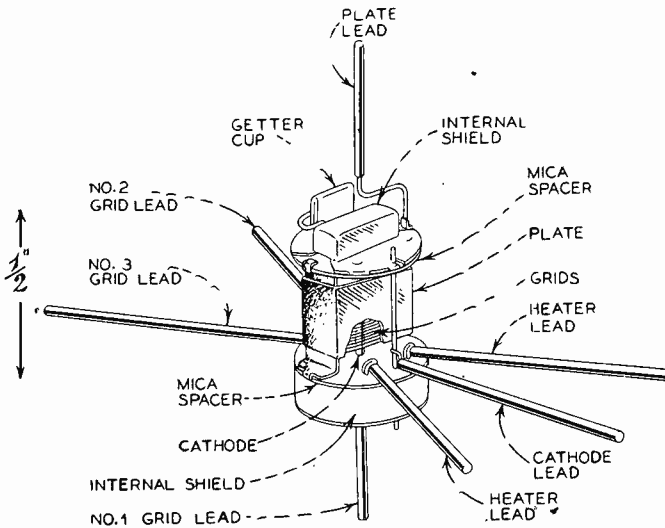
Fig. 3—Internal structure of the pentode.
