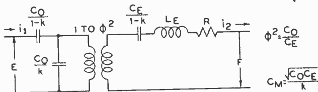
Fig. 5—Electromechanical representation of a piezoelectric crystal, employing an ideal transformer.
