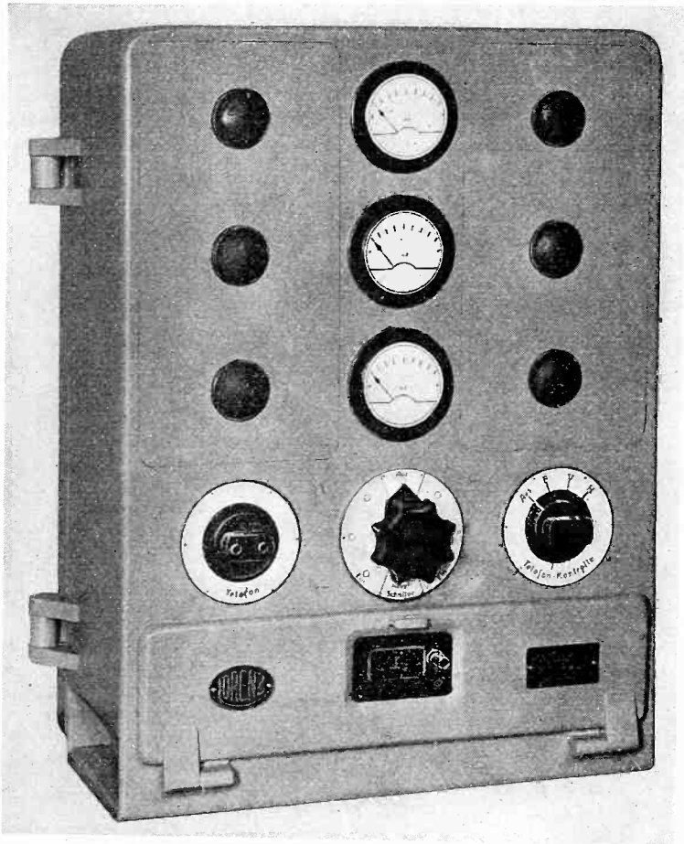
Fig. 8—Remote control of apparatus.
