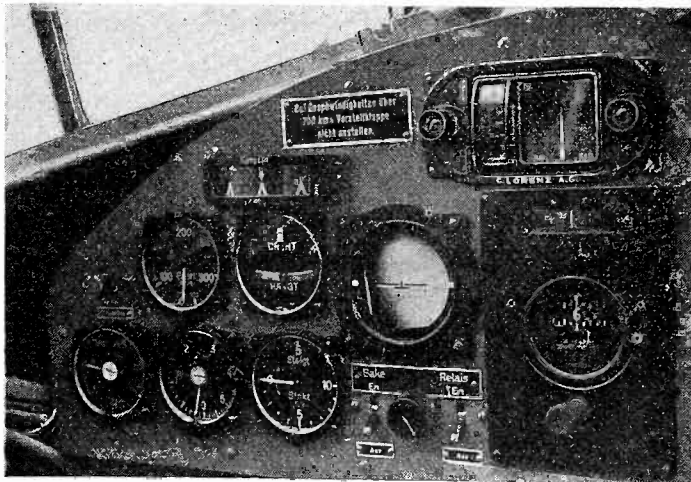
Fig. 12—Visual indicator assembly on the pilot's instrument panel.
