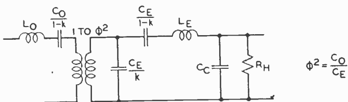
Fig. 6—Electromechanical representation of a loud speaker.
