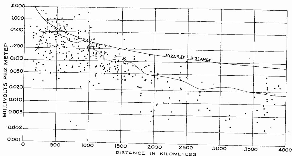
Fig. 5—Night field intensity measurements reduced to one kilowatt of radiated power and given as a function of distance for the broadcast stations in the United States; the irregular curve represents a running average of the data.
