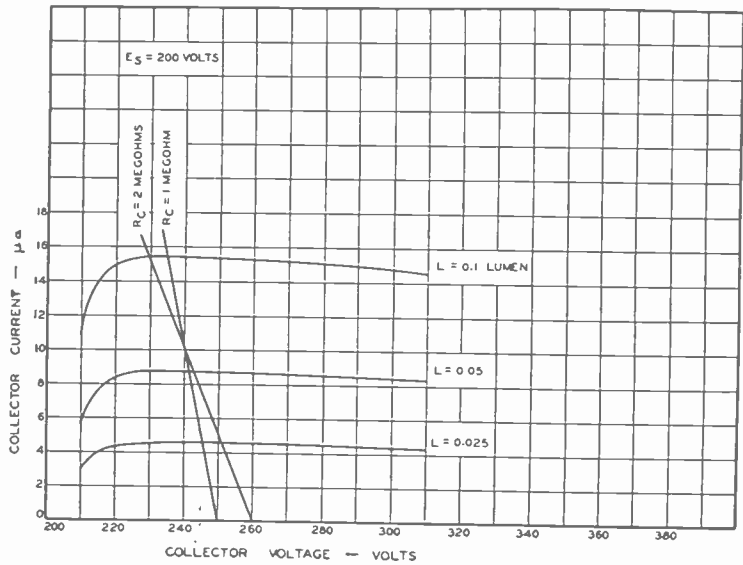
Fig. 5—A typical output family.
