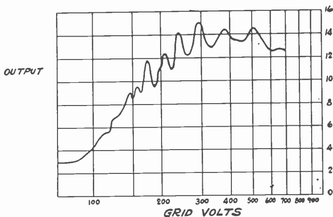
Fig. 10—Sensitivity—grid-potential characteristic, positive-grid detector, at 3300 megacycles.
