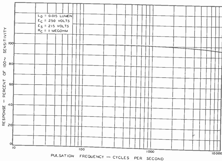
Fig. 6—The response—pulsation-frequency characteristic. The ordinates represent the ratio of response to that of a vacuum -863 type.
