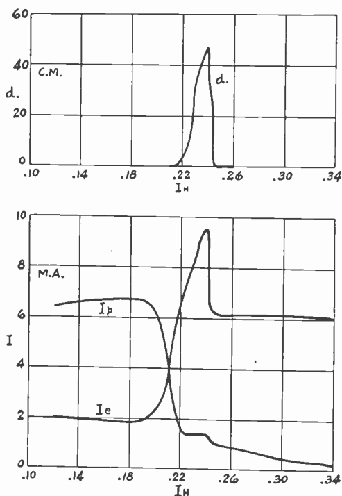
Fig. 5—Plate-current—magnetic-field characteristics, oscillating condition, end-plate magnetron.
