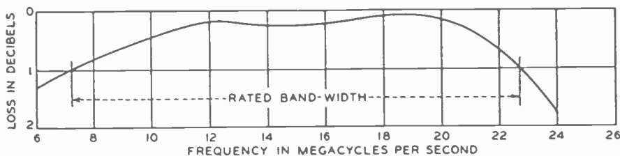
Fig. 20—Loss versus frequency curve for the experimental coupling equipment, shown in Fig. 19, when used to connect an antenna balanced impedance of 778 ohms in parallel with 5 micromicrofarads to a pipe-line unbalanced resistance of 80 ohms.
