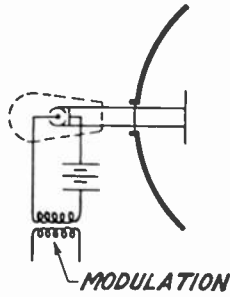
Fig. 6—Plate modulation and radiation system; nine-centimeter transmitter.
