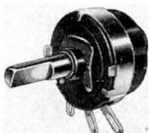
Front view of Type JS Bradleyometer showing locking projections which prevent rotation on panel.
