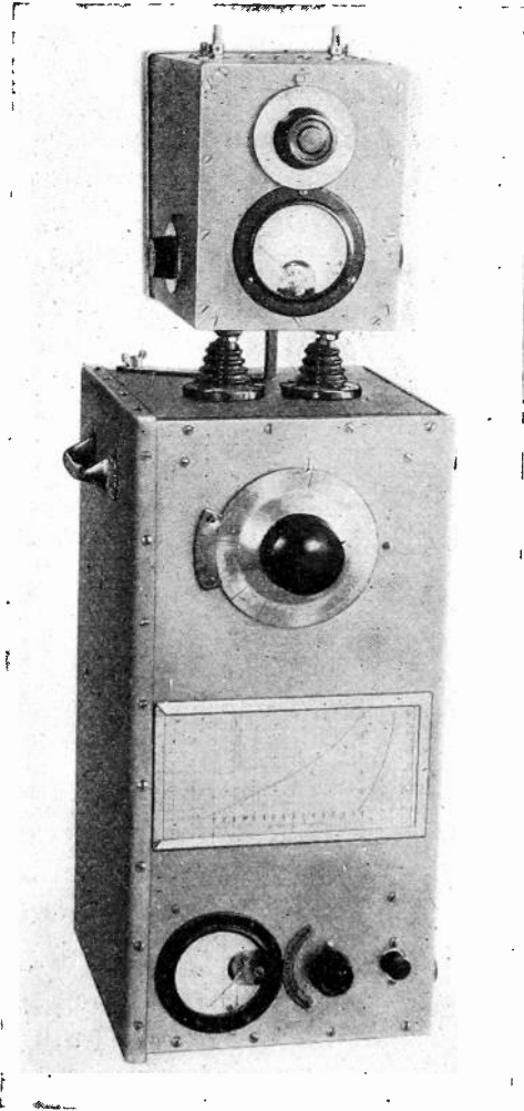
Fig. 17—Impedance measuring equipment and balanced oscillator.
