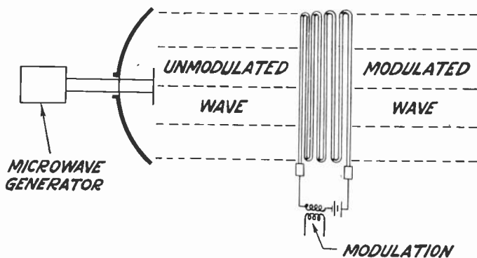
Fig. 8—Diagrammatic representation of ionic modulator.
