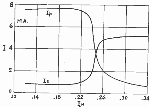
Fig. 4—Plate-current—magnetic-field characteristics, nonscillating condition, end-plate magnetron.
