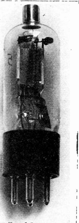
Fig. 1—A typical developmental secondary emission phototube. The data and characteristic curves given here were taken on a tube of this kind.
