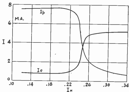
Fig. 4—Plate-current—magnetic-field characteristics, nonoscillating condition, end-plate magnetron.
