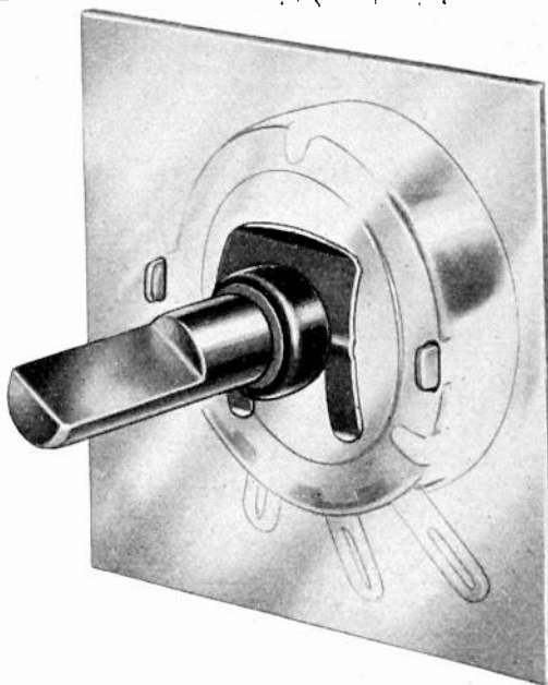
Type J Bradleyometer with cover removed to show contact mechanism and terminals.
