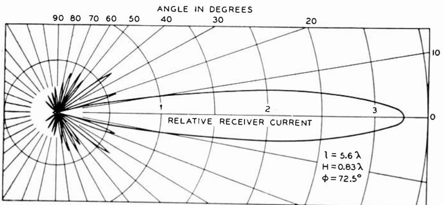
Fig. 4—Maximum output design. Receiver current versus azimuth angle for a 17.5-degree wave angle.
