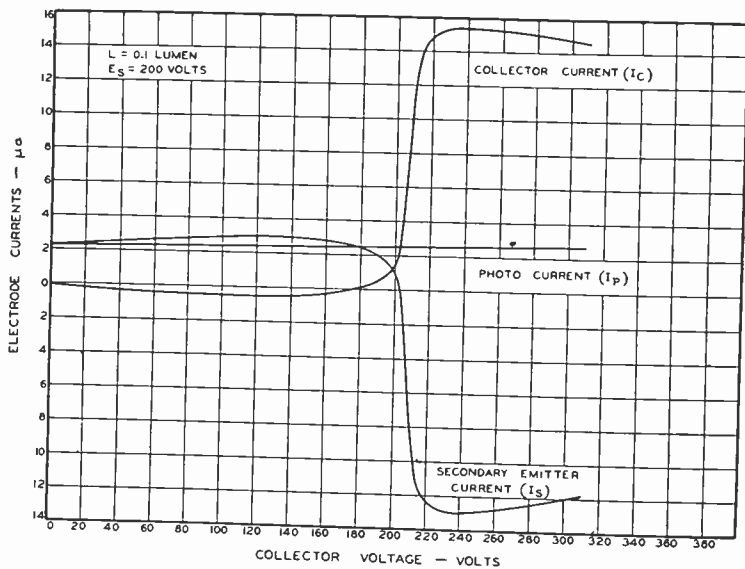
Fig. 3—The variation of the electrode currents with collector voltage for a typical tube of the kind shown in Fig. 1.
