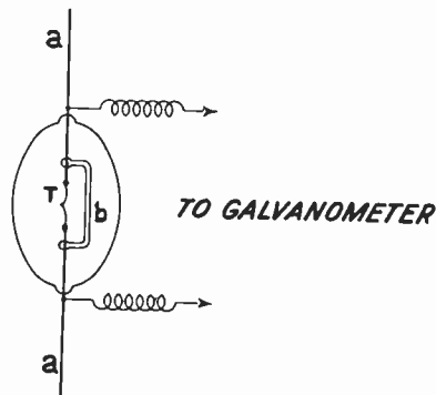
Fig. 1—Half-wave thermojunction radiation indicator.
