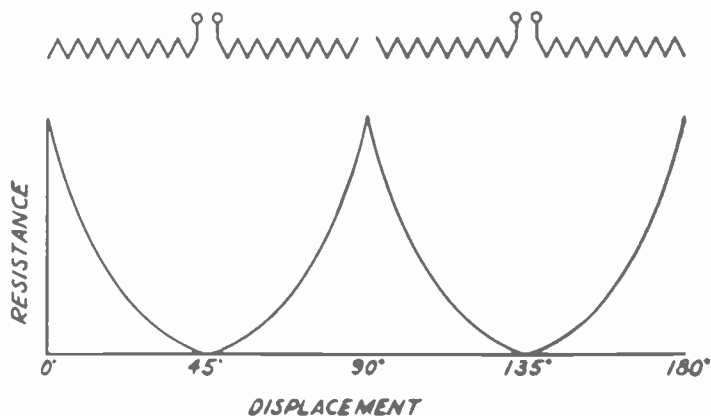
Fig. 5—Rheostat characteristic.
