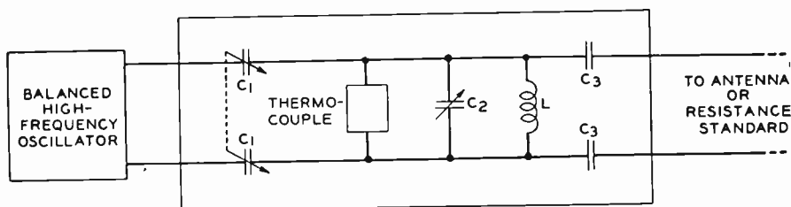
Fig. 16—Schematic diagram of impedance measuring equipment.
