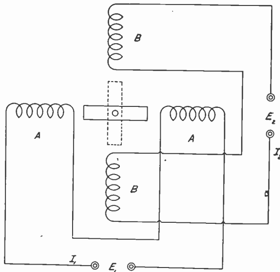
Fig. 1—Pertaining to motor principle.
