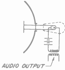
Fig. 13—Circuit, magnetron detector.
