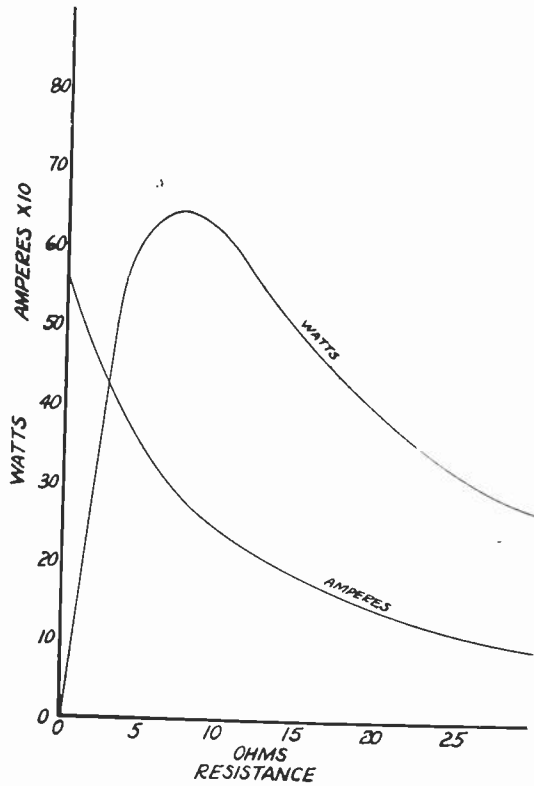
Fig. 3—Rheostat characteristics.
