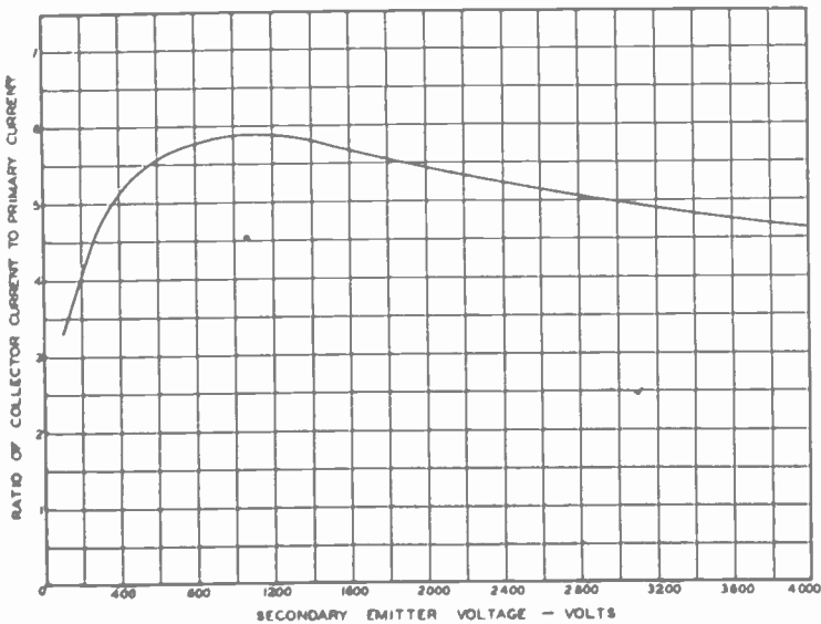
Fig. 2—The ratio of collector current to primary current as a function of the secondary emitter potential. These data were taken on a beam tube, the secondary emitter consisting of an oxidized silver surface sensitized with caesium.
