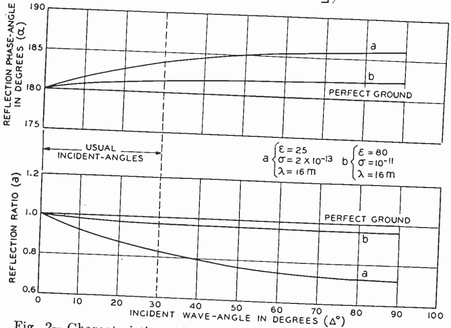
Fig. 2—Characteristics of horizontally polarized wave reflections from various types of ground.
