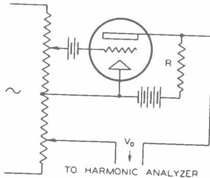
Fig. 2—Arrangement for measuring distortion in a vacuum tube amplifier.
