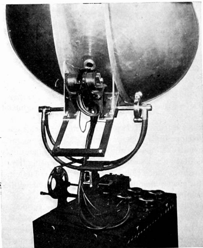
Fig. 7—Nine-centimeter transmitter with power supply units.
