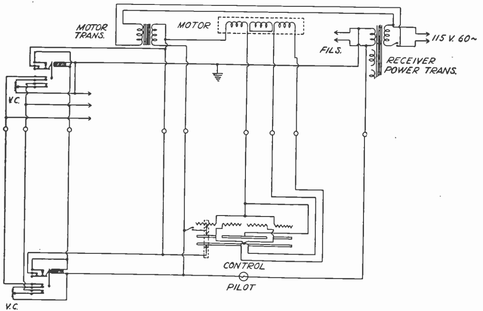
Fig. 8—Complete circuit diagram.
