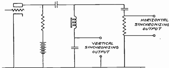
Fig. 11—Circuit for separation of vertical and horizontal synchronizing signals from the composite synchronizing signal by means of very simple frequency selective circuits. Figs. 11 and 12 show the circuit and char-
