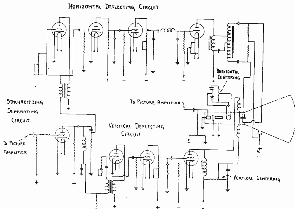
Fig. 21—Schematic arrangement of kinescope deflecting circuit.
