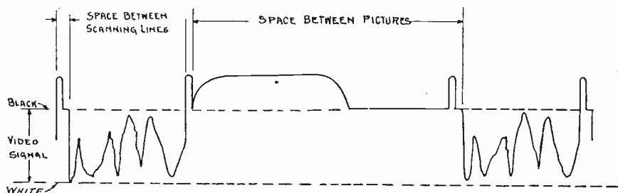
Fig. 7—Composite signal as received.
