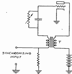
Fig. 15—The blocking oscillator.
