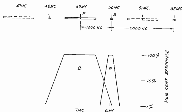
Fig. 1—Channel arrangement and receiver selectivity characteristic.
