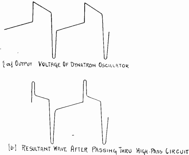
Fig. 14—Voltage wave shapes obtainable with dynatron oscillator.
