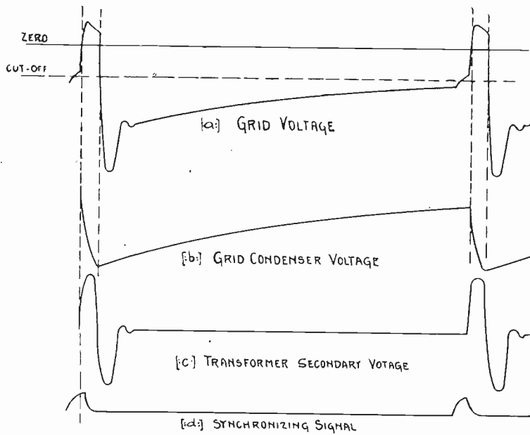
Fig. 16—Blocking oscillator circuit voltage.
