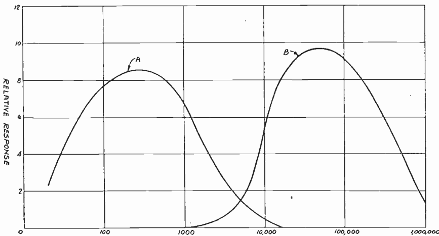
Fig. 12—Response characteristics of circuit shown in Fig. 11.
