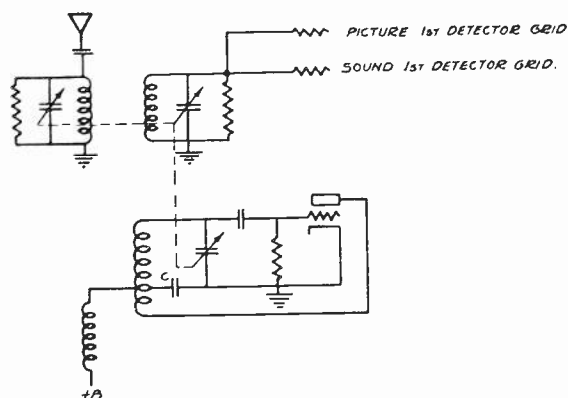
Fig. 2—Radio-frequency and oscillator system.
