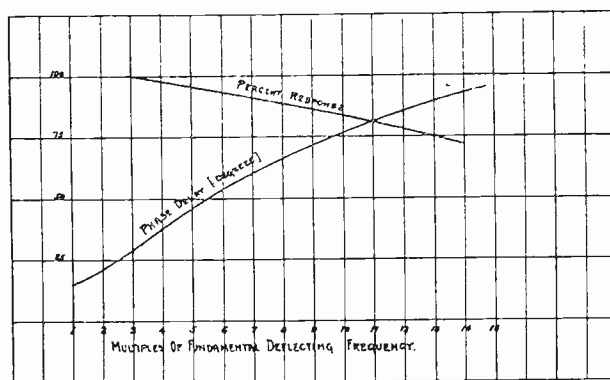
Fig. 20—Response and phase delay characteristics of horizontal deflecting circuit.
