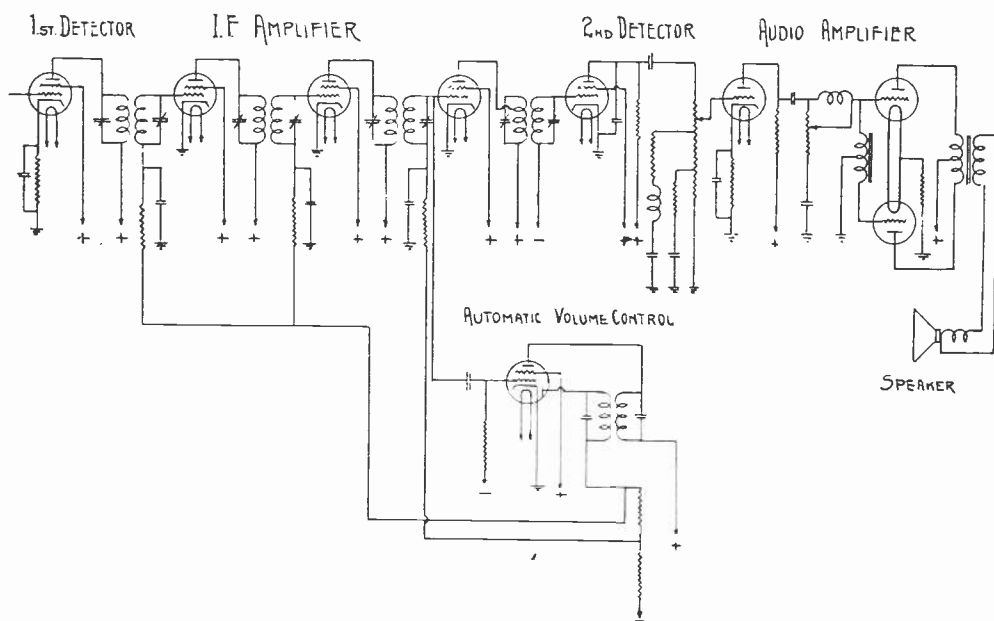
Fig. 3—Receiver sound channel.
