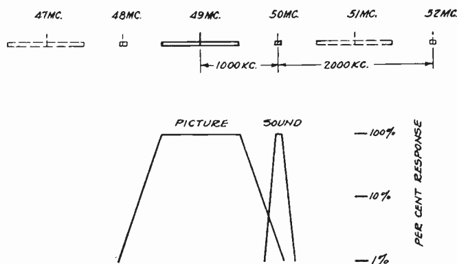
Fig. 1—Over-all transmitter and receiver selectivity characteristics.
