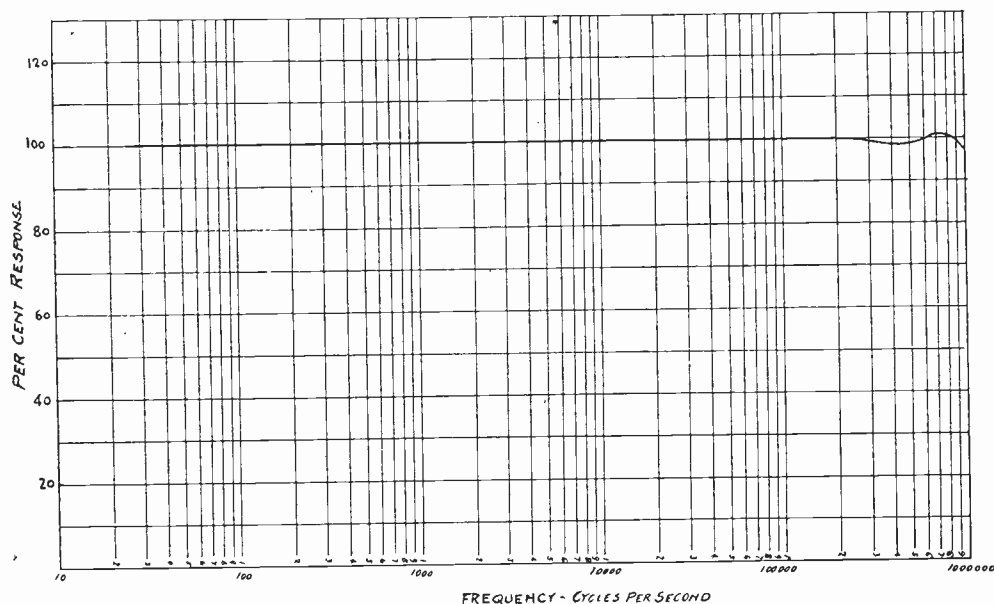
Fig. 6—Receiver video amplifier characteristics.
