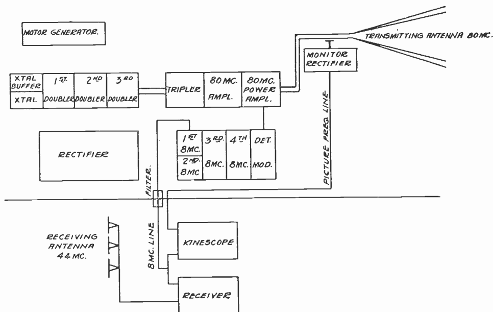
Fig. 1—Block diagram of relay station at Arney's Mount.
