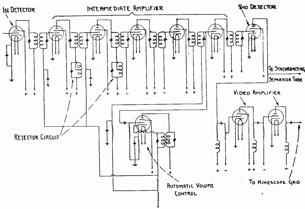
Fig. 4—Receiver picture channel.
