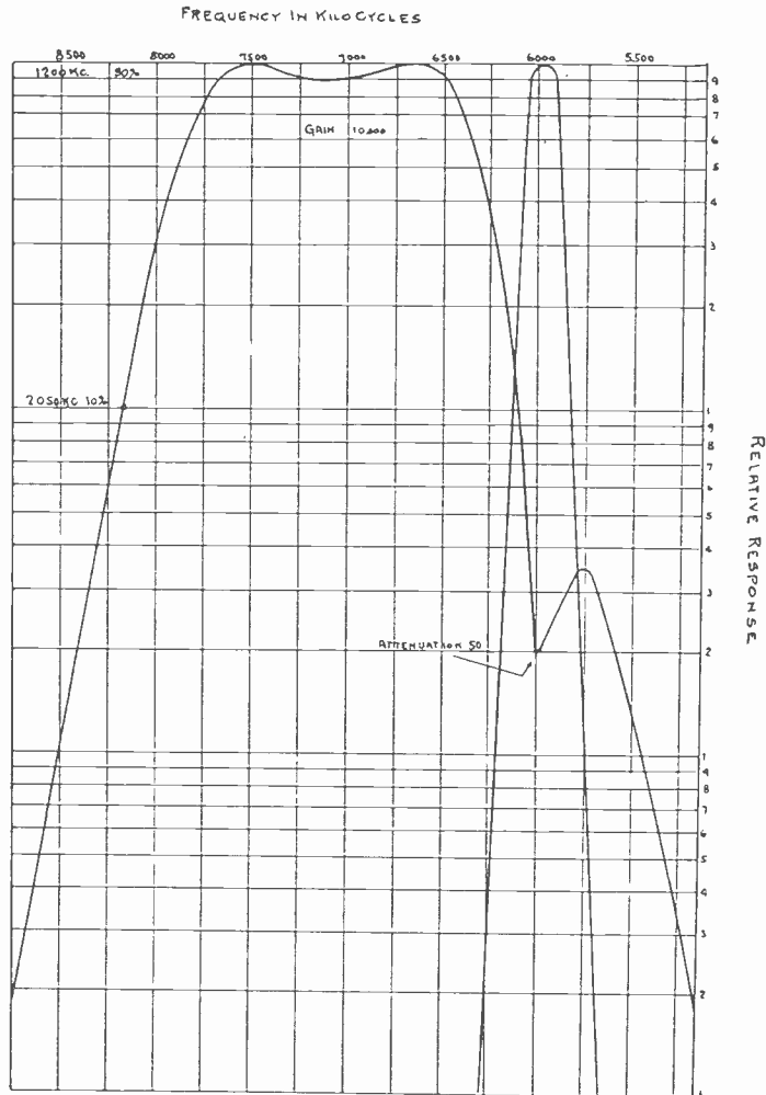
Fig. 5—Sound and picture intermediate-frequency characteristics.
