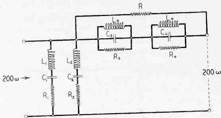
Fig. 7—Equalizer for moving-coil microphone.
