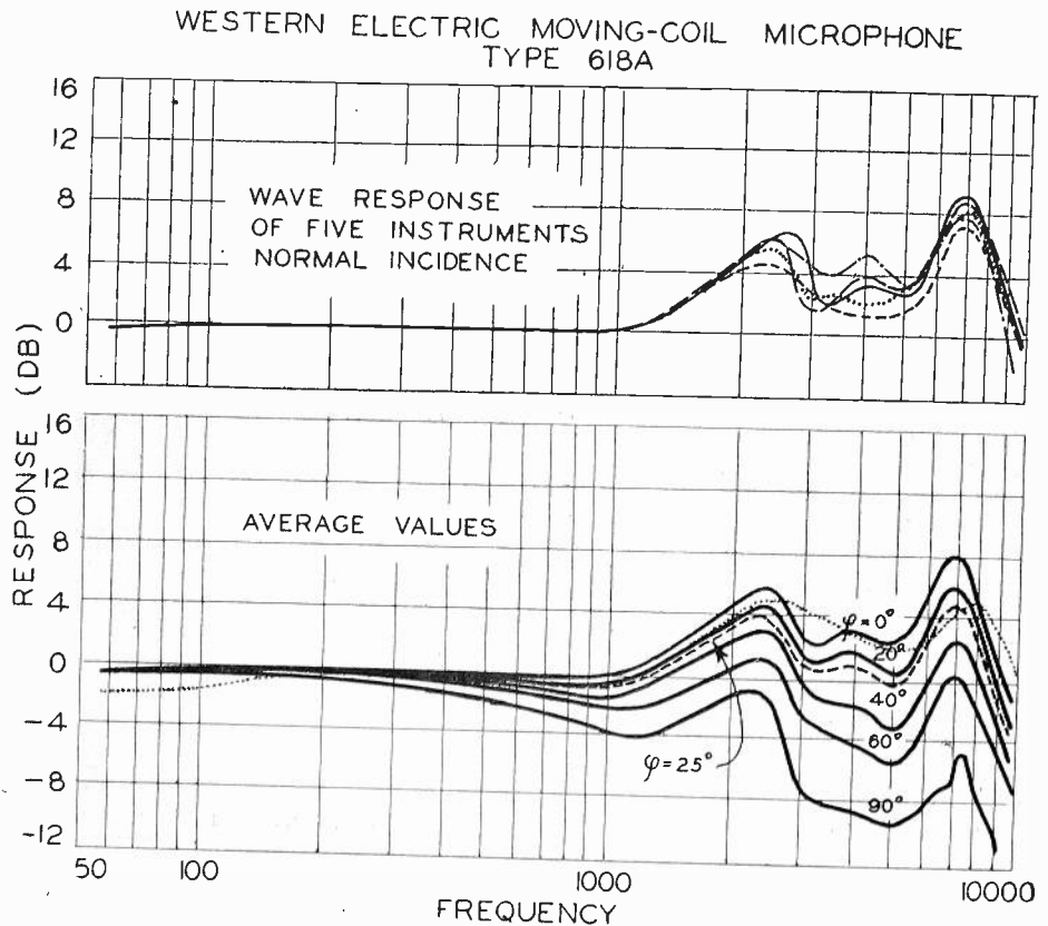
Fig. 6—Wave response of five Western Electric moving-coil microphones, Type 618A.
