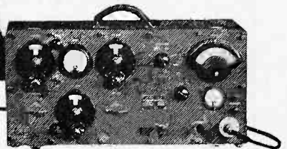
← BEAT FREQUENCY OSCILLATOR TYPE TMV-52-E Range 20 to 17,000 cycles. Constant output. Low harmonic content. Open circuit output 25 volts. Vibrating reed calibration indicator.
