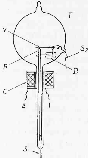
Fig. 1—Experimental model of the chopper.
