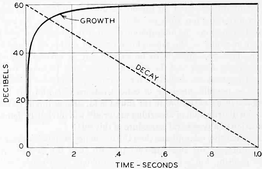
Fig. 21—Growth and decay of sound in a reverberant room.
