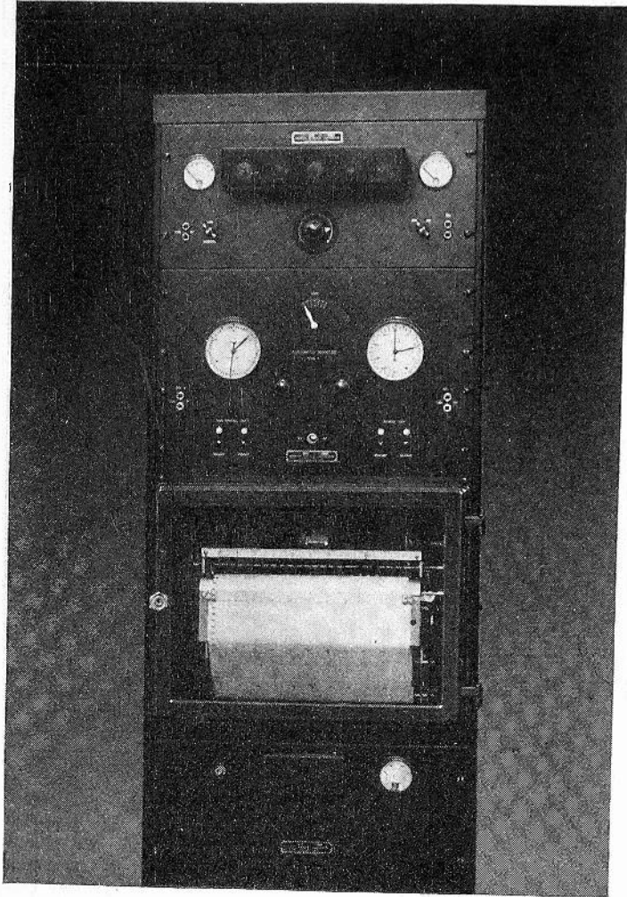
Fig. 31—Photographic view of automatic monitor and volume level recorder.
