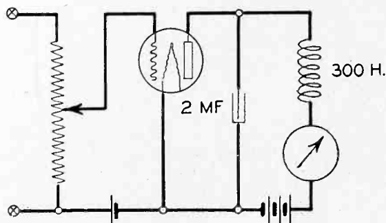
Fig. 26—Common type of volume level indicator.
