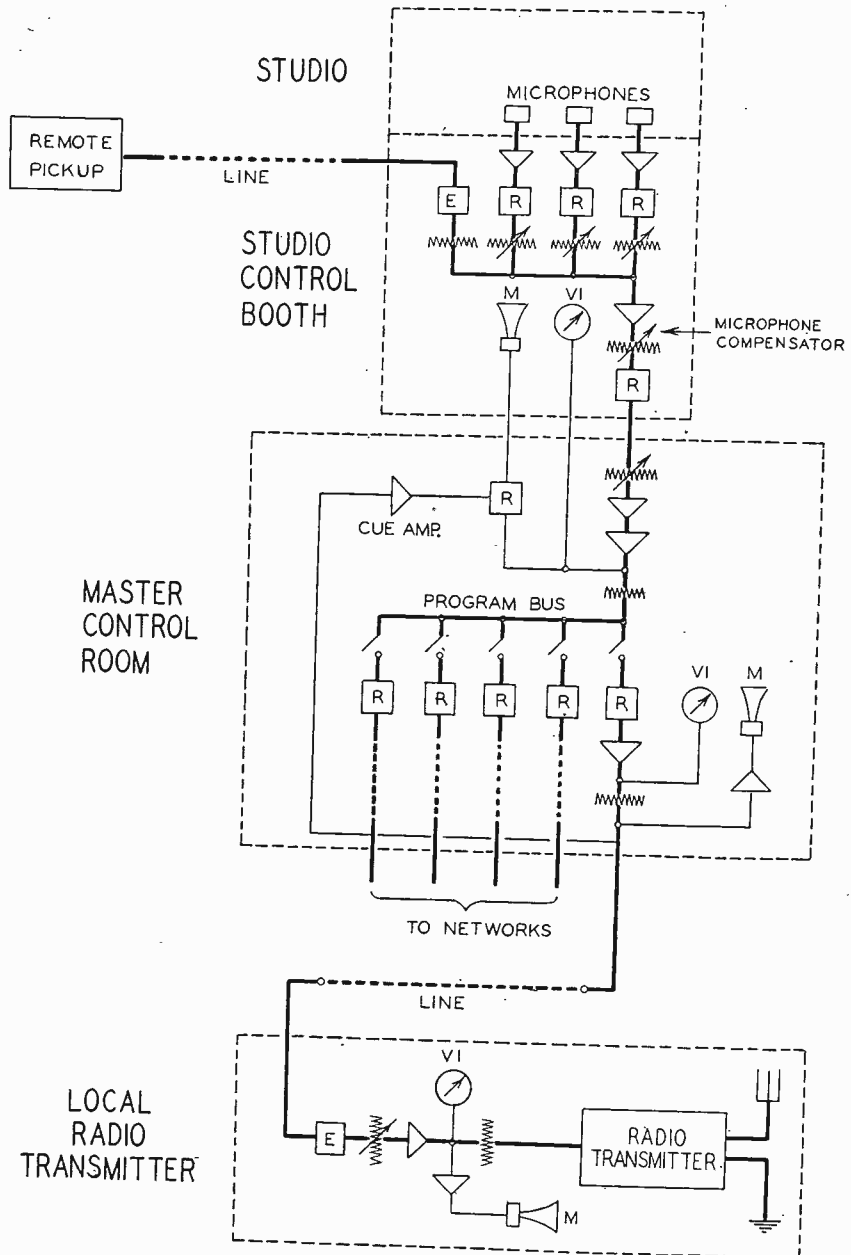
Fig. 1—Schematic diagram showing the circuit organization of a typical broadcast transmitting system.
