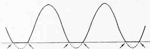
Fig. 24—Illustrating “breaks” produced by overmodulation in a radio transmitter.
