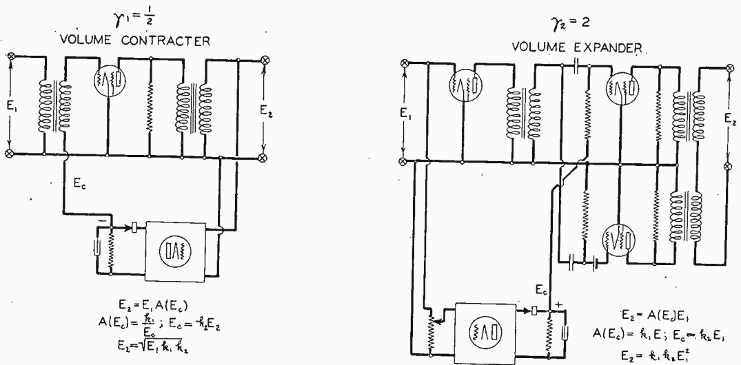
Fig. 34—Schematic diagrams of automatic contractor and expander; contraction gamma = 0.5; expansion gamma = 2.
