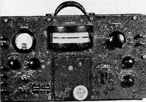
FIELD INTENSITY METER TYPE TMV-75-B → Frequency range 500 kc to 20,000 kc. Field intensity range 20 microvolts/meter to 6 volts/meter.
