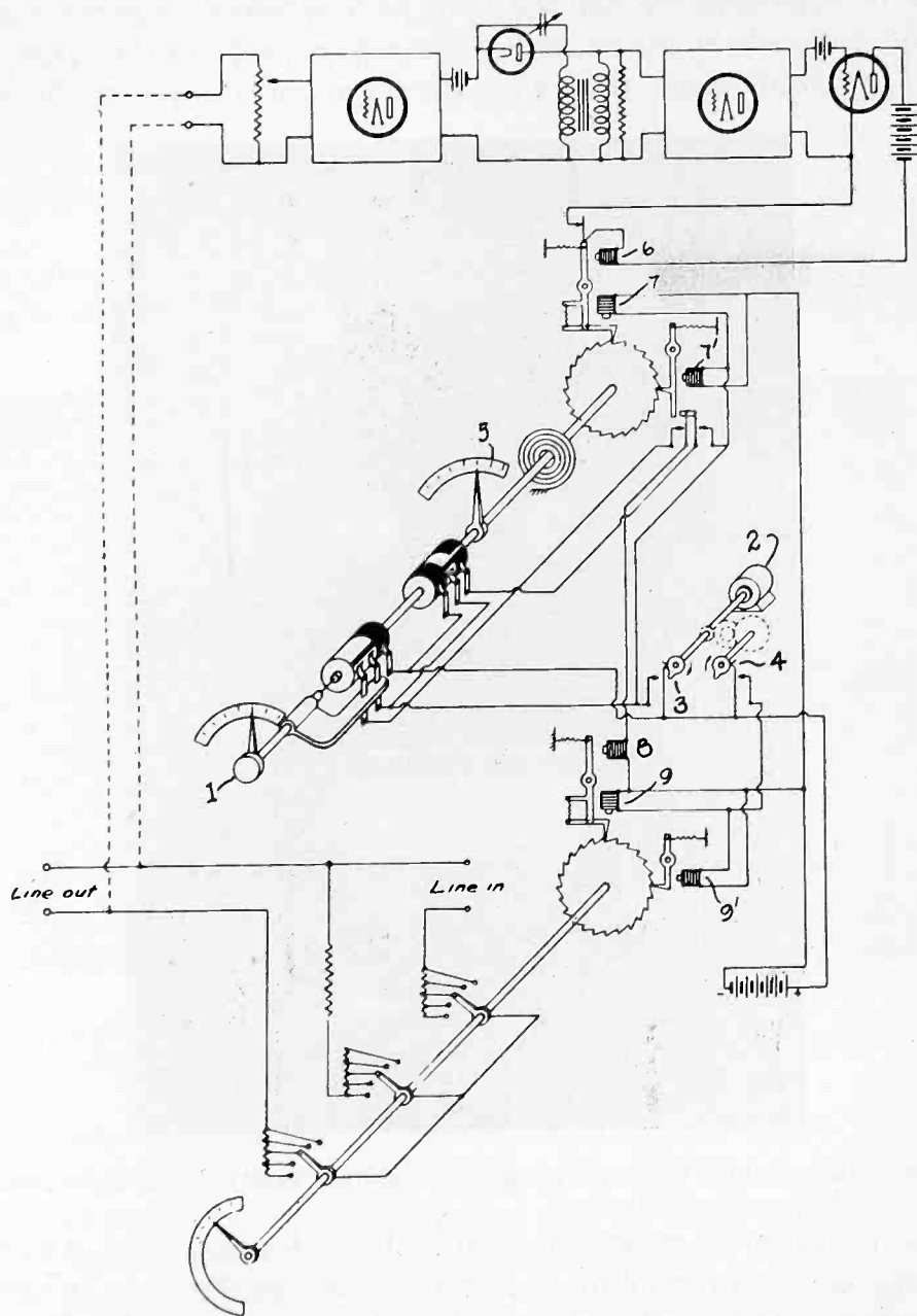
Fig. 30—Schematic diagram of automatic volume level limiter, based upon peak counts.
