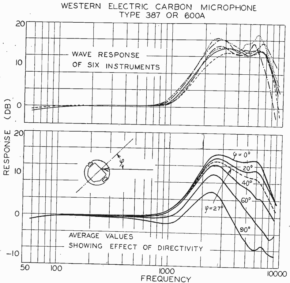
Fig. 2—Wave response of six Western Electric Type 387 or 600A carbon microphones; (upper curves) normal incidence; (lower curves) at various angles of incidence.
