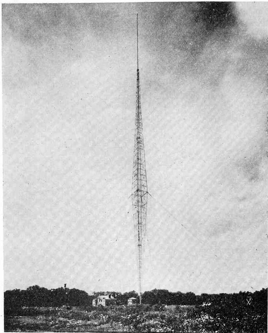
Fig. 40—Vertical antenna of guyed cantilever type as installed at WABC, Wayne, New Jersey; height = 675 feet.
