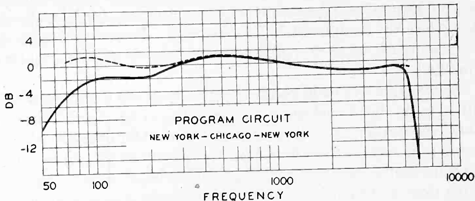
Fig. 23—Transmission of long-distance program circuit.
