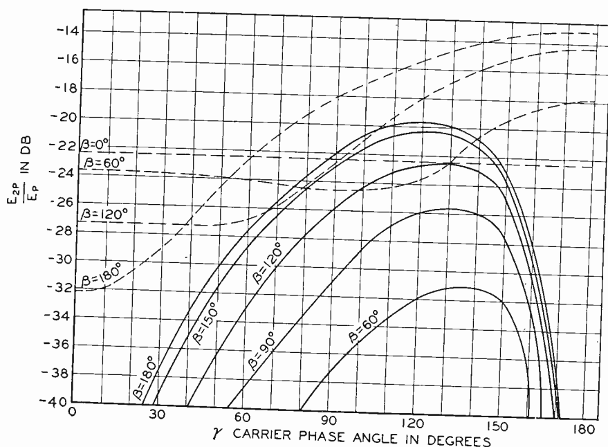
Fig. 10—Ratio of second harmonic to fundamental audio-frequency output under the conditions of Fig. 8. The full lines are for a linear detector, the dashed lines are for a square-law detector.
