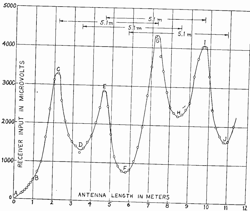
Fig. 4—Curve showing effect of antenna length on receiver input. Wavelength of received radiation 5.1 meters. Receiving antenna vertical and located 2.7 kilometers distant from the transmitter.
