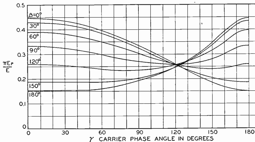
Fig. 8—Fundamental audio-frequency output of a linear detector under the action of two waves of the type shown in Fig. 1. K = 0.5 , M = m = 0.3 .
