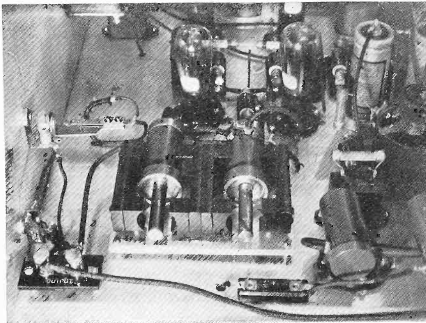
Fig. 11—Photograph of the two-section filter with one pair of coils removed to show the rods.
