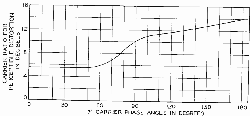
Fig. 20—Effect of carrier phase angle on field strength ratio at which distortion becomes perceptible in the output of a linear rectifier. \beta = 180 degrees for all of the modulation frequencies; i.e., there is no relative time delay but the polarity of the program frequency supply to one modulator is reversed. Both stations are modulated 80 per cent on peaks.
