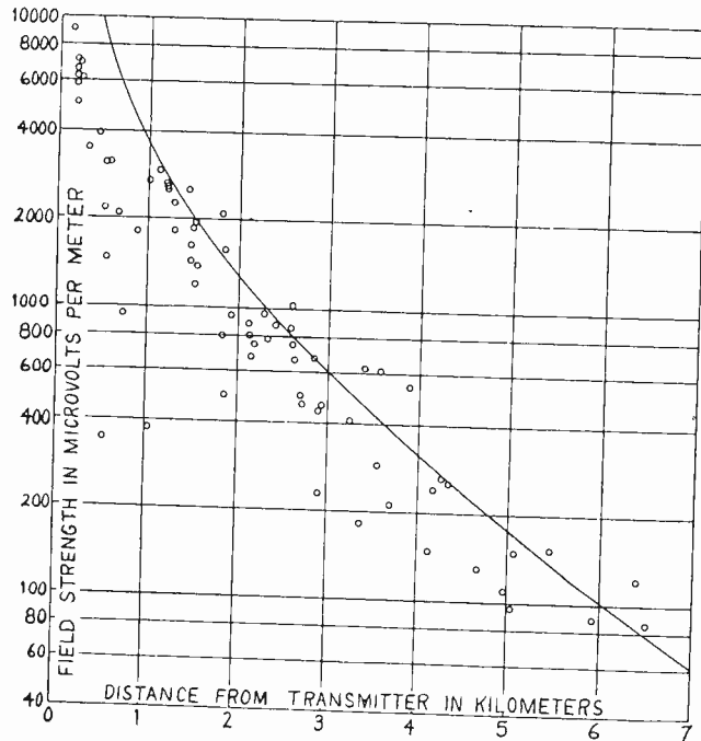
Fig. 2—Attenuation curve for 5.1-meter radiation. \alpha = 0.36 .
