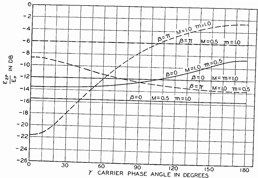
Fig. 13—Typical curves showing the effect of unequal degrees of modulation. K = 0.5 .
