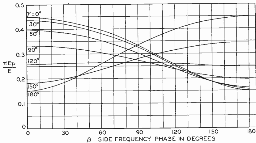
Fig. 11—The data of Fig. 8 plotted with \beta , the side frequency phase angle, as abscissa.
