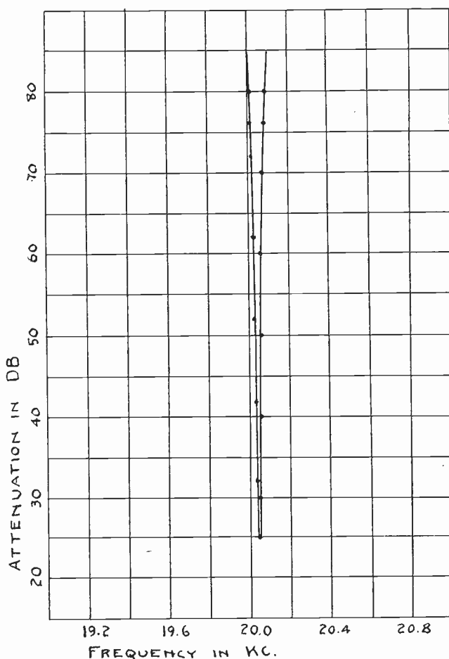
Fig. 8—Attenuation curves for two "water-quenched" monel rods in series coupled by a vacuum tube.
