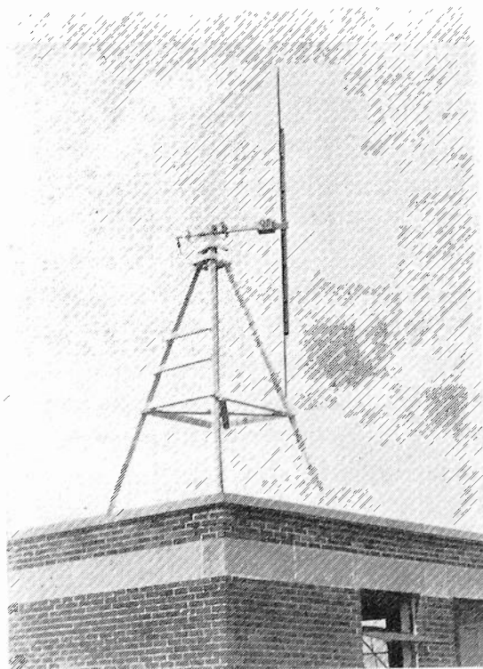
Fig. 1—Tower on roof of elevator house on the Physics building, showing transmitter with cover removed and the antenna in vertical position.
