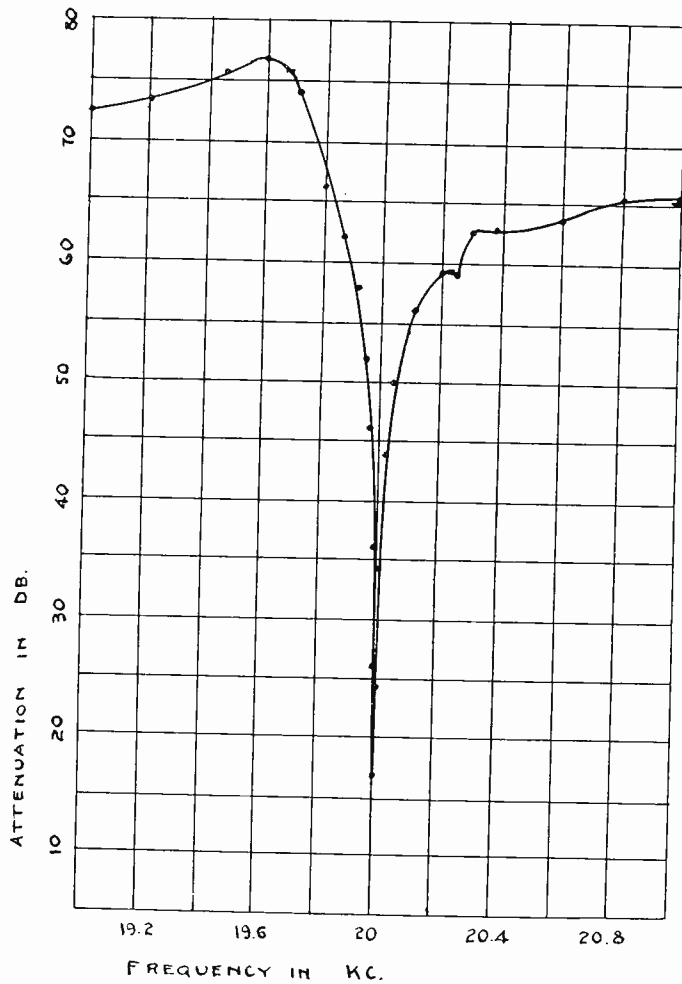
Fig. 5—Attenuation curve for monel rod, 1/2 inch diameter.
