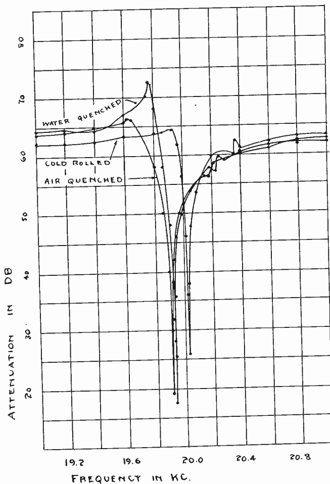
Fig. 6—Attenuation curves for 1/2-inch monel rod in coils which clear it by 3/32 inch, for various conditions of heat treatment.
