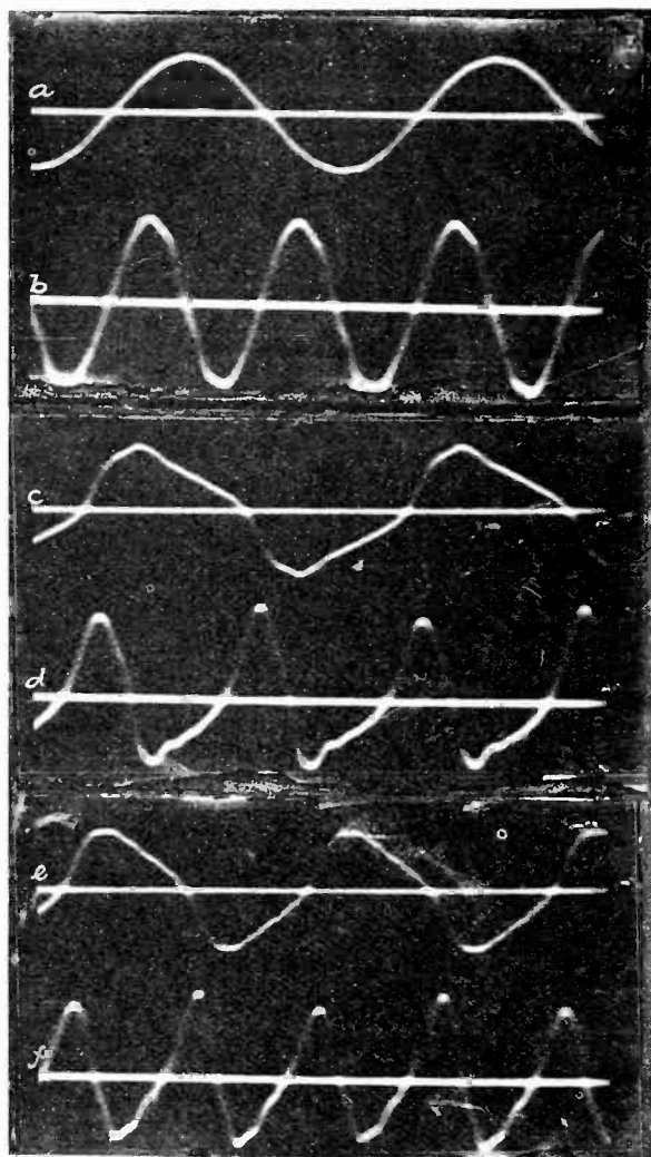
Fig. 17—Oscillograms showing operation of beacon amplifiers.
