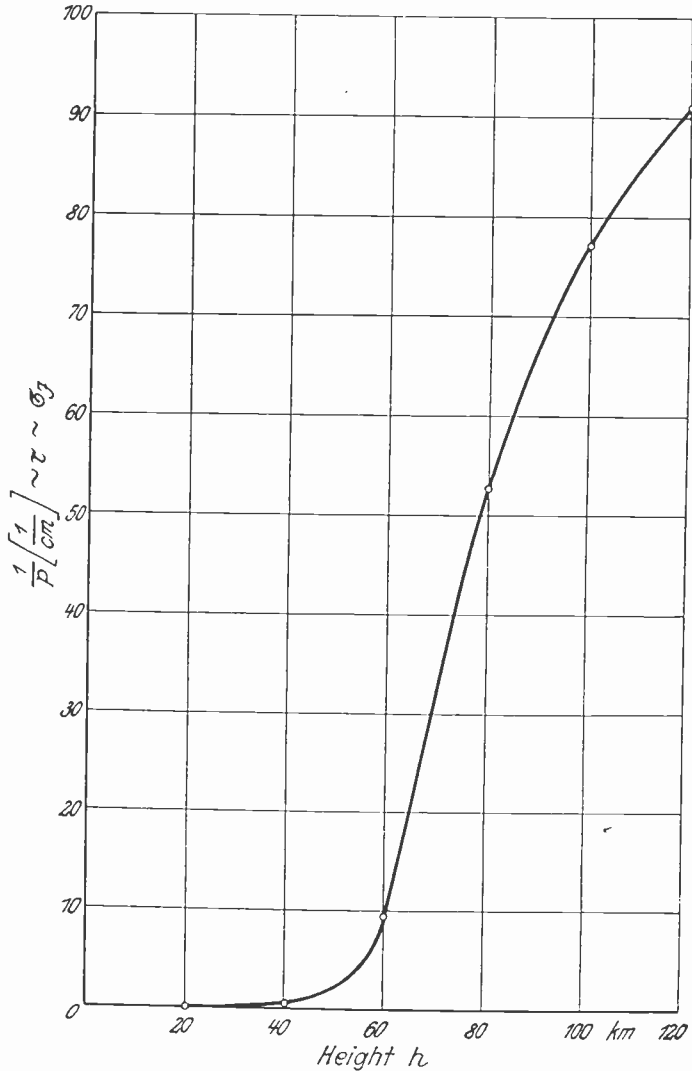
Fig. 1—Reciprocal of the air pressure 1/p ( \sim \tau , \sim \sigma_J ) in [1/\text{mm Hg}] as function of the height h above the earth (km).
