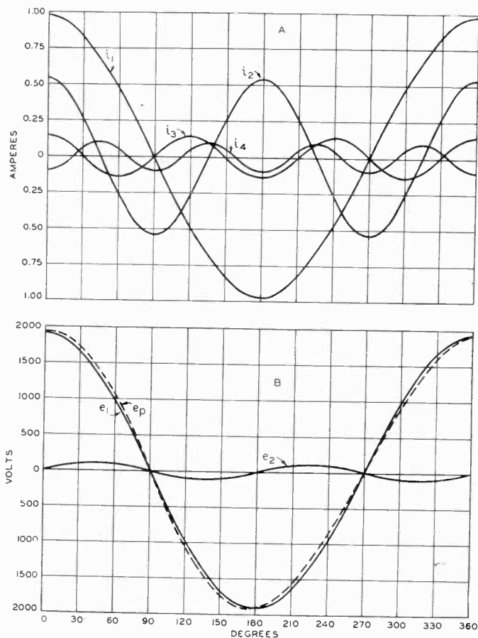
Fig. 5A—First four components of i_0 , Fig. 4B.
