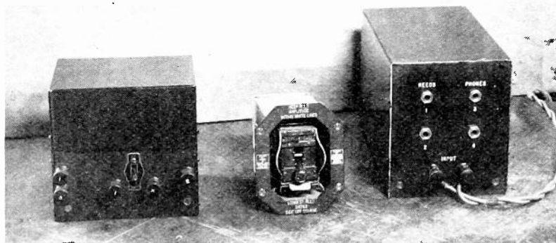
Fig. 23—Filter unit and amplifier.
