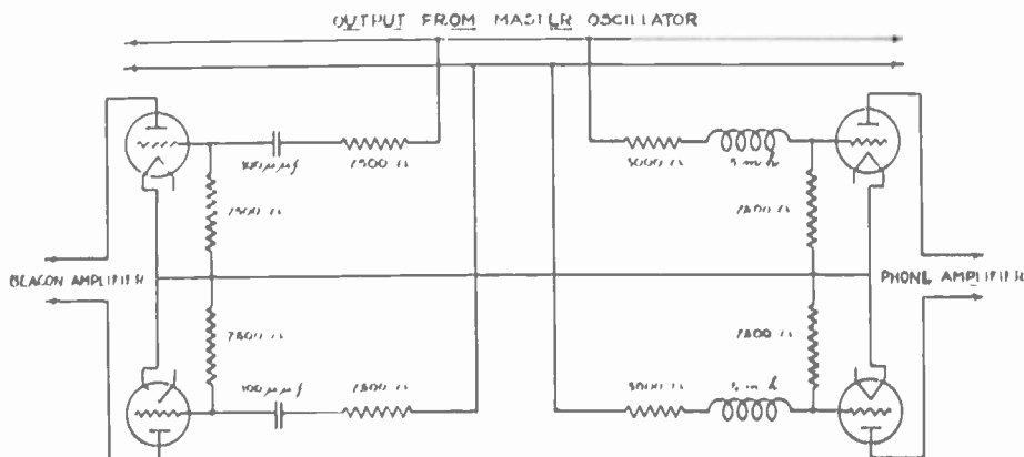
Fig. 7—Electrical circuit diagram of phase-shifting unit.
