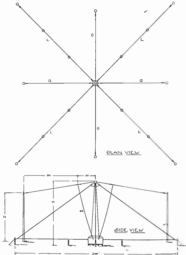
Fig. 18—Antenna system.
