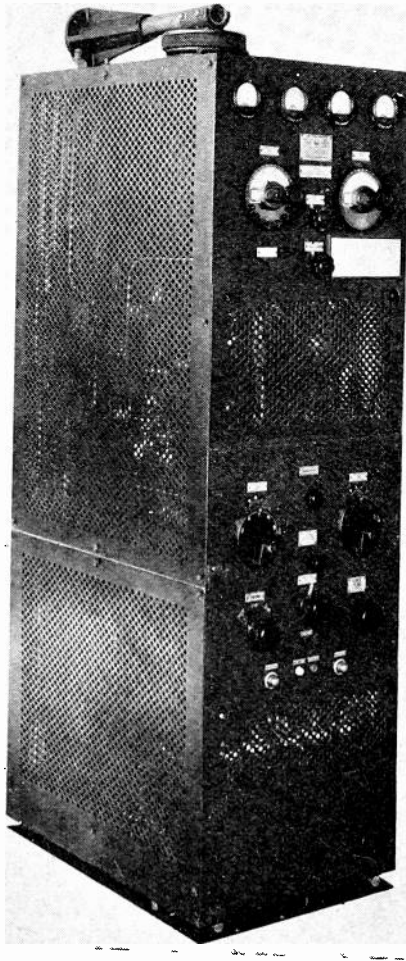
Fig. 7—ET-3674 combination transmitter.
