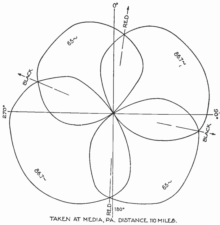
Fig. 19—Polar patterns for combined transmitting set.
