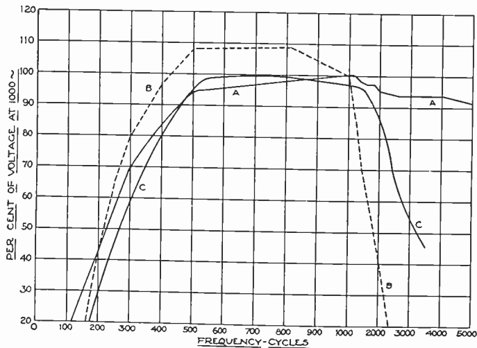
Fig. 16—Fidelity characteristics of speech equipment.
