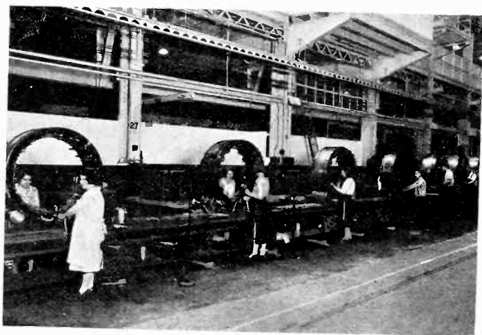
Assembling stators for electric locomotives at the Westinghouse plant.
