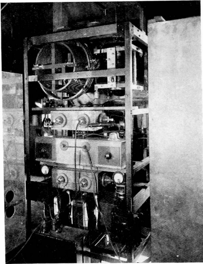
Fig. 9—Radiophone and carrier amplifier unit—rear view.
