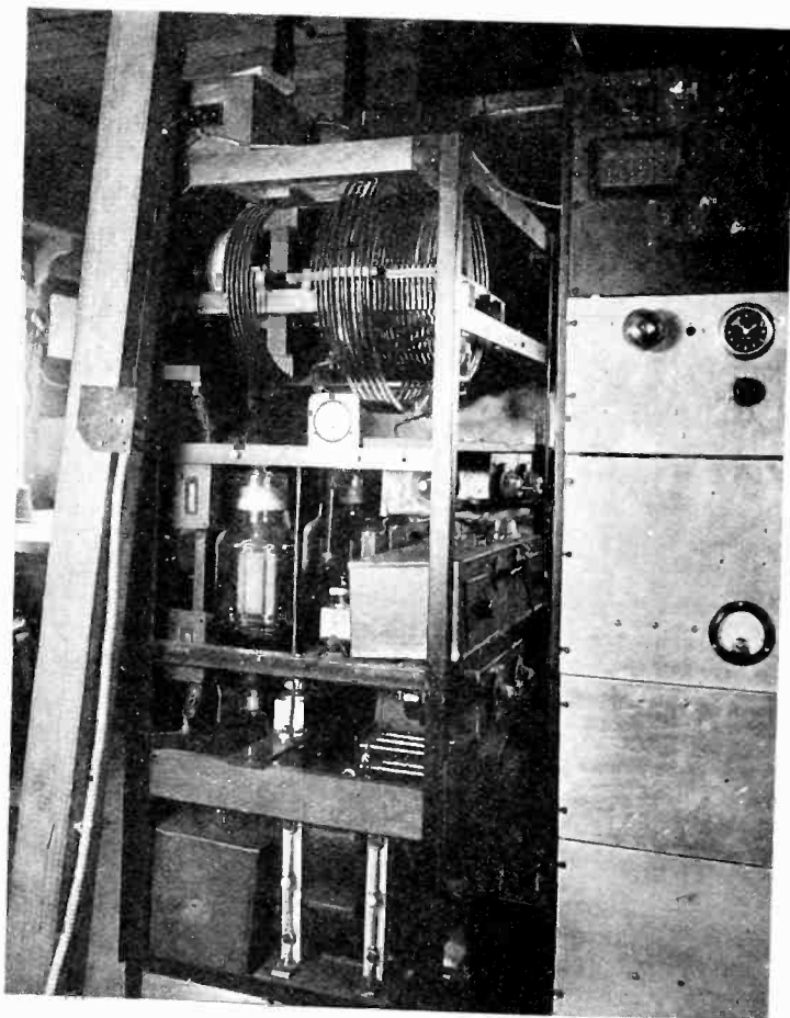
Fig. 8—Radiophone and carrier amplifier unit—side view.
