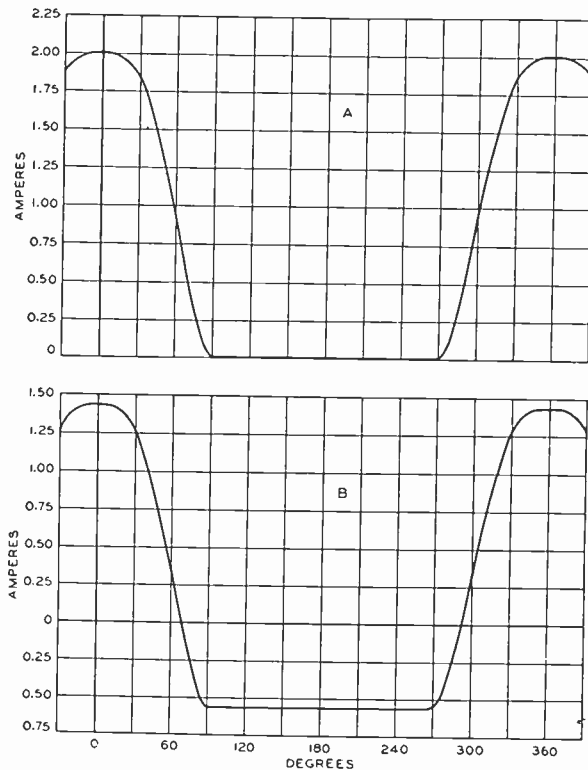
Fig. 4A—Pulsating plate current wave, i_p .
