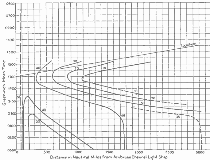
Fig. 20—Approximate variation of radio field strengths with distance and time of day. Contour lines indicate maximum expected field strengths in decibels above 1 microvolt per meter. Frequency 8 mc. Winter. Corrected to 1-kw radiated power.
