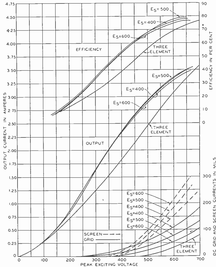
Fig. 15—Dynamic output and efficiency of a screen-grid tube compared to that of a three-element tube. E_b = 3000 volts, E_c (at cut-off), Z_0 = 1500 ohms.
