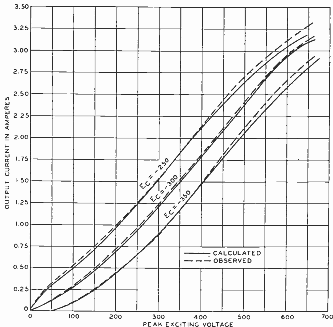
Fig. 11—Calculated and experimental dynamic characteristics of Western Electric No. 251-A tube E_b=3000 volts, Z_0=2000 ohms, \mu=10 .
