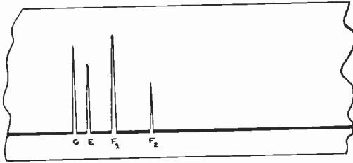
Fig. 2—Diagram showing type of oscillogram which may be obtained by the group retardation method.
