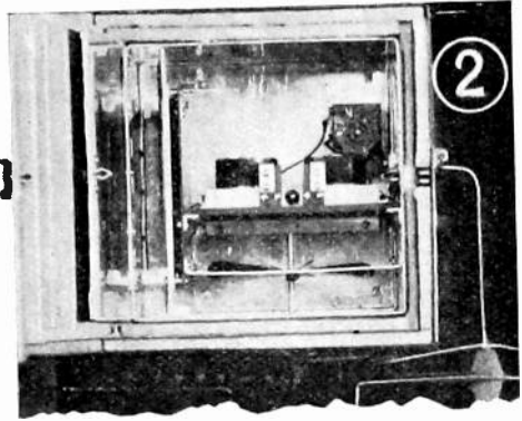
Crystal oven of DeForest Frequency Control unit, showing grouped members and fan.
