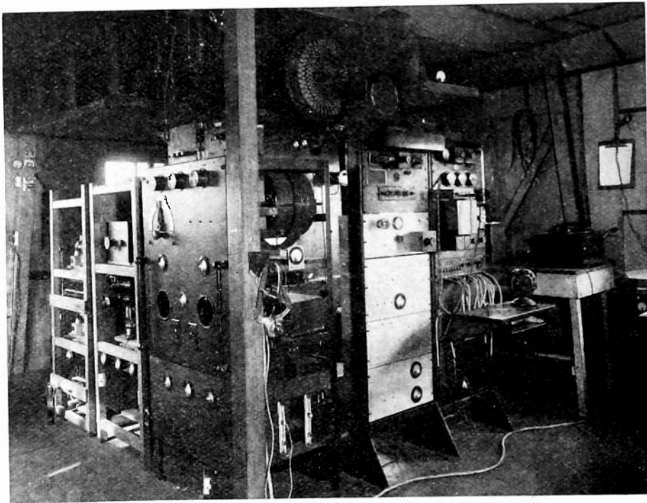
Fig. 4—General view of the experimental transmitting set at College Park.
