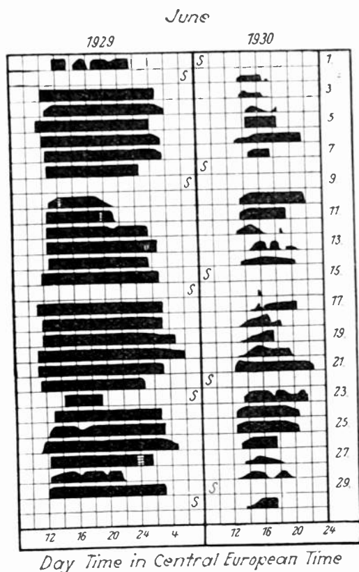
Fig. 6—Comparison of reception amplitudes in Geltow of a 16-m wave from New York in June, 1929, and in June, 1930.
