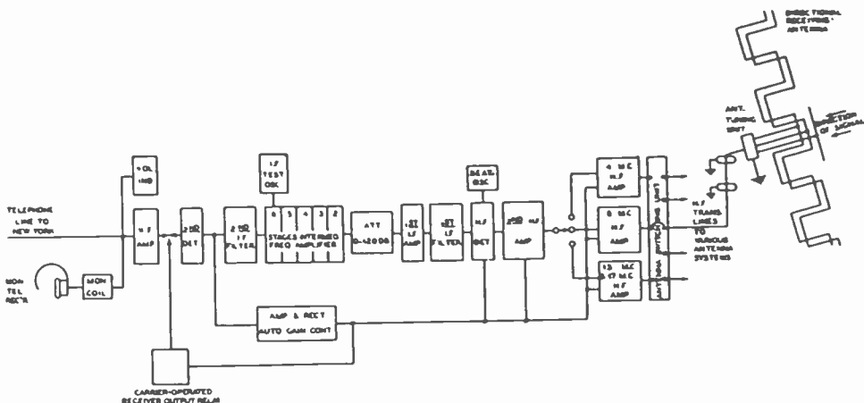
Fig. 5—Block schematic of radio receiving system at Forked River, New Jersey. (1) Intermediate frequency filters adjusted to pass band 395 kc. (2) Operation of carrier-operated receiver output relay is such that when a carrier is being received, the receiver output is "normal," but when no carrier is received, the output of the receiver is "cut off."
