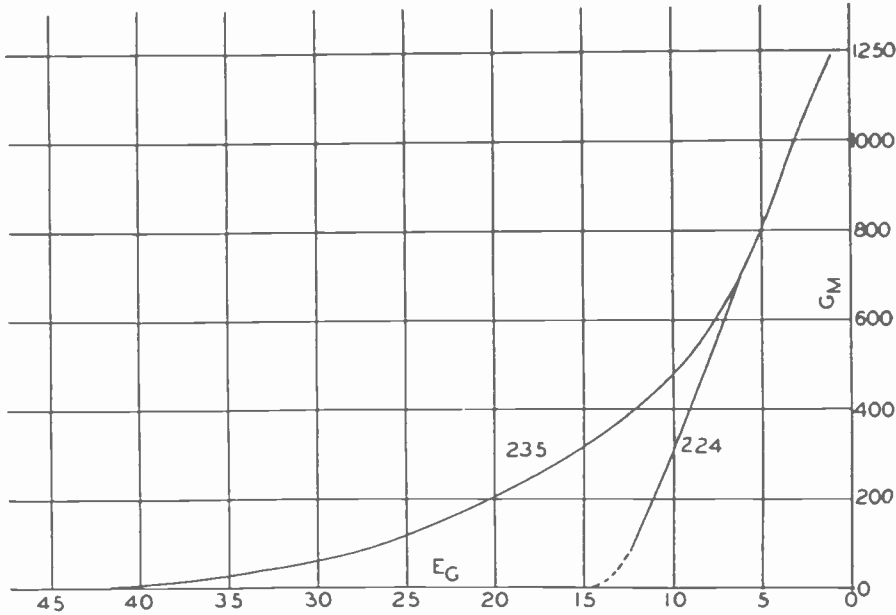
Fig. 5—Comparison between G_M curves, Type 224 and 235. E_p = 180 E_{SG} = 90
