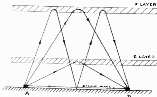
Fig. 1—Diagram showing various paths by which pulse may arrive at receiving station.
