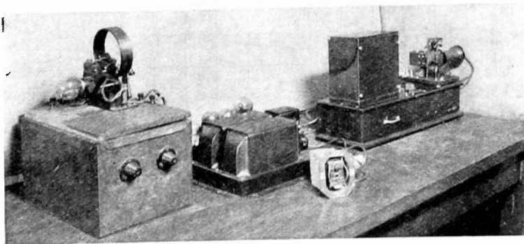
Fig. 15—Equipment used to check phase relations.
