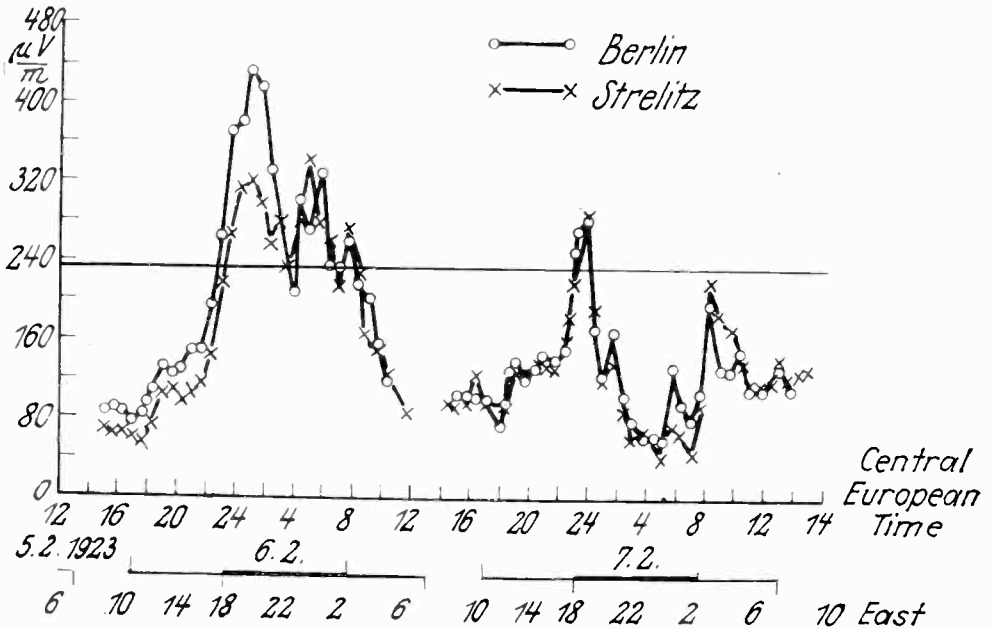
Fig. 2—Reception measurements of the sending station WQK (Rocky Point, \lambda = 16,400 \text{ m} , f = 18.3 \text{ kc} ) in Berlin and Strelitz.
