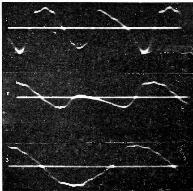
Fig. 14—Oscillograms showing means of checking phase relations:
