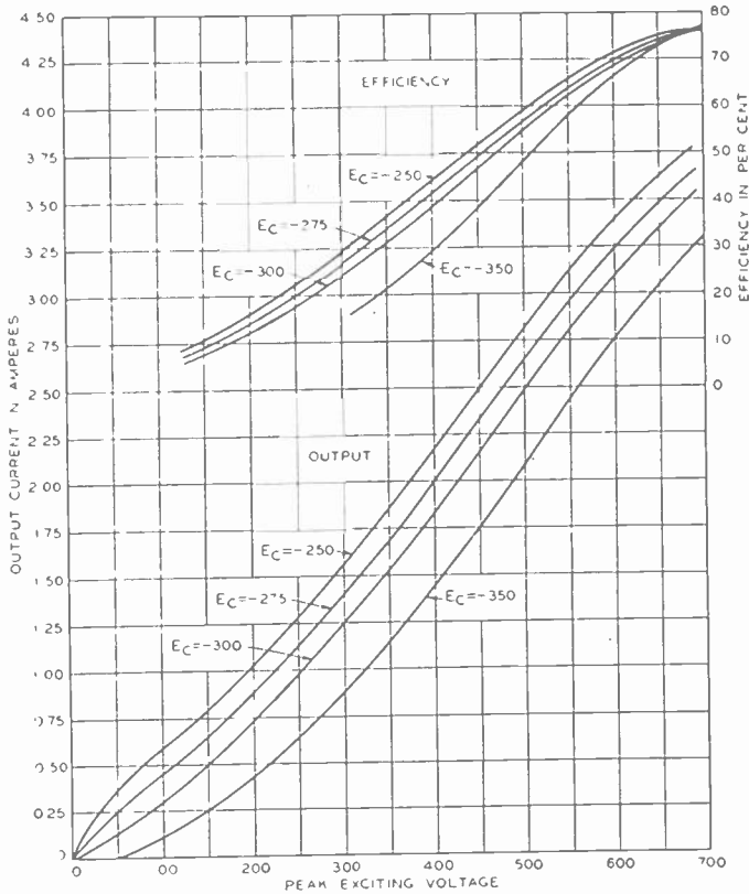
Fig. 12—Dynamic output and efficiency of a three-element tube. E_b = 3000 volts, \mu = 10 , Z_0 = 1500 ohms.
