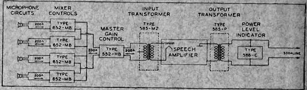
A speech-input unit made up from standard General Radio units.
