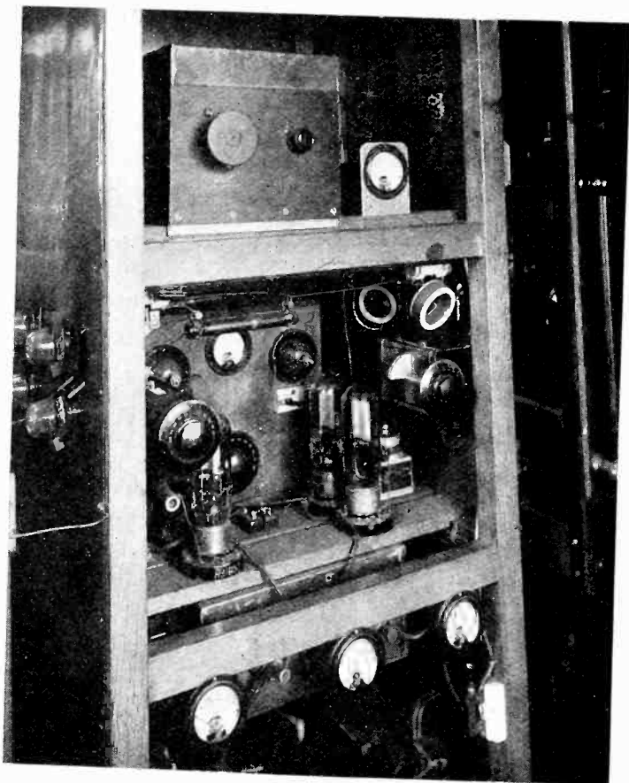
Fig. 5—Front view of master oscillator unit.
