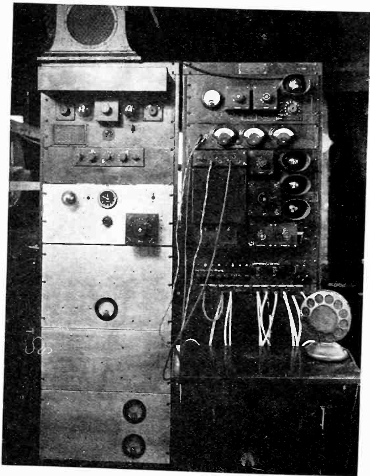
Fig. 10—Speech input equipment.
