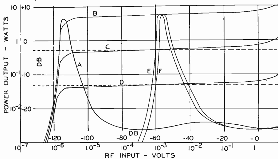
Fig. 6—Overload characteristics; manual vs. automatic sensitivity control.
