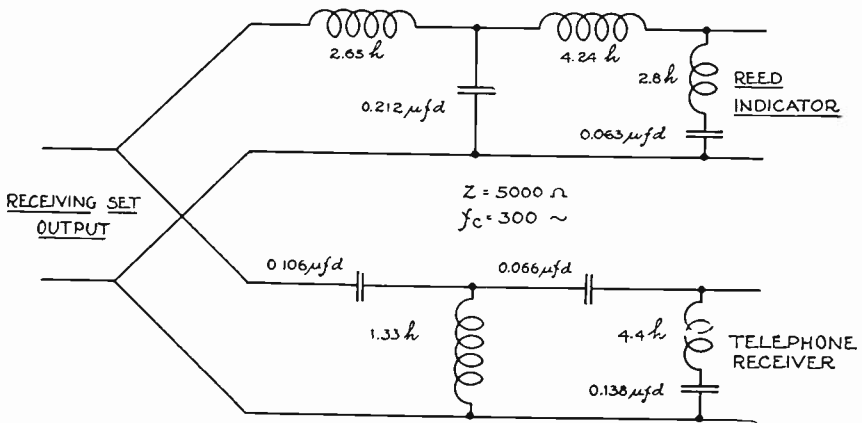
Fig. 21—Filter unit for use on airplane.
