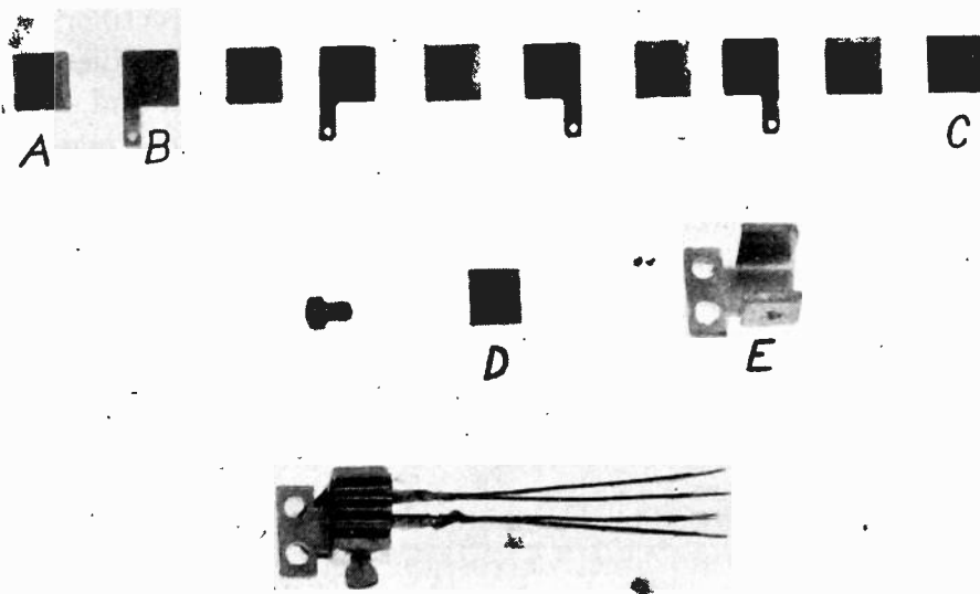
Fig. 3—The copper-oxide full-wave instrument rectifier.
