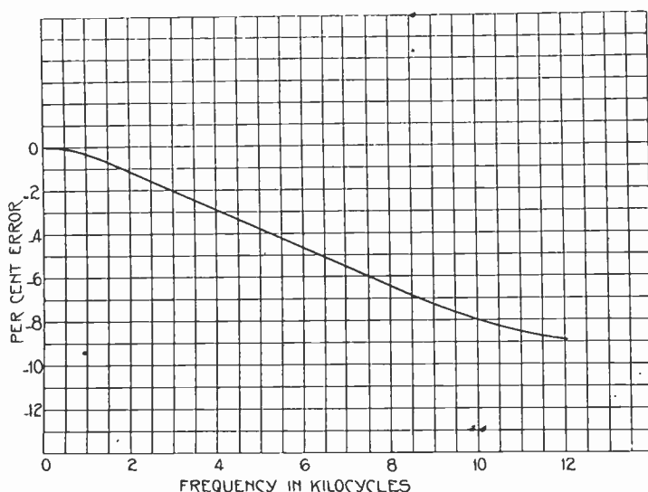
Fig. 8—Frequency characteristics of low range rectifier voltmeters.
