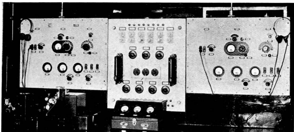
Fig. 6—Telefunken transmitter monitoring apparatus with oscillograph-rectifier, oscillating detector for the third harmonic, amplifier, and rectifier for single and double current and recording equipment for direct monitoring in the immediate vicinity of the transmitter.
