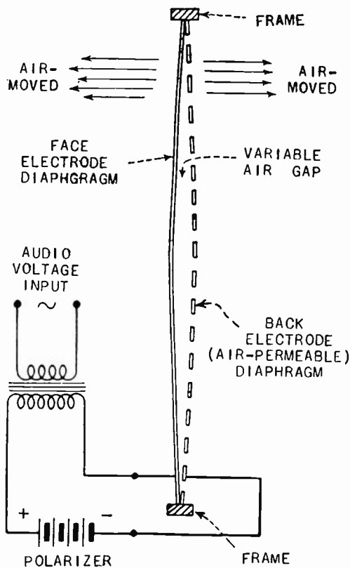
Fig. 2—Operating principle.
