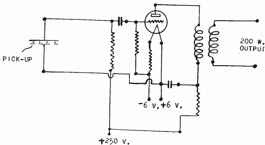
Fig. 8—Pick-up circuit.
