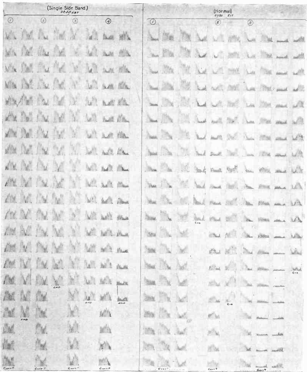
Fig. 10—Distortion of voice band in short-wave transmission.
