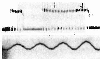
Fig. 12—Rectangular wave-form of the modulation of a short-wave transmitter at Nauen, showing the light point of the oscillograph overshooting the zero line. 50-cycle timing wave at bottom.
