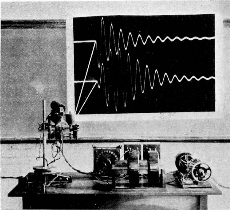
Fig. 3—The transient visualizer with projection oscillograph.
