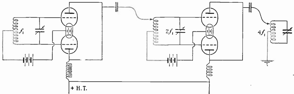
Fig. 5—Theoretical diagram of frequency doubling apparatus.
