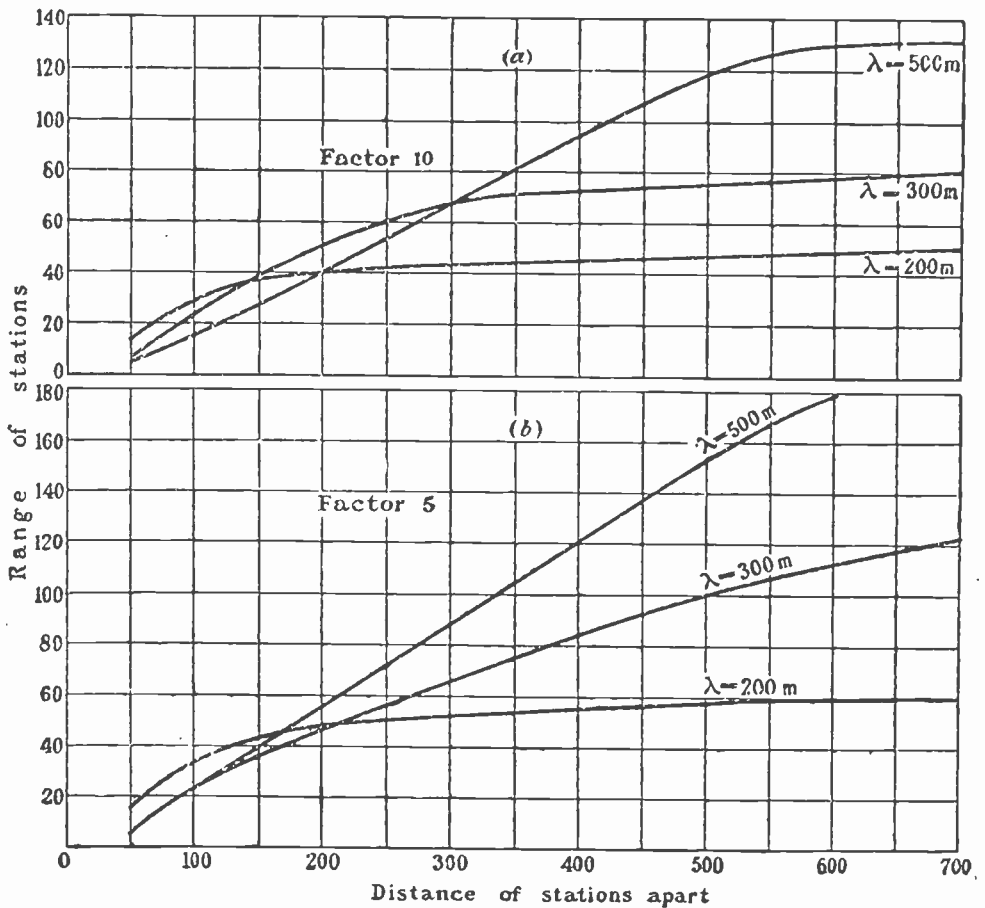
Fig. 3—Range of two equal power stations sharing same wavelength, at different distances apart and different factors.
