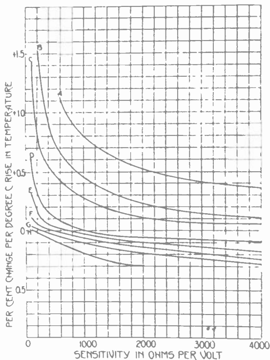
Fig. 10—Temperature coefficients of rectifier voltmeters as a function of voltage range and sensitivity.
