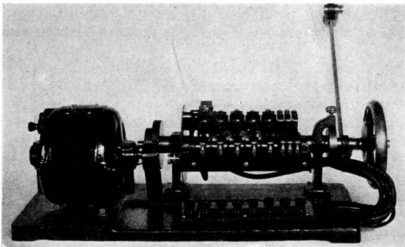
Fig. 2—The transient visualizer.
