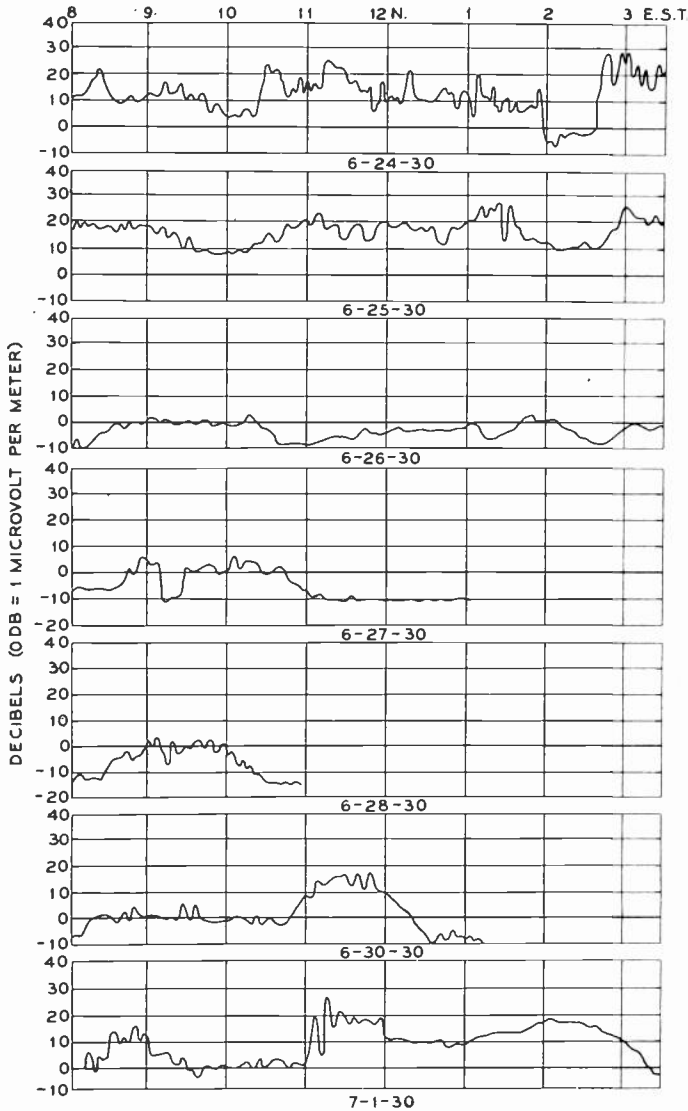
Fig. 9—Magnetic storm effect, oscillograms of received carrier.
