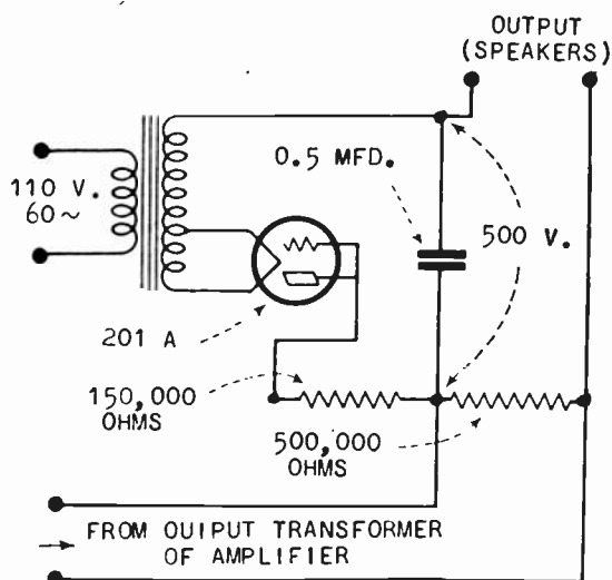
Fig. 7—Polarizer circuit.
