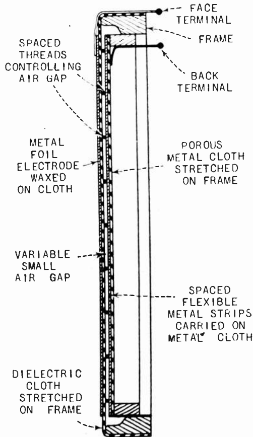
Fig. 1—Acoustic condenser structure.
