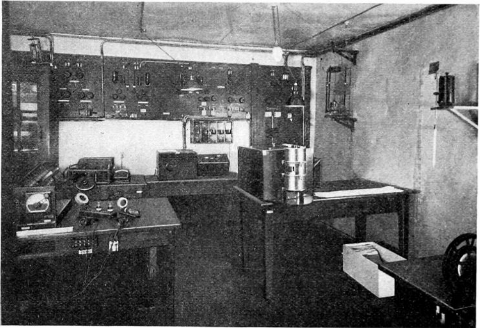
Fig. 3—Continuation of Fig. 2. Left: 160-ke test generator with quartz standards. Right: standard test circuit with mirror galvanometer and reading lamp. Center at rear: rough measuring apparatus.
