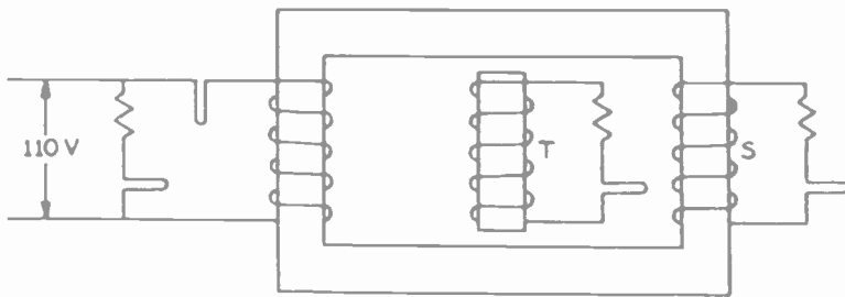
Fig. 10—Circuit diagram of magnetic shunt transformer.
