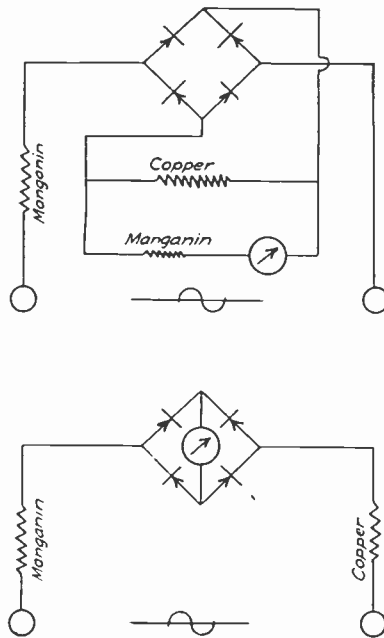
Fig. 13—Compensating schemes for temperature errors.
