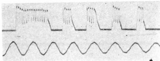
Fig. 10—Monitor record of a short-wave transmitter at Nauen with slightly distorted signaling. 50-cycle timing wave at bottom.
