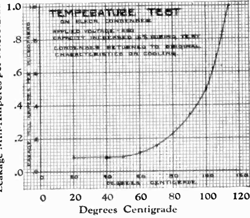
TEMPERATURE TEST on Elkon Condenser Applied Voltage 450. Capacity Increased 16% During Test. Condenser Returned to Original Characteristics on Cooling.
