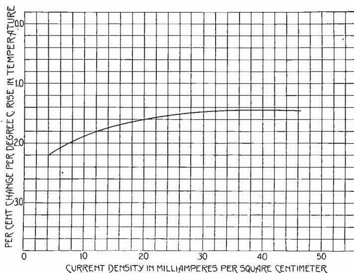
Fig. 11—Temperature coefficient of rectification ratio.
