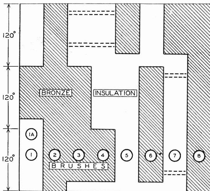
Fig. 1—A development of transient visualizer drum.
