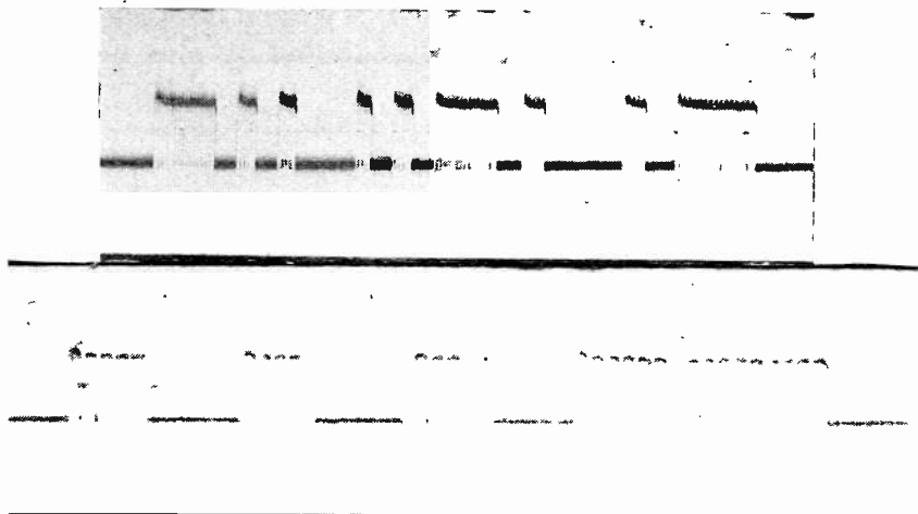
Fig. 11—100 per cent modulation of a short-wave transmitter at Nauen with good keying at a speed of 240 words per minute; above for slow, and below for fast, operation of the oscillograph drum.
