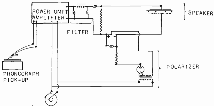
Fig. 5—Operating circuit.
