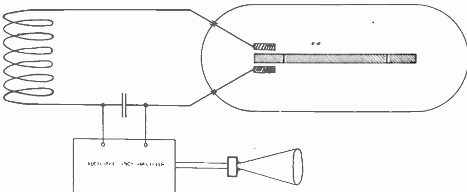
Fig. 7—Diagram of a luminous resonator excited in the 4th harmonic, with coupling coil and amplifier for acoustic determination of resonance.
