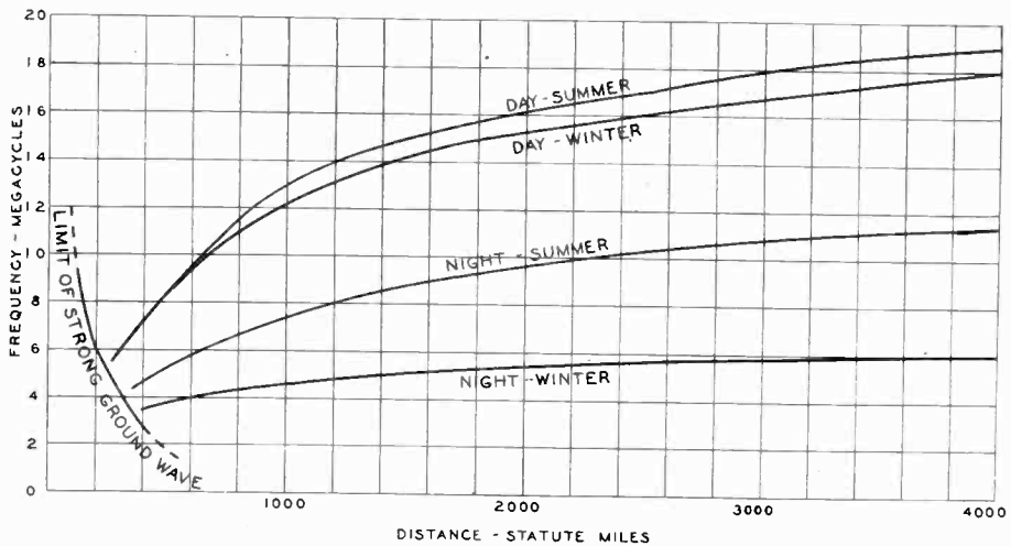
Fig. 11—Frequency-distance characteristic.
