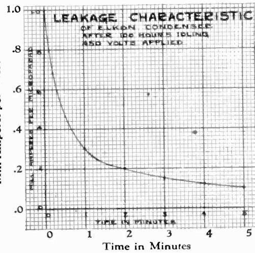
(Above) Leakage Characteristic of Elkon Condenser after 100 Hours Idling 450 Volts Applied
