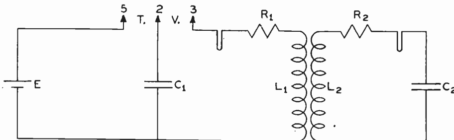
Fig. 4—Diagram of connections for coupled circuits.
