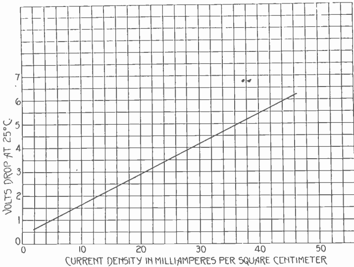
Fig. 5—Forward voltage—current density characteristics.
