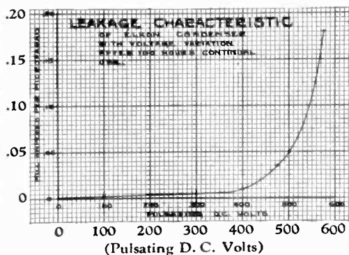
(Above) Leakage Characteristic of Elkon Condenser with Voltage Variation after 100 Hours Continual Use
