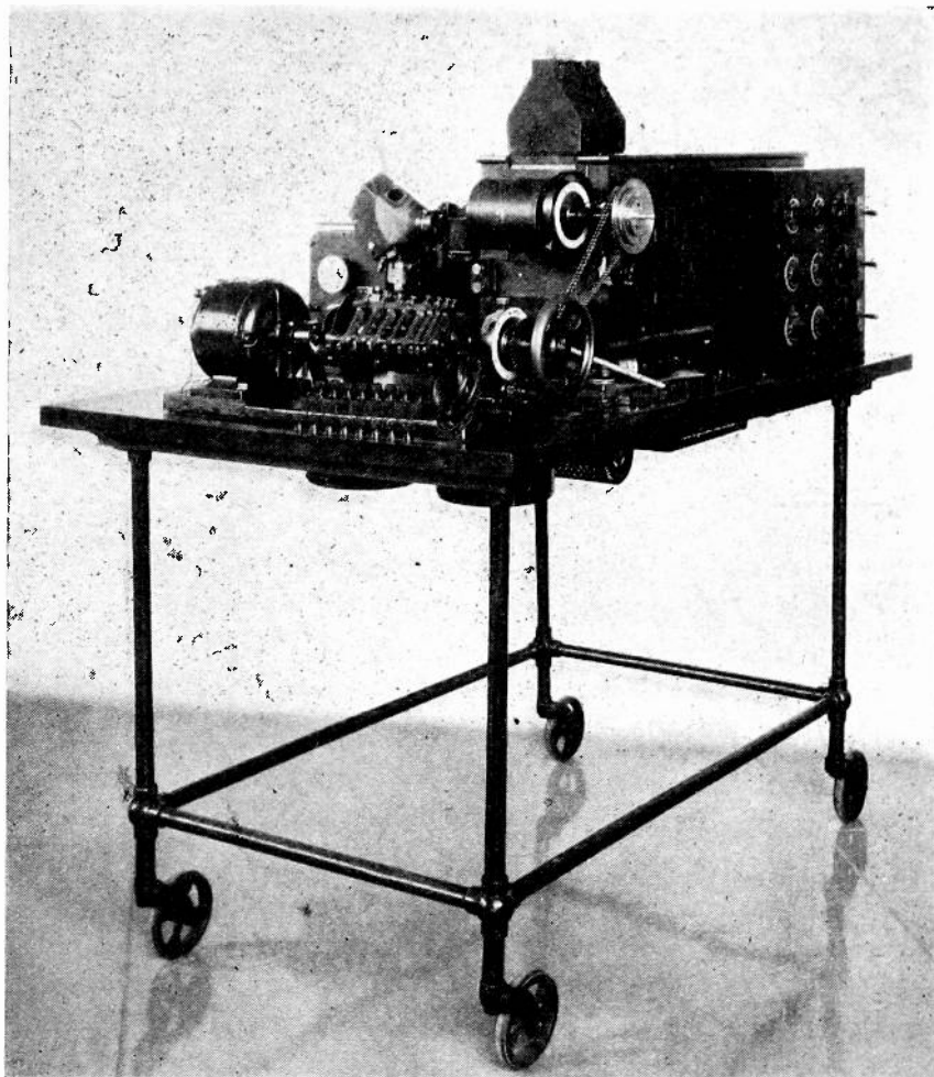
Fig. 5—Equipment arranged for obtaining coördinated oscillograms.
