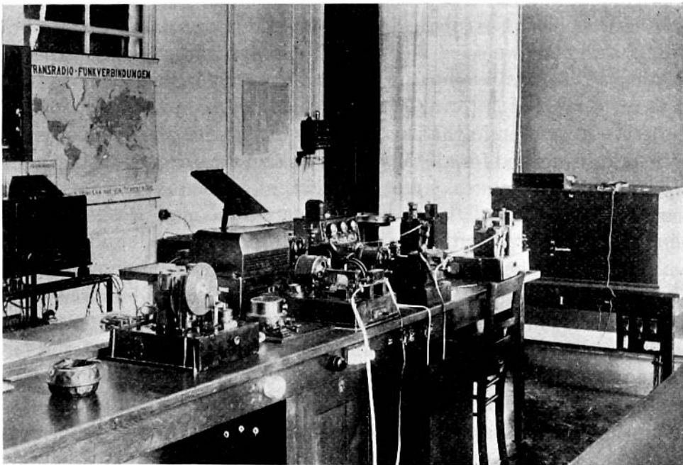
Fig. 11—Partial view of the Nauen monitoring room.
