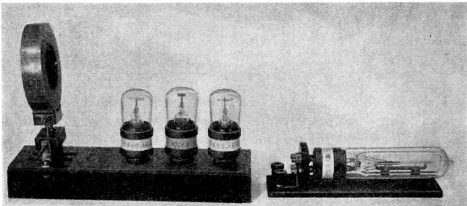
Fig. 4—Old (left) and improved (right) luminous quartz resonators.
