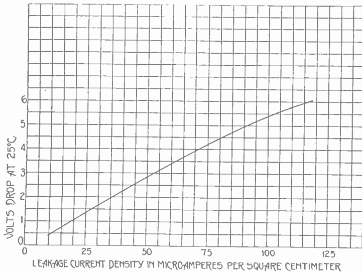
Fig. 7—Leakage voltage—current density characteristics.
