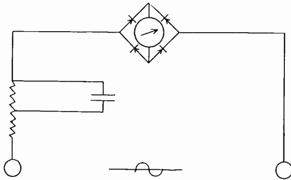
Fig. 9—Diagram of frequency compensation.
