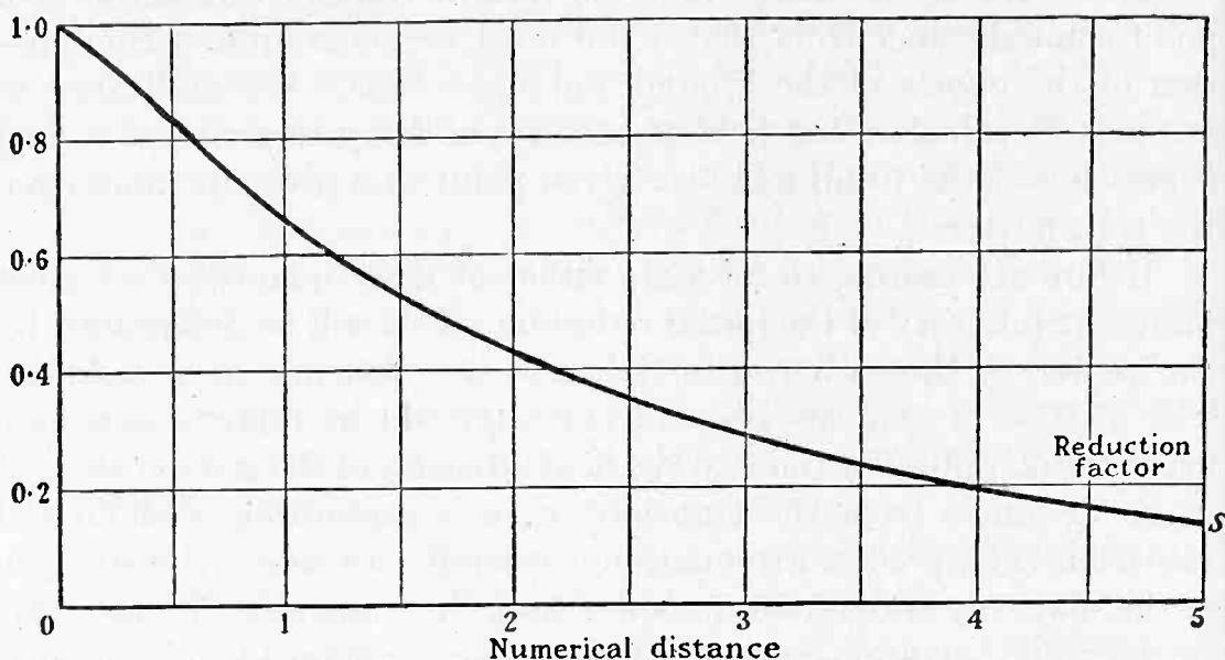
Fig. 1—Sommerfeld's theory.
