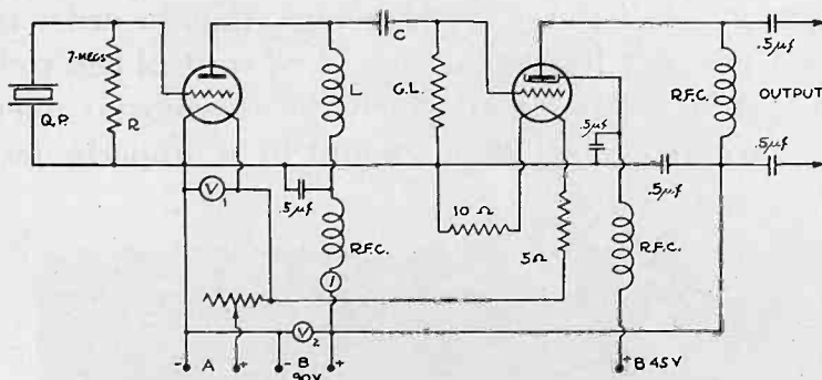
Fig. 1—Complete piezo-oscillator circuit diagram.
