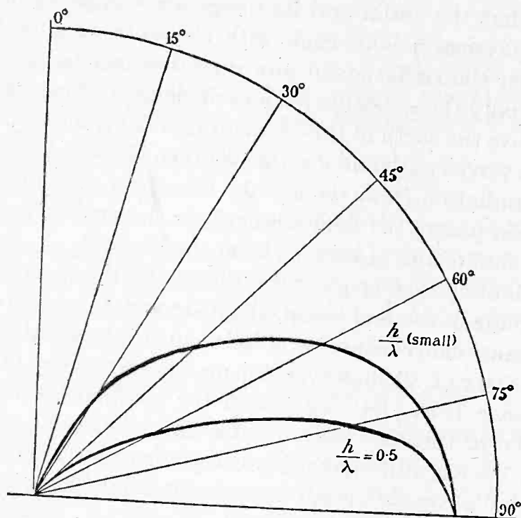
Fig. 5—Vertical polar diagram of radiation for 1/2-\lambda and 1/4-\lambda (or less) aerials. Drawn for the same maximum radiation intensity in the horizontal plane. (Stuart Ballantine, loc. cit.)
