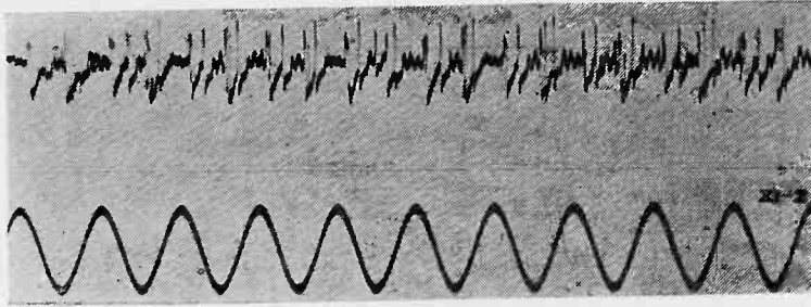
Fig. 16—One-inch arc between copper 1.03 amperes, 5730 v.
