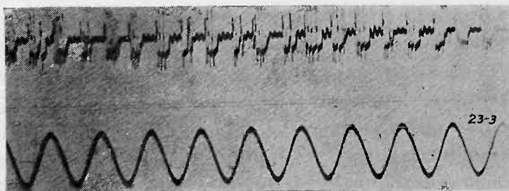
Fig. 13—Leakage from cut-out hangers to brace bolts on cross-arm.
