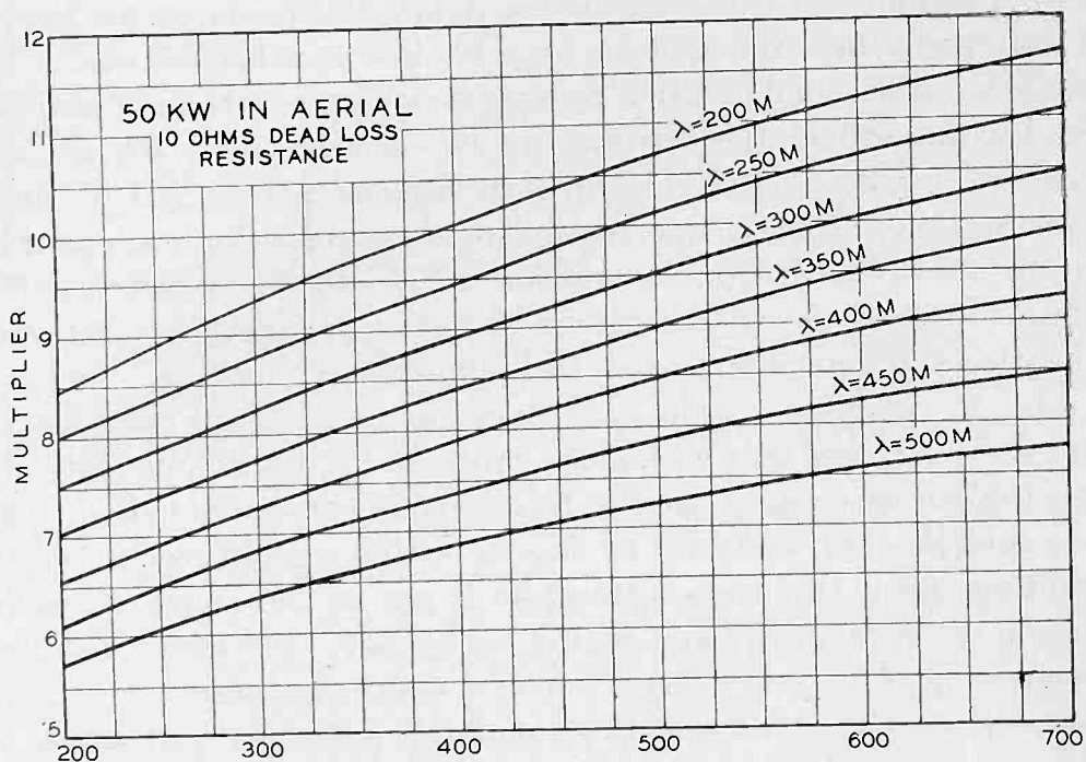
Fig. 11—Multipliers for theoretical attenuation curves.
