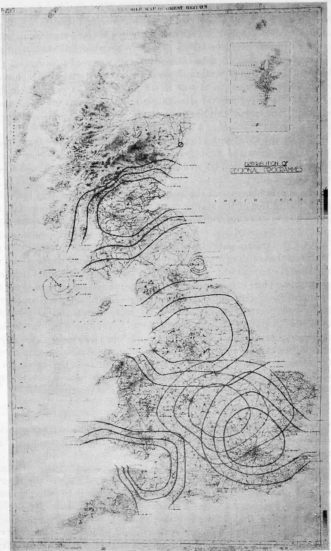
Fig. 13—Field-strength contours, calculated regional programs.
