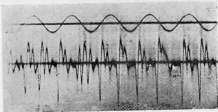
Fig. 5—Violet-ray appliance.
