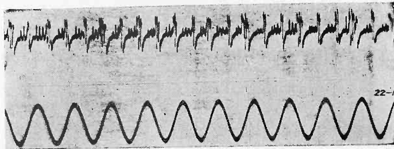
Fig. 14—Cut-out with arcing contact 2880 v.
