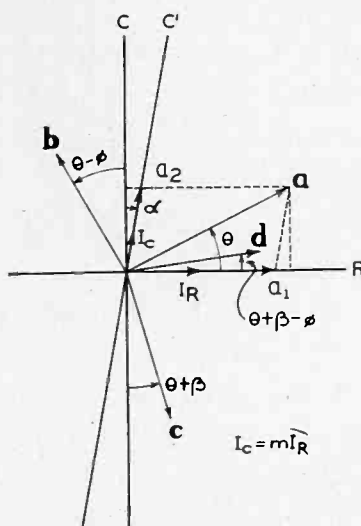
Fig. 4—Vector relations of potentiometer axes and test voltages.
