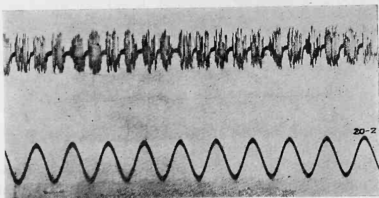
Fig. 11—High resistance found on 6900 v.
