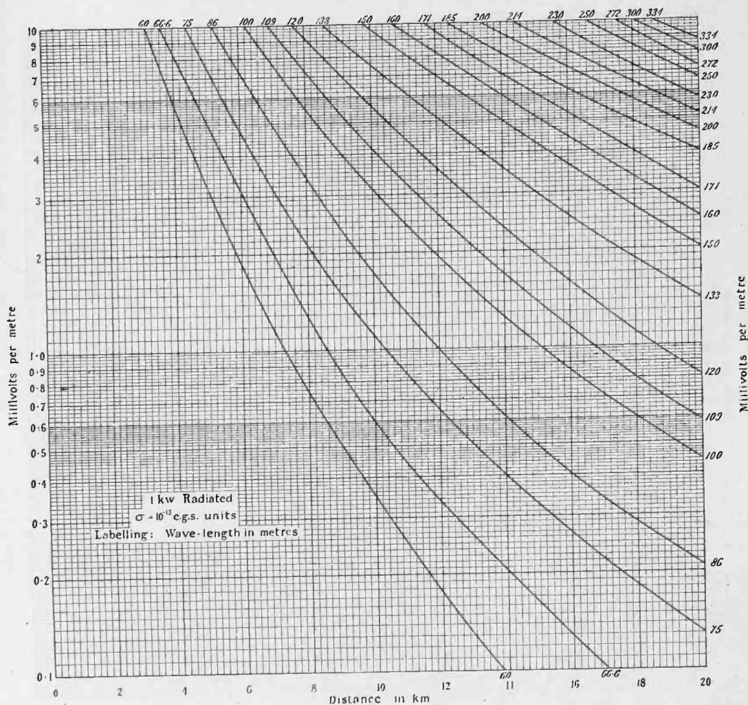
Fig. 2a—Field intensity vs distance (attenuation curves).
