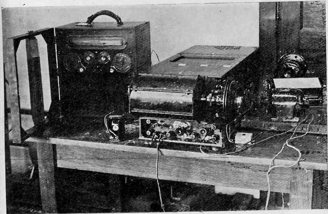
Fig. 1—Portable radio receiver, coupling transformer, and the oscillograph. ular frequency and this gives no indication of the source of interference.
