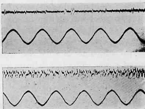
Fig. 10—Interferences sometime found on 33,000-v, 60-cycle line.
