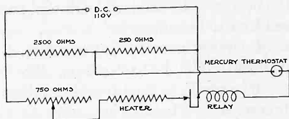
Fig. 2—Temperature-control circuit diagram.
