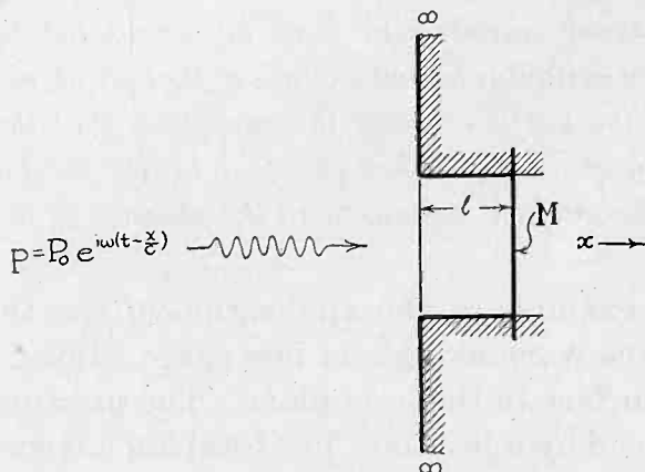
Fig. 1—Illustrating circular membrane at end of cavity of length l ; infinite baffle.
