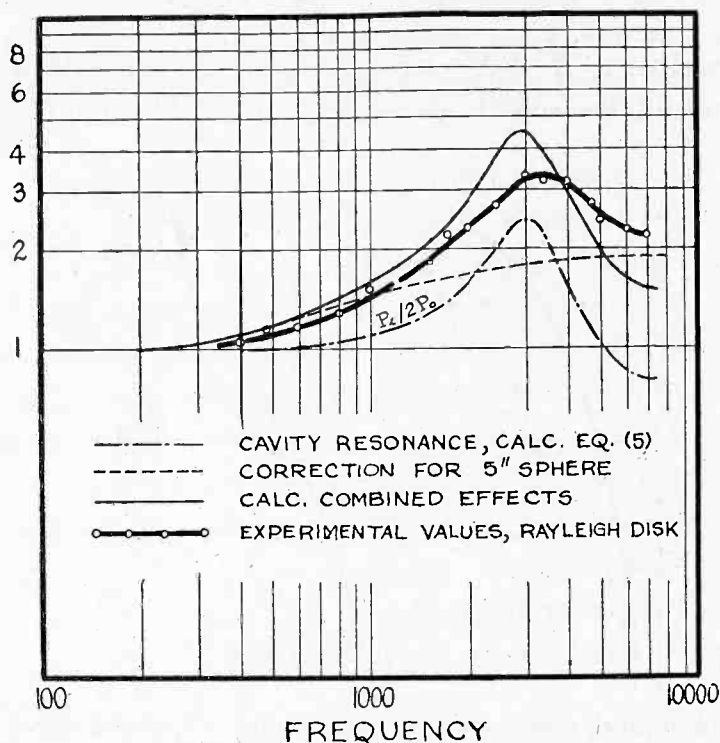
Fig. 3—Calculated and experimental (Rayleigh disk) values of increase of response due to cavity resonance and to reflection; condenser microphone No. 2.
