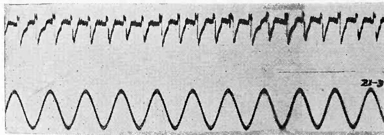
Fig. 15—One-fourth-inch arc between copper 1.03 amperes, 5730 v.
