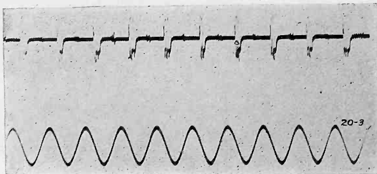
Fig. 12—Leakage across open cut-out 6900 v.
