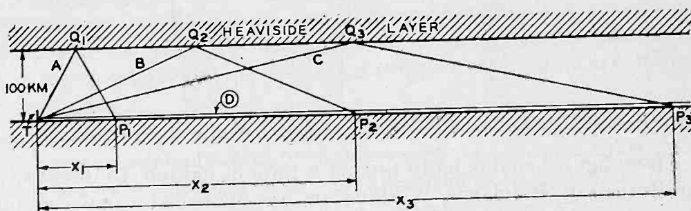
Fig. 4—Illustration of assumptions made in considering effect of space ray.
