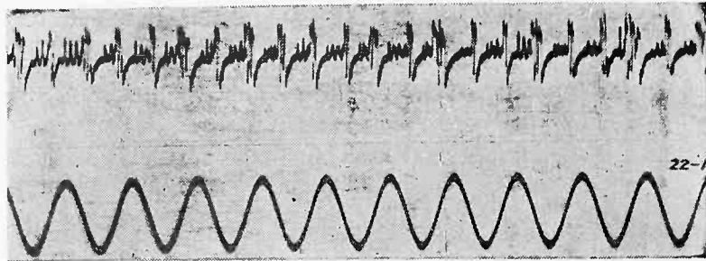
Fig. 14—Cut-out with arcing contact 2880 v.
