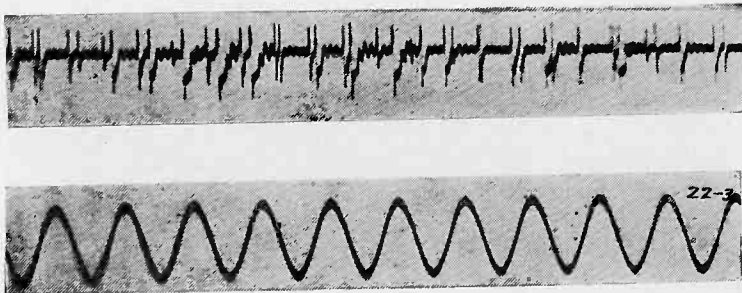
Fig. 17—One-inch arc between steel rods 1.03 amperes, 5730 v.
