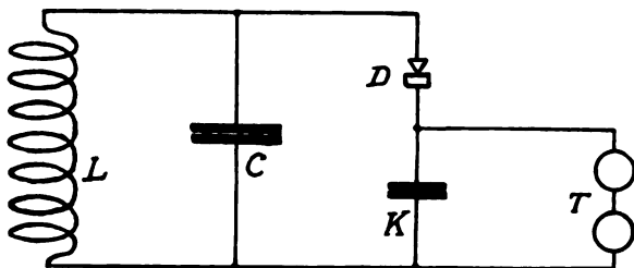
FIGURE 1—Typical Detector Circuit
