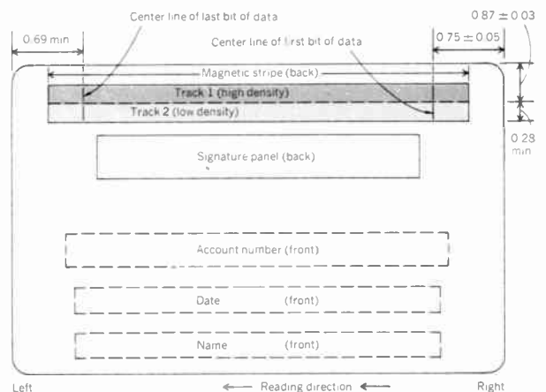
[1] Magnetic-stripe credit card layout. Standard specifications include both machine-readable stripe and embossed characters for optical character recognition applications. Dimensions are in cm.
