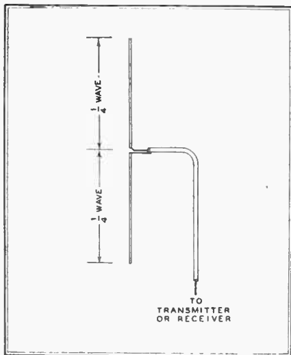
FIG. 1. SIMPLE VERTICAL HALF-WAVE DIPOLE
