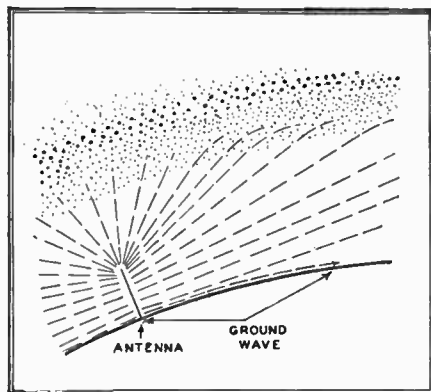
FIG. 24. LEFT: AM BROADCAST TRANSMISSION DURING DAYLIGHT HOURS IS BY MEANS OF THE GROUND WAVE. SKYWARD TRANSMISSION IS ABSORBED IN REGION BELOW E LAYER. RIGHT: AT NIGHT, SKYWAVES, RETURNED TO EARTH, GIVE LONG-DISTANCE COVERAGE, BUT CAUSE FADING IN THE OUTER PORTION OF THE AREA REACHED BY THE GROUND WAVE
