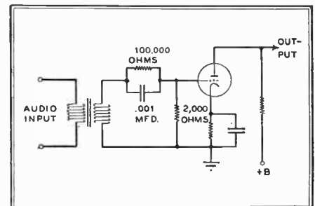
FIG. 48. NETWORK FOR INTRODUCING PRE-EMPHASIS
