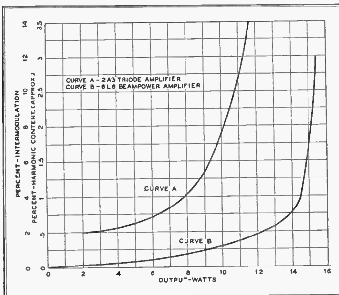
FIG. 9. COMPARISON OF INTERMODULATION WITH 2A3'S AND 6L6'S
