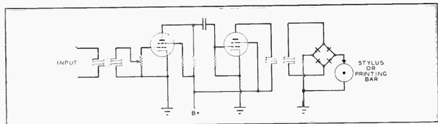
FIG. 6. AMPLIFIER AND FULL-WAVE RECTIFIER EMPLOYED FOR FACSIMILE RECORDING
