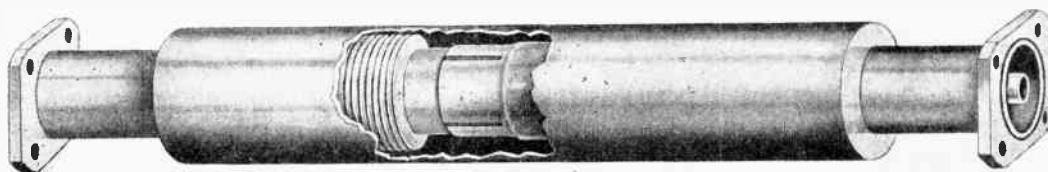
FIG. 15. THIS EXPANSION FITTING IS DESIGNED TO INTRODUCE ONLY NEGLIGIBLE REFLECTIONS IN THE LINE
