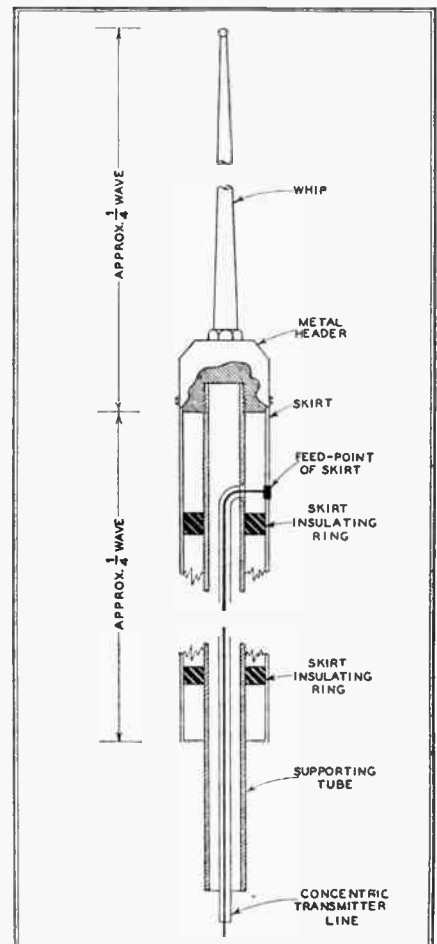
FIG. 5. SHUNT-FED TYPE OF COAXIAL, VERTICALLY POLARIZED ANTENNA
