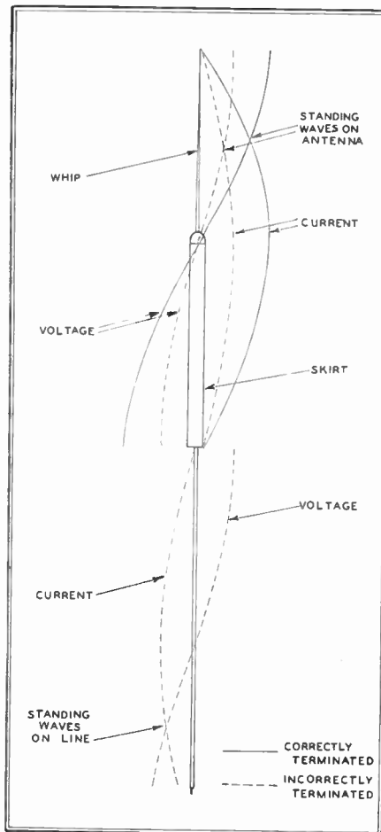
FIG. 6. EFFECTS OF CORRECT AND INCORRECT ANTENNA TERMINATIONS
