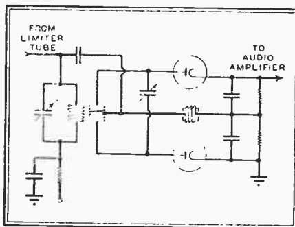
FIG. 62. CENTER-TUNED TYPE OF DISCRIMINATOR CIRCUIT
