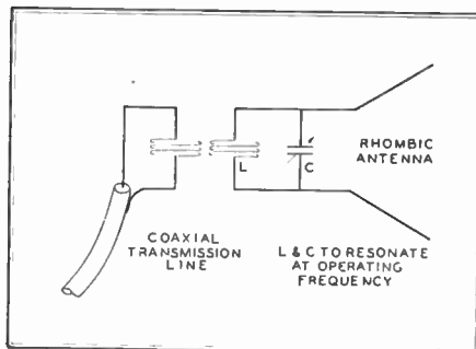
FIG. 14. SIMPLE MATCHING TRANSFORMER
