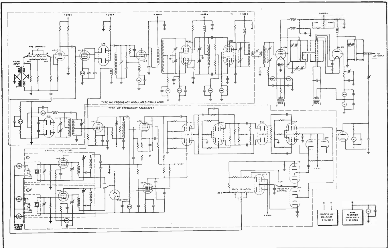
Schematic diagram of a 1-kw FM transmitter. In type FM-3 transmitter, the r.f. driver has two type 4-125A tubes, and the power amplifier uses two type WL-473A tubes, both in push-pull, and the h.v. rectifier uses six type WL-872A tubes.
