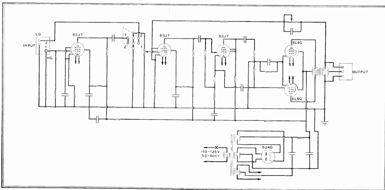
FIG. 10. SCHEMATIC DIAGRAM OF THE AMPLIFIER DESIGNED TO DRIVE THE DUPLEX TYPE LOUDSPEAKER
