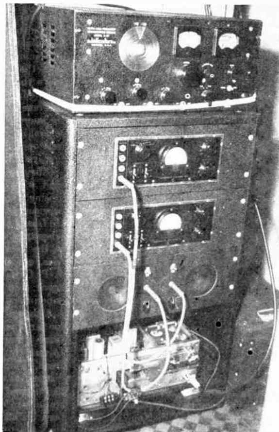
FIG. 7. VISUAL AND AUDIO EQUIPMENT USED ON THE ROCK ISLAND TEST CAR FOR MEASURING RADIO RECEPTION
