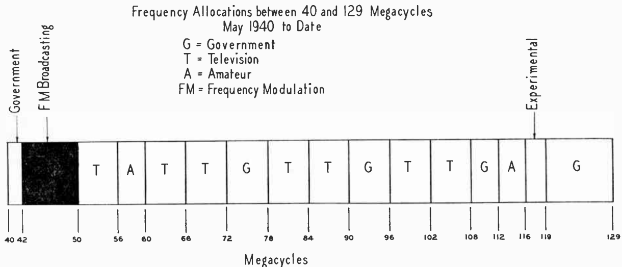
FIG. 2. FREQUENCY ALLOCATIONS, 40 TO 129 MC., AS THEY WERE SET UP BY THE FCC IN MAY, 1940
