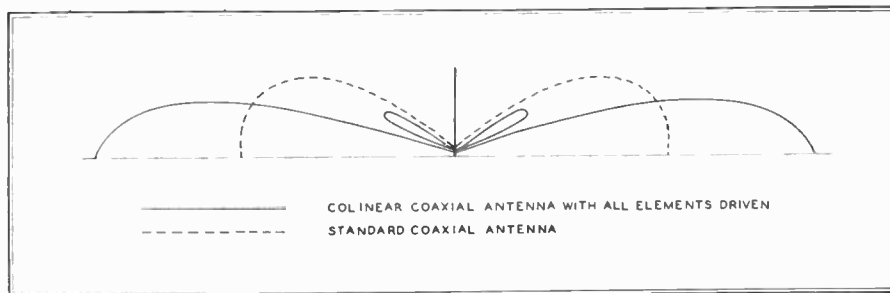
FIG. 11. LOWER ANGLE OF RADIATION GIVES COLINEAR COAXIAL GREATER RANGE
