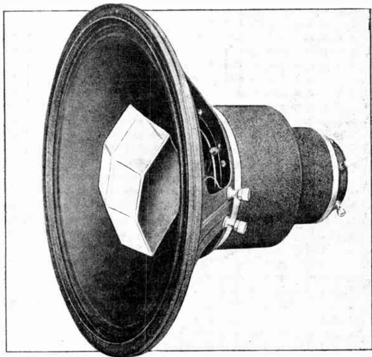
FIG. 1. THE ASSEMBLED DUPLEX SPEAKER, SHOWING POSITION OF THE DIFFUSER
