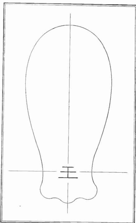
FIG. 16. RADIATION PATTERN OF THE HORIZONTAL REFLECTOR-DIRECTOR
