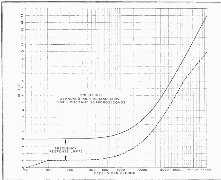
FIG. 3. STANDARD PRE-EMPHASIS CURVE. TIME CONSTANT 75 MICROSECONDS
