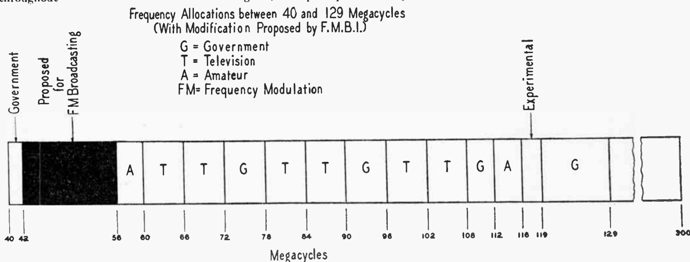
FIG. 4. AMPLE CHANNELS WERE MADE AVAILABLE FROM 129 TO 300 MC. TO COMPENSATE TELEVISION FOR GIVING 50 TO 56-MC. BAND TO FM
