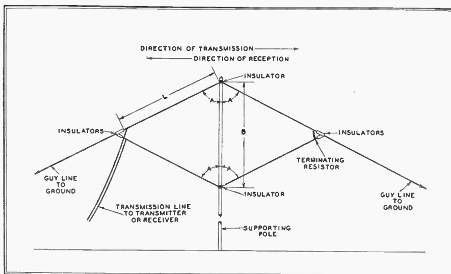
FIG. 12. FULL RHOMBIC IS FOR HIGHLY DIRECTIONAL TRANSMISSION OR RECEPTION
