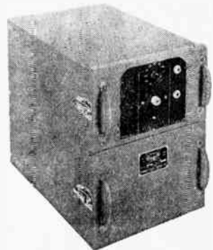
COMCO Model 210, 15 Watt, FM VHF 152-162 Megacycles Mobile Transmitter Receiver for Taxicabs, Police Cars, etc. Size 10 \frac{1}{4} " x 13 \frac{1}{2} " x 14 \frac{3}{4} ", weight 50 lbs.
