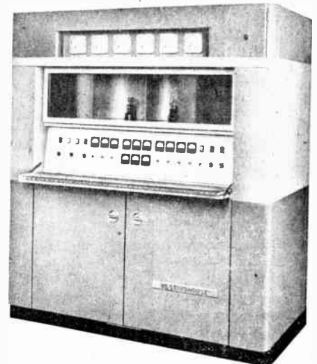
Centrally-located control panel is easily accessible through door that folds out of the way. Control panel includes power switches; electrically-driven tuning controls and their position indicating instruments; 6 meters in center panel associated with low power stages; controls for continuously variable line voltage and P.A. plate voltage and indicator lights.
