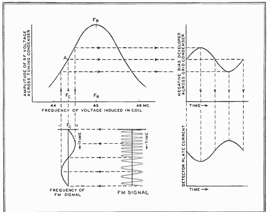
FIG. 50. TUNED-CIRCUIT DETECTION FROM ELEMENTARY RECEIVER, FIG. 49
