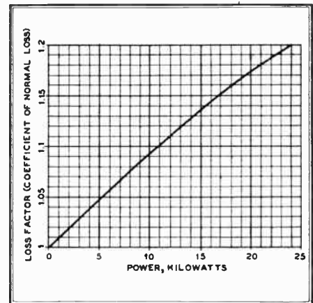
FIG. 10. RESISTANCE & INSULATION LOSS
