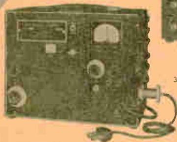
MODEL 78 - FM STANDARD SIGNAL GENERATOR 86 to 108 megacycles. Output: 1 to 100,000 microvolts
