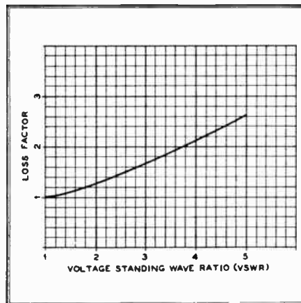
FIG. 9. LOSSES DUE TO STANDING WAVES
