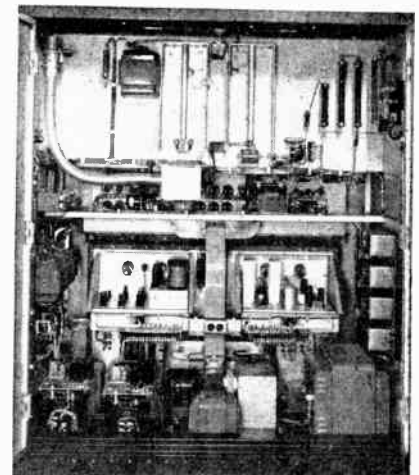
Large windows in rear doors permit inspection of interior. Flexible output transmission line can be seen at upper left. Note convenience power outlet, and lamp for lighting mounted at top of cubicle.
