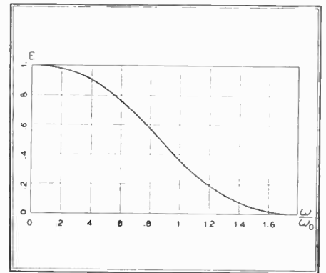
FIG. 3. NETWORK CHARACTERISTIC
