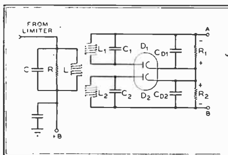
FIG. 59. DETUNED-CIRCUIT TYPE OF DISCRIMINATOR CIRCUIT
