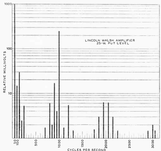
FIG. 9. L-W AMPLIFIER AT 25-WATT OUTPUT LEVEL
