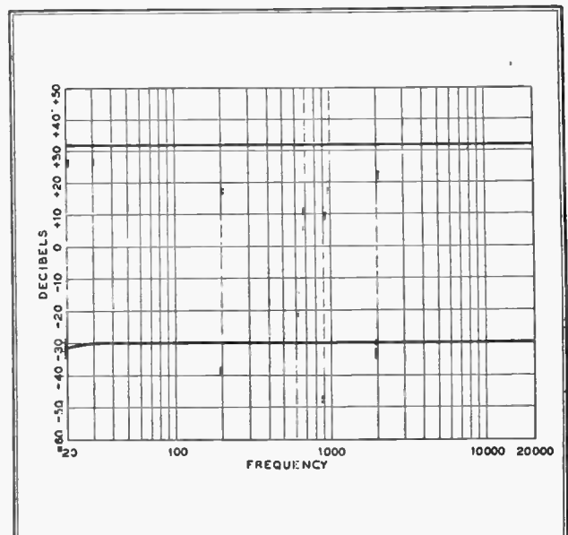
FIG. 11. FREQUENCY CHARACTERISTICS OF THE AMPLIFIER
