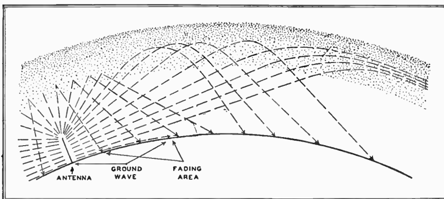
FIG. 24. LEFT: AM BROADCAST TRANSMISSION DURING DAYLIGHT HOURS IS BY MEANS OF THE GROUND WAVE. SKYWARD TRANSMISSION IS ABSORBED IN REGION BELOW E LAYER. RIGHT: AT NIGHT, SKYWAVES, RETURNED TO EARTH, GIVE LONG-DISTANCE COVERAGE, BUT CAUSE FADING IN THE OUTER PORTION OF THE AREA REACHED BY THE GROUND WAVE
