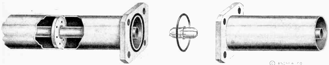
FIG. 11. CONSTRUCTION OF JOINTS FOR INNER AND OUTER CONDUCTORS, AND GAS SEAL BETWEEN 20-FT. LENGTHS
