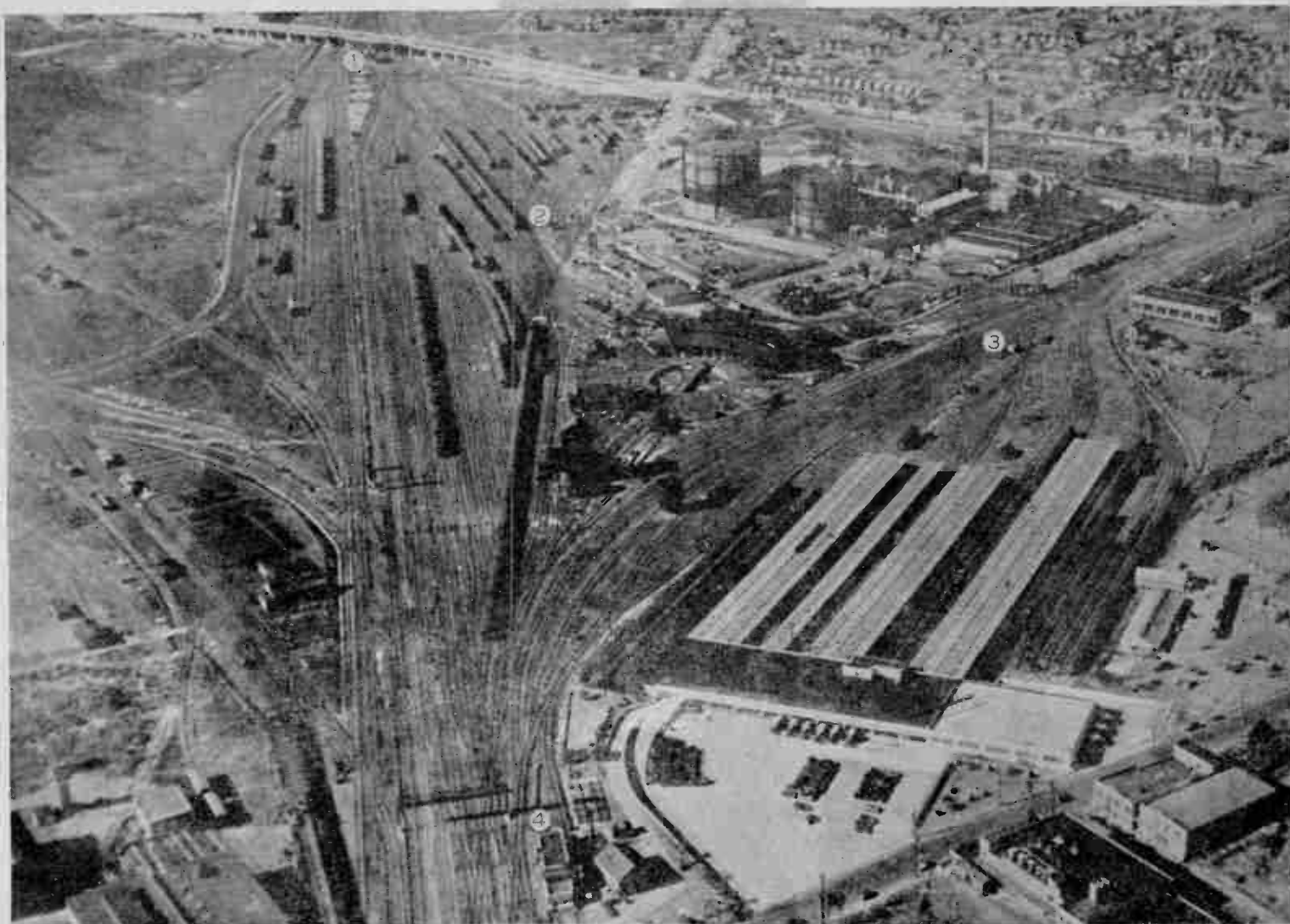
FIG. 13. WESTERN END OF THE TERMINAL. MYRTLE VENUE TRANSMITTER-RECEIVER, POINT 4, CAN BE OPERATED REMOTELY FROM BEAVER STREET TOWER, POINT 1; FROM YARDMASTER'S OFFICE, POINT 2, IN THE COACH YARD; OR FROM THE YARDMASTER'S OFFICE IN THE RAILWAY EXPRESS PLANT, POINT 3. ALL SWITCHING ENGINES ARE WITHIN RADIO RANGE OF 1 OR 2.
