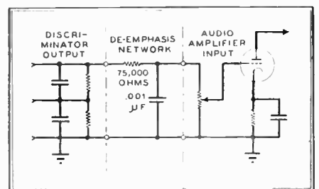
FIG. 66. POSITION OF DE-EMPHASIS NETWORK IN FM RECEIVER
