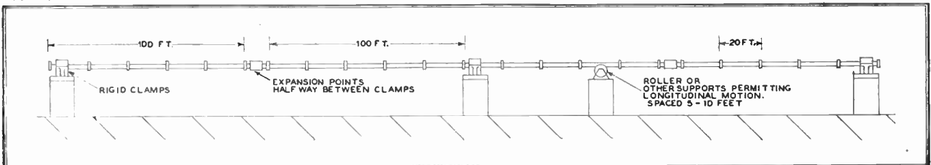
FIG. 23. PROPOSED CONSTRUCTION FOR A LONG LINE COMBINES RIGID AND ROLLER MOUNTS, AND EXPANSION JOINTS
