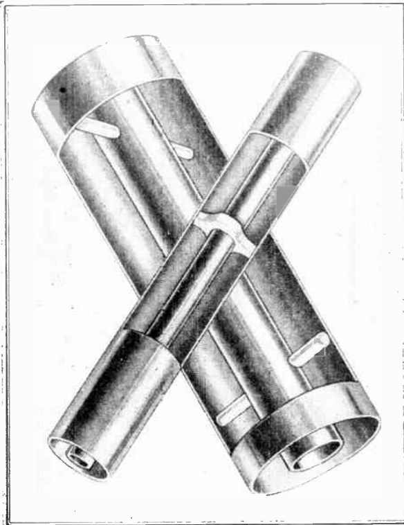
FIG. 1. INTERNAL CONSTRUCTION OF COAXIAL LINES
