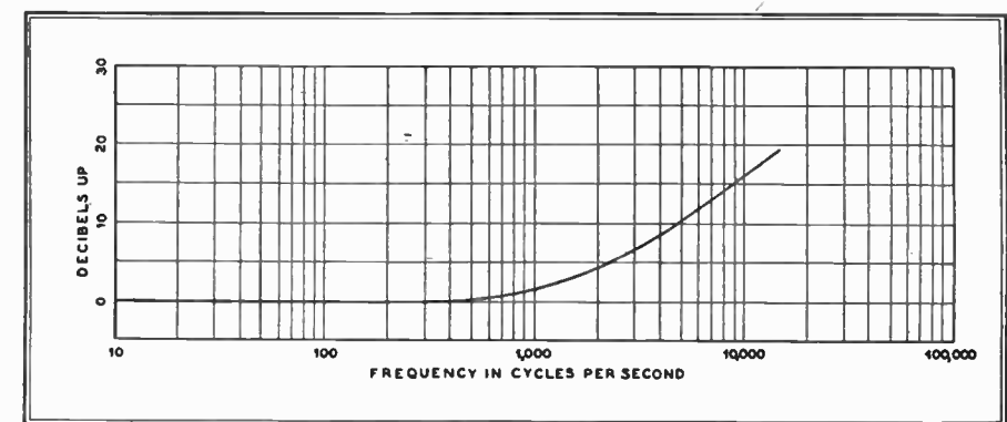
FIG. 16. STANDARD PRE-EMPHASIS CHARACTERISTIC FOR FM TRANSMITTERS
