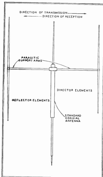
FIG. 17. REFLECTOR AND DIRECTOR ADDED TO A COAXIAL TYPE ANTENNA
