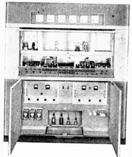
All openings to live circuits are equipped with interlocks and grounding switches. Aluminum cubicle provides excellent shielding at 100 mc. In lower section of cubicle are plug-in frequency modulated master oscillator and frequency control units, low-voltage rectifier tubes and high voltage rectifier tubes. Relays, left to right, are: 250, 400 and 2000-volt overload protection; bias protection for r.f. driver and P.A. tubes, and time delay relay to protect mercury vapor rectifier tubes.
