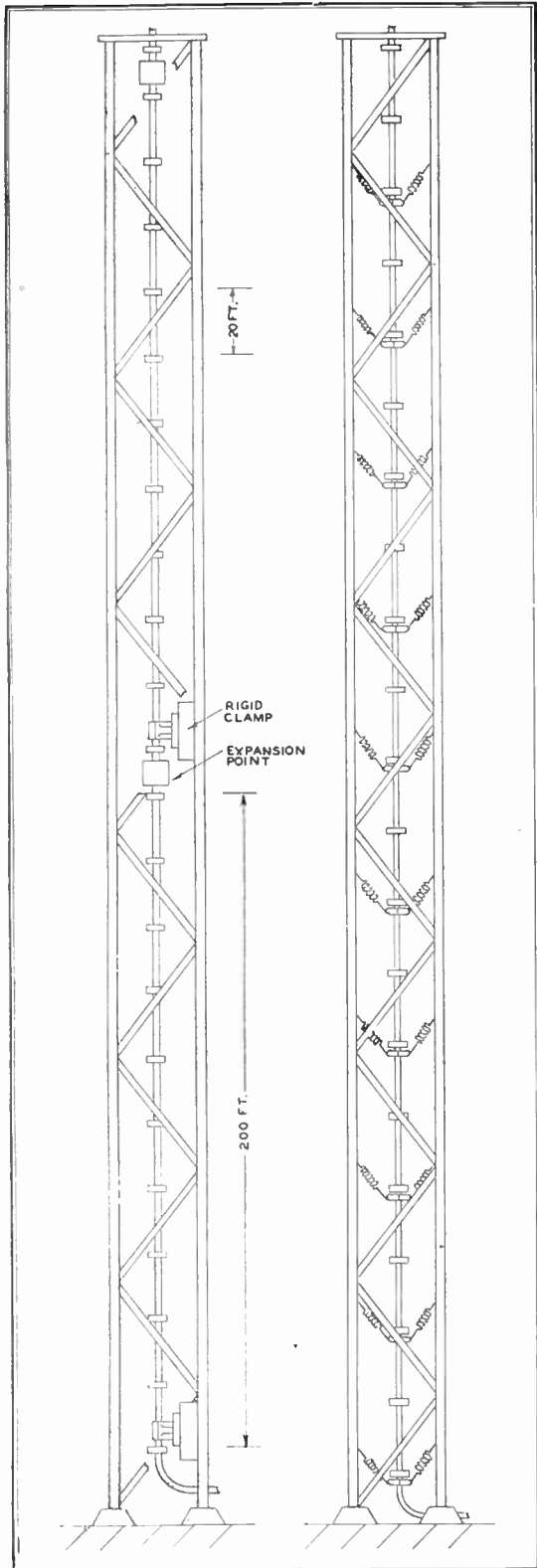
FIG. 21A, LEFT. RIGID LINE MOUNTING. FIG. 21B, RIGHT. SPRING SUSPENSION FOR VERTICAL RUN
