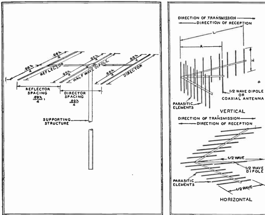
FIG. 15, LEFT: A HORIZONTALLY POLARIZED DIPOLE AND DIRECTIVE ARRAY. FIG. 18, RIGHT: VERTICAL AND HORIZONTAL TYPES OF CORNER REFLECTOR ANTENNAS
