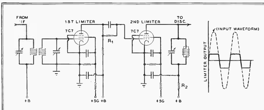
FIG. 58. CIRCUIT NOT EMPLOYING GRID LEAK IN THE FIRST STAGE. RIGHT, CURVES SHOWING THE INPUT WAVE FORM AND RESULTING OUTPUT
