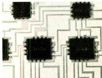
Beam lead bonding techniques are simpler and permit closer spacing of chips.
