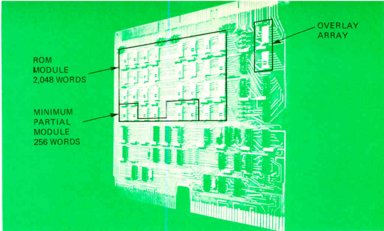
2. Overlay key. In this implementation, ROM module is 2,048 words, but the minimum ROM block is 256 words. To permit overlay by individual words, an extra 2,048-bit overlay array (upper right) is added to the module, identifying each word as "valid" or "not valid."
