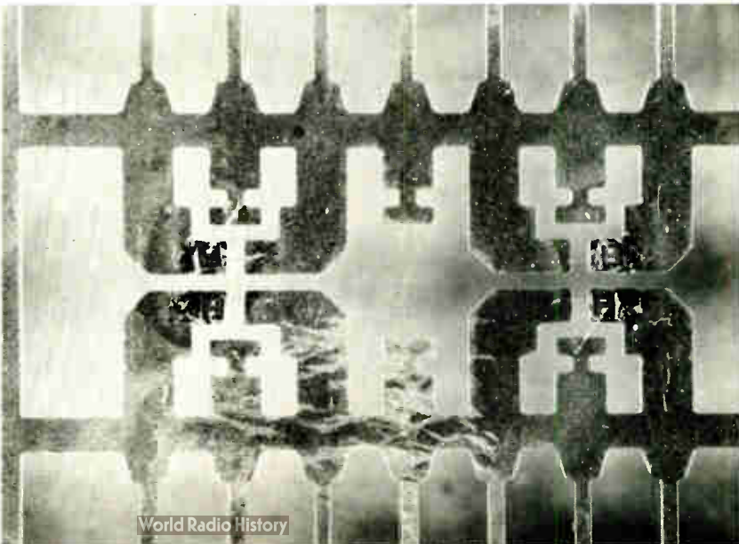
Growth. Outside the power area, field-effect transistors and multiple devices are hot items and growing hotter. Above is a dual-gate FET for tuner/mixer applications; left, a diode array in a single package for computer switching; right, four diodes on a single lead-frame for driving core memories. All are from TI.
