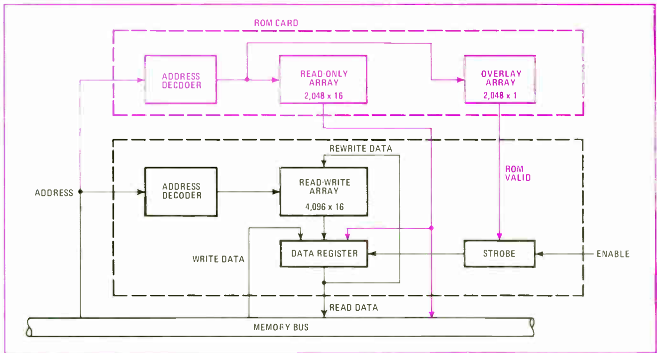
3. Overlaid connections. Read-write memory is conventional in every respect (black). Data from overlaid read-only memory (color) enters data register and is copied back into read-write array. Overlay array identifies the ROM words for which overlay occurs.
