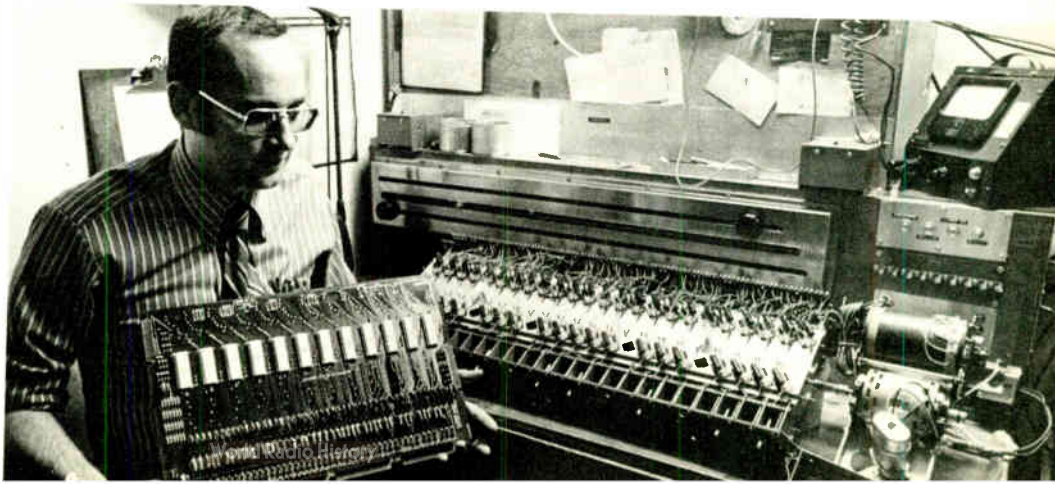
The new and the old. John L. Lavey, manufacturing vice president, holds Hammond's new LSI tone generator. Old electro-mechanical model is atop the desk beside him.
