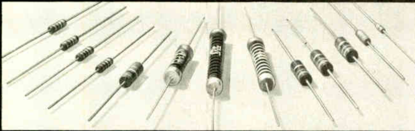
CARBON COMPOSITION
