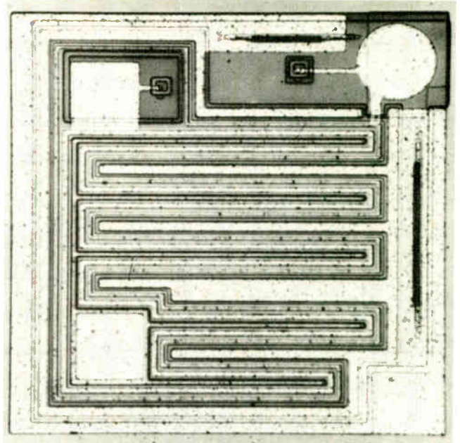
FET blanket. TI's new double-gate FET is one of many that have a nitride-passivated coating to increase stability.
