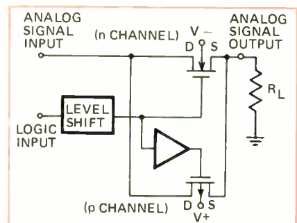
Analog switch. Latch-up is avoided by floating gate with extra diode (not shown).
