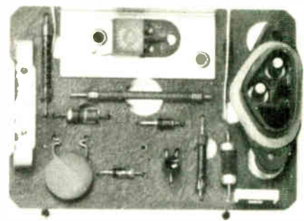
Under the hood. Chrysler unit contains a 40-V, 3-4-A discrete device from RCA, typifying use for cars' voltage regulators.
