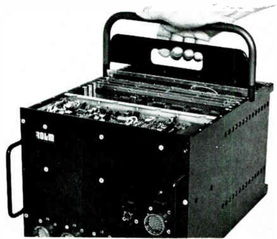
5. Painless extraction. The boards can be removed with a special handle. The holes in the sidewall hold screws that tighten the wedges.
