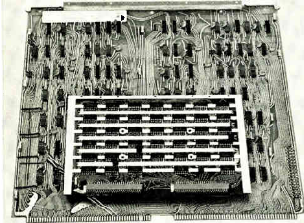
1. Down to size. For ruggedization, 15-inch circuit board in Nova is replaced by 7-by-10-inch board, which is less likely to bend or break. For better cooling, copper frame runs under IC packages, while copper buses between packages handle power distribution. Fork-type pc connectors replace plated-edge connections on Nova board. Four holes near center of board are for screws that hold board cover.
