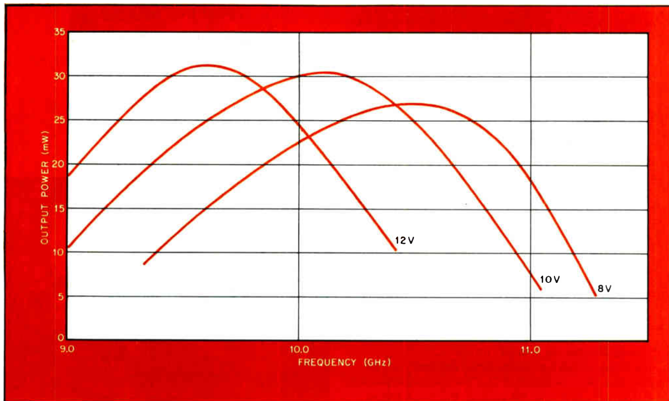
3. Output power. Operating frequency of a typical 10-mW Gunn flange oscillator varies with dc bias, but the operational 3-dB bandwidth remains about 1.5 GHz for each bias voltage setting.
