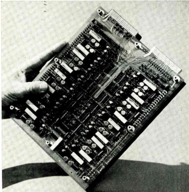
Memory sandwich. Two circuit cards hold the electronics, and the core stack plugs into both.
