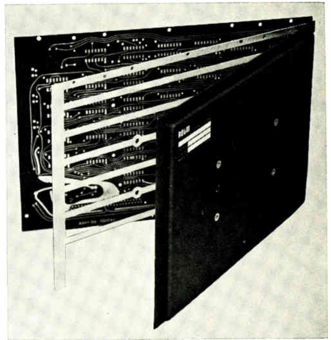
2. Tough cookie. Boards are protected with a "cookie sheet" cover fastened with four screws. Copper heat frame is applied separately to the pc board.
