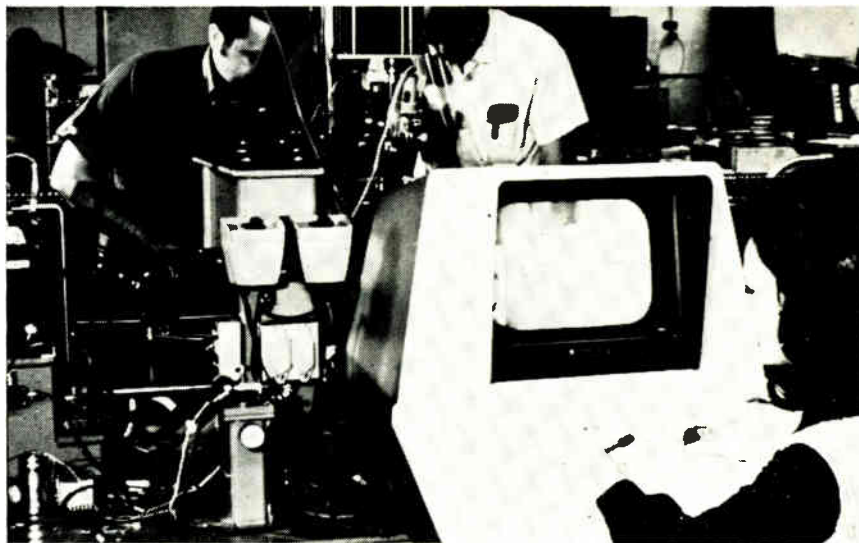
Series. Each substrate in Hugle Industries' automated bonding and testing system for hybrid circuits is checked for alignment, before chip bonding, with split-screen TV. Operator aligns marks on each end of substrate.
