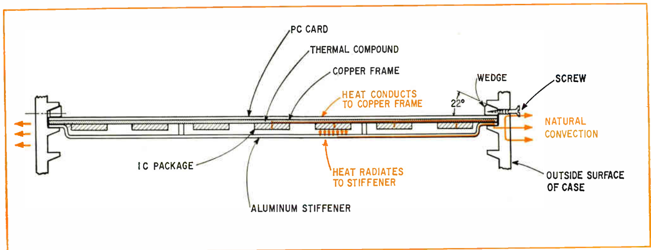
3. Hold tight. Board and cover, when inserted in case slot, are locked in place via a wedge that's pulled tight by a screw through the sidewall. Heat flows from the IC to the copper frame and then to sidewall. Wedge presses cover edge against copper heat frame. Cover also collects radiated heat from IC and conducts it to sidewall.
