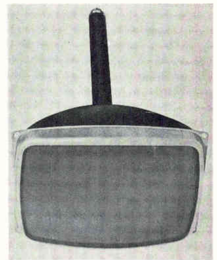
Multibeam scan. Seven beams in tube sweep phosphor dots as a unit.
