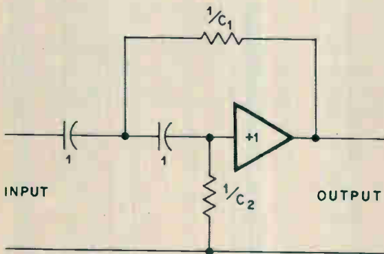
SECTION TYPE 1
