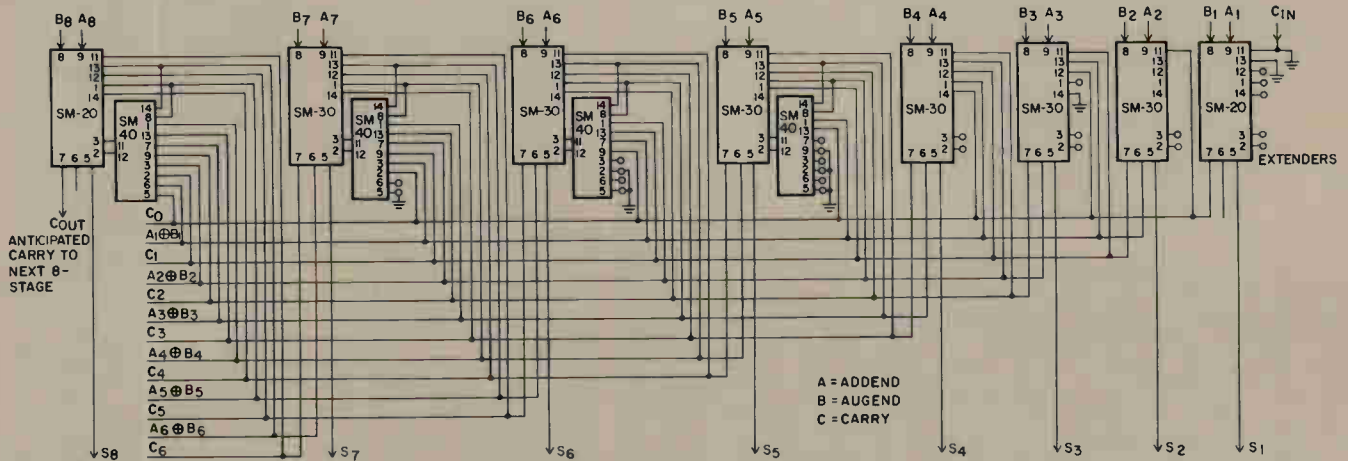
Fig. 1. Anticipated carry adder is up to 4.5 times faster than adder systems using ripple carry propagation.
