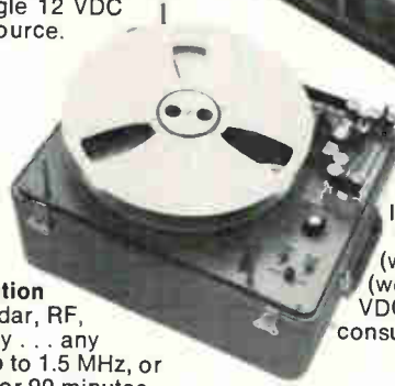
PI-6200 Portable Instrumentation Lab quality. Pushbutton operation. Low-cost ¼" tape. Up to 8 channels with three switchable FM or Direct record/reproduce speeds—0.375, 3.75, 37.5 ips—provide time contraction or expansion in 1:10:100 ratio. Optional loop adaptor and remote control. Operates on any power: 105 to 125 or 210 to 250 VAC; 48 to 400 Hz + and -12 VDC.
