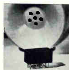
Solid state photocell relays can be furnished to switch up to 300 v a-c or d-c at low current levels directly with the photocell, or switch high current levels with built-in transistors. Off-on resistance ratios are obtainable from 100 to 1 to greater than 1,000,000 to 1. Control voltages may be selected from 6 to 120 v a-c or d-c. Electro-Tec Corp., Ormond Beach, Fla. [344]
