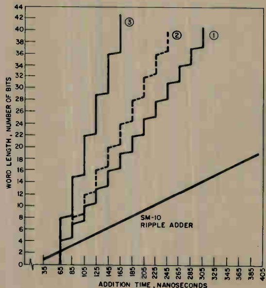
Fig. 6. Operating speed for (1) 3-bit stage added to 4-bit stage, (2) 4-bit stage with SM-40 expander added to 4-bit stage, and (3) 7-bit stage added to 7-bit stage.
