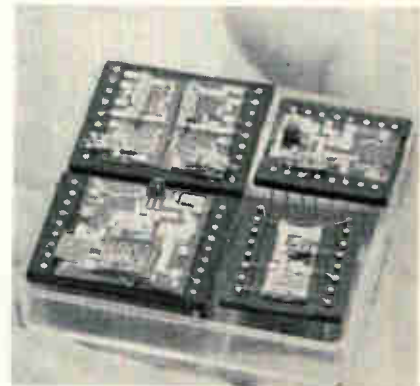
Handful. Hybrid circuit for tv tuner has yttrium-oxide capacitors.
