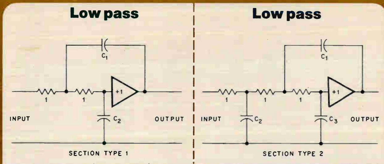
Four fundamental resistor-capacitor networks form the basis for active-filter synthesis.
