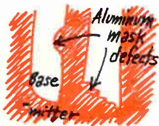
EMITTER-BASE SHORT IN HIGH-POWER TRANSISTOR
