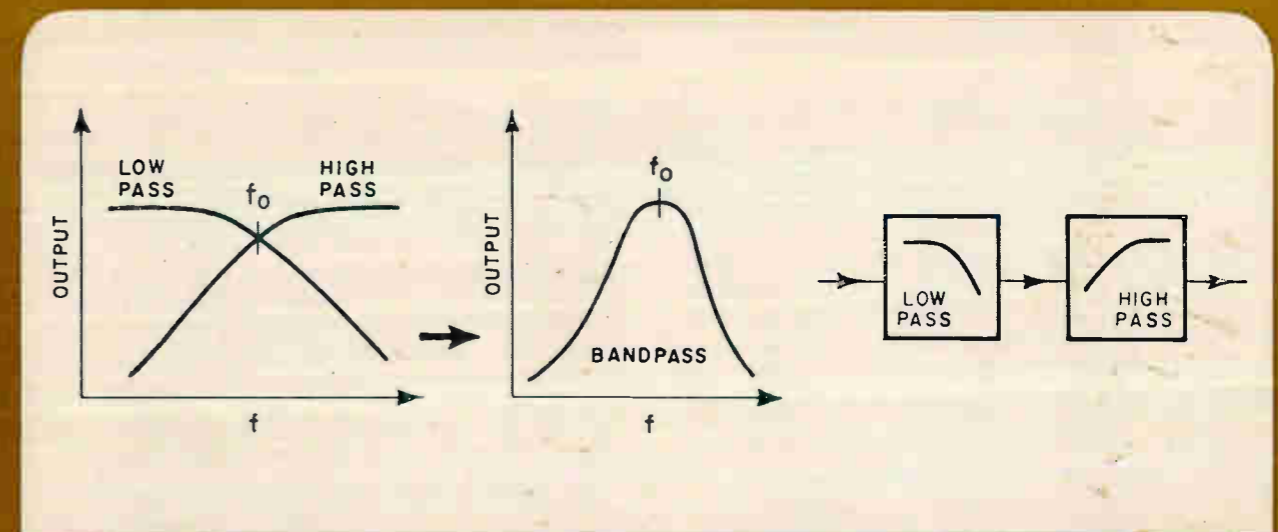
Two ways of combining low- and high-pass networks for different bandpass characteristics.
