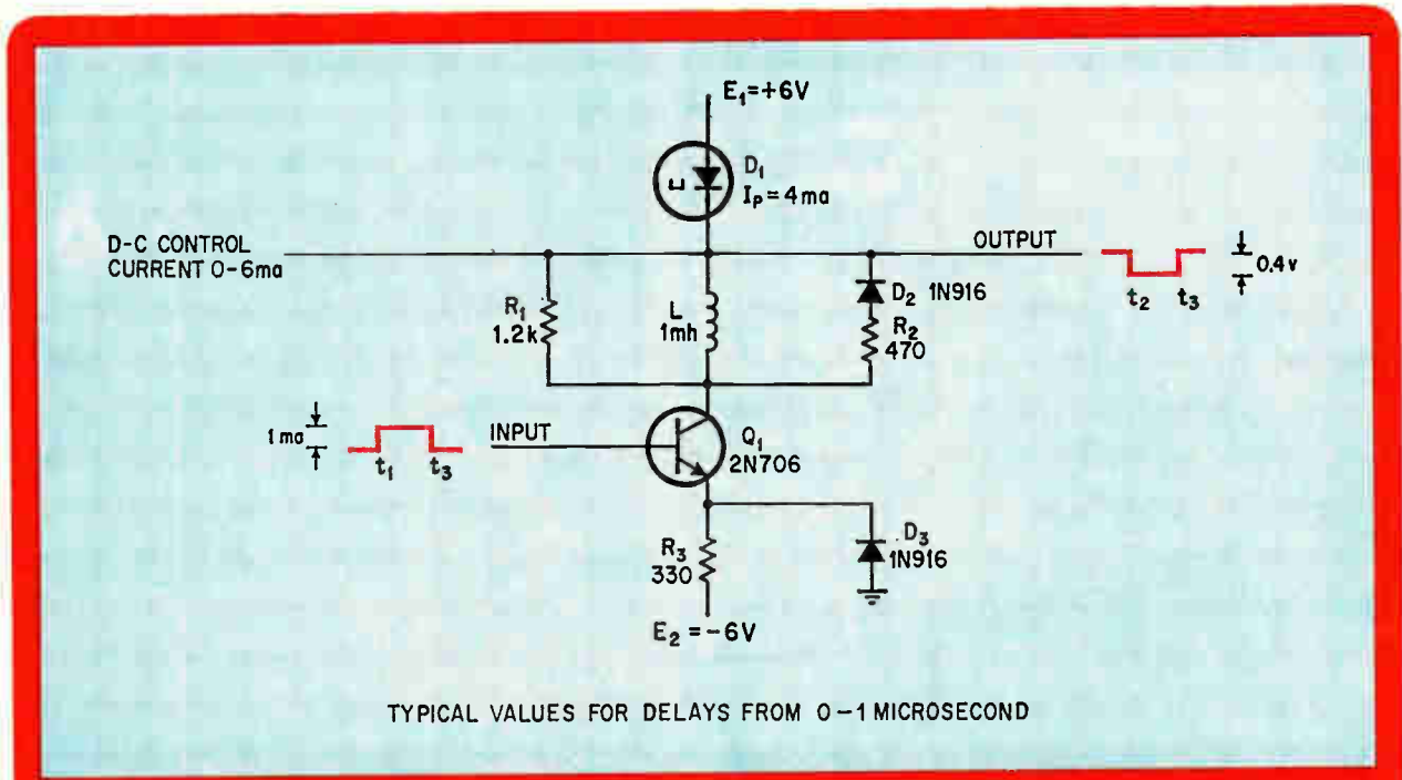
Smooth adjustment. The current in the inductor increases linearly until the tunnel diode's peak current is reached. At that point, the diode changes to its high voltage state. The delay between the leading edges of the input and output signals is proportional to the control current.
