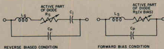
Fig. 1 Small-signal equivalent circuit of PIN diode.
