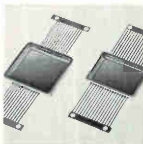
All-metal IC enclosure meets requirements of specification MIL-STD-883, including 3-hour helium bombardment at 90 psi. Designated the Butterfly case, it is intended for monolithic and hybrid IC's in high reliability applications. It is offered in 2 sizes: 0.750 x 1 in. and 1 x 1 in. Flat covers are available for each. Tekform Products Co., 2780 Colorado St., Anaheim, Calif. [346]
