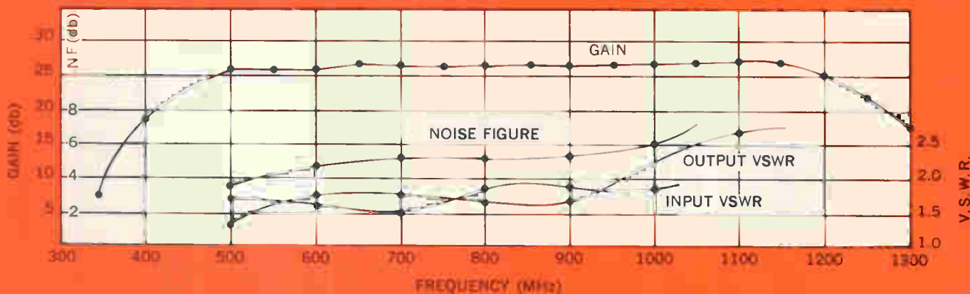
TYPICAL CHARACTERISTIC CURVES MODEL ESN 5001 LOW NOISE BROADBAND AMPLIFIER
