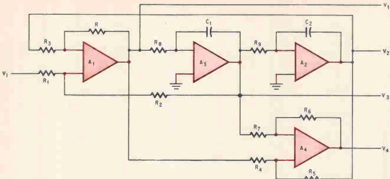
Miller integrator. One approach to achieving a desired transfer function is to use a basic Miller integrating network consisting of amplifier and RC network. Several such units are employed here to produce second-order transfer functions.
