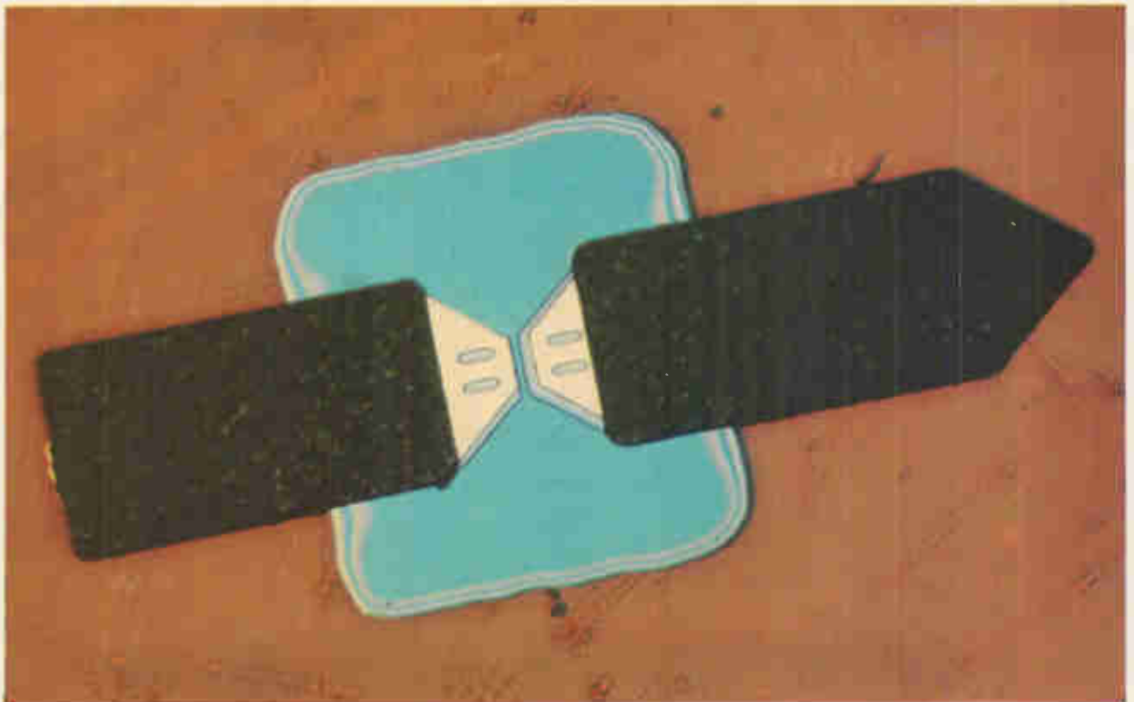
Isolationist. This surface-oriented pin diode, developed by Texas Instruments for use in the MERA program as a transmit-receive switch, has beam leads and provides better than 20-db isolation with an insertion loss of less than 0.5 db. Total capacitance is 0.1 pf and series resistance is 3 ohms.
