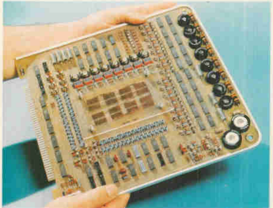
All together. Arrayed around mats of memory cores in center are the drive and decode electronics that make this assembly a complete memory.
