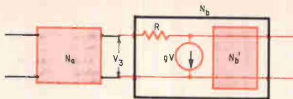
Horowitz' synthesis. This cascaded arrangement achieves its RL transfer function from the zeros developed in the N_a and N_b' networks.
