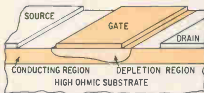
View. Cross-section of MES FET shows 1-micron gate. It's in the form of legs paralleling the sides of drain.
