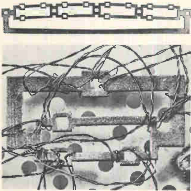
Magnetic logic. Four-stage logic structure (top) is building block of magnetic memory being developed for NASA. Lower photo shows how structure is wound.
