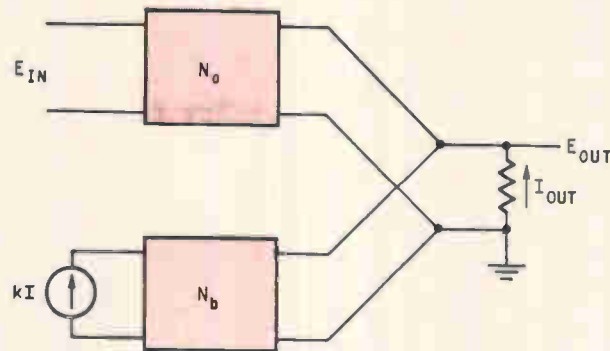
Kuh's method. An open-circuit voltage transfer function within a constant multiplier is made possible with a single control source and a few RC elements.
