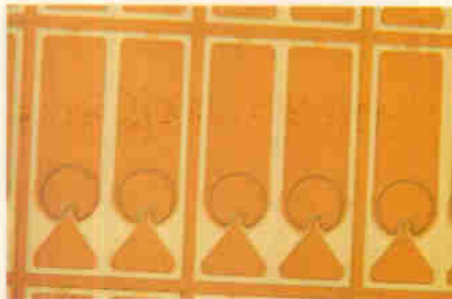
Broad beams. A group of Schottky-barrier beam-lead diodes from Sylvania's semiconductor division are lined up in the upper photo, while the lower shows a single diode placed in the center of the "tails" side of a penny. The devices are intended for use at about 13.3 gigahertz.
