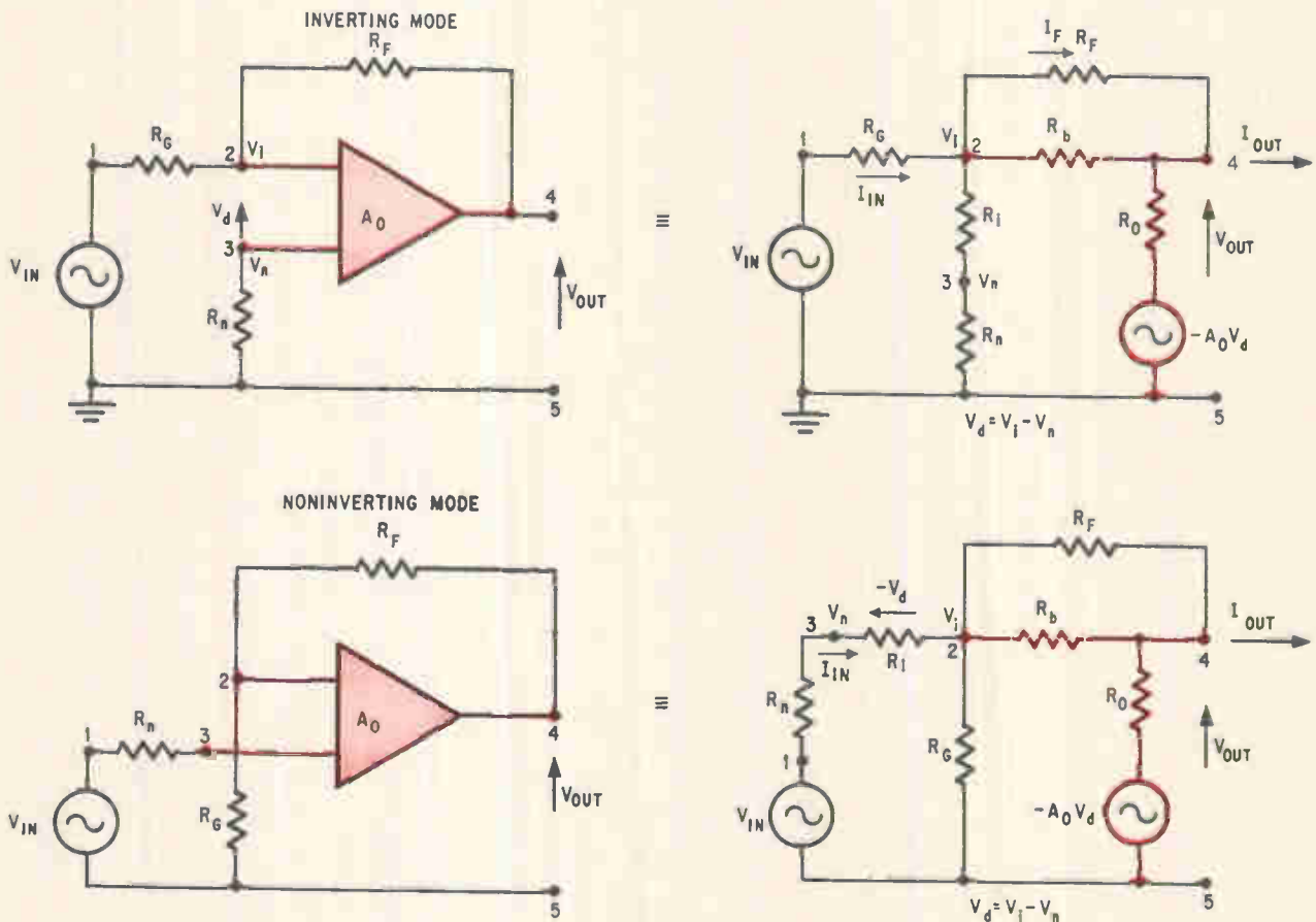
Operating modes. Terminal connections are indicated for both the inverting and noninverting modes of operation of an operational amplifier. At the right are the respective equivalent circuits for both modes.
