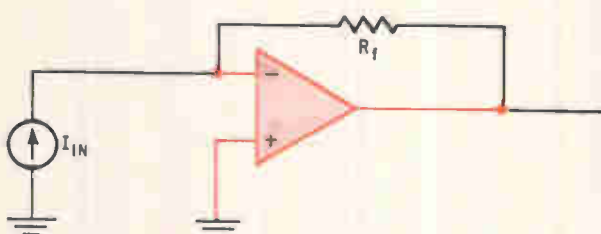
(c) CURRENT-CONTROLLED VOLTAGE SOURCE
