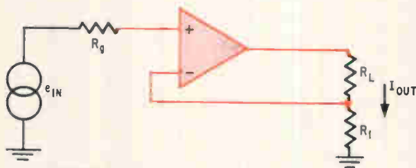
(b) VOLTAGE-CONTROLLED CURRENT SOURCE
