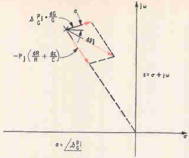
Pole displacement. The vector diagram represents the pole displacement for an active RC feedback network consisting of an active device G and resistors and capacitors. These passive components must track closely.
