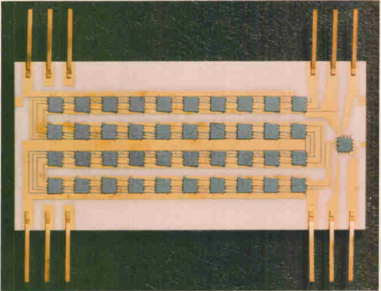
Big shift. Built by Bell Labs, this shift register has beam-leaded, insulated-gate FET stages with a single bipolar stage as a buffer. The substrate measures 0.625 by 1.3 inches.
