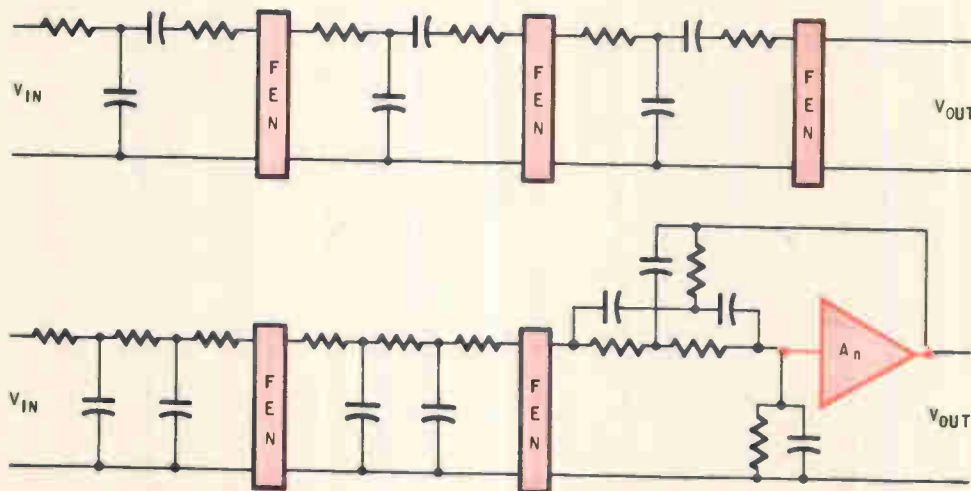
FEN filter synthesis. A sixth-order bandpass filter (top drawing) and a sixth-order elliptic lowpass filter (bottom drawing) are built with frequency emphasizing networks (FEN's). These units provide the RC networks with resonance properties similar to those of LC networks.
