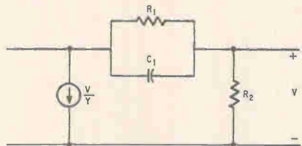
Zero section. A single transmission zero is produced in the right-half plane with this typical active-zero section.
