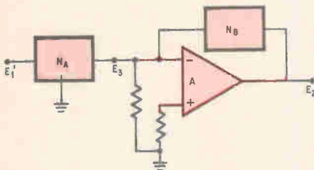
Simultaneous operation. A single operational amplifier is used to provide both the zeros and poles of a desired transfer function. It accomplishes this result through externally connected RC networks.
