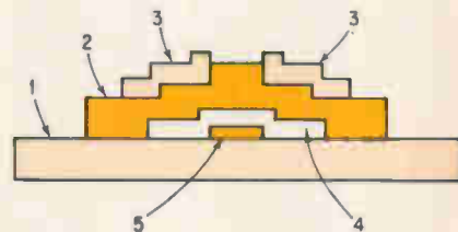
Parts. Thick-film FET's elements are substrate (1), semiconductor layer (2), source and drain (3), dielectric layer (4), and gate (5).
