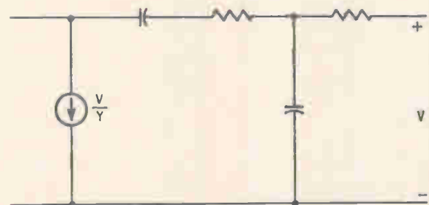
Pairing. Several groups of zero transmissions, including complex pairs, can be achieved with this active network. A controlled source is required for the transmission zero.
