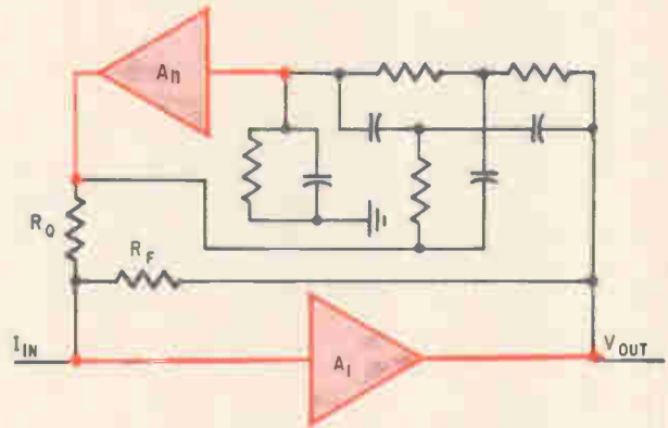
Frequency emphasizing networks. Circuit on top provides medium Q transfer functions; for high selectivity the bottom network is used.
