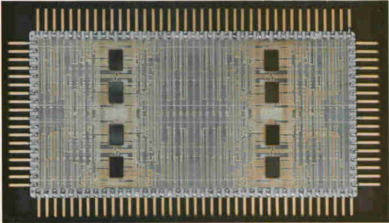
Leading somewhere. Experimental module built by Raytheon's Missile Systems division uses eight 40-gate TTL modules with beam leads. The top layer of the metalization pattern on the substrate sets up the circuit configuration.
