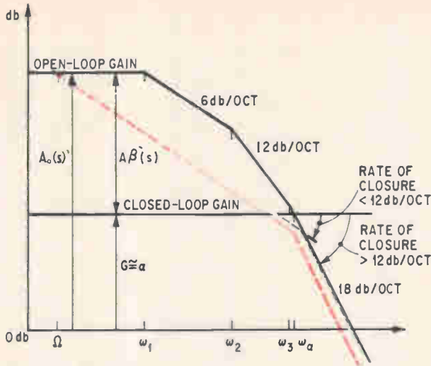
Graphing the gains. Bode plots for the open-loop and closed-loop gains of a typical operational amplifier. Dashed line represents the gain response of a modified op amp whose stability is assured by added RC components.
