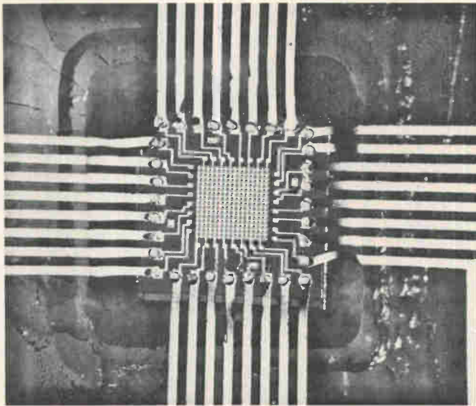
Over the edge. In this read-only memory from MIT's Lincoln Lab, the beam leads are formed on the substrate overhanging the cavity into which the chip is inserted.
