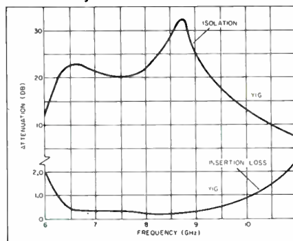
BANDWIDTH CURVE
