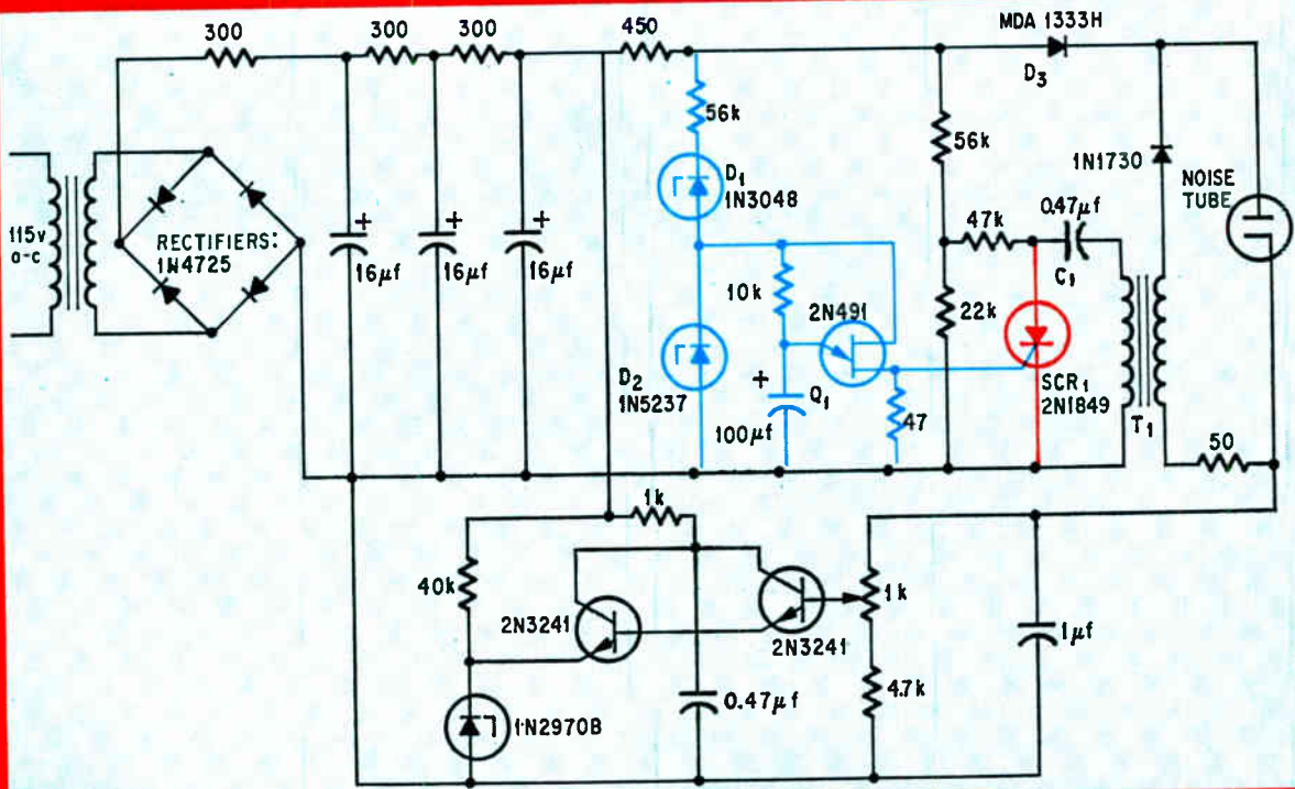
Double duty. The unijunction's triggering of SCR, causes a high voltage to develop in the secondary of T_1 . This high voltage fires the gas tube. The filtered d-c voltage at the anode of D_3 keeps the tube in conduction.
