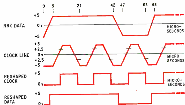
Reshaped signals. Data pulses are shifted relative to the clock pulses to keep the data stable during clocking. Clock triggers at \pm 2.5 volts, data at zero-crossing points.
