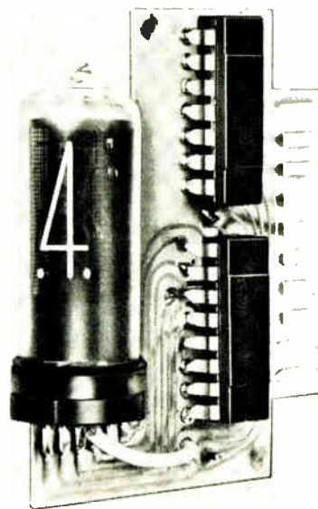
Package deal. A Nixie tube with drive circuitry from Burroughs goes for about $20. The tube alone is listed at $3.95.
