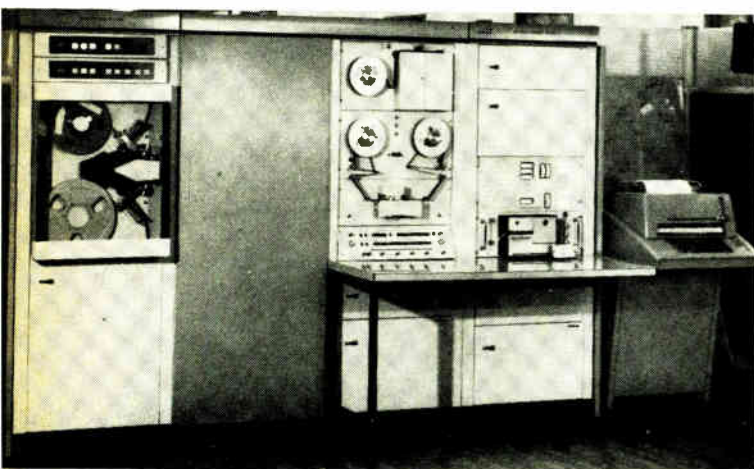
Automatic tester. Test programs are on tape; SDS 910 computer runs 500 tests in three seconds and prints results on strip of paper sent with module for rework.
