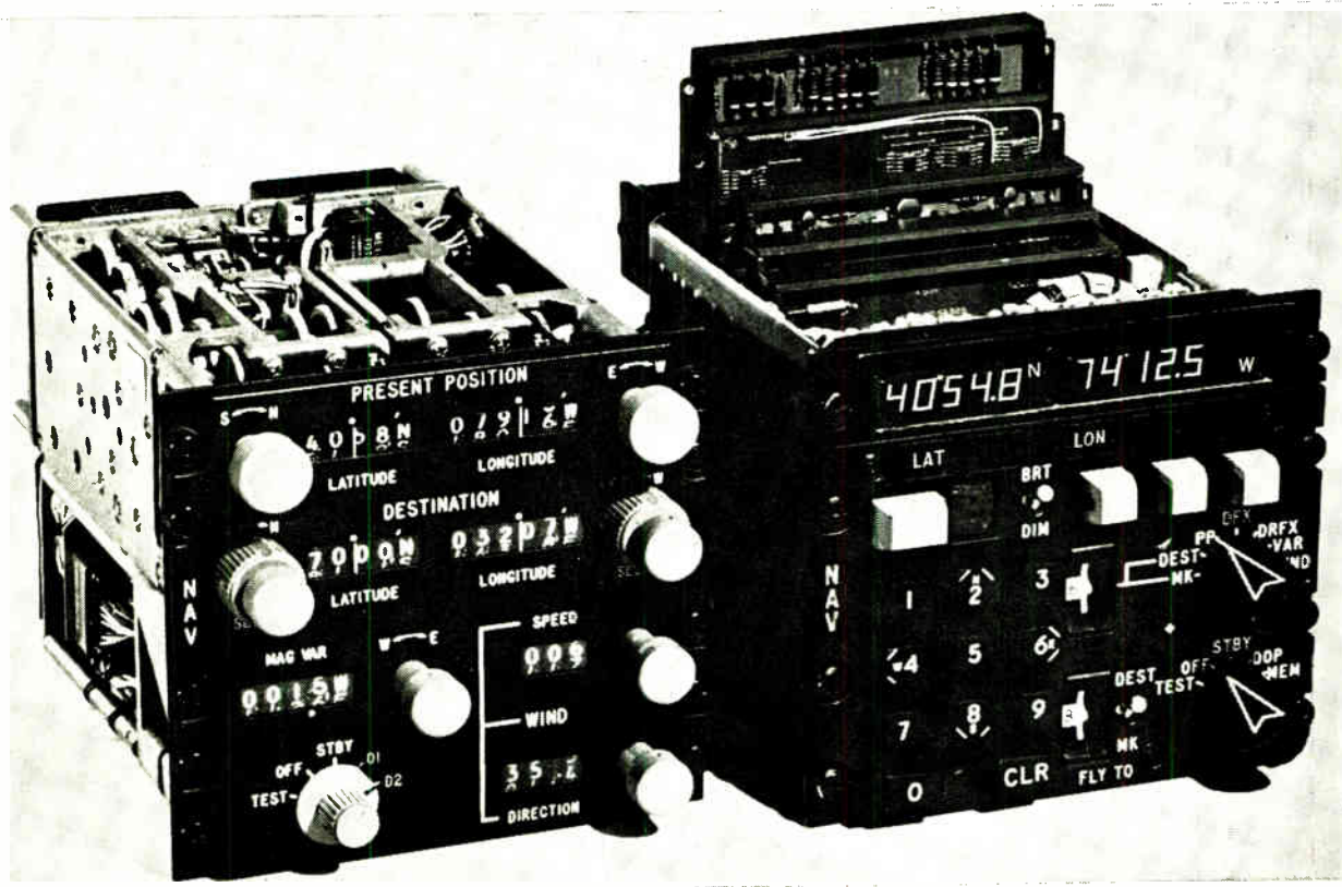
One for one. Control-display unit, right, is designed with digital techniques for doppler navigation system; it has a telephone-type keyboard and numerical readouts. It can be plugged into the place of the older analog unit.
