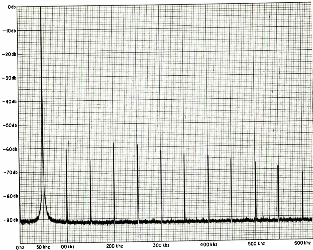
Wide range. New wave analyzers can provide recordings with 90 decibels dynamic range. This plot is of an oscillator output with the analyzer set at 1-kHz window, sweeping at 1 kHz per second
