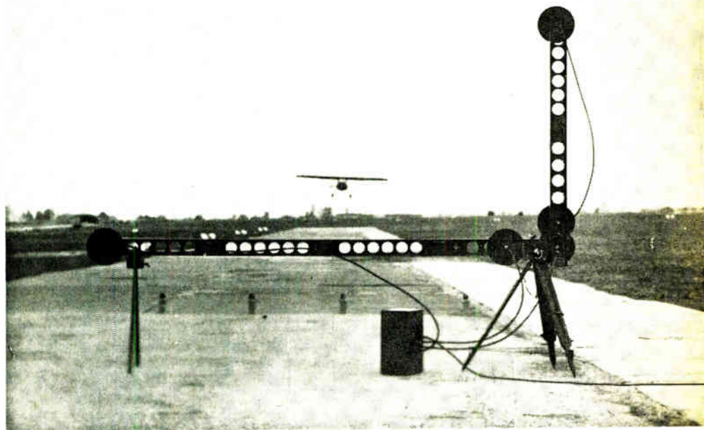
Handy guide. Setac landing equipment sets up in a trice at any airstrip. Three antennas on horizontal beam handle azimuth pattern. Elevation angle pattern comes from antenna pair on vertical beam.
