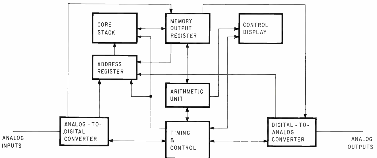
Analog in and out. Converters on input and output of the Micro-Minac digital computer make it compatible with the analog system already aboard the aircraft.
