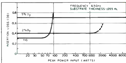
POWER CURVE
