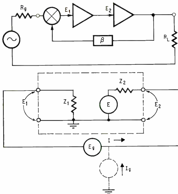
Loop gain. The wave analyzer can be used to measure an amplifier's loop gain by inserting a voltage with a current probe in the feedback loop, as shown in the equivalent circuit. The current source, shown dashed, can be used in an alternate scheme for different impedance levels.
