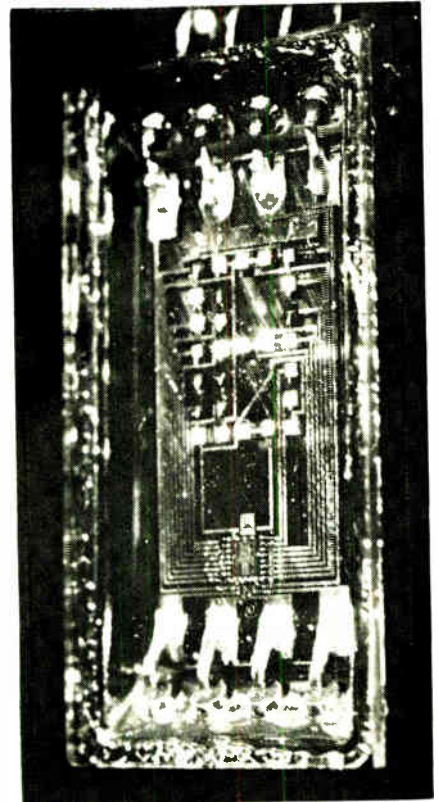
Five spot. The number five appears in the 5x7 diode matrix of this prototype solid-state display from Hewlett-Packard. Logic and display elements are incorporated in a single package only 0.162-inch thick.
