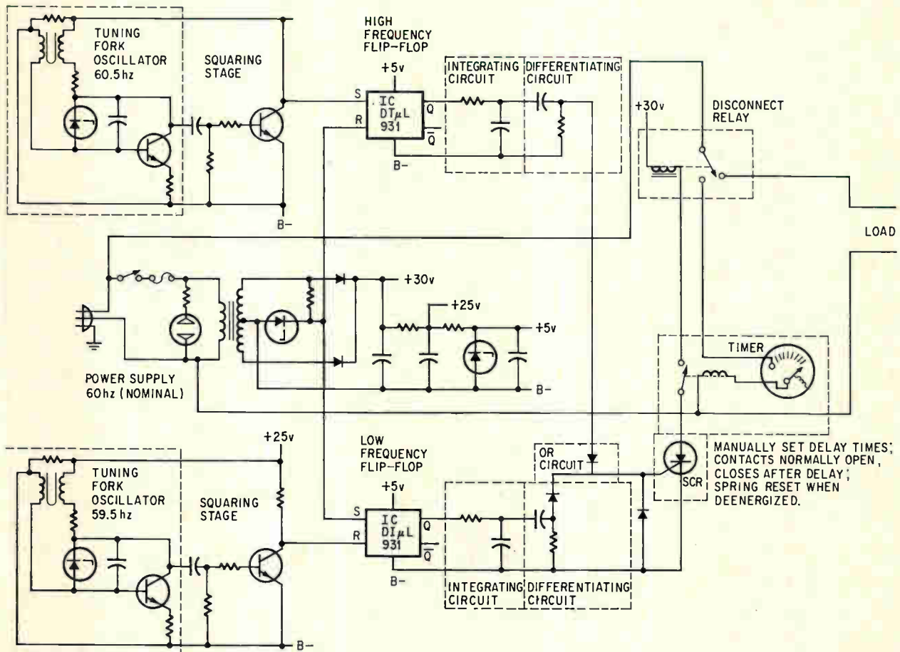
Phase into pulse. In each monitoring channel, a tuning-fork oscillator generates a reference frequency for comparison with the line frequency. An excessive difference between the two is converted—in flip-flop, integrating, and differentiating circuits—into a pulse that triggers the SCR.
