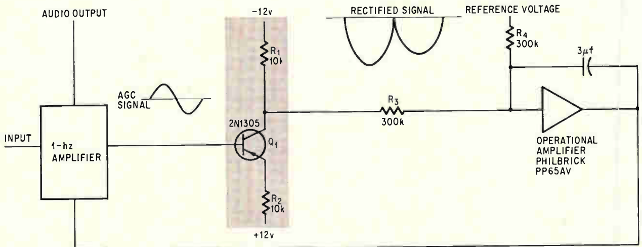
Rectifying transistor. A d-c voltage, proportional to the agc signal level, is supplied to the input of the operational amplifier by Q_1 . The transistor, inverts the positive portion of the agc signal. Because it saturates the transistor, the negative portion of the signal can be transferred directly to the collector and results in full-wave rectification.
