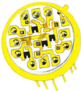
Uncased Chips – Thermal Bond Construction – Hermetic T08 Pack
