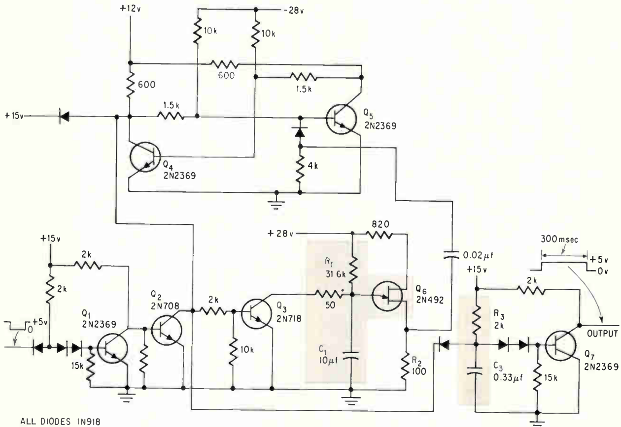
Unijunction control. The multivibrator when triggered by the unijunction transistor turns off Q_7 and places the 5-volt collector supply on the output. When C_1 discharges through R_1 , the unijunction transistor removes the trigger and the multivibrator turns off. After C_3 charges through R_3 , Q_7 turns off and the output is placed at ground.
