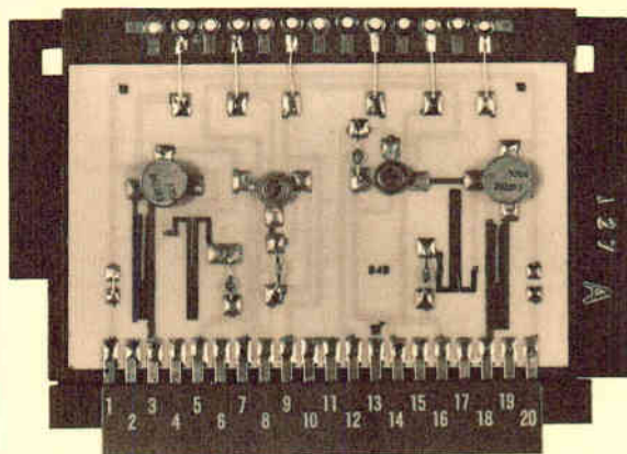
Thick-film/ceramic logic card. Here discrete components are mounted with thick-film/micro-electronic substrate components. Connectors are again the same as for the standard IC package.
