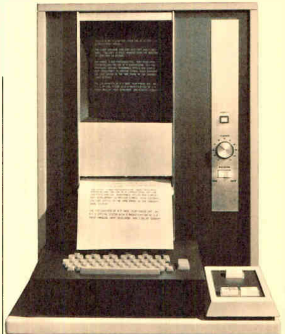
3M "129" Display CRT Print Module. Information retrieved from computer memory bank is displayed on screen at top. Press "print" button and information on screen will be reproduced on dry paper, below, within 10 seconds.
