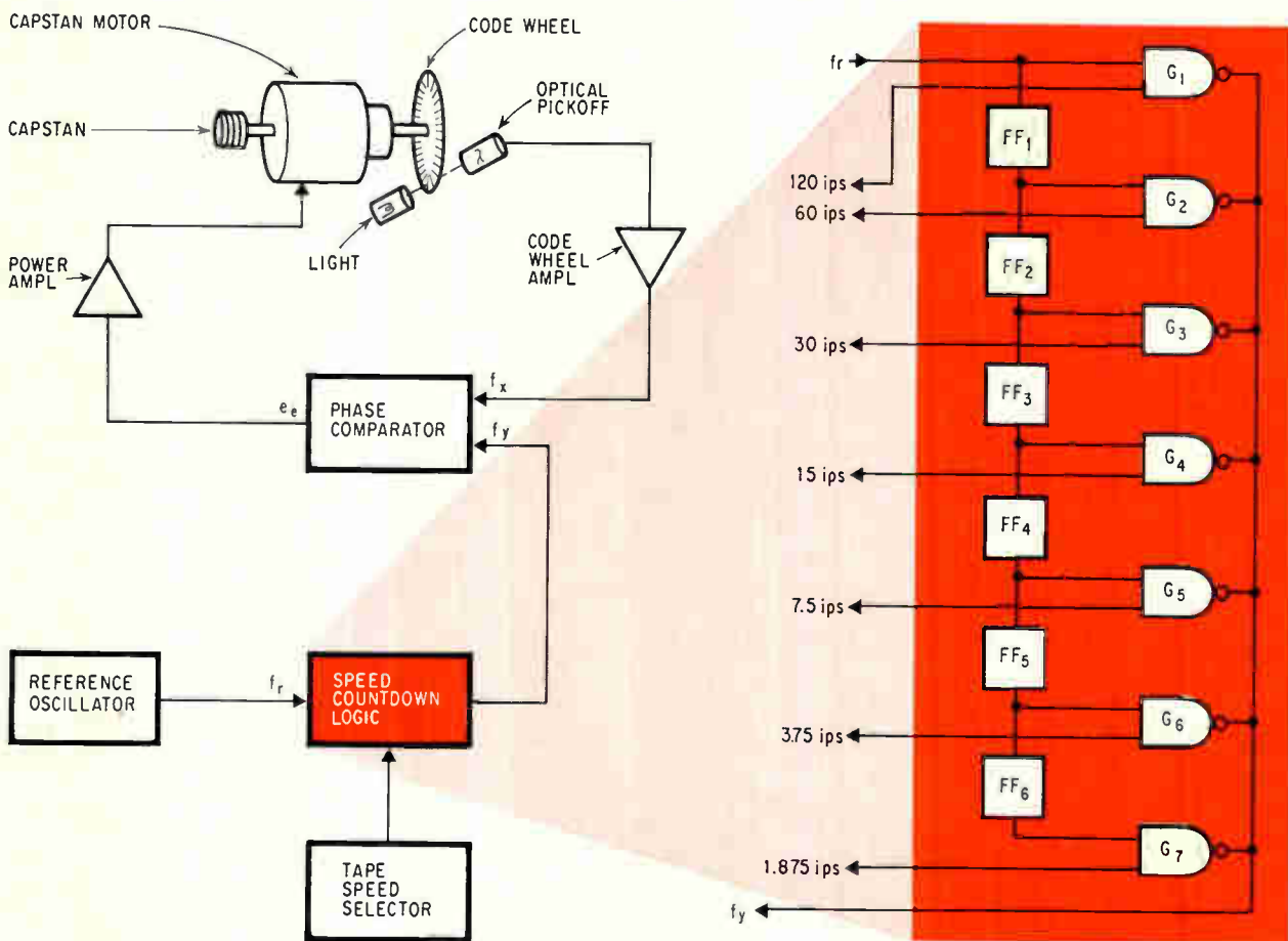
Digital speed control. Capstan speed is controlled by phase-locked servo loop. Optical pickoff signal's frequency and phase is compared to signal from reference oscillator. Output of comparator either increases or decreases signal to power amplifier to bring capstan to desired speed. Logic diagram of speed countdown circuit shows how reference frequency is controlled digitally.
