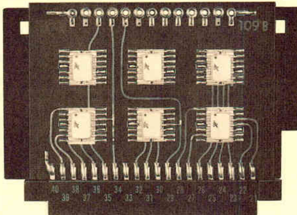
Integrated-circuit logic card. Double-sided board contains up to 12 IC flatpacks or dual in-line plug-in packs. Standard board has a 40-pin double-row male connector mounted at lower edge.
