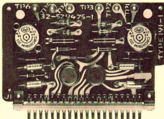
Discrete-component circuit logic card. This package uses the same male connector and configuration as the IC package; both types may be freely intermixed at chassis level.
