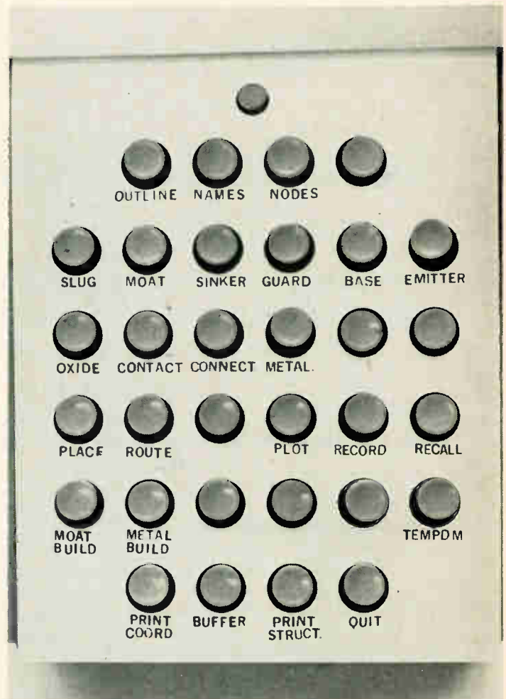
Function keyboard. Each of the 32 keys triggers a discrete function. Pressing the plot key, for example, causes a Calcomp plotter to draw the output.
