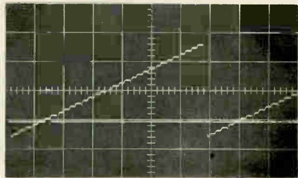
Speed of the Paramatrix. In the two upper oscilloscope traces, the staircase waveforms are of the X-coordinate output from the transformer, viewed over one complete picture scan of about 2 milliseconds. The lower traces in the upper photographs show one of the interpolator outputs, with a fine sensitivity setting in the photo at left and coarse sensitivity at right. The two lower photographs are of the Y-coordinate output on an expanded time scale; the entire staircase takes as much time as one step in the upper photos. The lower traces in the lower photographs show the interpolator output again (left) and the output of the coincidence unit. Note the pulse at left.
