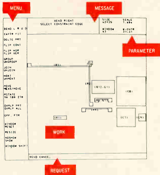
Screen areas. Five basic sections of the screen used by the designer to develop an IC layout.
