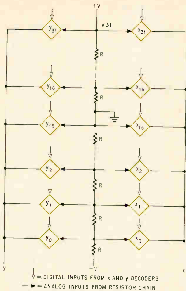
Digital-to-analog converter. Diamond gates (color) convert each of the x and y input coordinates from the digital decoder into an analog voltage.
