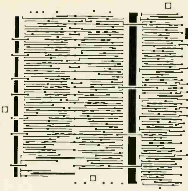
Generated artwork. Interconnection pattern for 122-element logic chip is generated 10 times oversize. Typical line width is 0.4 mil.
