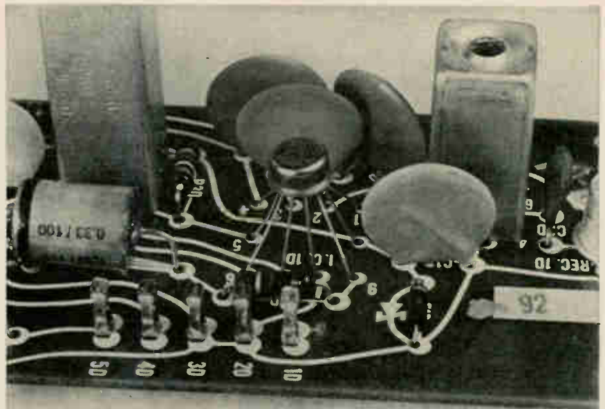
Replacement part. Audio IC in Motorola color-tv set replaced 15 discrete components; chip incorporates 15 resistors, 12 transistors, and 12 diodes.
