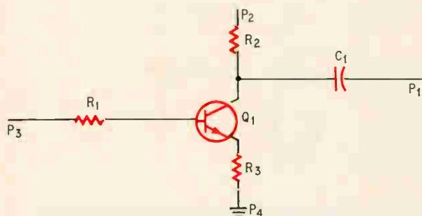
Force analogy. Contact points P_1 , P_2 , P_3 , and P_4 in this single-transistor circuit are fixed to components C_1 , R_1 , R_2 , and R_3 , shown in color, whose leads are assumed to be elastic. If the components are allowed to assume a position in which the net forces acting on each component are zero, the elements come to rest. The relative position of the components at this time becomes a possible board layout.
