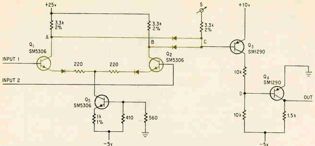
Comparator circuit. A binary 1 output appears when the two inputs are equal within a sensitivity margin determined by the setting at S. The circuit portion in color does the actual comparing. Point C follows the lower of the two collector voltages A and B, depending on which transistor is conducting more heavily.
