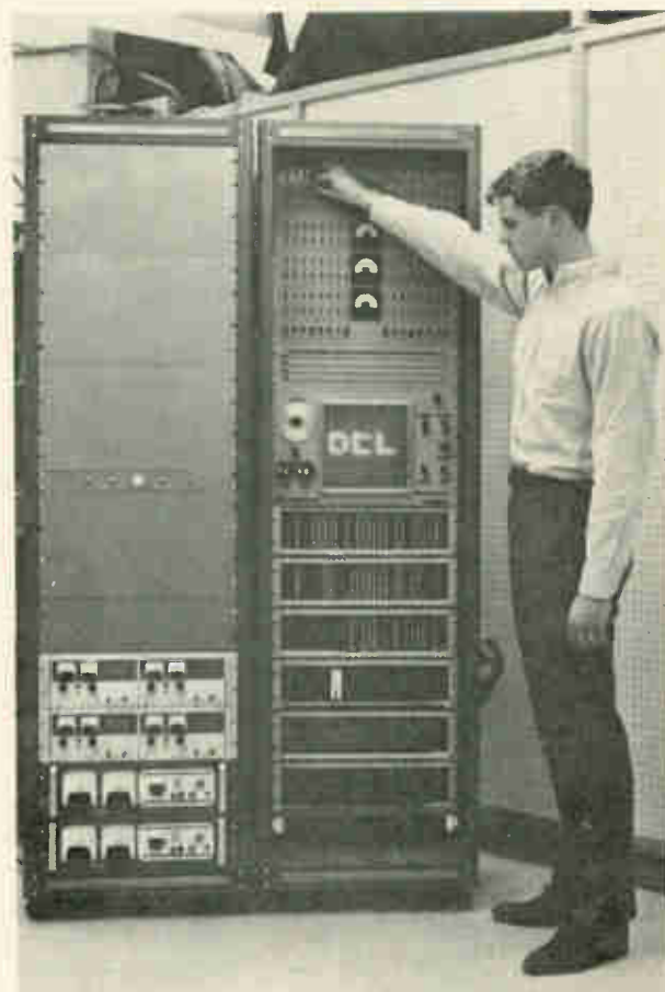
Prototype Paramatrix. Unit fits in half a rack, because it uses only about 50 printed circuit cards for its major functions, and another 68 cards for the display matrix flip-flops and drivers. The other half of the rack contains the input simulator. The second rack here contains power supplies shared by the Paramatrix with other projects in the laboratory.
