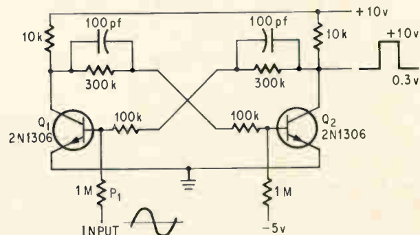
Adjustable hysteresis. Input signals, which exceed the threshold level set by potentiometer P_1 , turn Q_1 on and Q_2 off, generating an output step.
