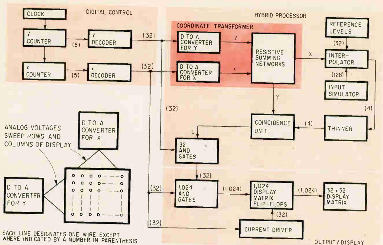
Three major parts. The Paramatrix sections are lightly tinted. The heavier tint indicates the coordinate transformer, which generates the input coordinates in response to an output scan by the digital control section.
