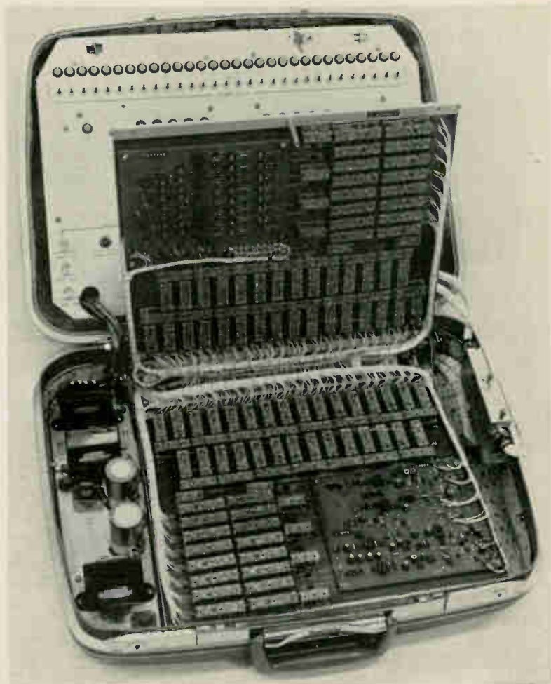
Suited for space. Bunker-Ramo's experimental memory, which fits into a 21-suitcase, operates on very low power.
