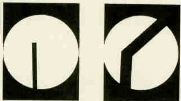
Sharp lines. Blown-up drawing of two typical line widths. Vertical line at left is generated by the y motion of the table. Diagonal line is achieved with successive x and y motions because the table can only move along one axis at a time.
