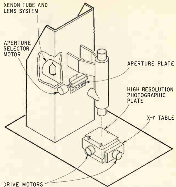
Light Table. Sensitized plate is exposed to light as the table moves in either x or y direction.
