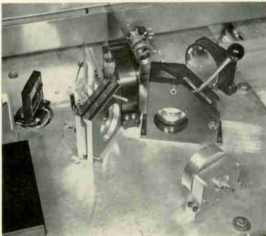
Crystal set. Diagram shows how light travels among prototype components set up in photo at left to record analog data such as photos or drawings. After exposure, a joy stick is used to lift the beam splitter out of optical path, and the crystal can be viewed from the rear. In this early model, the stepping motor for the KBr crystal holder is below the table.
