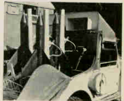
Tank buster. The "Shmell" antitank missile has 2,500-yard range.
