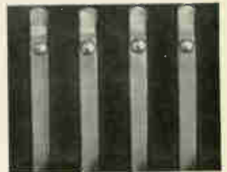
Cut-away Amphenol PMT connector shows welded gold dots on contacts
