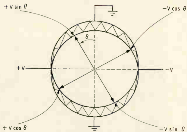
Rotation. A sine-cosine potentiometer connected to the power terminals of a network of diamond gates (color) enables the gates to generate analog signals that match the rotation angle of the potentiometer.
