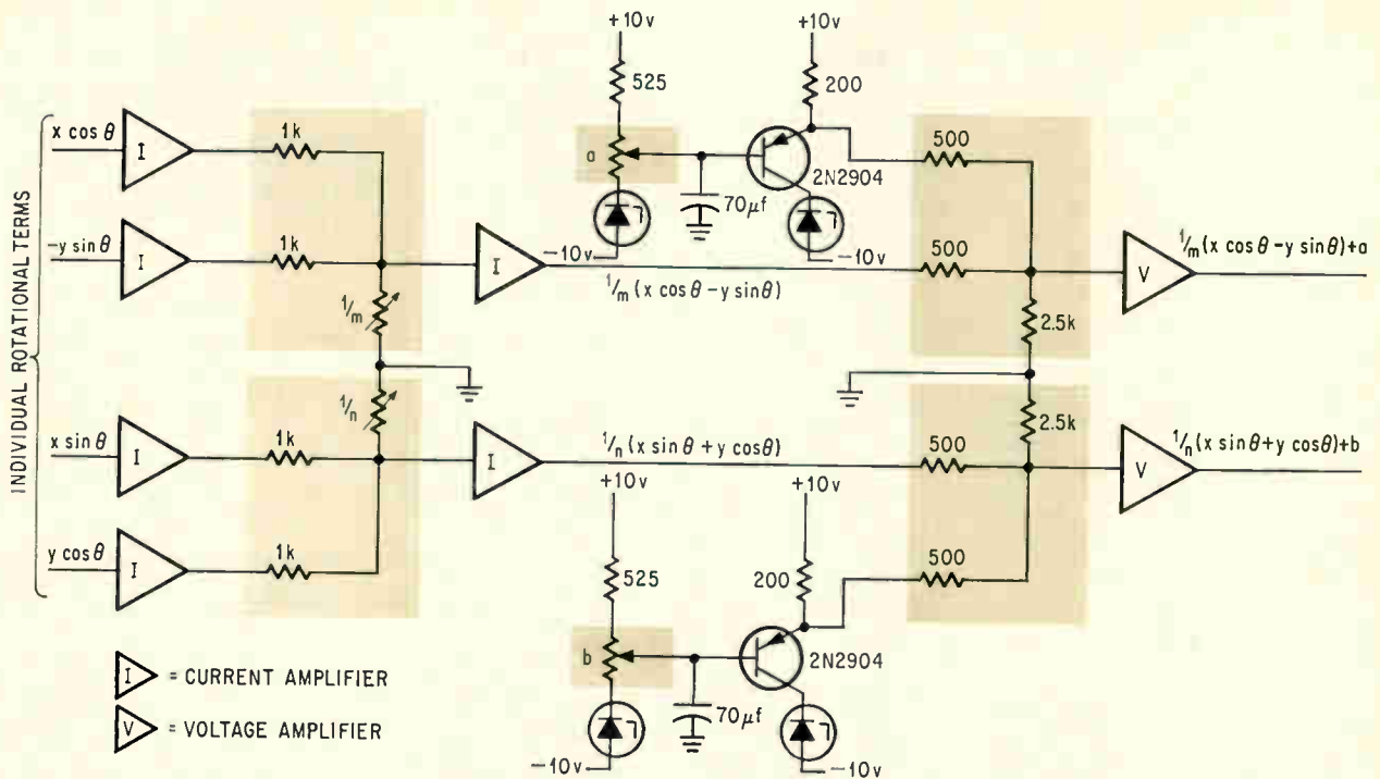
Adder. Resistive summing network (tinted at left) adds up the rotational terms and supplies the factors for magnifying or demagnifying the picture. Current amplifiers isolate the network from the preceding diamond-gate terminals. Translation terms are added by the second-stage summing network at right. Voltage amplifiers at the output boost the signal to sufficient strength for the interpolator and coincidence unit, and the potentiometer circuit provides the translation terms to the second-stage summing network.
