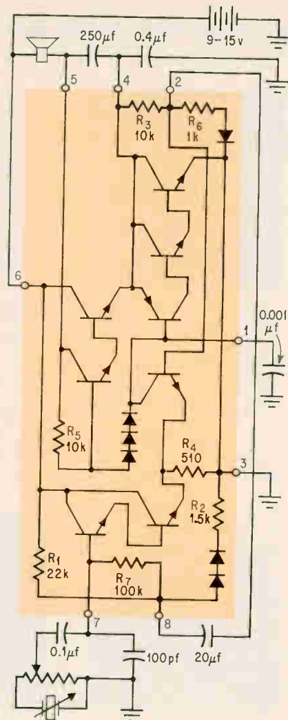
Push-pull. Output stage delivers more than a watt to speaker.
