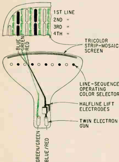
Double-barreled. Jatron color-tv tube has only two guns instead of the usual three, and strips instead of phosphor dots.
