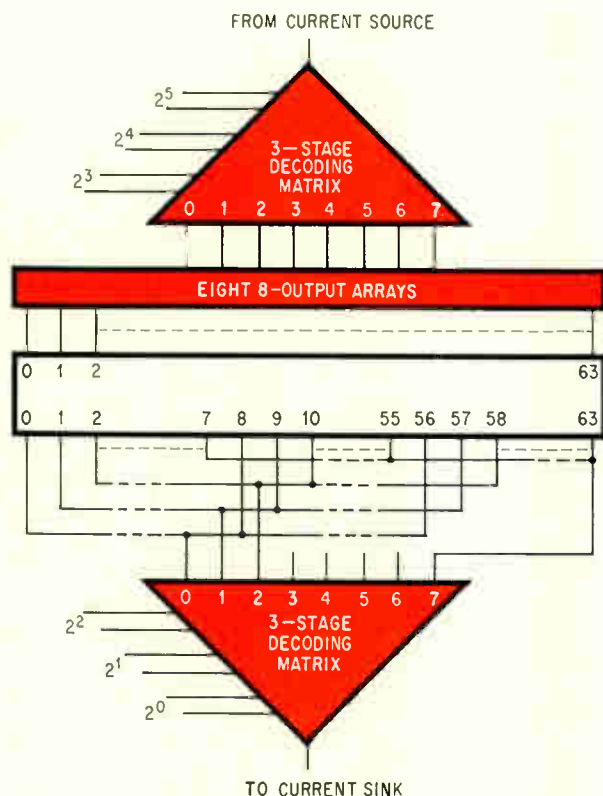
Double-ended decoder. Two 3-stage matrices and eight 8-output arrays can provide complete memory address decoding and driving cheaply. All the stages shown in color would be glass-switch arrays.
