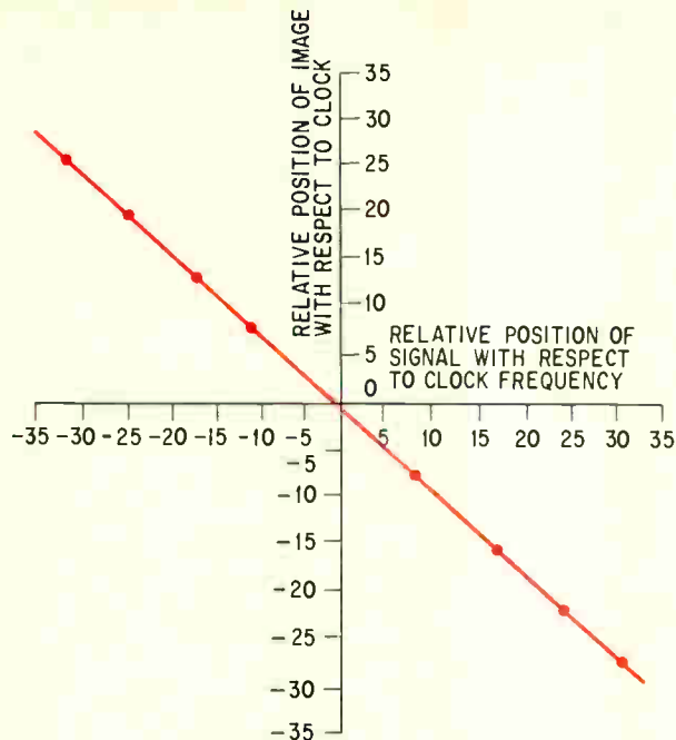
Image response. Relative location of the image frequency is plotted with respect to the clock frequency to enable the designer to locate a third-order image response.
