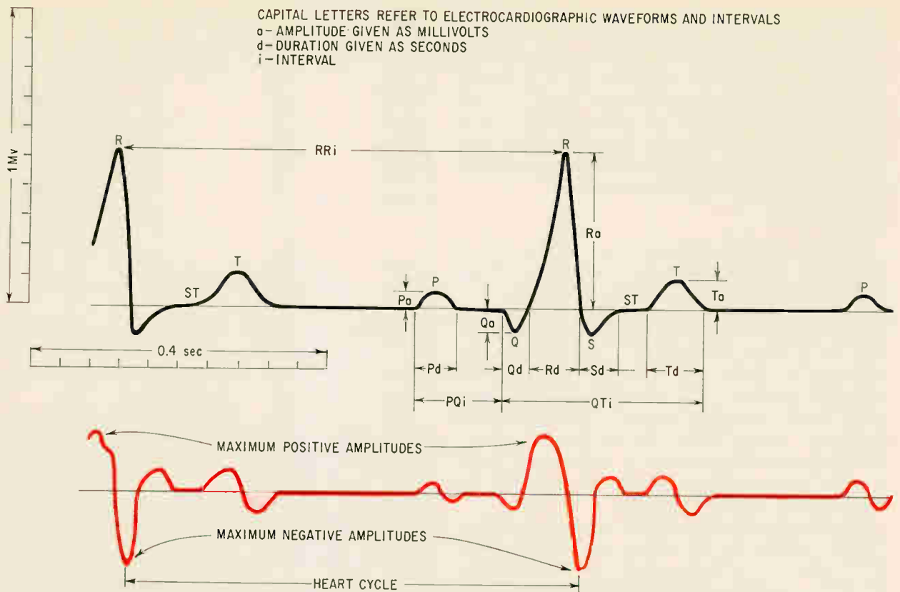
Starting line. Reference for the start of the heart cycle is the first derivative (lower curve) of the EKG waveform. The maximum negative value is the starting point. Once this is established for the computer's program logic, the machine can identify the significant components in the cycle (upper curve).
