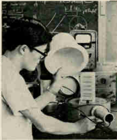
On the block. Yagi antenna for doppler-radar traffic sensor is made of foil strips cemented to polystyrene foam block. The "hat" is antenna's radome.
