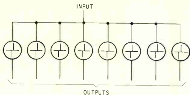
Multiple array. Proposed eight-output threshold switch array could be batch-fabricated on a single monolithic chip.
