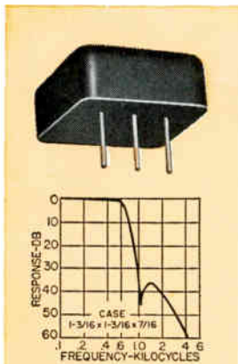
560 ~ Telemetering low pass filter. Available from 400 ~ to 70 KC. \pm 7.5% bandwidth flat to 1 db. Attenuation greater than 35 db beyond the 2nd harmonic of \pm 7.5% frequency. Impedance 47K ohms. MIL-F-18327B. Wt. 0.8 oz.
