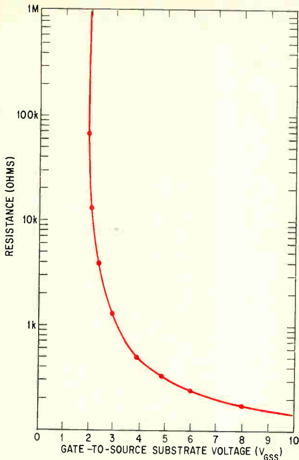
Switching capabilities. Plot of gate-to-source substrate voltage versus resistance for an MOS field effect transistor indicates a value of 200 ohms when V_{GSS} equals 5 volts. Resistance increases infinitely at V_{GSS} of 2 volts.
