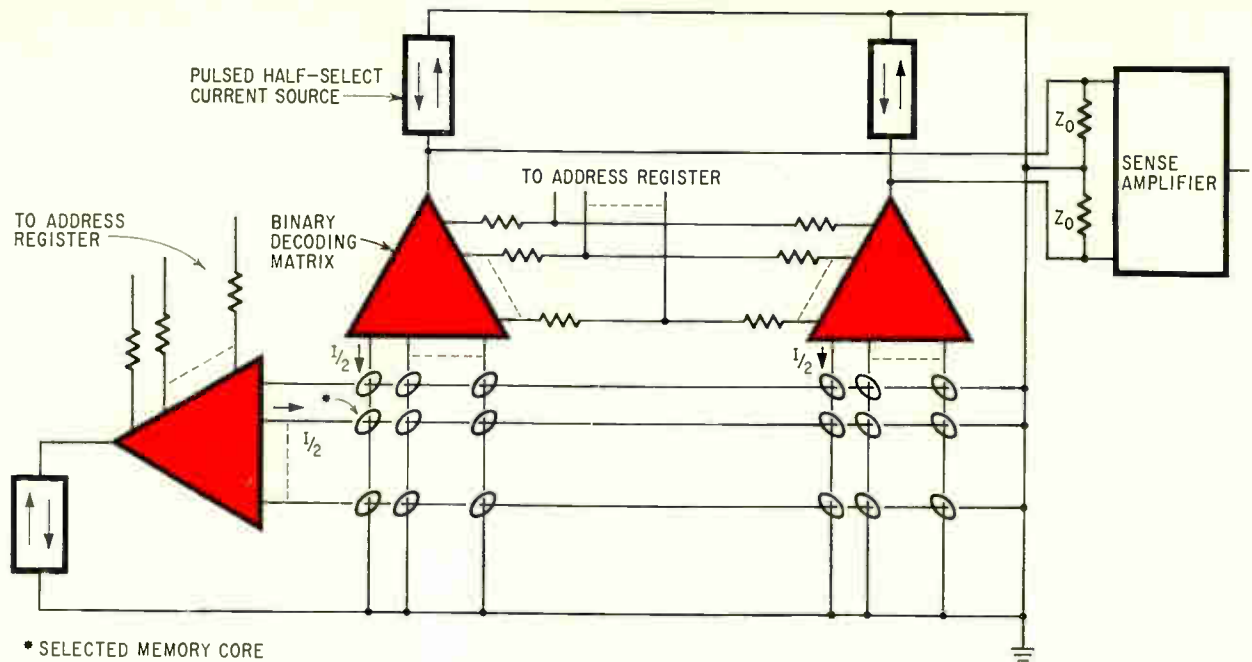
Looped select lines. Three decoding matrixes (color) in a 2\frac{1}{2} -dimensional memory provide all addressing capability plus simple connections.
