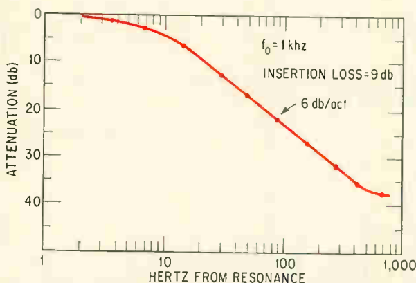
Frequency-response. Shunt- and series-switched digital filters with a single-section RC low-pass filter have identical frequency-response curves. Both types yield a response similar to that of an LC-tuned network.
