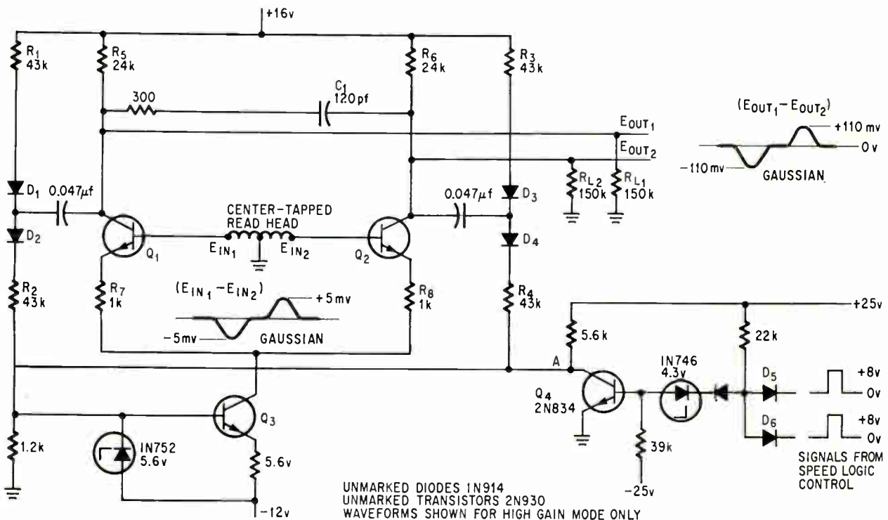
Digital gain control. Positive signals at D 5 and D 6 turn on Q 4 , and forward bias diodes D 1 , D 2 , D 3 , and D 4 so that resistors R 1 , R 2 , R 3 , and R 4 load the amplifier and reduce its gain.
