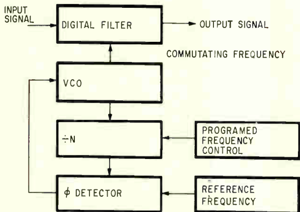
Frequency hopping. Stages for a digitally controlled system indicate the operation sequence. By regulating the voltage-controlled oscillator from the phase detector, the commutating frequency changes, thereby retuning the digital filter.
