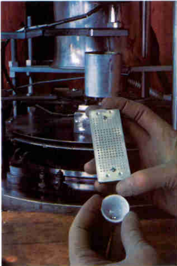
Carbon electrodes. Tiny carbon balls held in the fixture in front of a vacuum deposition chamber will become threshold switches when coated with glass film.
