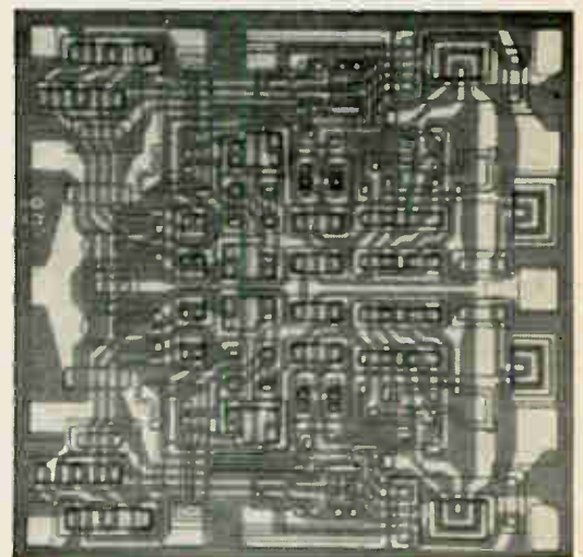
Compatible. DTL flip-flop fits TTL pins.
