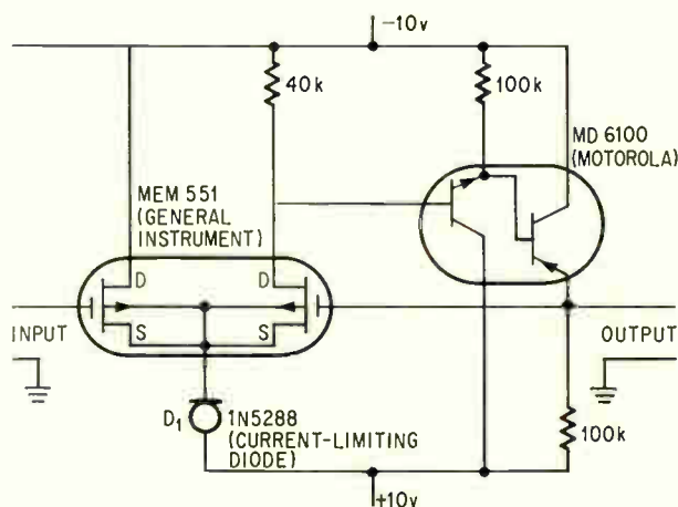
Improvement. Modified MOS FET buffer achieves excellent thermal stability with complementary output transistors.
