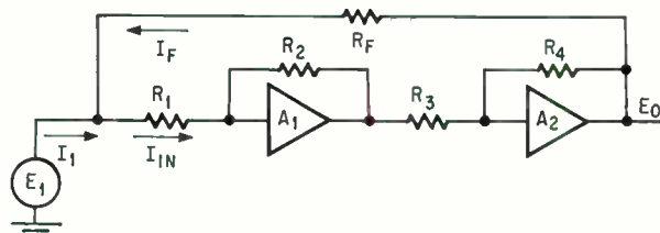
Equivalent circuit. Operational amplifier for negative impedance converter replaces transistors Q_1 and Q_2 in the original schematic with amplifiers A_1 and A_2 .
