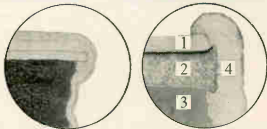
(a) Typical section of an electroplated hole, showing heavy build-up of metal plating at the orifice.
