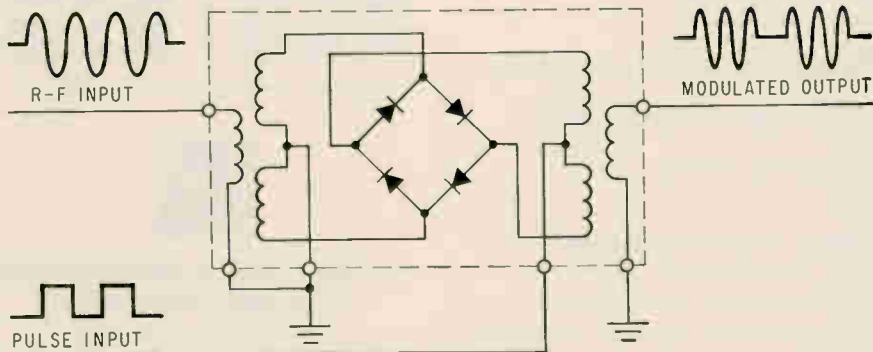
Power saver. Bridge of hot carrier diodes needs no power supply.
