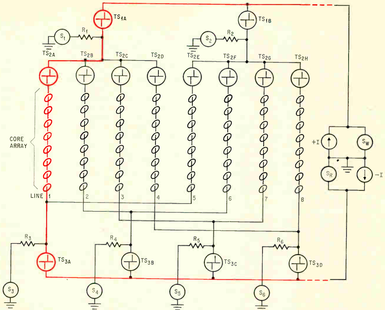
Dual-polarity drivers. Partial internal decoding is possible when threshold switches are applied as dual-polarity drivers. External decoding is still required for switches at bottom. One complete loop for a half-select current is shown in color.
