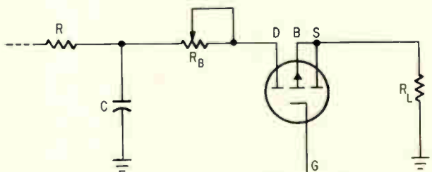
Reducing noise. For the FET, a balance network incorporating a potentiometer reduces the zero-signal voltage to below 50 microvolts.
