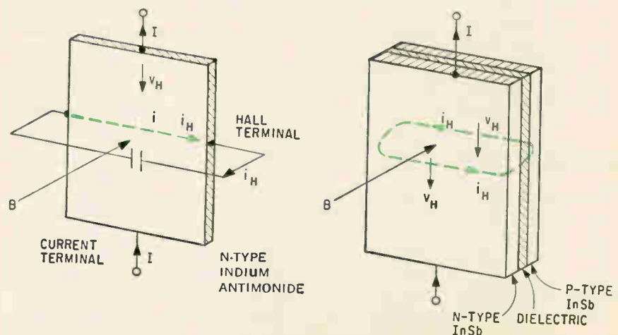
Inductive slab. Basic solid-state inductor (left) consists of InSb slab with external capacitor connected to two of its four terminals. Dielectric sandwiched between two slabs gives device internal capacitor.
