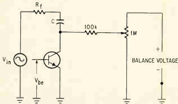
Balance network. To reduce zero-signal voltage of a shunt-switched filter, a nulling arrangement is applied.
