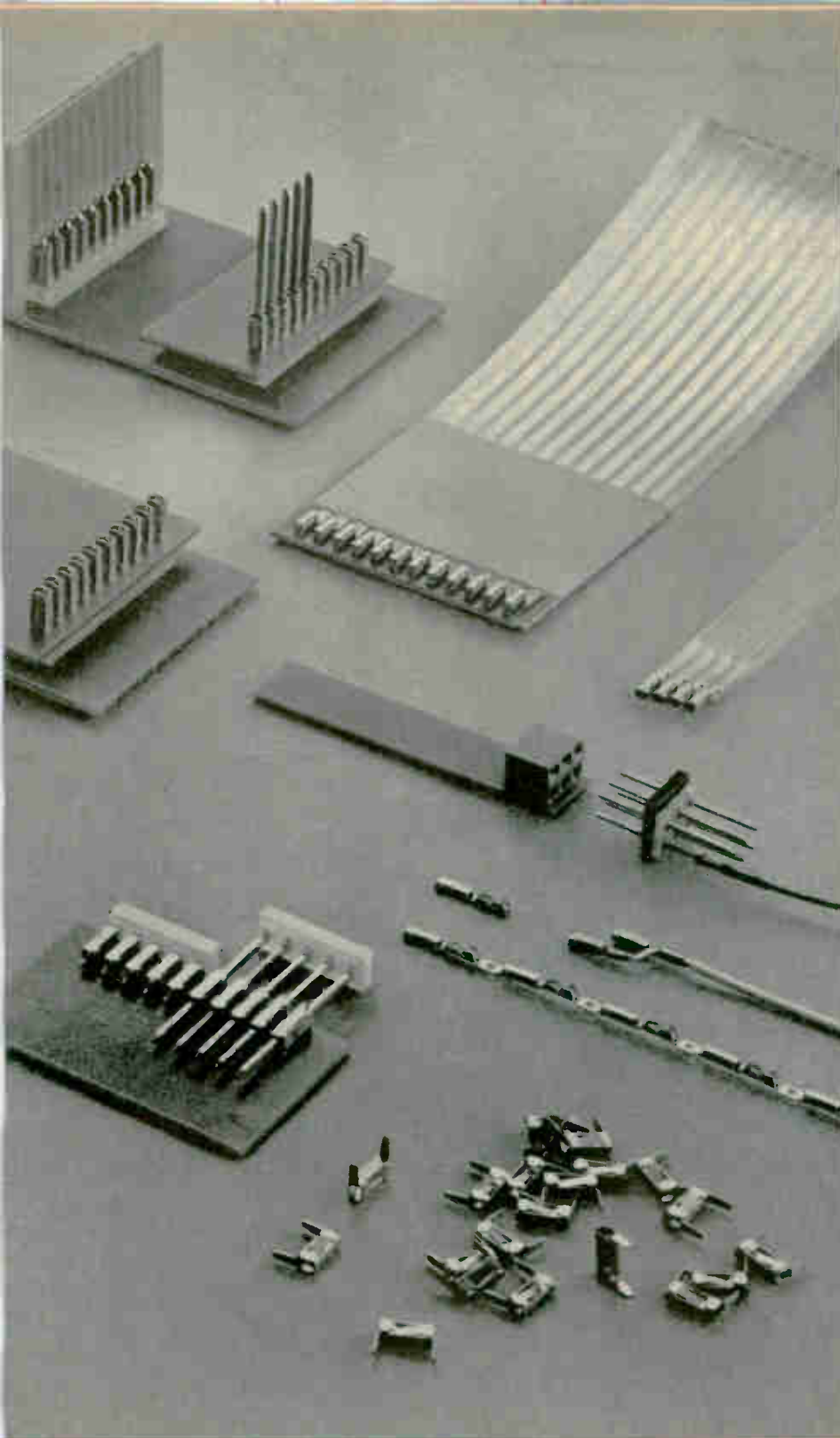
Automatic machines can stake contacts to printed circuit boards at rates of up to 1800 an hour
