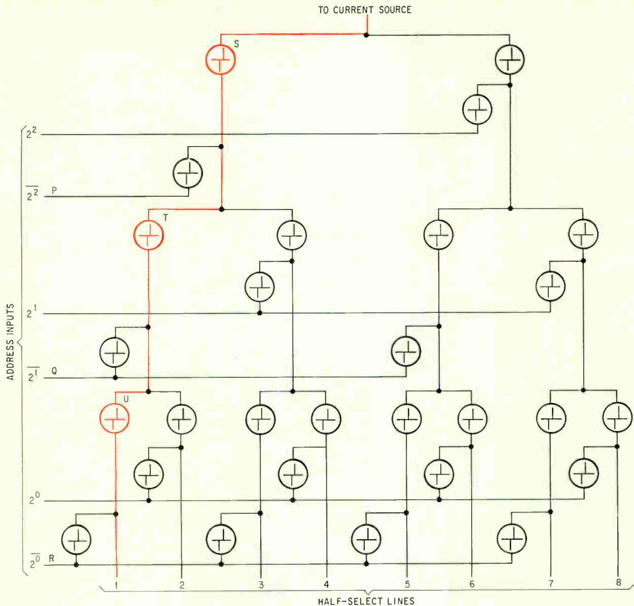
Alternative design. Binary decoder that doesn't require external resistors is made with doubled number of threshold switches, still in single monolithic array. Again, the first half-select line is picked by the switch routing shown in color.
