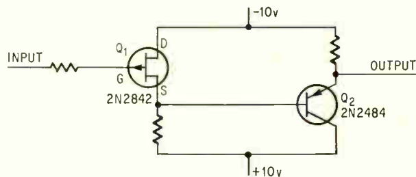
Drift-prone. Simple buffer amplifier is a source follower attached to a conventional emitter follower.
