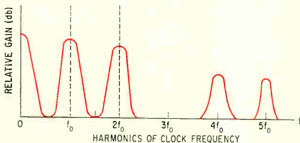
Harmonic response. Frequency spectrum of a three-section digital filter (above) indicates that the bandpass response at the third harmonic is zero. Plot (right) shows how harmonic responses are attenuated with respect to the fundamental frequency. Since the curves were obtained for a three-section filter the value of gain is zero for every harmonic multiple of three.
