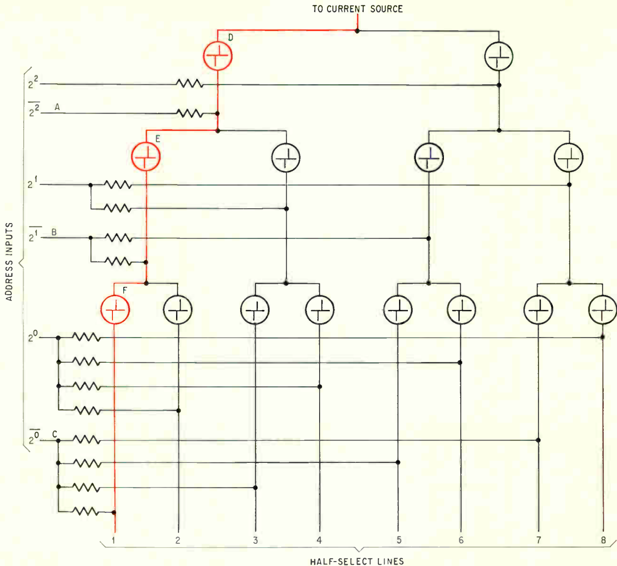
Three-stage matrix. Full internal decoding is possible with threshold switches arranged as binary decoder. As in simpler designs, lines are isolated from one another and all current is routed through the switches, as shown in color for one half-select line. Resistors are external; remainder may be a monolithic circuit.
