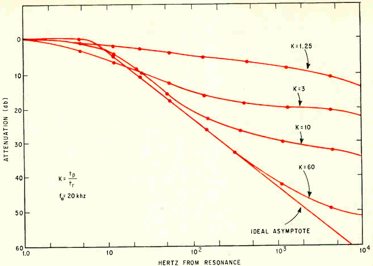
Varying k . As the ratio of pulse time to rise time increases, the shape of the frequency-response curve changes. Plots are obtained for a digital filter centered at 20 kilohertz.
