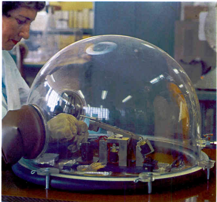
Plastic bubble. During sealing, plastic bubble (also shown on the cover) maintains an inert atmosphere around the switch. A diode envelope is in the sealing nest. When the operator lowers the sealer's arm, it will press the top lead into the envelope and turn on a resistance heating coil.
