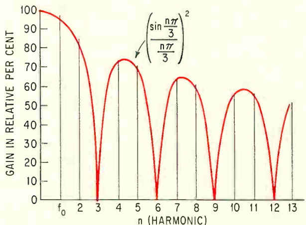
Harmonic response. Frequency spectrum of a three-section digital filter (above) indicates that the bandpass response at the third harmonic is zero. Plot (right) shows how harmonic responses are attenuated with respect to the fundamental frequency. Since the curves were obtained for a three-section filter the value of gain is zero for every harmonic multiple of three.
