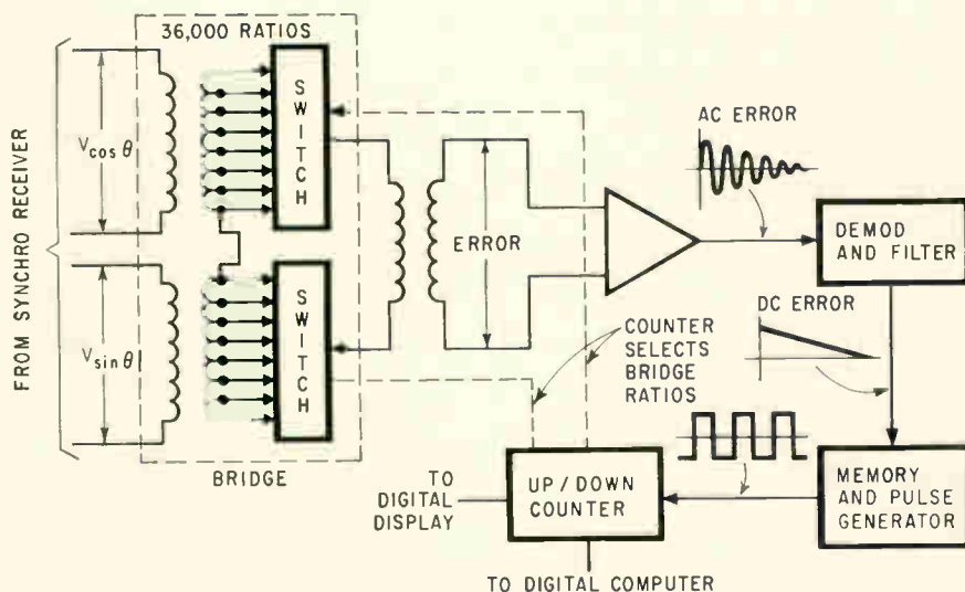
Imbalance at work. Error voltage caused by bridge imbalance drives pulse generator. Output pulses feed an up-down counter to advance digital display.
