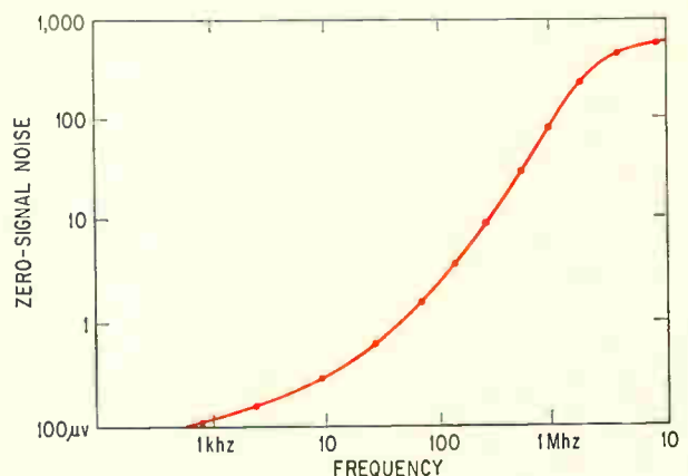
Shifting center frequency. As f_0 increases, the zero-signal noise increases rapidly.
