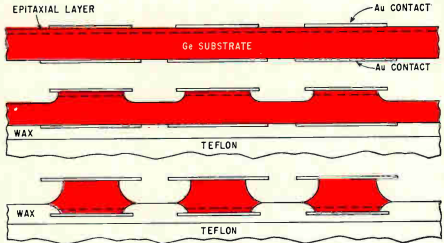
How to make an Impatt. Gold contacts are first deposited on both sides of a germanium slice. With a Teflon and wax support on the opposite side, the junction side is then etched. Finally, the slice is inverted and the diode pellets are etched out. This time the junction side is supported by Teflon and wax.
