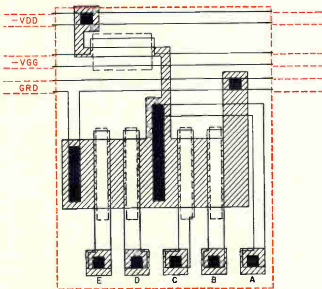
Do-it-yourself. Integrated circuit users can design their own complex circuits with a set of decals supplied by the Microelectronics division of the Philco-Ford Corp. Decal outline, at left in color, corresponds in area and in input-output connections to the composite mask for Philco's building blocks. Decal for an AND/NOR logic function is at right.
