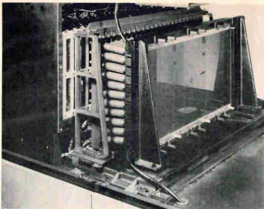
Quick as a flash. Three glass matrix plates, backed by xenon flash units, are the source of type characters in Photon's Zip 901 phototypesetter.
