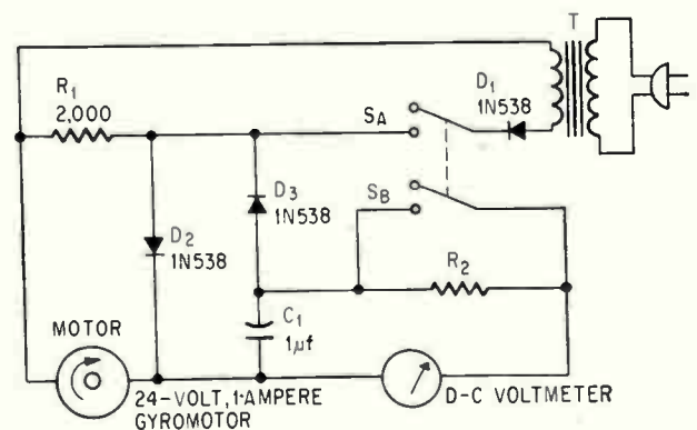
Counter-emf from the motor charges capacitor C_1 between power pulses to indicate motor speed.
