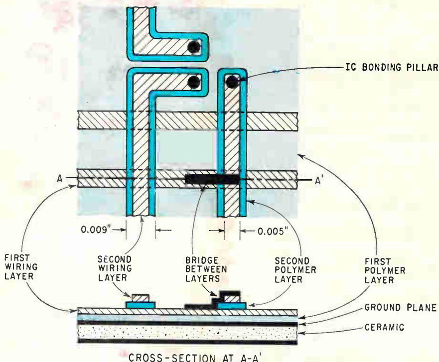
Chip connections. Layers of plastic will insulate layers of thin-film wiring in British firm's new method of interconnecting IC's for computers.
