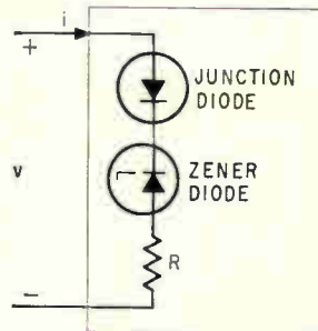
A PRACTICAL REALIZATION OF A CONCAVE RESISTOR
