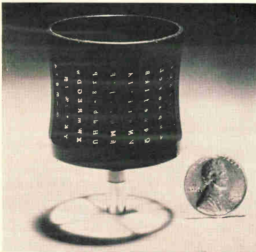
Shot glass. In Fairchild's recently introduced PhotoTextSetter 2000, small "font" can project as many as 264 different type characters.
