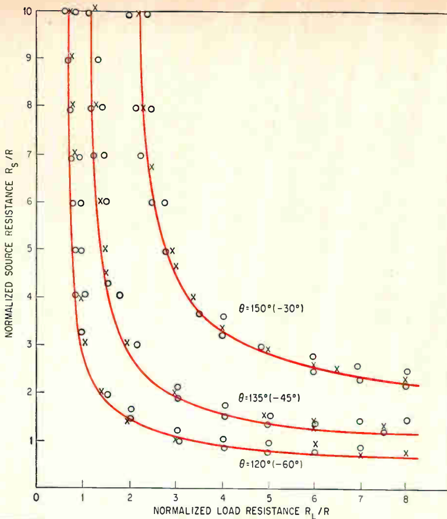
Stability plots for angles in the second quadrant.
