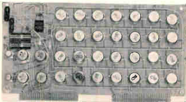
MOS shift registers in TO-5 cans operate at a 1-megahertz bit rate. These 16-, 20-, and 32-bit devices are used to store problems in the calculator's active memory. The p-c boards measure 6\frac{1}{2} \times 4\frac{5}{8} inches.
