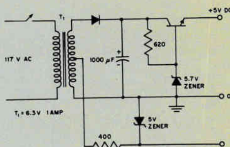
Fig. 2—Power source for low-frequency generator.
