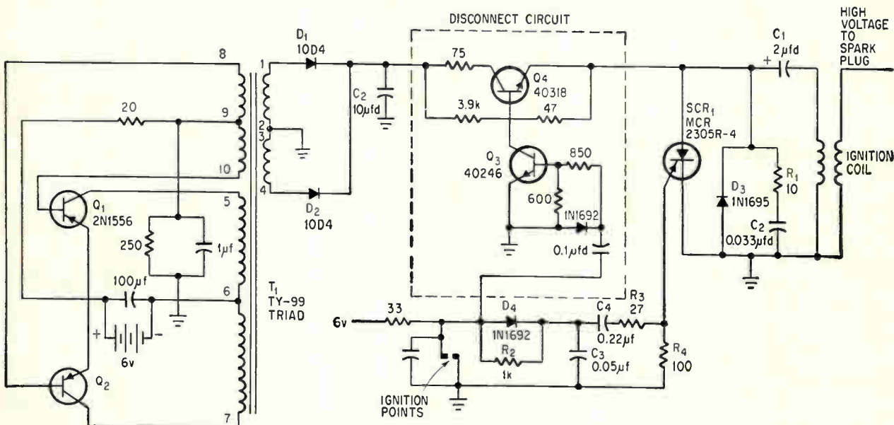
Transistors Q_3 and Q_4 in the disconnect circuit isolate the power supply while capacitor C_1 discharges through SCR_1 .
