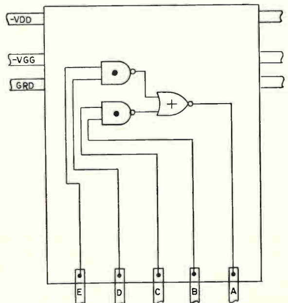
Do-it-yourself. Integrated circuit users can design their own complex circuits with a set of decals supplied by the Microelectronics division of the Philco-Ford Corp. Decal outline, at left in color, corresponds in area and in input-output connections to the composite mask for Philco's building blocks. Decal for an AND/NOR logic function is at right.
