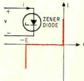
i-v CURVE OF A ZENER DIODE
