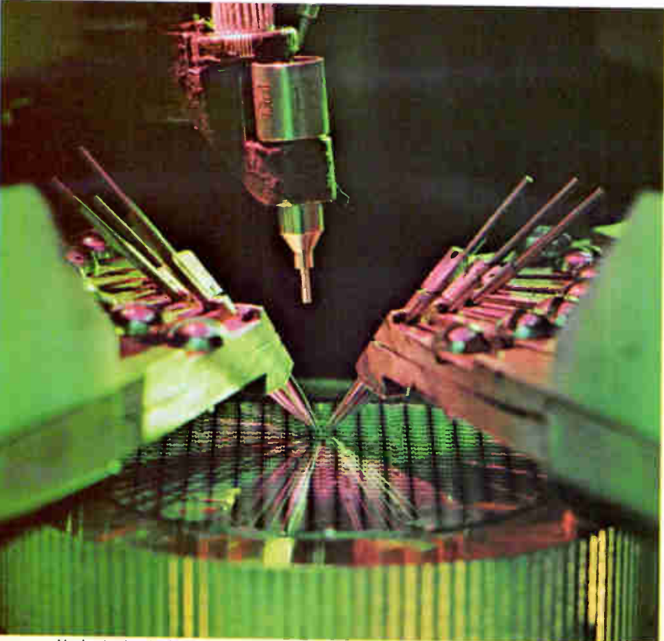
Mechanized water-level testing with this 14-point probe.
