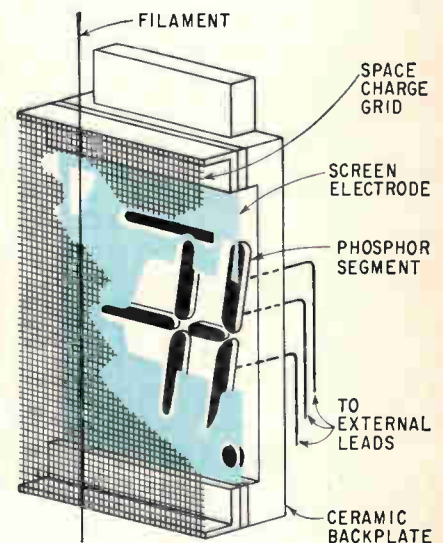
Planar display. New digital readout tube draws as little as 15 volts. Cathode mounted up front in envelope is invisible when number-segments glow.
