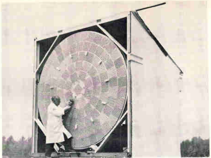
In the round. Technician installs new dipoles on secondary array of RCA's experimental electronically scanned phased-array radar.
