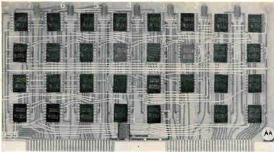
Diode-transistor-logic IC's are in TO-88 flatpacks. The multifunction devices include triple three-input NAND gates, RST binaries, and dual four-input line drivers. The N prefix denotes an operating range of 0° to 70°C—a limited range suitable for ground support equipment.
