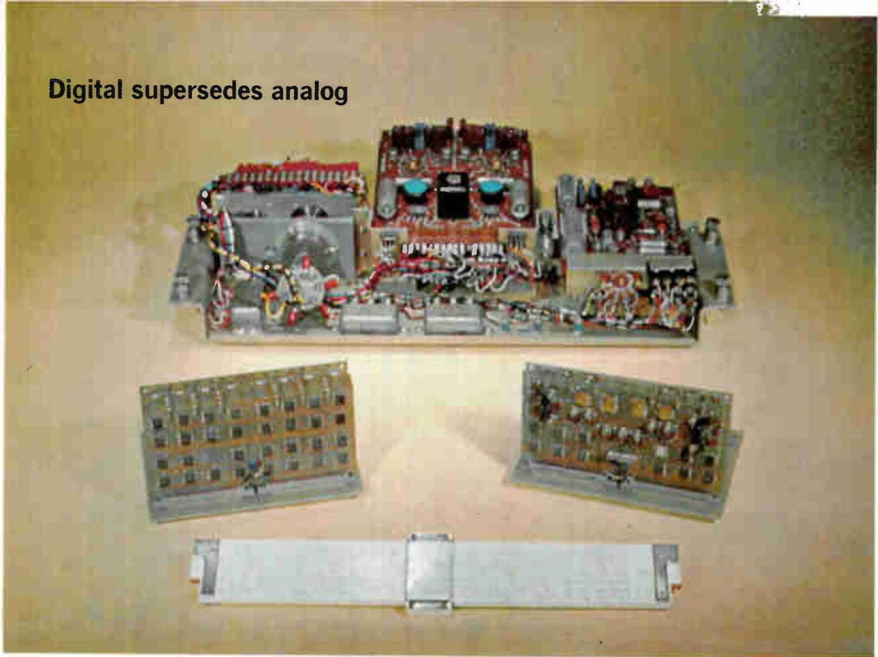
Analog resolver in the background dwarfs IC equivalents. Four-board IC version, left, uses MOS shift registers, and bipolar arithmetic, logic, and timing. A later two-board version at the right has MOS shift registers and digital differential adders, plus bipolar timing.
