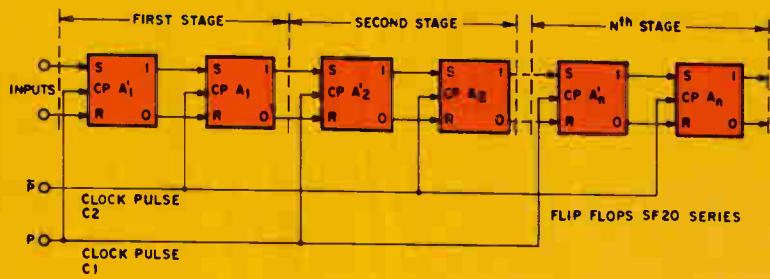
Fig. 2—Shift register—dual rank.
