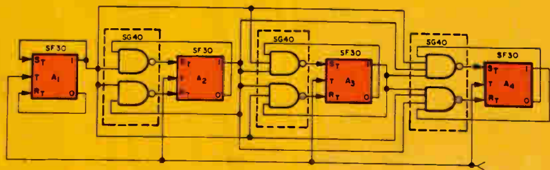
Fig. 3—Synchronous binary counter with SRT flip-flops.
