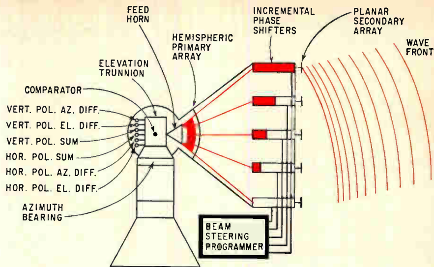
New phase. In an electronically scanned antenna mounted on conventional monopulse pedestal, beam-steering programmer excites ferrite phase shifters to phase-delay signals that are picked up by the primary array's dipoles; the beam can be steered \pm 5^\circ around antenna's axis to form a 10^\circ cone.
