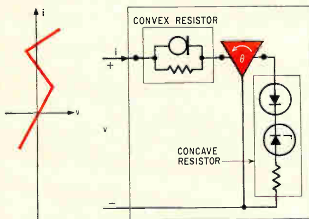
Current-controlled i - v curve (top) is obtained with a convex resistor connected to an R-rotator and a concave resistor. Two concave resistors connected to an R-rotator (right) produce voltage-controlled i - v curve.
