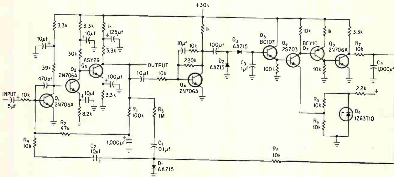
Transistors Q_1 , Q_2 , and Q_3 constitute a basic amplifier in which the gain is controlled by a correction signal generated by the remainder of the circuit.
