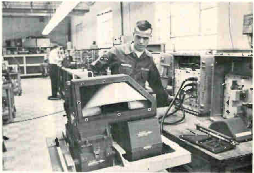
Auxiliary data annotation system prints in binary form information on the sensor being used, altitude, longitude, and time. Data is presented on the 4-inch cathode-ray tube on top of the unit. The goal is to add data in easy-to-read alphanumeric symbols.
