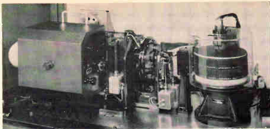
Spinner. In the Photon 713-40, a rotating character drum (right) is set and characters are projected as a stationary internal flash unit is fired.
