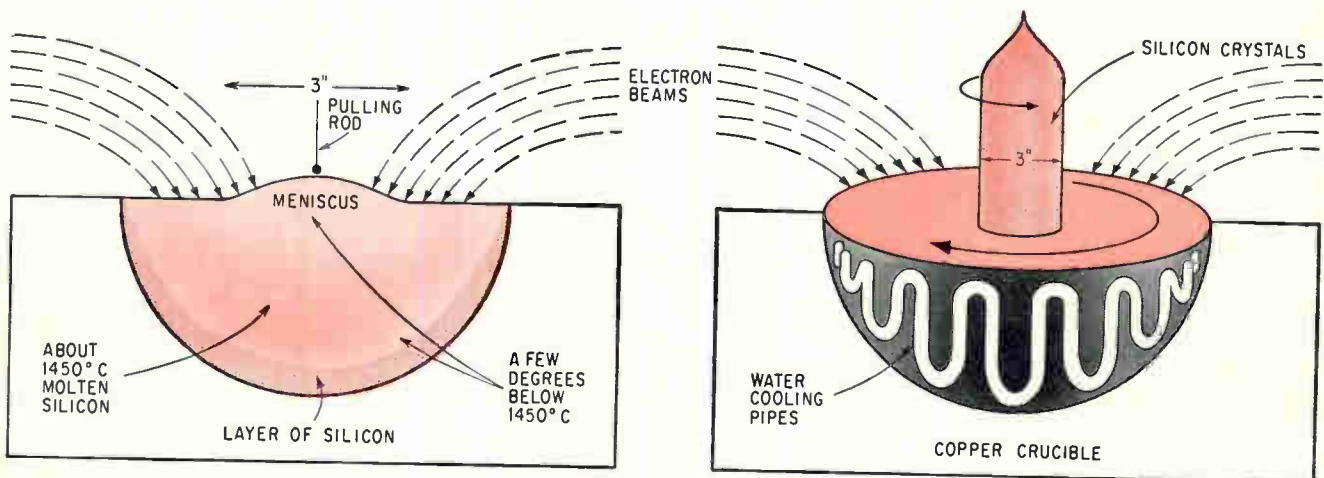
Crystal-pulling. High-purity silicon crystal rods, up to three inches in diameter, are produced by process developed by Temescal Corp. of Berkeley, Calif. The advantage of the technique lies in its repeatability. Large, high-purity crystals are needed in increasing numbers as more companies turn to large-scale integrated circuits.
