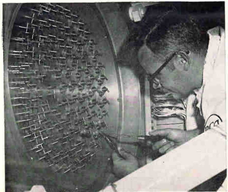
Each dipole on the primary array is oriented to the geometric center; array's configuration enables it to transmit cross-polarized beams.
