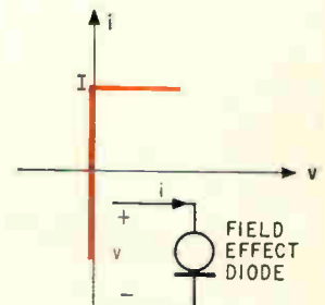
i-v CURVE OF A FIELD EFFECT DIODE
