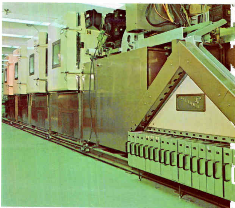
MR. ATOMIC tests each Sylvania IC in four temperature-controlled chambers.
