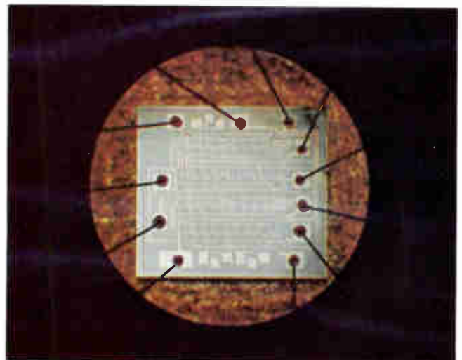
MOS shift register by Philco-Ford Microelectronics division is typical of those in calculator. It can be connected as a dual 8-, dual 16-, single 24-, or single 32-bit delay.
