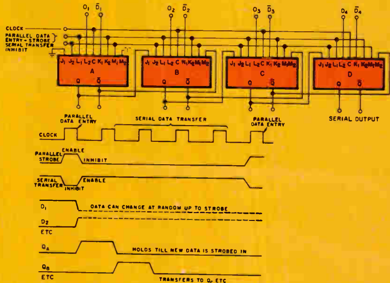
Fig. 5—In parallel to serial converter data is inserted through one set of DRed Inputs on each flip-flop.
