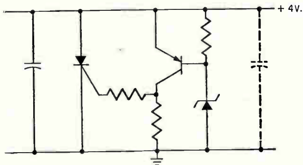
Thyristor sensing circuit protects integrated circuits from overvoltage. It detects voltages above 6 v and shunts the power source. Capacitor at right represents bypass capacitors on logic boards.
