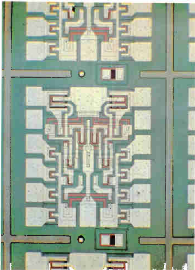
Dual buffer, Signetics' NE156, is used in clock and capacitive line-driving applications and is typical of the calculator's monolithic DTL circuits. Each of the two symmetrical sections contains four input diodes, four transistors, and seven diffused resistors.
