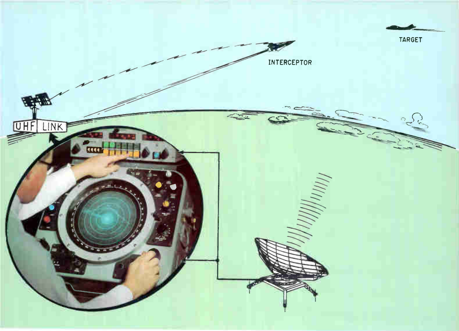
Ground-based radar operator zeroes in on the target, controls data input to the intercept calculator, and selects appropriate intercept tactics. The calculator confirms the target's location and computes distance, velocity, and time to intercept.
