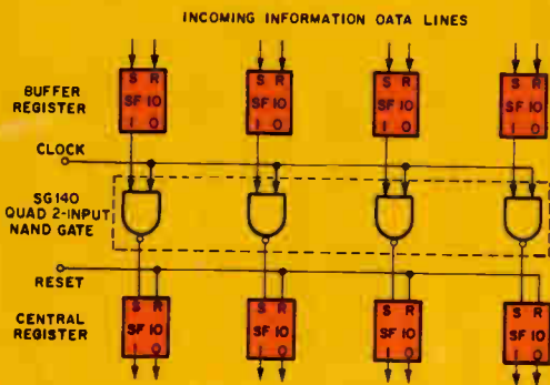
Fig. 1—Flip-flop register application.
