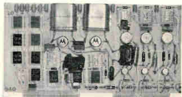
Clock circuit using these transistors and conventional discrete components is typical of those circuits in the calculator that don't lend themselves to all-IC construction.
