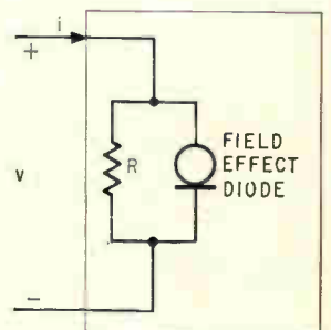
A PRACTICAL REALIZATION OF A CONVEX RESISTOR
