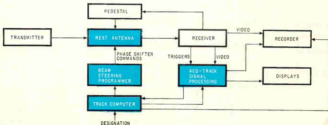
On a new track. Adding the components, in color, converts conventional monopulse radar systems into phased arrays that can follow up to 20 targets simultaneously; the technique, developed by RCA, can be used on any dish-type antenna.
