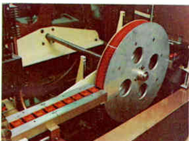
Fifth testing station tests 30 switching parameters at 25°C.
