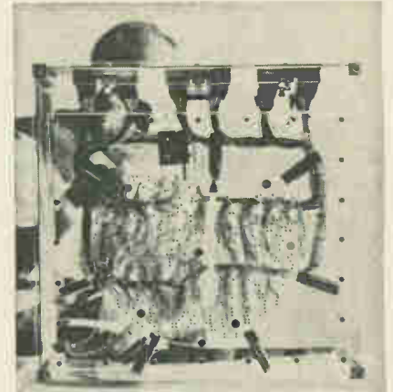
View through transparent chamber shows wiring harness between probe and multipin connectors, for connection to an automatic circuit analyzer.
