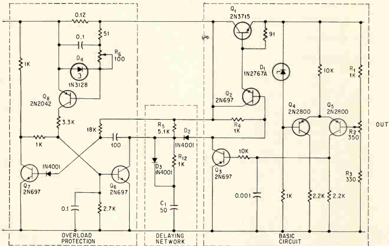
Regulator includes an overload circuit—to protect the series pass-transistor, Q_1 , against damage from short-circuited loads—and a delaying network to prevent oscillations when connected to a capacitive load. The network does not increase the response time under varying load conditions.
