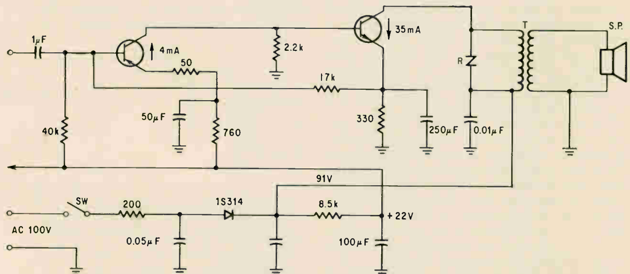
In the output stage of a home radio, a high voltage passivated mesa transistor is protected by a silicon varistor.
