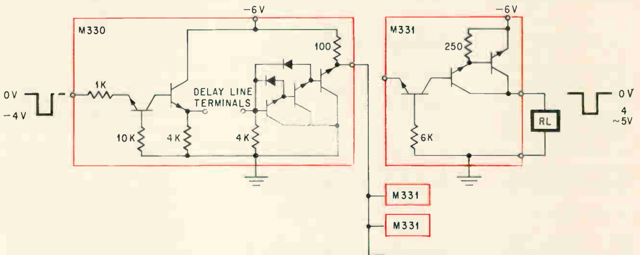
Synchronizing signal is distributed to several television cameras by this integrated circuit composed of two chips (photos). One chip (circuit diagram in box at left) is input section, other is output. Additional output chips for more cameras can be added in parallel.
