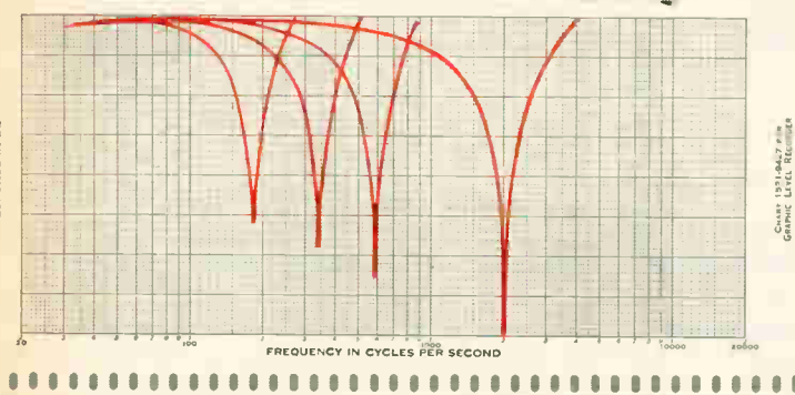
Recording of transmission characteristics of an adjustable notch filter for four different frequency settings. This plot is a permanent ink recording on 4-inch-wide chart paper. Dynamic recording range is 40 dB (20- and 80-dB dynamic ranges also available). Recorder chart speed and pen writing speed can be set over ranges of 2.5 to 75 in/min and 1 to 20 in/s, respectively.
