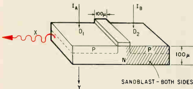
Roughening two parallel faces of a laser diode by sandblasting redirects the light to the other sides. Light transmitted in the Y direction by diode D_1 depends on current carried by diode D_2 , as shown by the curves.
