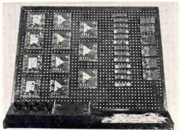
Computer fundamentals laboratory unit, made by Philco for student use, has clip leads for interconnections.
