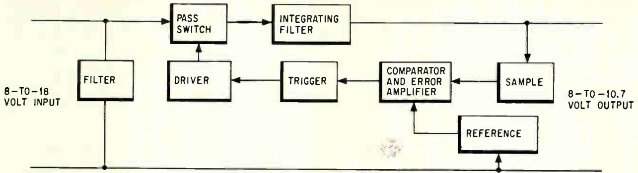
Block diagram of the 10-volt 1-ampere regulated supply.
