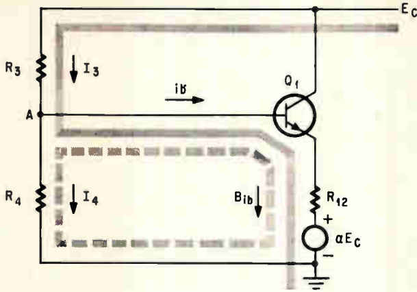
Equivalent complementary monostable circuit
