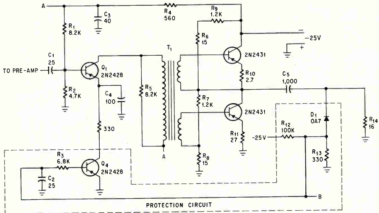
The protective portion of the circuit is contained within the dashed lines.
