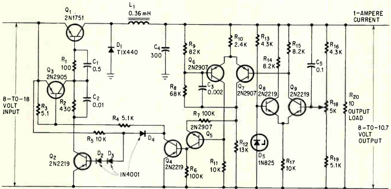
The circuit allows efficiencies from 90% to 97% depending upon the input voltage.
