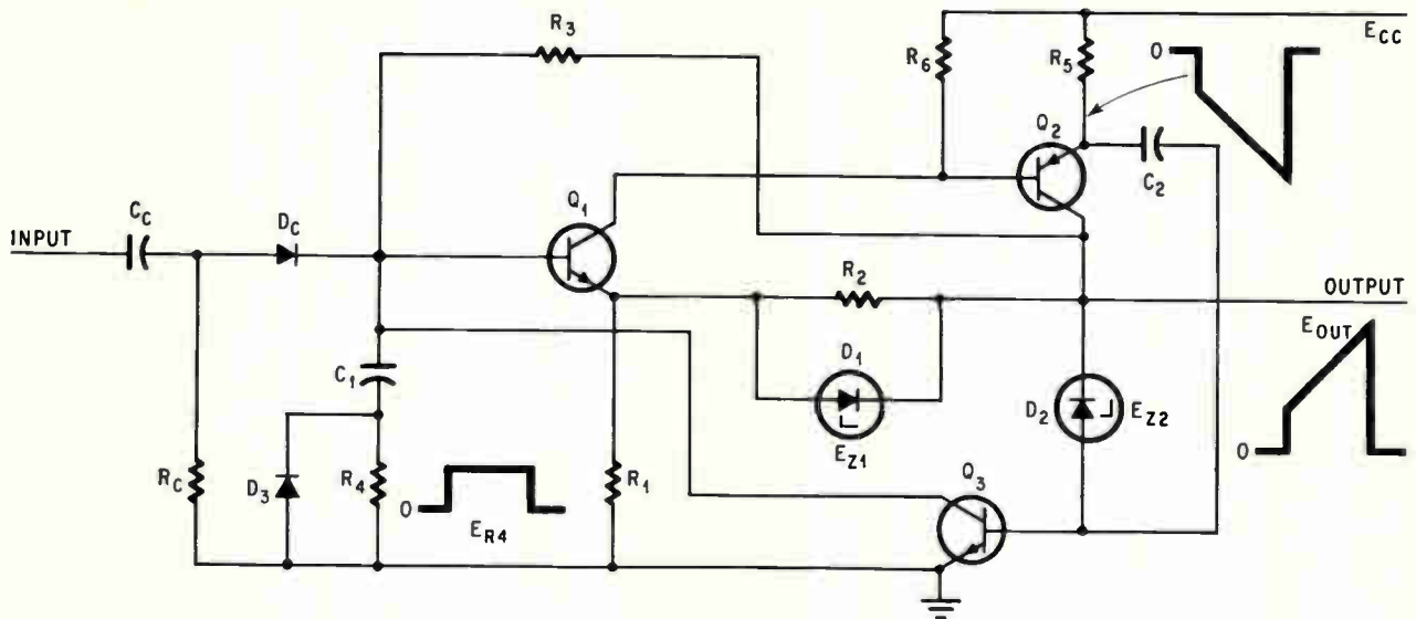
Modified complementary monostable circuit
