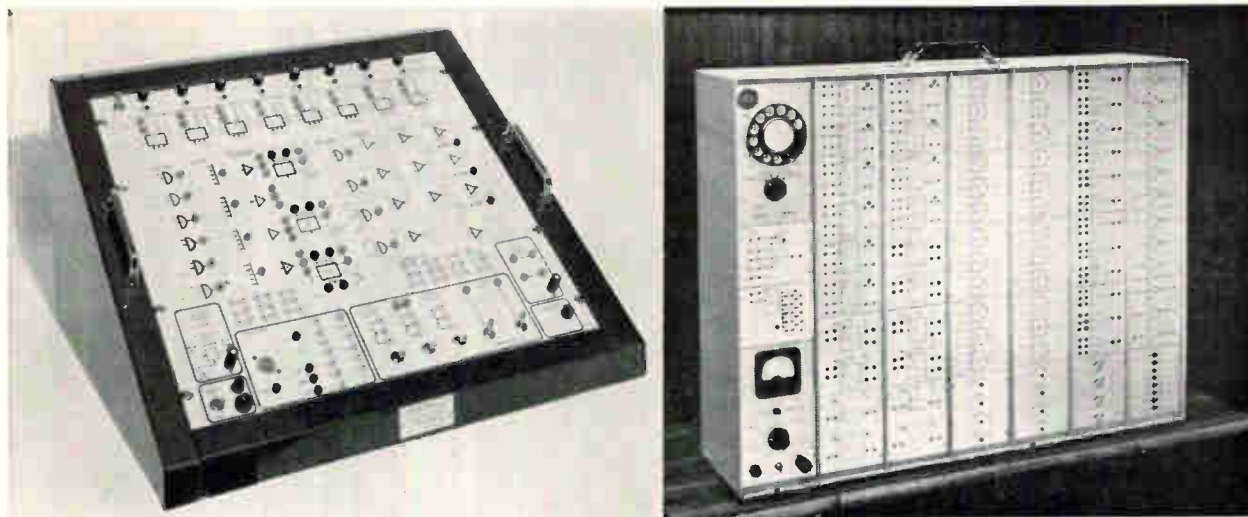
Desk-top logic trainers, in fixed configuration (left) by Epsco and in variable layout (right) by Vitro.
