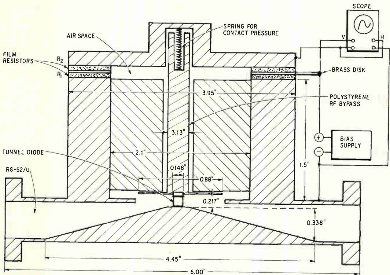
Cross-sectional view of tunnel diode mounting arrangement
