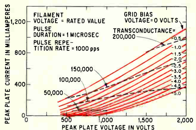
Average plate characteristics for pulsed operation
