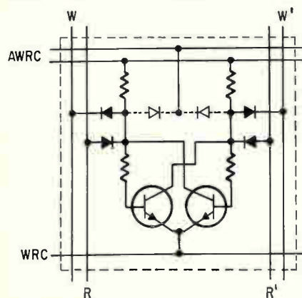
Microelectronic element wired as part of a memory.
