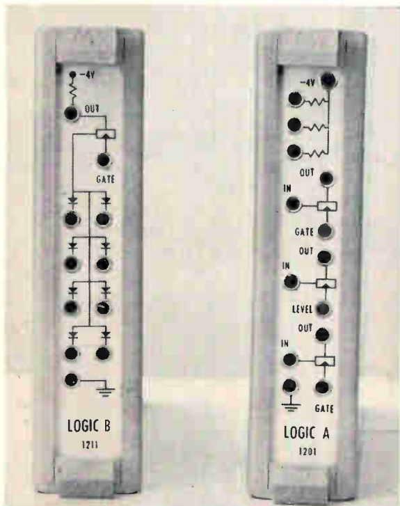
Front-panel logic modules by Digital Equipment (top) and H-W Electronics (bottom left); training aid incorporating H-W modules (bottom right).
