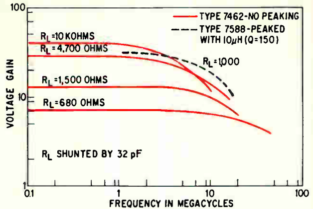
Single-stage gain versus frequency for ceramic-tube video amplifiers
