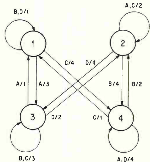
Typical element state-transition table defines the behavior of each element under given stimuli, top. The same information can be represented in a sequential state diagram, bottom.
