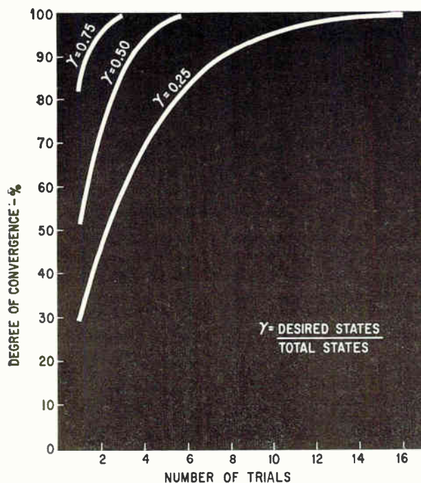
The degree of convergence for an array of 100 four-state polystable elements, such as used in the experiments, can be shown to vary with the value of ratio \gamma .
