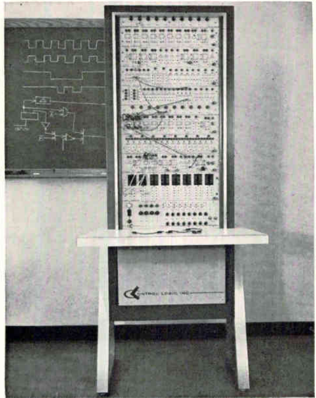
Fixed-panel console by Control Logic, for various combinations of panels.
