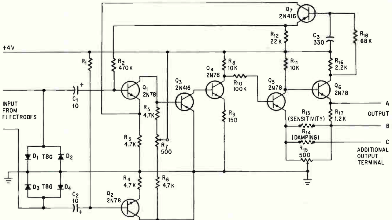
Low-level a-c amplifier circuits provides automatic temperature compensation.
