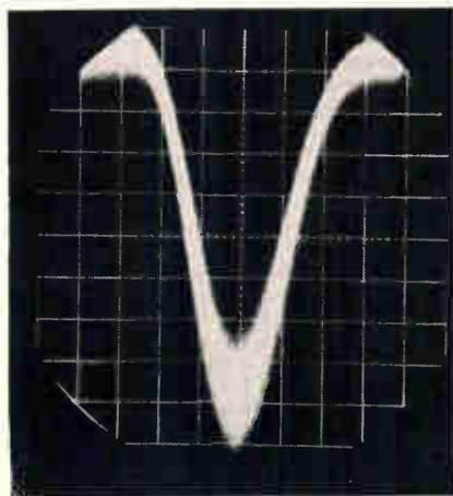
Output waveform observed on oscilloscope. The bias voltage is 340 millivolts; the output amplitude is 20 db above noise; the frequency is 7565 Mc.
