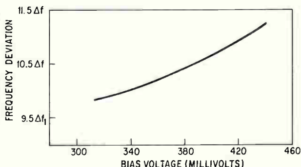
High-frequency deviation characteristics in terms of \Delta f_1
