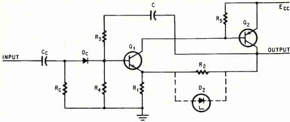
Basic complementary monostable circuit
