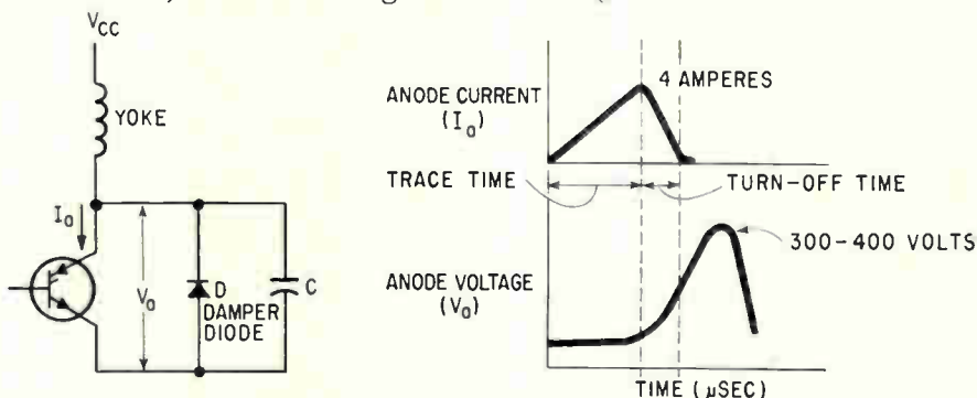
Simplified horizontal-sweep circuit (left). The turn-off time (see waveform at right) is minimized to limit heat generation in the controlled rectifier.
