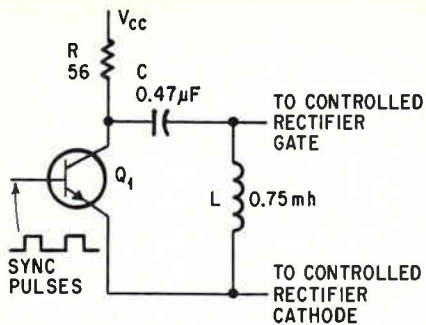
New driver circuit. Sync pulses saturate the driver transistor permitting capacitor C to charge.
