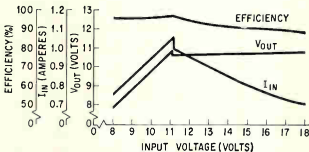
The characteristics of the regulated output plotted for various input voltages.
