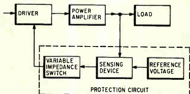
Block diagram for the audio amplifier driver and output stages.
