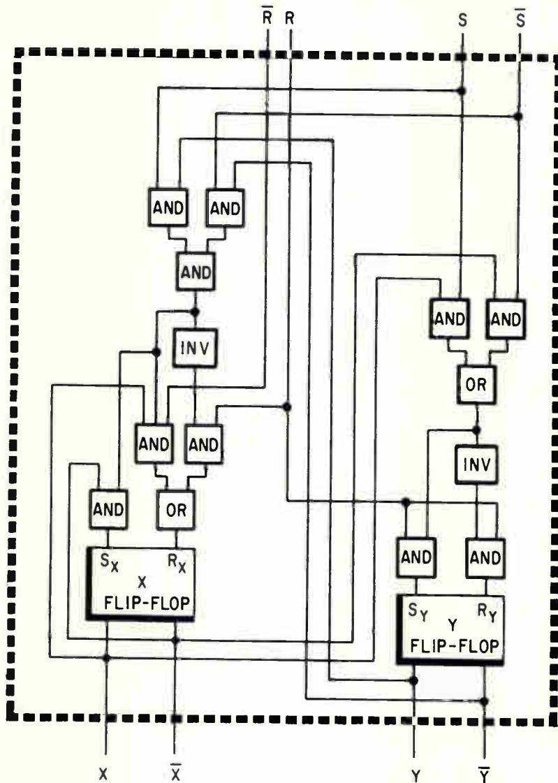
Logical implementation of a typical polystable element, with inputs R and S and outputs X and Y, can be built using standard digital logic modules for gates and flip-flops.
