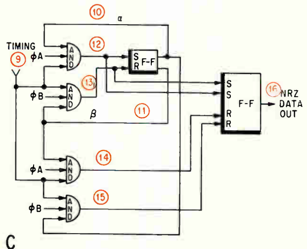
Recording system (A), phase-locked oscillator (B) and decoder (C) of the diphase recording system.
