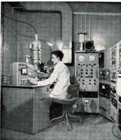
Electron-beam system gives both a qualitative and quantitative analysis of inclusions in steel.
