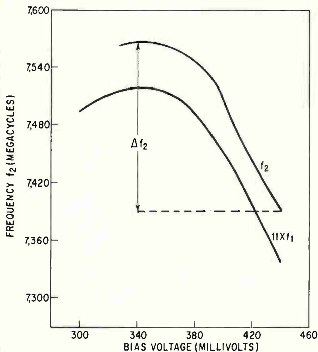
High-frequency characteristic ( f_2 ) and postulated eleventh harmonic of f_1
