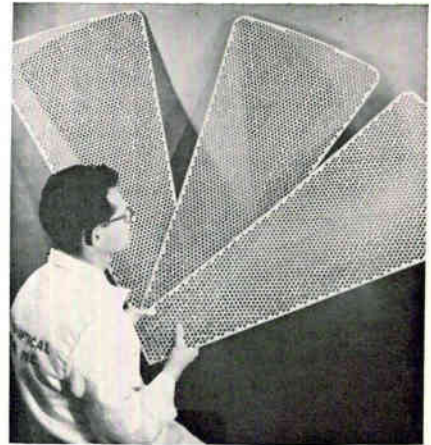
Parabolic sections, called petals, are made of hollow nickel plate only 1 mil thick.
