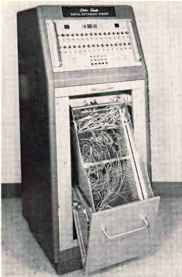
Plugboard trainer by Delco Radio for teaching or checking out digital systems
