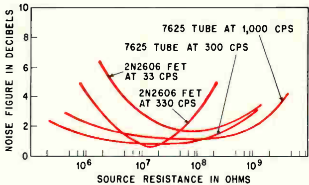
Comparison of noise figure versus source resistance for ceramic tubes and field-effect transistors
