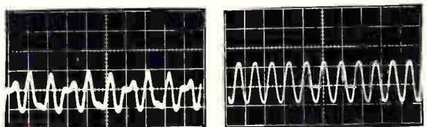
Accurate detection of data, and alternate one-zero nrz message, as played back from the head (left) and the diphase signal from the tape (right). The signal has been filtered through an Inter-range Instrumentation Group standard pcm premodulation filter.
