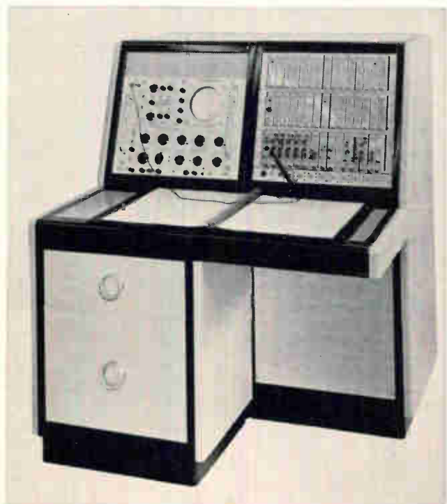
Front-panel logic modules by Digital Equipment (top) and H-W Electronics (bottom left); training aid incorporating H-W modules (bottom right).
