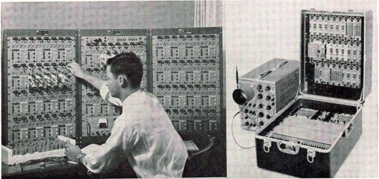
Front-panel cards show logic diagrams for T-series circuits (left) and high-speed U-series modules (right), both by Engineered Electronics.
