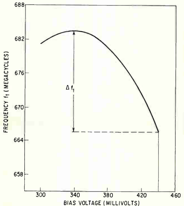
Low-frequency characteristic for the A650
