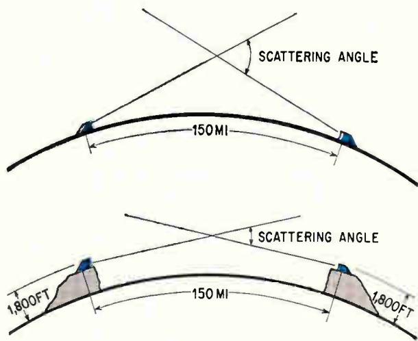
Two pairs of sites (color) for the same distance may produce considerably different angles. Since a small scattering angle is generally desired, sites with good elevation are chosen.
