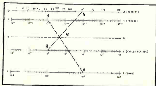
Nomograph simplifies phase-shift calculations.
