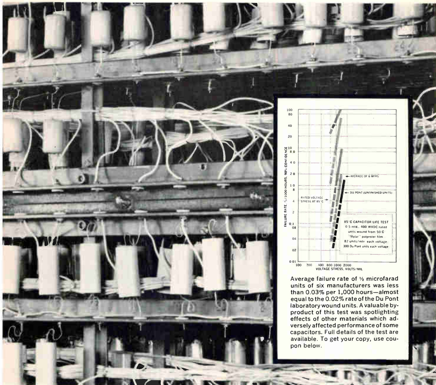
Commercial capacitors on test racks at Inland Testing Laboratories of Cook Electric Company in 23,000,000 unit-hour Du Pont reliability test.
