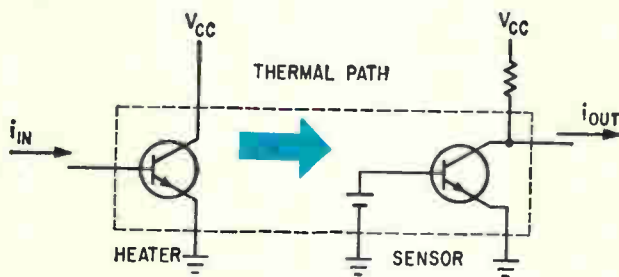
Thermal transfer element consists of heater and sensor transistors in a common silicon substrate.
