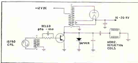
Video horizontal deflection with the Delco DTG-1010
