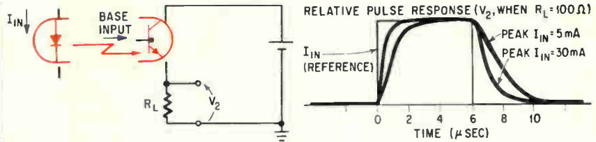
The simple isolated line coupler (A) has the basic circuit shown in (B) and exhibits the typical pulse response (C). Its isolation properties extends from d-c to the cutoff frequency of the device.
