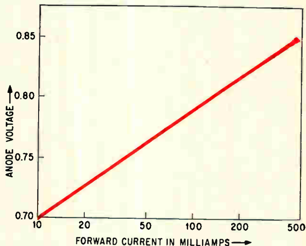
Voltage drop in conducting switch. Graph uses a semi-logarithmic plot.
