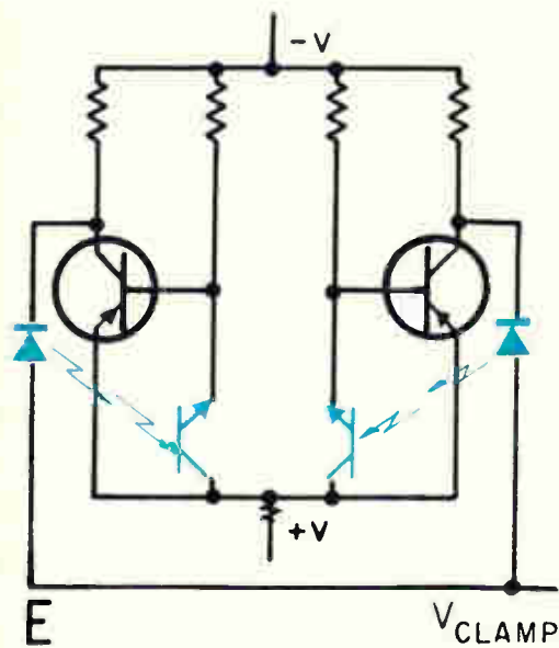
Six versions of the symmetrical Eccles-Jordan flip-flop circuit have photon coupling: between the collector-to-collector and the series-base element (A); between the collector-to-collector and the shunt-base element (B); between the series collector and the shunt-base element (C); between the series emitter and the shunt-base element (D); between the collector clamps and the shunt-base element (E), and between the shunt collector and the collector-base element (F).
