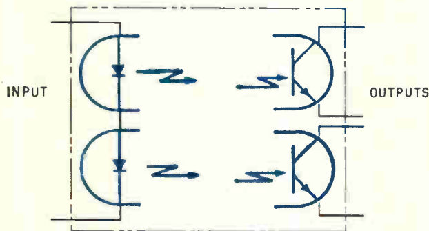
Optical devices improve the speed and reliability of the double-pole, single-throw relay.
