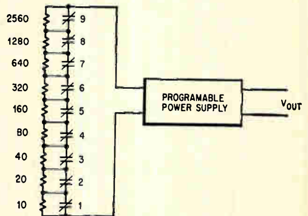
Technique for programming a power supply, with a binary-weighted resistor string controlled by normally-closed relay contacts. Output voltage is KR_{1n} , where K equals IV/(100 \text{ ohms}) .
