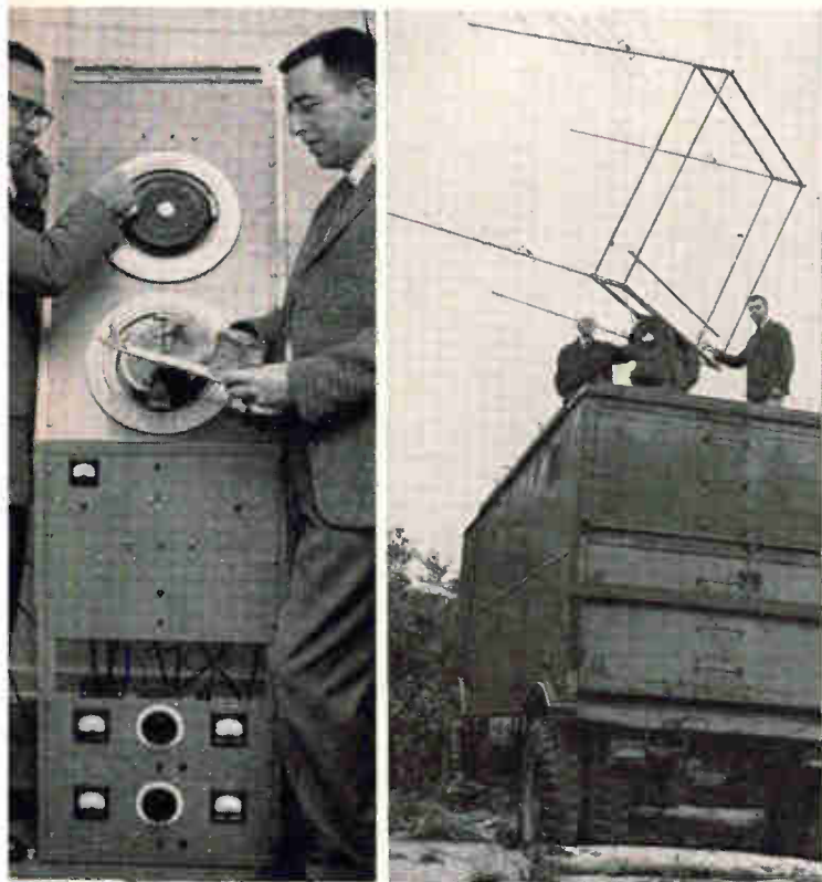
Canadian station at Ottawa has antenna programmer (left) to point the antenna directly at the satellite. Antenna at right was built by Danish Meteorological Institute from available radar equipment and has a gain of about 15 db.
