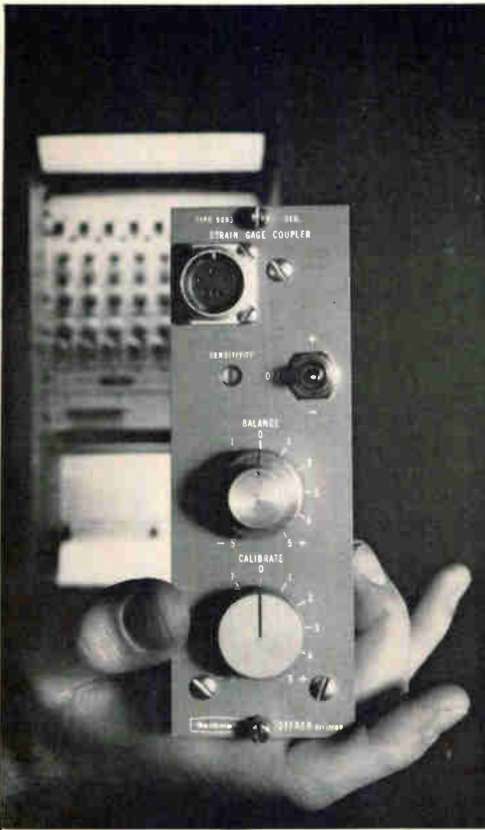
LOW-COST PLUG-IN INPUT COUPLERS ALLOW THE TYPE S RECORDER TO ACCOMMODATE A WIDE RANGE OF INPUT SIGNALS. 23 STANDARD COUPLERS ARE AVAILABLE.
