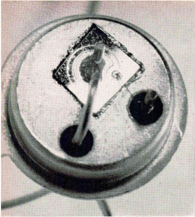
Desensitized silicon pnpn switch, prior to encapsulation.
