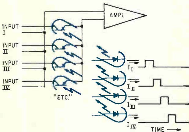
Information on the n-parallel input channels is fed serially to the single-channel multiplex amplifier. The time-sequencing controls are electrically separated from the information signals.
