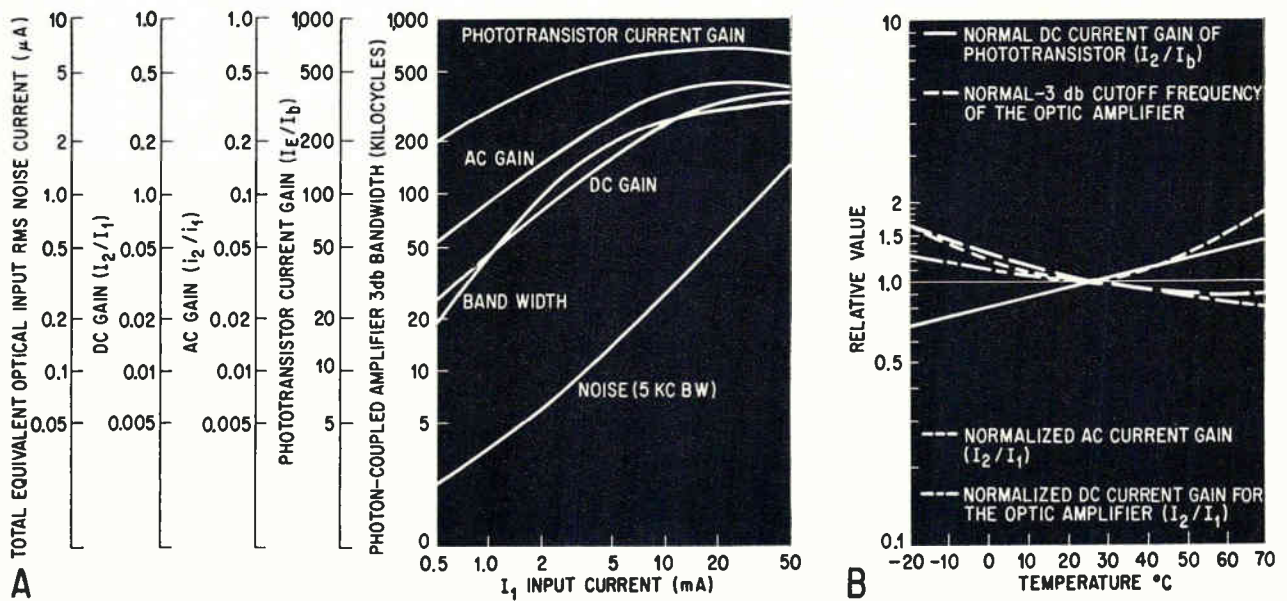
Parameters vary with the input current which is the primary independent variable for the photon-coupled amplifier (A). Some important parameters are temperature-dependent (B).
