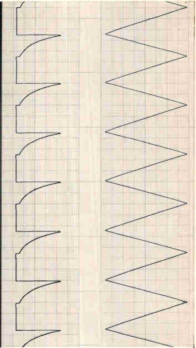
OFFNER TYPE S DYNOGRAPH® IS SERVO CONTROLLED AT THE PEN POINT TO ASSURE LOCKED-IN ACCURACY.
