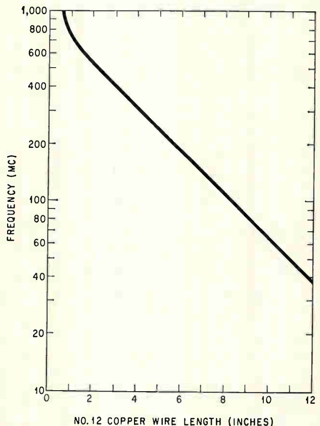
Chart gives lengths of tank coil wire.
