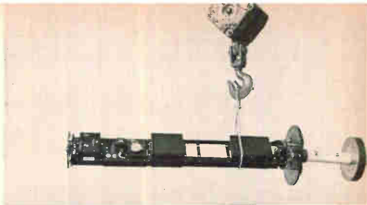
Free-floating buoy retransmits Consolan signals to keep the base station or research vessel aware of the buoy's position.
