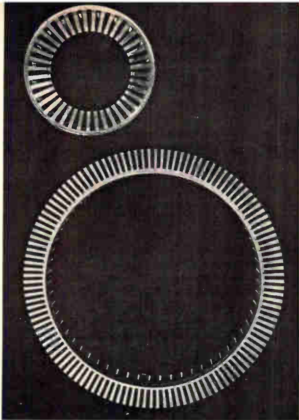
Microwave anode structures demonstrate intricacy of parts as frequency rises. Vane lengths are about one-quarter wavelength. Largest of these disks is about four inches in diameter.
