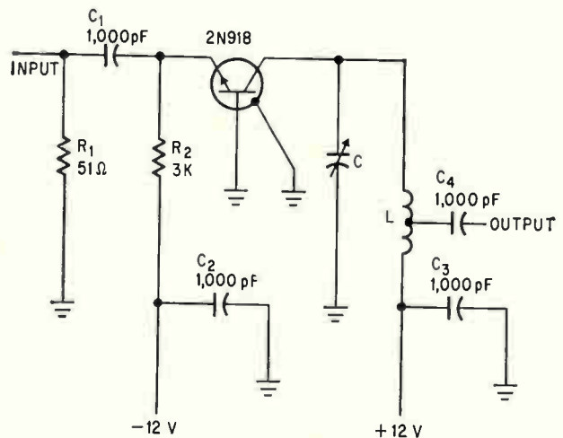
One-stage amplifier or frequency doubler
