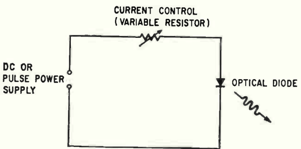
Simplified circuit diagram of a radiation-emitting optical diode
