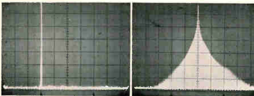
Spectrum analyzer scope shows calibrated 2-Gc sweep, 60-db dynamic range. A pure 800-Mc signal is shown at left. Sweep is 2 Gc centered at 1.2 Gc. Vertical scale is 10 db/cm. Absence of second harmonic signal demonstrates suppression of internally generated responses. Photo at right displays spectral analysis of 800 Mc. 1 \mu sec pulse. Sweep is 300 Mc. centered at 800 Mc. Vertical scale is 10 db/cm.
