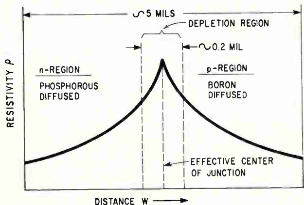
The resistivity profile of the special diffused varactor enhances charge storage. The electric fields set up by the steep resistivity gradients keep the minority carriers close to the depletion layer.
