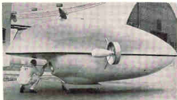
Deepstar research vehicle is designed to attain a depth of 4,000 feet. Later versions may reach 12,000 feet.
