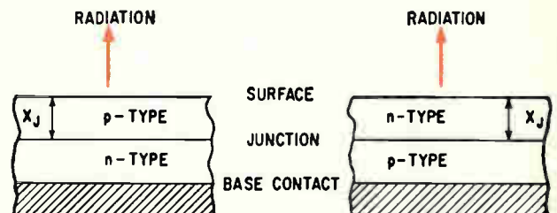
Basic geometry for the p- and n- surface, employed as the exit surface of diode radiation
