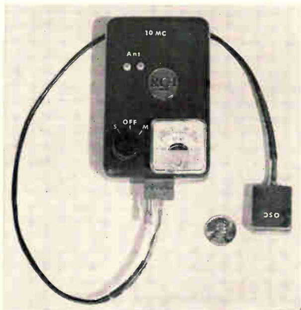
Prototype of the 10-ounce transmitter for operation at 10 mc shows the separate oscillator capsule that is held in the armpit for temperature stability.
