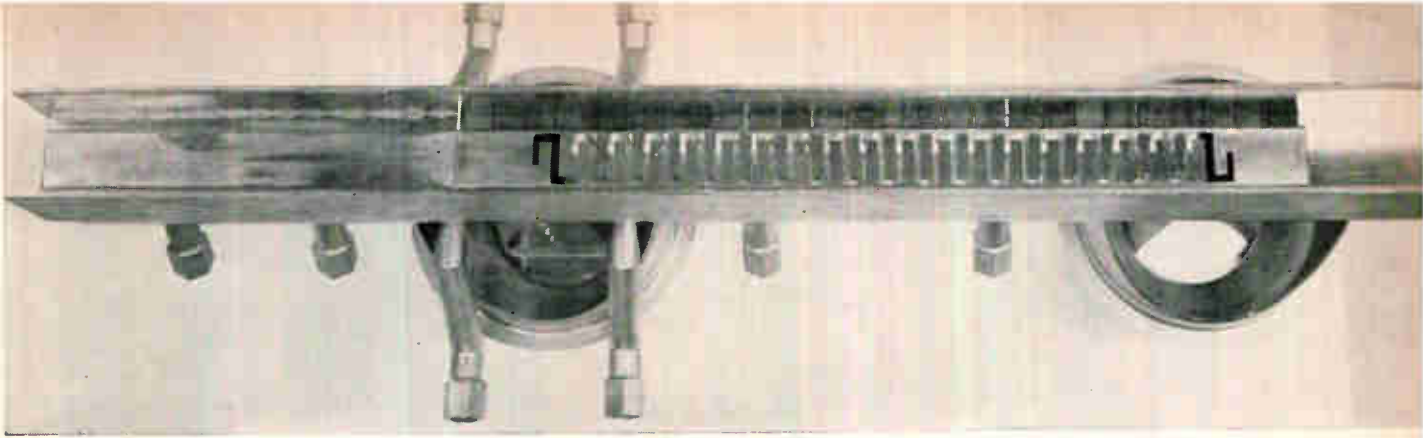
Superpower crossed-field amplifier, a Litton L-3778, with r-f input at right and delay line exposed. This tube has a bandwidth about four times as broad as a klystron's.
