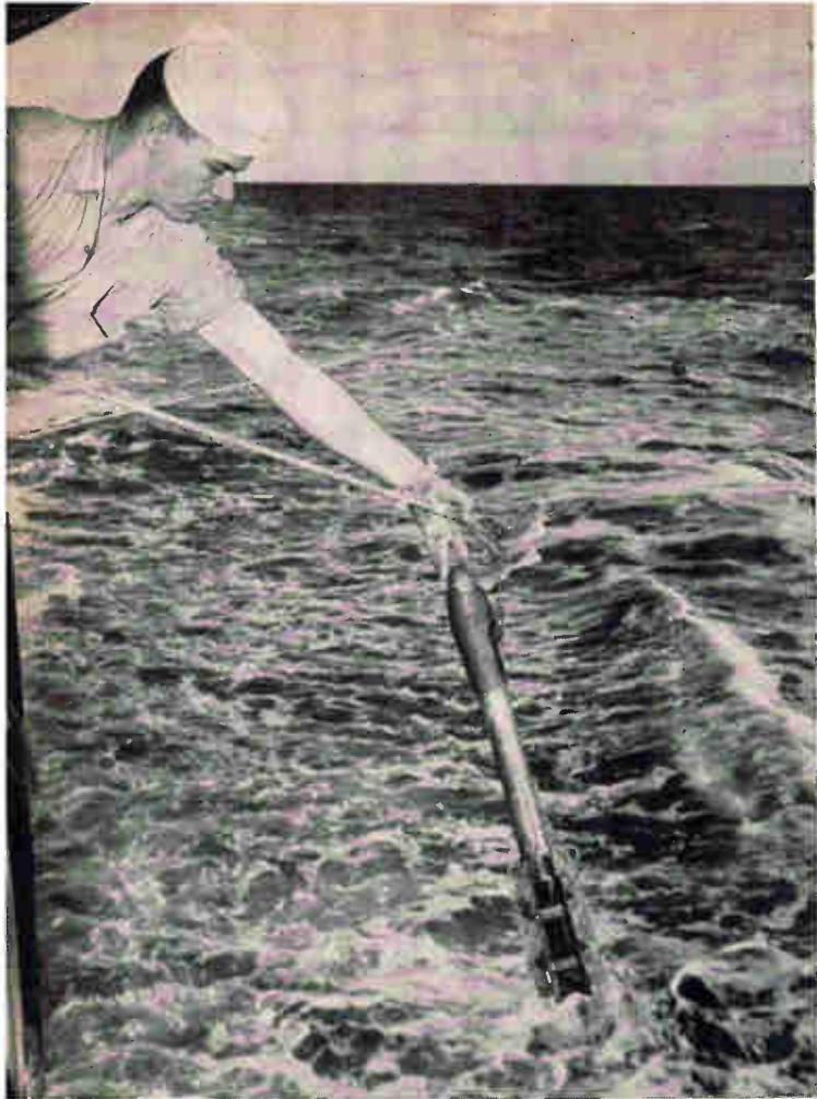
BT WINCH plunges hundreds of feet of wire, with a bathythermograph attached, into the sea.
