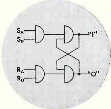
Flip-Flop Circuit
