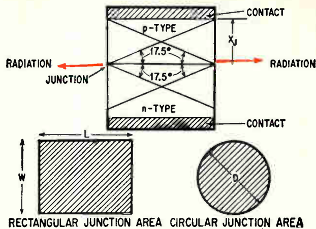
Rectangular and circular junction geometries, in each case using edge emission.
