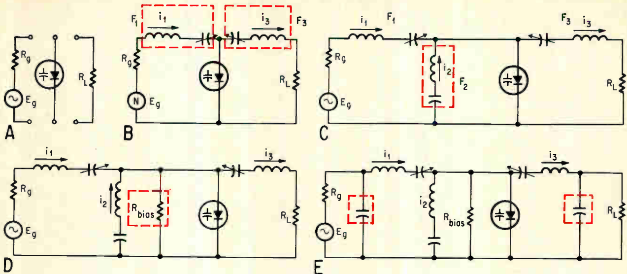
Development of a multiplier circuit starts with a varactor converting the signal to harmonic current through the load (A). Input and output circuits (color) are added for suitable current paths (B). If the desired load current is at the third or fourth harmonic, an idler circuit (color) is added (C). A bias resistor (color) provides bias voltage (D). Input and output matching capacitors (color) provide proper matching between the source and load (E).
