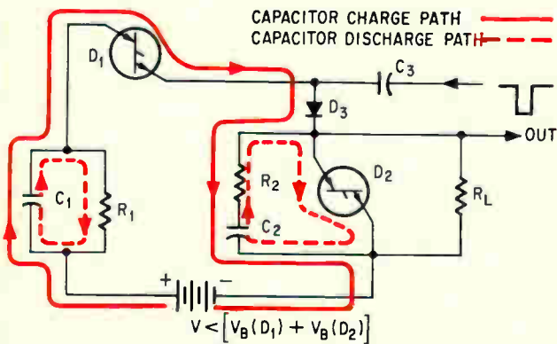
Synchronized staircase wave generator using four-layer diodes.
