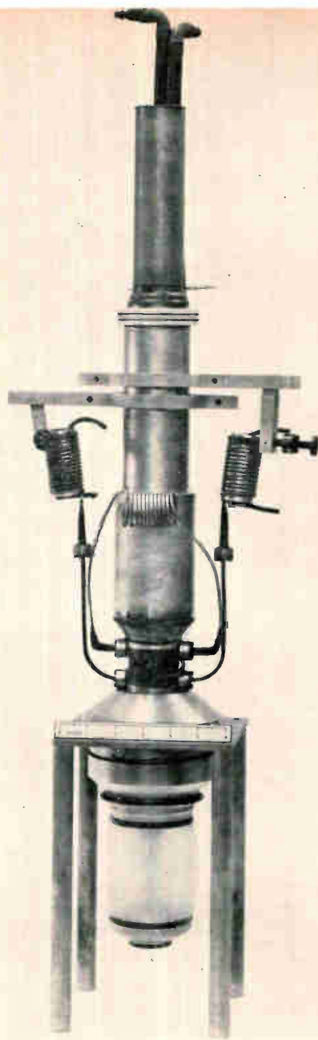
Backward-wave oscillator made by the Watkins-Johnson Co. is capable of 100 kw peak power at 100 Gc. Twin waveguides, shown at left and right of the tube, connect to coiled lossy waveguides of stainless steel, which act as loads.
