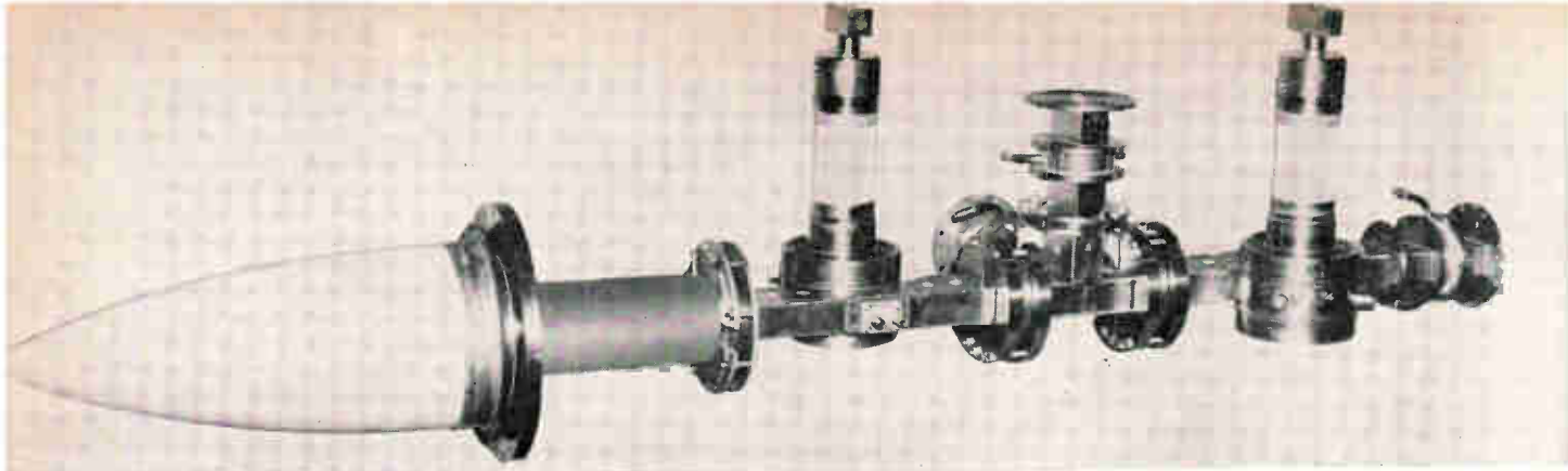
Raytheon Amplitron, shown without electromagnets attached, is about six feet long.
