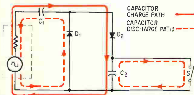
Basic staircase wave generator.
