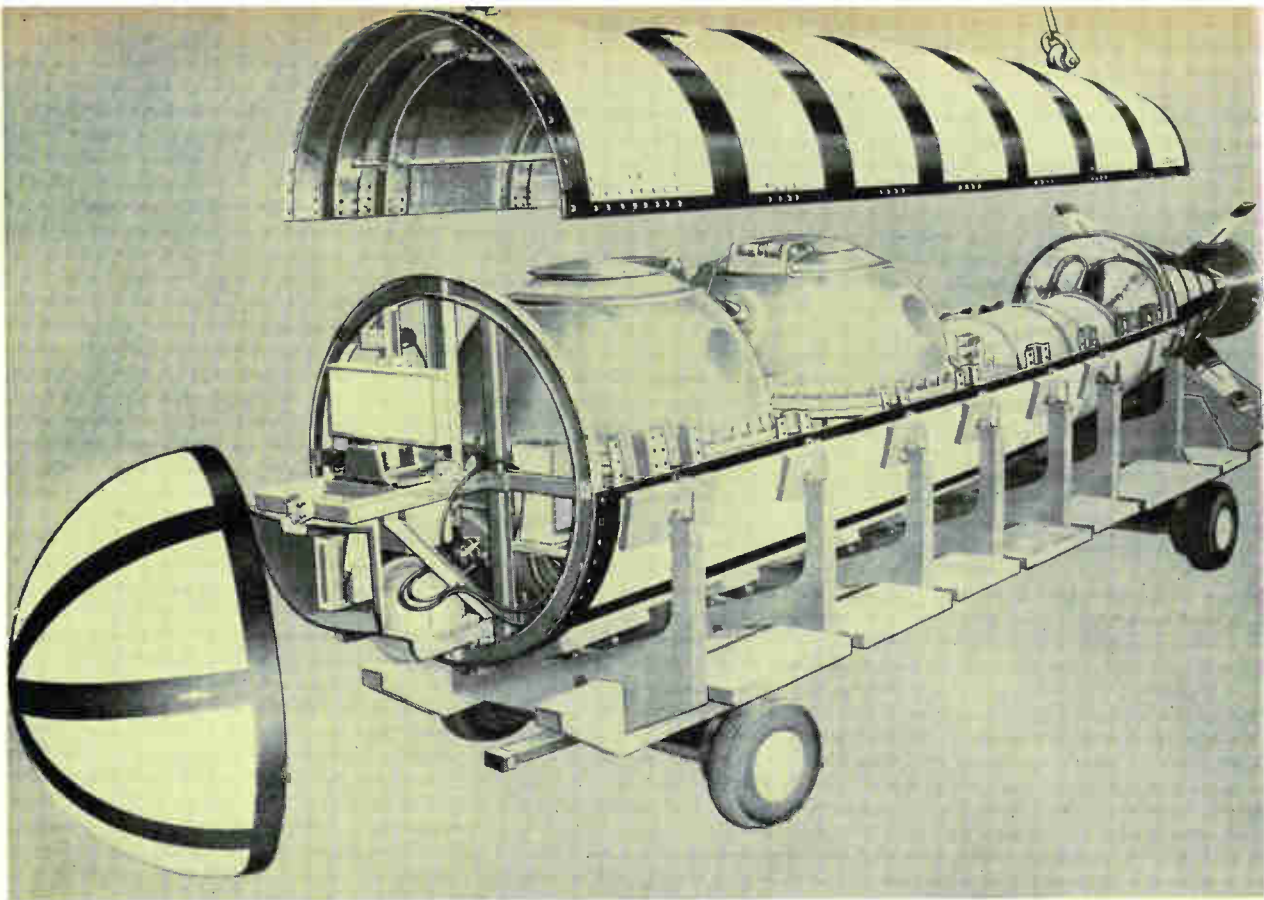
Two-man submarine Moray has separate pressure spheres for electronics equipment and for the crew.
