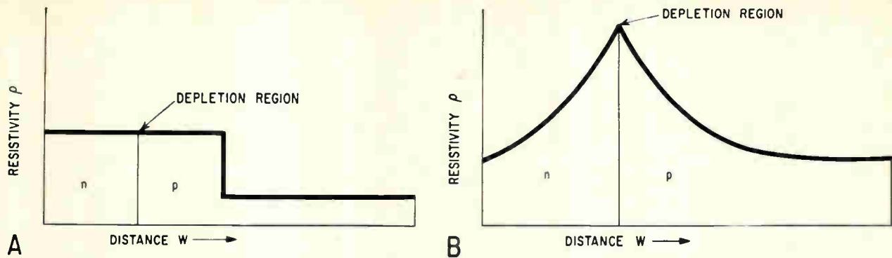
Typical resistivity profiles are for the abrupt, or step, junction (A) and for the linear-graded junction (B). Step junction has constant resistivities near the depletion region; linear-graded junction has an impurity concentration that decreases linearly as the depletion region is approached.
