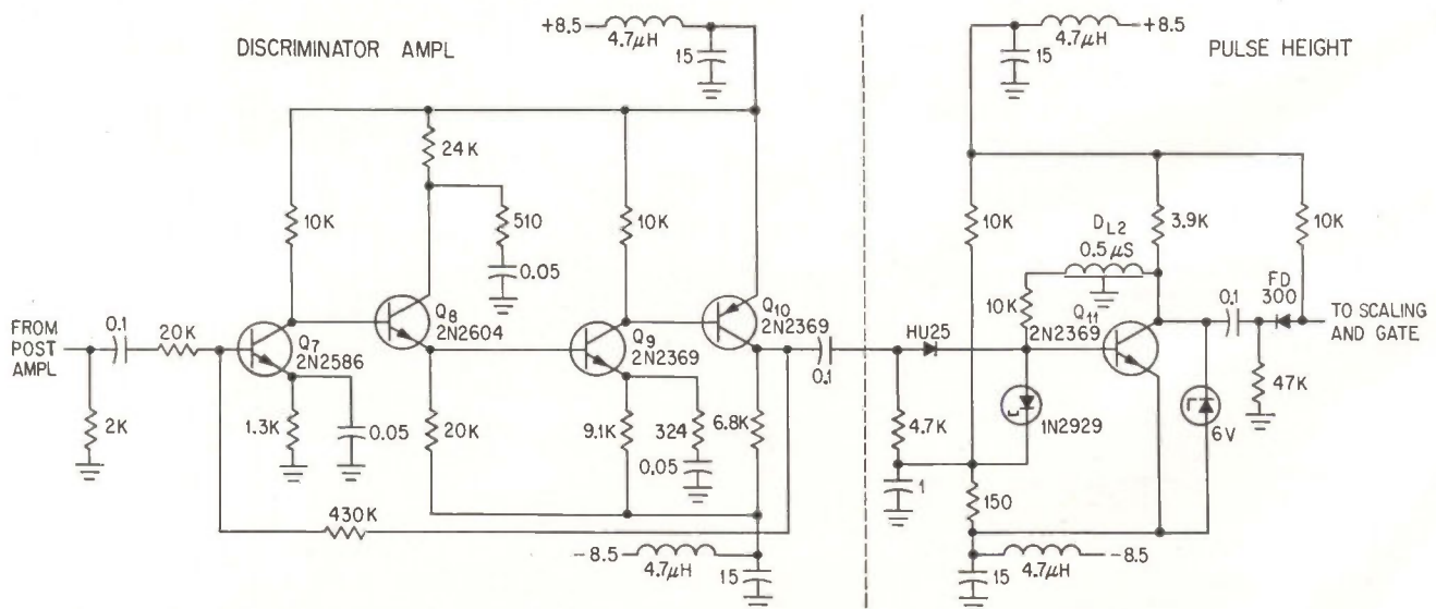
DISCRIMINATOR AMPLIFIER feeds pulse height circuit. Tunnel diode at input to pulse height circuit does not pass small pulses or low level noise—Fig. 4
