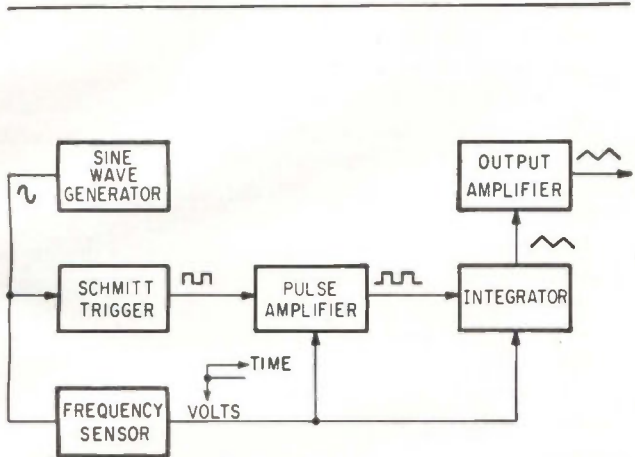
TRIANGULAR-WAVE generator uses a frequency sensing circuit to keep amplitude constant—Fig. 1
