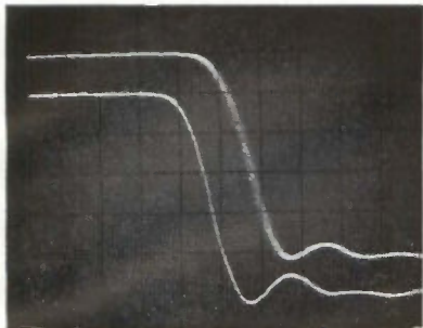
Upper trace shows step response with 100% sampling efficiency; lower with 20%. Rise times are 80 ps and 50 ps, respectively; sweep speed, 50 ps/cm.
