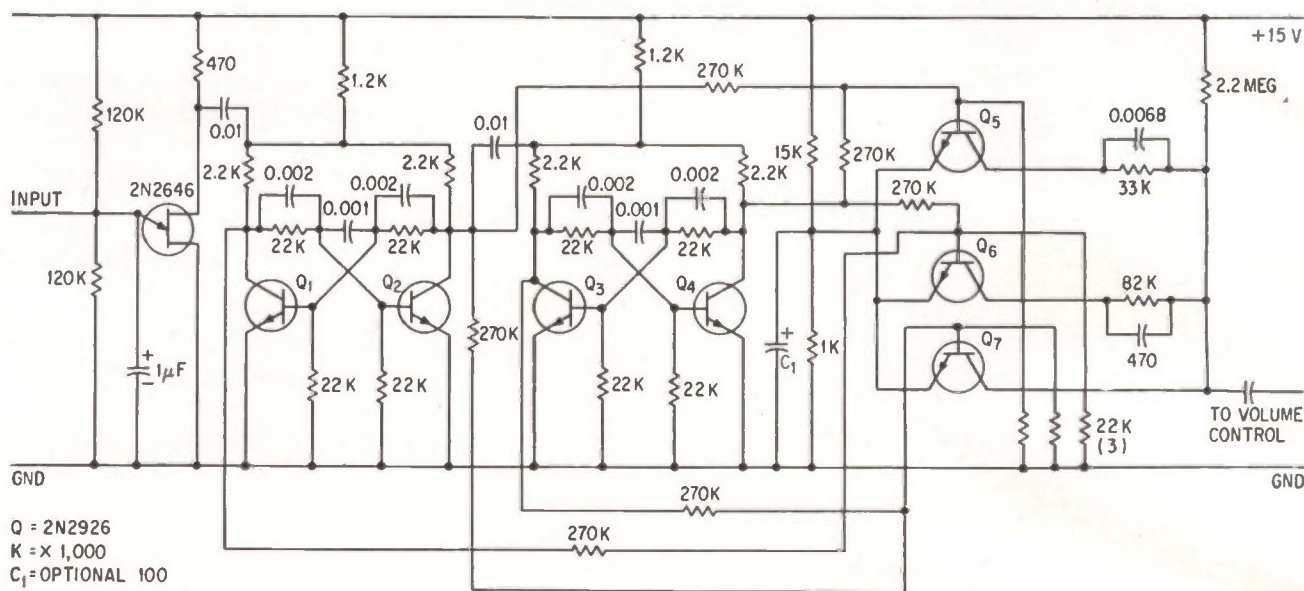
SOLID-STATE stepping switch performs all the functions of a conventional stepping relay using low-cost silicon transistors. The unijunction transistor threshold detector combines the two functions of level detection and trigger pulse generation
