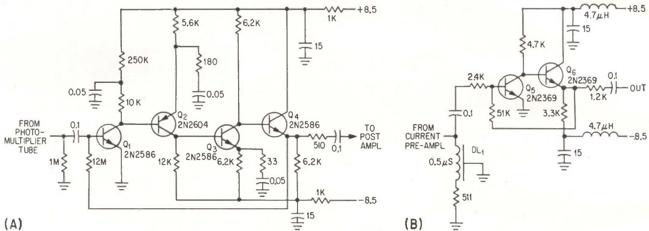
CURRENT PREAMPLIFIER (A) is a-c coupled from multiplier phototube and to following or post amplifier. Feedback holds gain change to \pm 5 percent over temperature range. Post amplifier (B) uses delay line for pulse shaping—Fig. 3
