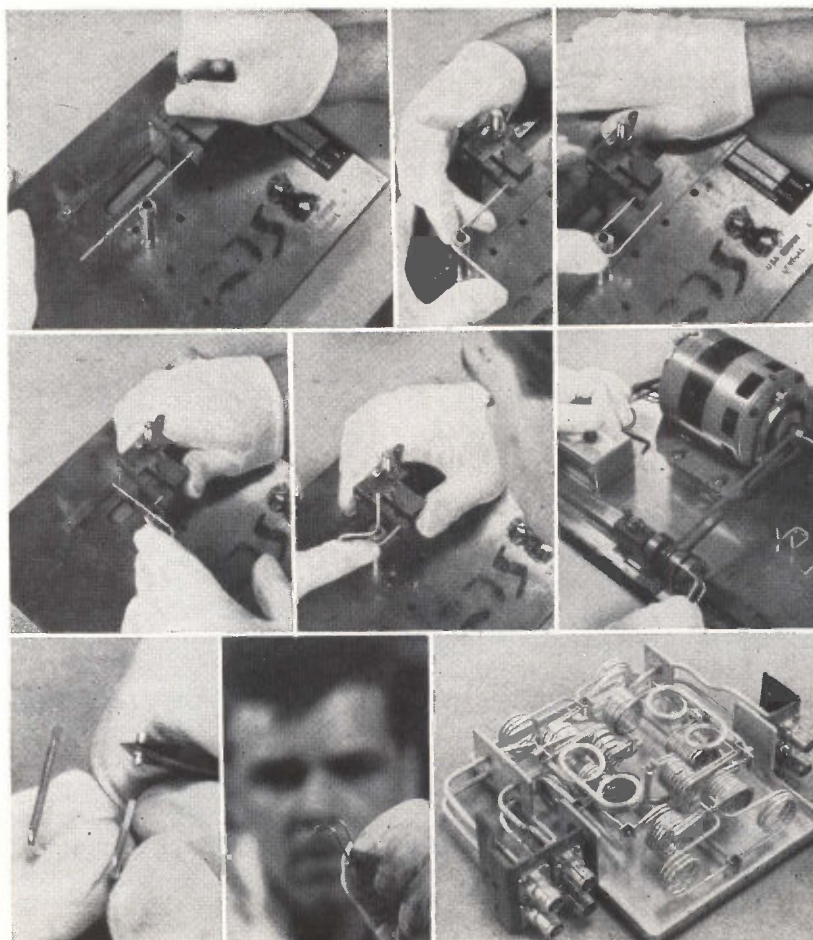
FORMING METHOD employed with adjustable fixture is shown by first five photos (see text for details). Shield is trimmed and removed. Parts are then assembled.
