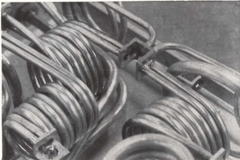
SHIELDS ARE SOLDERED to interconnect bracket, and inner conductors are soldered inside the bracket, in this phase comparator assembly
