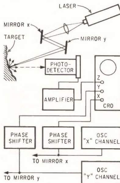
EXPERIMENTAL setup of laser camera system. (A) shows the path of the laser beam, (B) the receiver and display electronics
