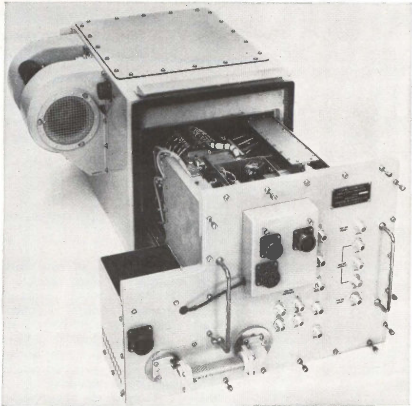
1,700-Mc feedbox equipment is shown above
