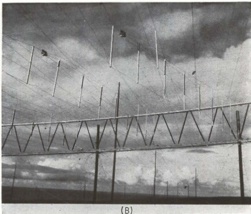
CONCENTRATION of wave energy by wire-grid lens shown in artist's drawing (A), and transmission-line coupler assembly installed in the lens (B)—Fig. 1
