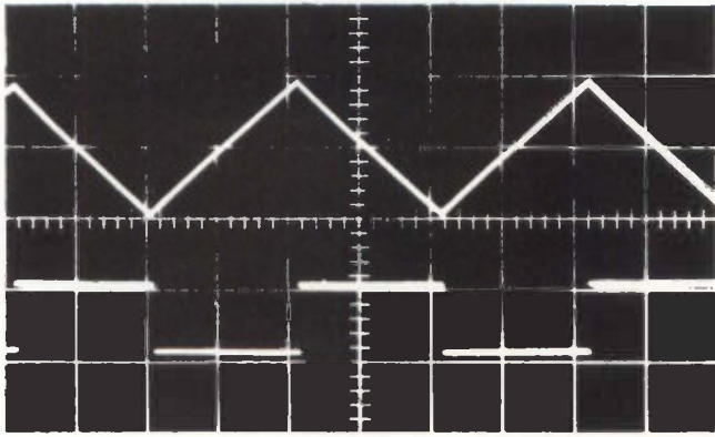
WAVEFORM is measured at the output of the amplifier for 500 cps. Scale is: vertical—5 v per cm and horizontal—500 \mu s per cm—Fig. 4
