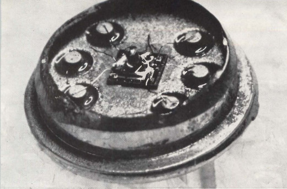
EXPERIMENTAL INTEGRATED sensing circuit constructed at Raytheon incorporates a piezo-junction accelerometer. Preliminary measurements indicate sensitivities of the order of 300 microvolts per g with a seismic mass of 0.1 gram. Work was described by W. Rindner, R. Wonson and G. Doering at the Solid-State Circuits Conference
