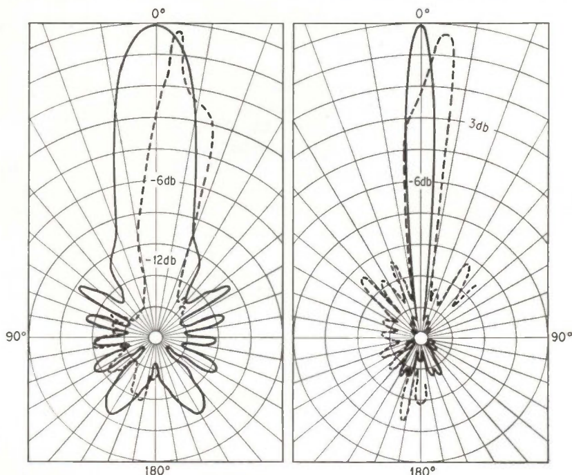
POLAR patterns showing calculated (solid) and measured (broken) plots of the array. Patterns were calculated for 4.0 Mc and 30 Mc, while measurements were taken at 3.8 Mc and 25 Mc—Fig. 2
