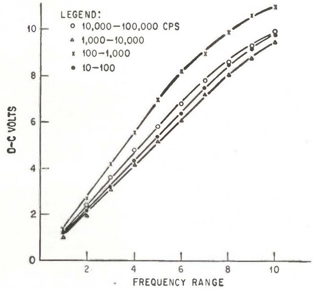
OUTPUT VOLTAGE of the frequency sensor is linear, except at the upper frequency range—Fig. 3
