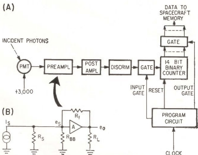
SPECIAL MULTIPLIER phototube (block diagram) can respond to single photon. To match multiplier phototube's high output impedance, preamplifier (B) is designed as current amplifier—Fig. 1
