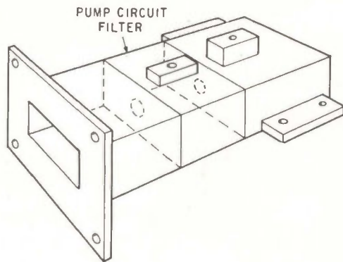
PUMP circuit with isolation filter (left) was necessary to provide isolation within the designed package. Signal circuit with idler rejection filter is shown at right
