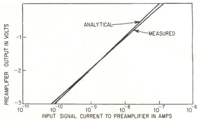
MEASURED and calculated transfer functions of preamplifier agree closely—Fig. 2
