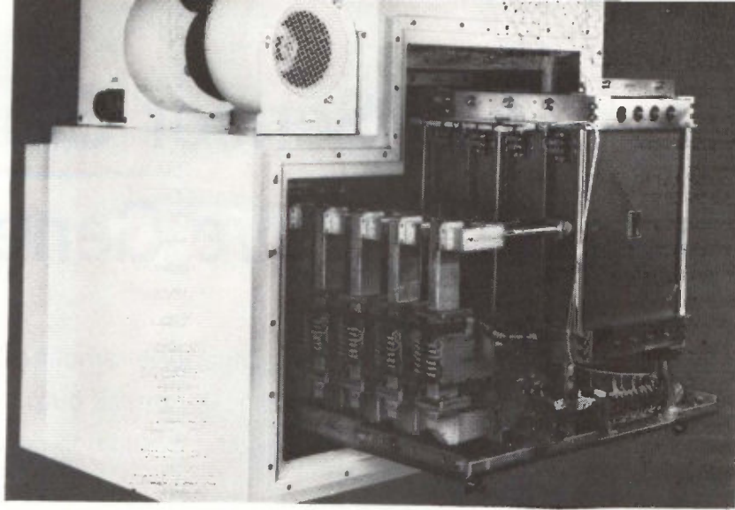
FEEDBOX equipment for operation at 400 Mc
