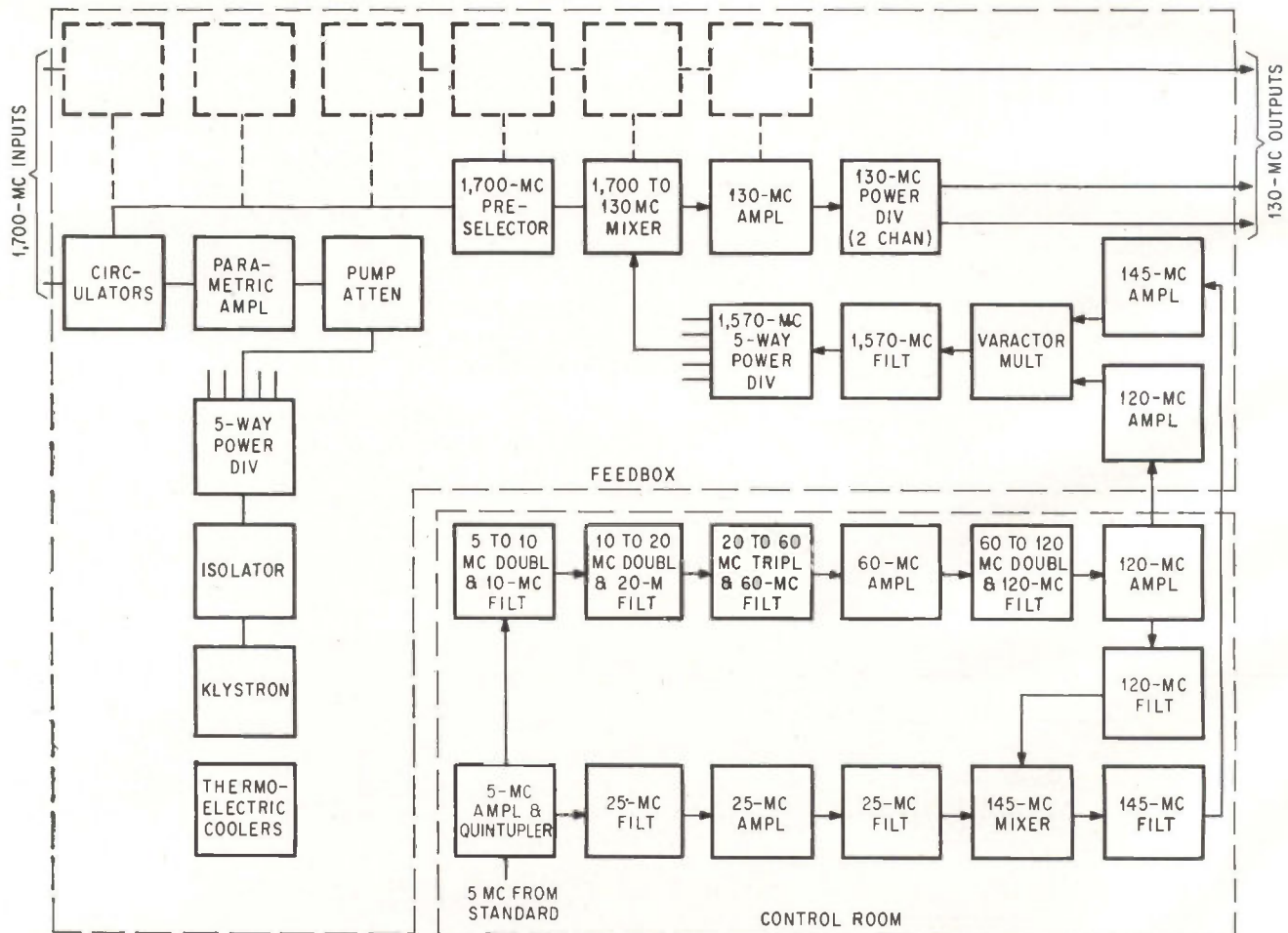
PARAMETRIC amplifier converter system for 1,700 Mc. The comparable system for 400 Mc is simpler as described in text
