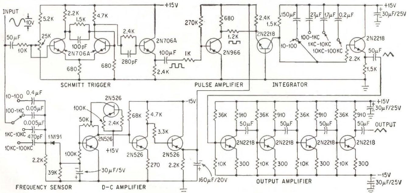
CIRCUIT of the triangular-wave generator uses 14 transistors—Fig. 2
