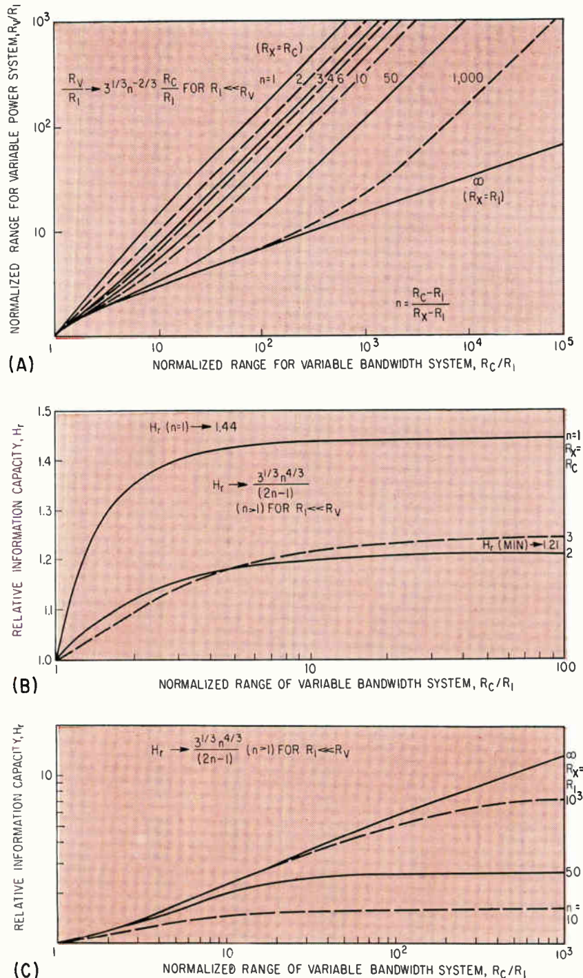
RANGE COMPARISON between variable-power and variable-bandwidth systems for equal total energy consumption (A); relative information capacity gain of variable-power system over variable-bandwidth system for equal energy consumption and n small (B) and n large (C)—Fig. 3
