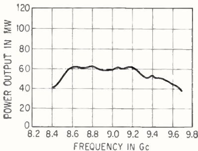
POWER OUTPUT versus frequency curve for a V-180B bwo—Fig. 2
