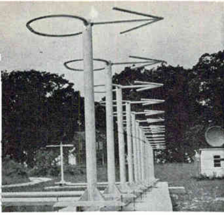
DIRECTIONAL ARRAY being tested by FAA could be used for low-cost ILS and may also improve all-weather landing systems
