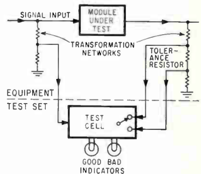
NETWORKS in equipment allow Fist test cell to test any equipment module
