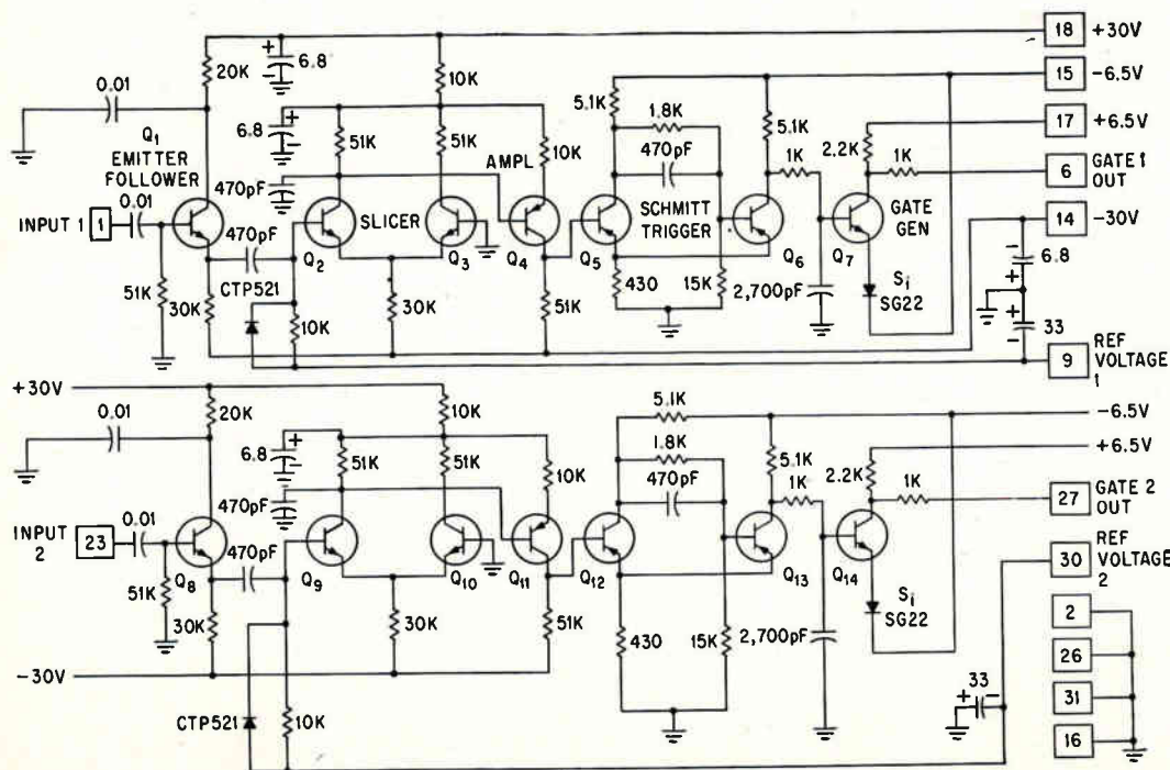
SLICERS are contained in two stages. Reference voltage will determine slicing level—Fig. 2
