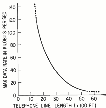
MAXIMUM DATA RATE versus telephone line length—Fig. 2
