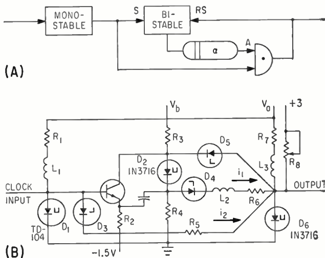
SIMPLICITY of concept is apparent in block representation (A) as well as in detailed circuit diagram (B)—Fig. 1
