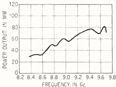
POWER OUTPUT versus frequency curve for a V-180A bwo—Fig. 1
