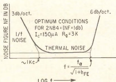
TRANSISTOR noise has two break points—Fig. 4
