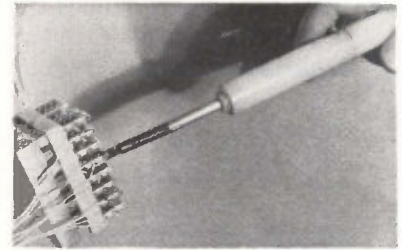
NON-DESTRUCTIVE residual-force test tool includes indicator in handle that registers tensile value of pull on connection
