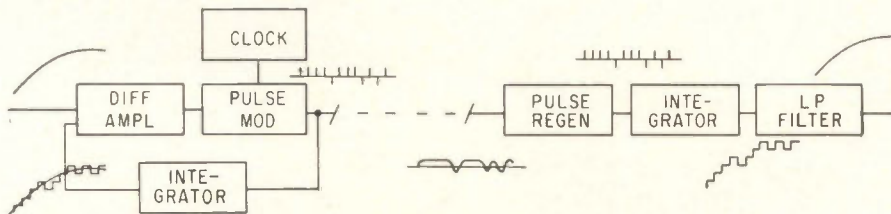
DELTA modulator uses feedback, quantized in amplitude and time, to obtain a faithful replica of the transmitted signal—Fig. 1
