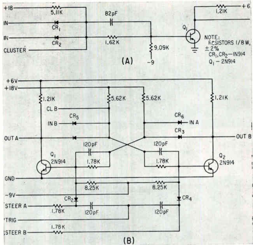
STANDARD GATE circuit is the most frequently used micromodule in the computer (A); shift register operates at a 1.6-Mc clock rate (B)—Fig. 3
