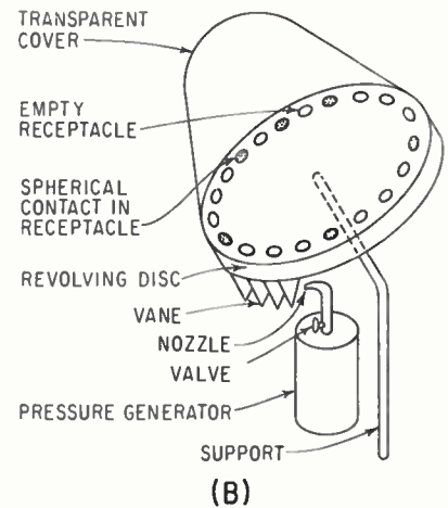
PINBALL PRINCIPLE of circuit interconnection, (A), is implemented by steel balls held in receptacles by individual magnetic fields, (B)—Fig. 2
