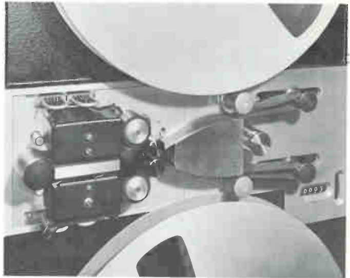
Close-up of PI-400 tape guiding mechanism. The tape chute reduces transverse vibration and positions the edges of the tape accurately to minimize skew. The bilateral symmetry permits the tape to be transported in either direction with equal control.
