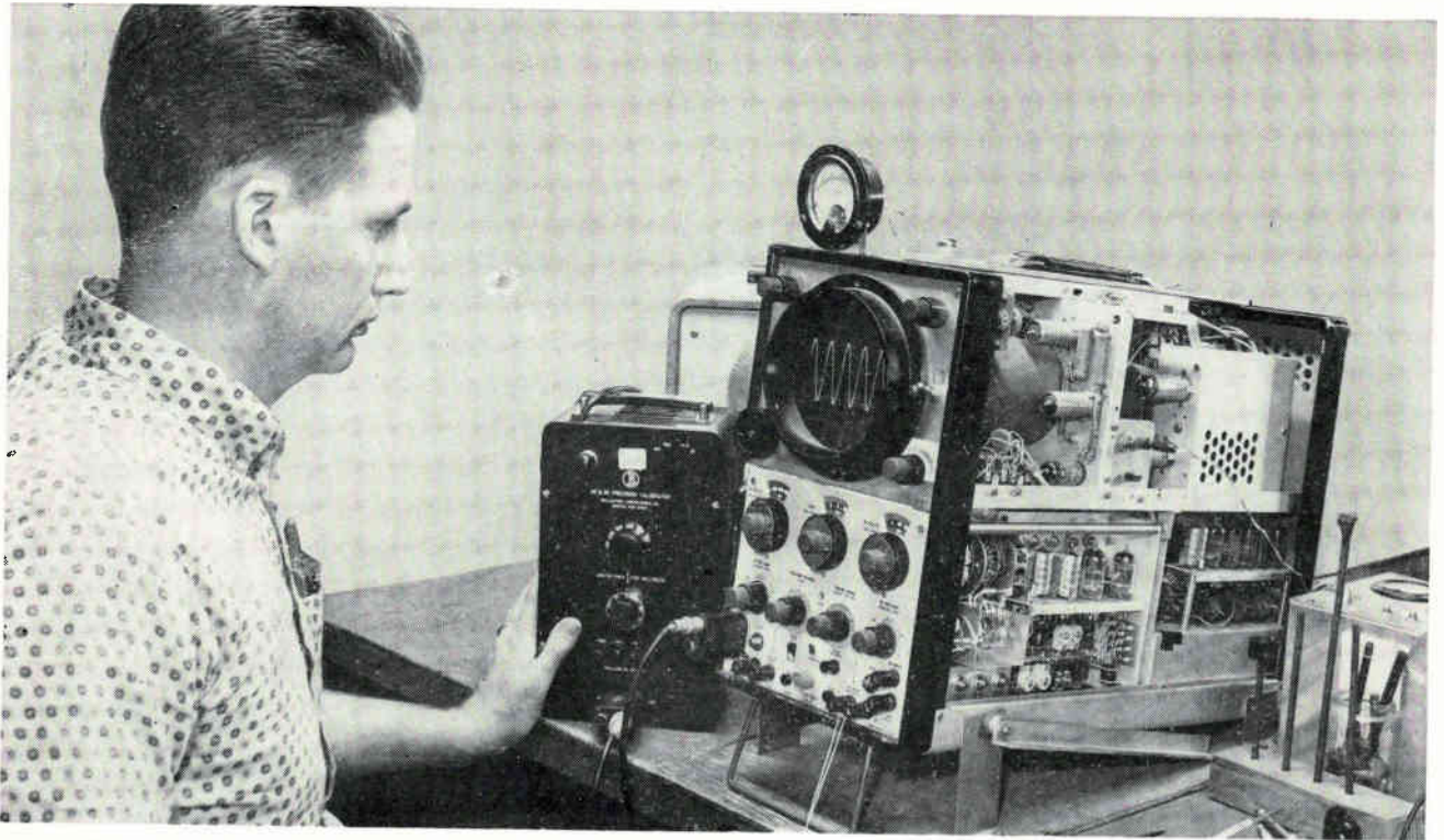
PRECISION D-C and A-C VOLTAGES are generated by Ballantine Laboratories calibrator (left) shown providing stable reference standard in oscilloscope calibration. Standards instruments and devices represent a maturing market
