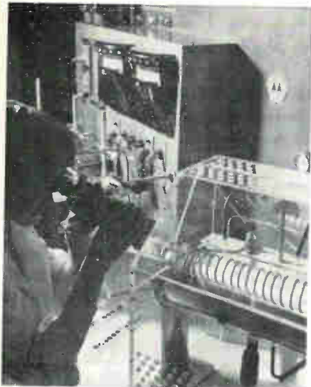
SILICON WAFERS are checked with optical pyrometer for exact temperature during growth of epitaxial layers, Motorola
