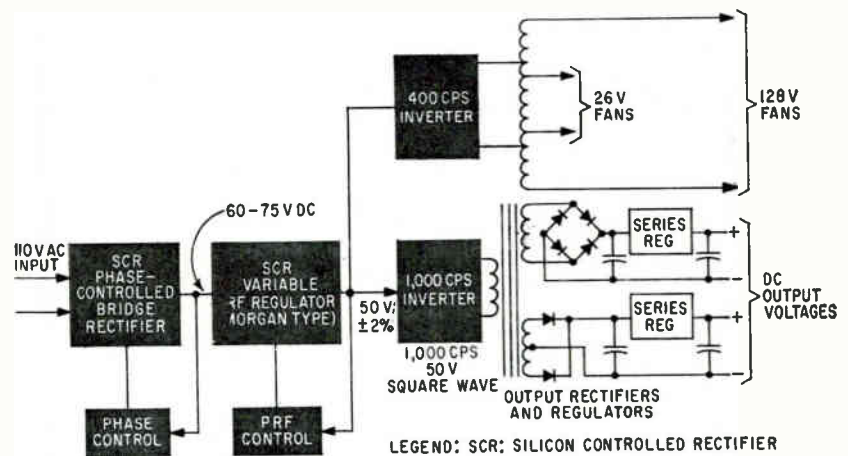
POWER SUPPLY for the computer uses several modern techniques to achieve high regulation from a widely varying power source—Fig. 4
