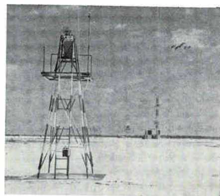
TRANSMISSOMETER receiver (foreground) measures strength of light from transmissometer transmitter (background) to determine visibility
