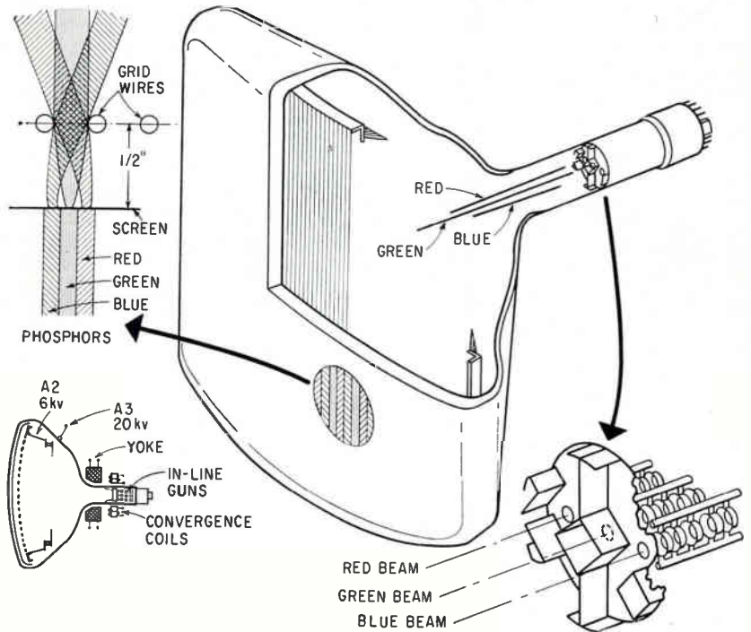
COLOR TUBE uses three electron guns, lower right, that focus on vertical array of color phosphors. Intense color image is produced after beams pass through relatively transparent second anode grid in front of phosphor array. Second anode is array of vertical grid wires
