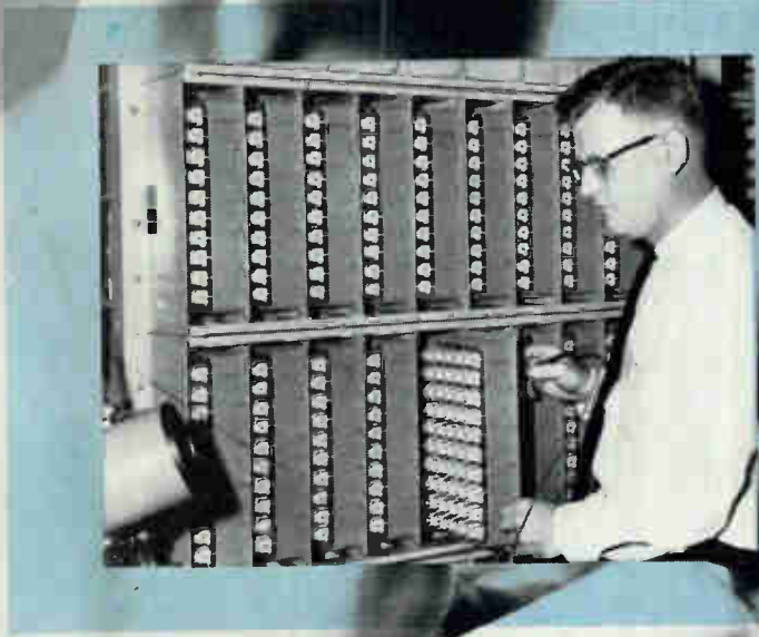
ELECTRONIC TELEPHONE EXCHANGE (inset), developed by Automatic Electric Co., a subsidiary of GT&E, is compatible with electro-mechanical switching equipment. Magnetic switches in hermetically sealed capsules (above) are used in switching matrix
