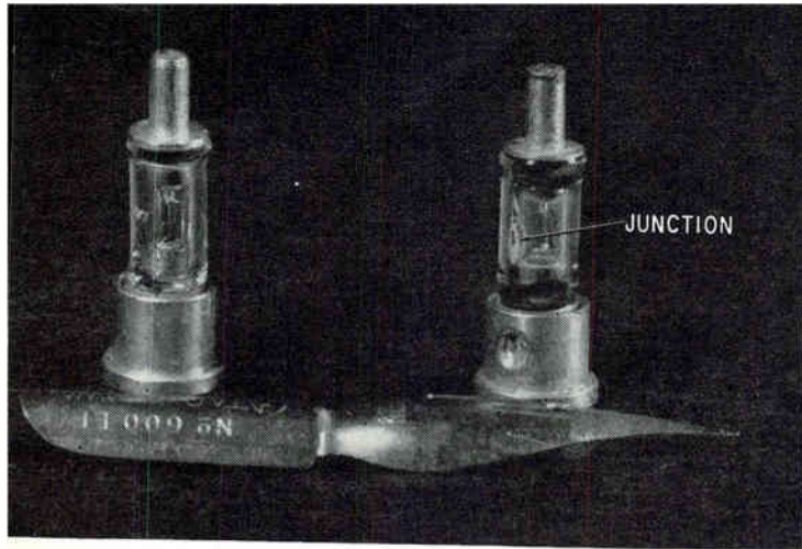
PARAMETRIC DIODES. Two kinds of silver-bonded, point-contact diodes (Ge and Si) have been tested. Shown here are Ge diodes, type GSB1B—Fig. 1
