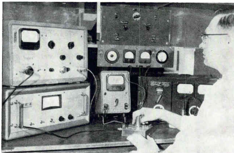
NOISE FIGURE of r-f amplifier in test jig (center) is measured using a meter that continually monitors noise figure and gives a direct noise-figure readout in db.
