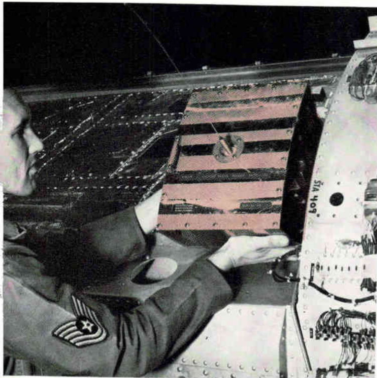
AMATEUR RADIO BEACON installed in Discoverer satellite provided ham radio operators with a chance to study propagation phenomena. The amateur constructed, 144 Mc package was launched into orbit from Vandenberg Air Force Base
