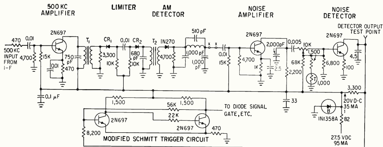
EVALUATION circuit diagram of the carrier-to-noise squelch system; modified Schmitt is triggered by output of noise detector—Fig. 2
