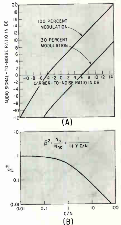
SIGNAL-TO-NOISE ratio at output of linear a-m detector plotted against carrier-to-noise ratio for 40-Kc i-f bandwidth, and 4-Kc audio bandwidth (A); ideal band-pass limiter noise-suppression characteristic (B)—Fig. 1
