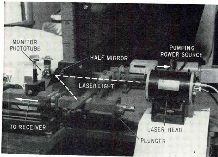
DOTTED WHITE LINE shows path of laser beam in experimental setup—Fig. 2
