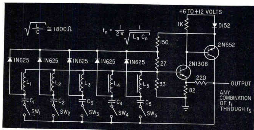
DIFFERENT PERMUTATIONS of one through five tones are generated by this circuit, enabling it to operate as a five-bit parallel encoder for industrial telemetry—Fig. 1
