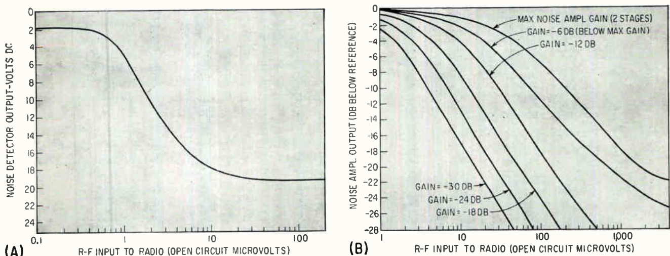
(A) NOISE DETECTOR d-c output plotted against r-f input of the test receiver (A) and noise-quieting characteristics of various noise amplifier gains (B)—Fig. 3
