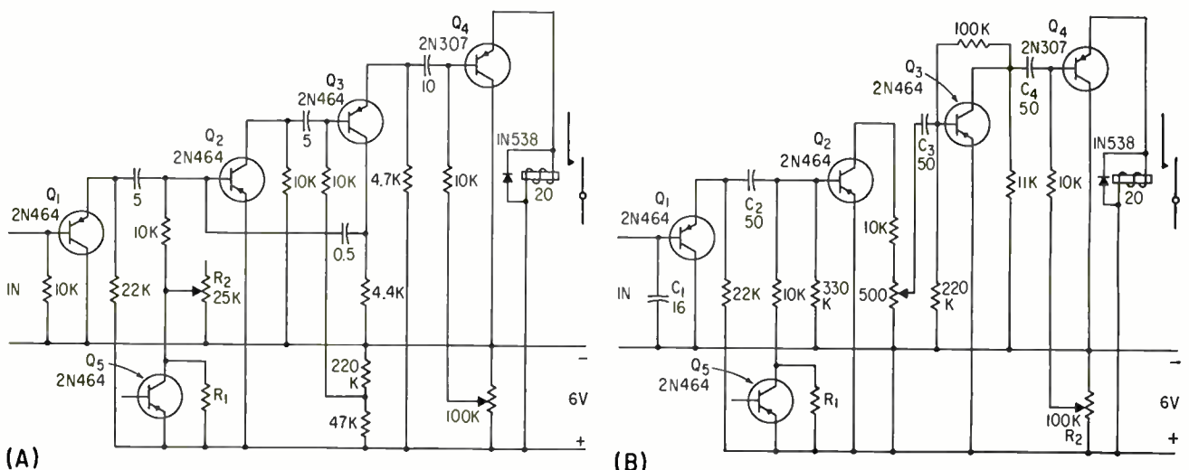
Circuits for the two types of amplifiers used in road-rail truck
