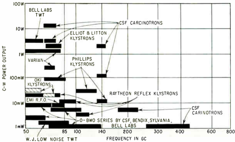
FIG. 1—Power levels for tubes either pulsed or operated c-w above 50 Gc
