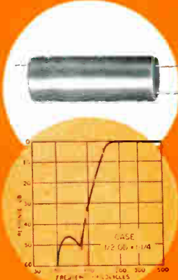
High frequency Mini-filters, .33 oz. MIL-T-27A Grade 3. 150 KC High Pass 3 db to 150 KC, down 45 db below 35 KC. 7500 ohms.
