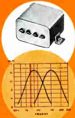
Curves of our miniaturized 90 and 150 cycle filters for glide path systems. 1\frac{1}{4}'' \times 1\frac{3}{8}'' .
