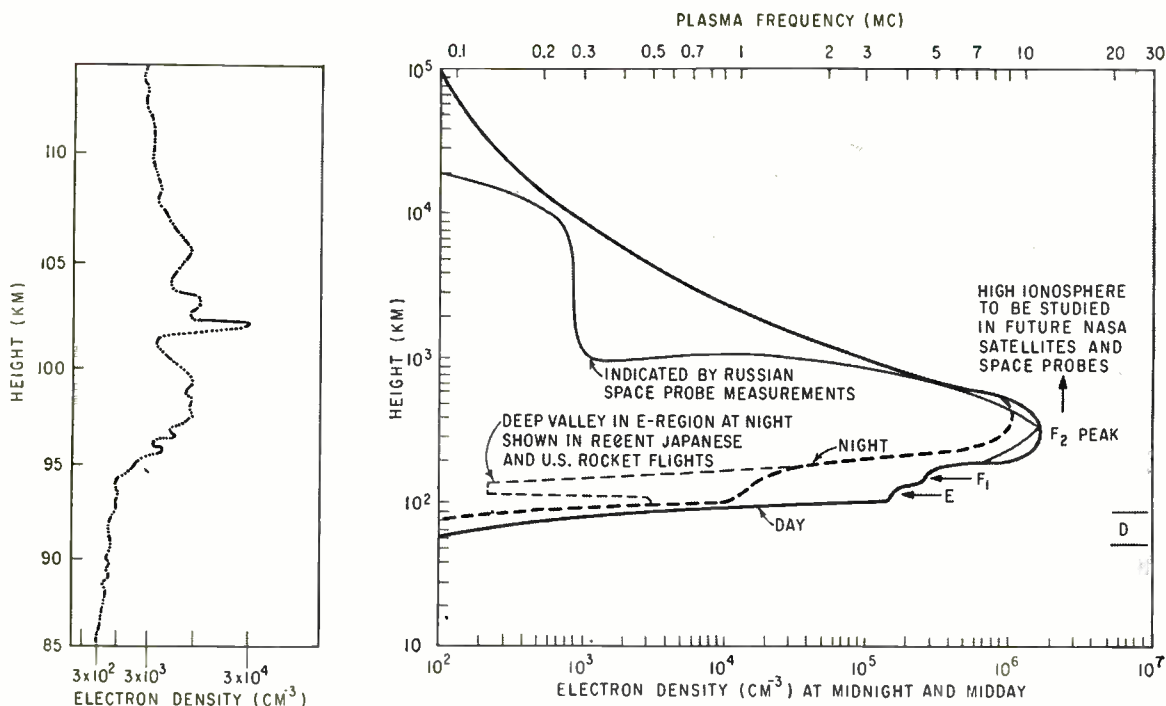
Electron density profile on ascent last Aug. 17; dots are extrapolations (left). Recent data shows changes (light lines, right) in ionospheric profile. Until a year ago, reliable measurements were made only at heights of 90 to 400 Km by day and 200 to 400 Km at night
