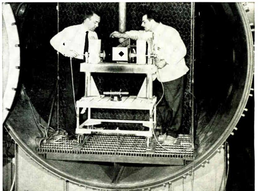
THE FRONT COVER. Final adjustments are made to microwave interferometer before projectile is fired from light-gas gun behind tank, passes where engineer holds suspended ball and impacts inside heavy door at left. Interaction of electromagnetic waves with ionized air in projectile wake may help solve re-entry communications blackout problem.
