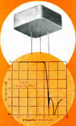
Miniaturized 3.5 KC low pass filter. 10K ohms to .0K ohms. Within 1 db up to 3500 cycles. Greater than 40 db beyond 4800 cycles.
