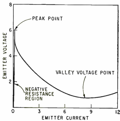
FIG. 1—Equivalent circuit (A) and characteristic curve (B) are shown for unijunction transistor
