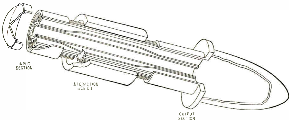
FIG. 14—Quasi-optical coupling would be used in a proposed electromagnetic amplifying lens
