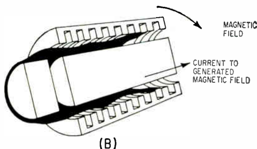
FIG. 12—Linear M-type backward wave oscillator (A) and cylindrical version using the same approach (B), where magnetic field is generated by a current in the sole
