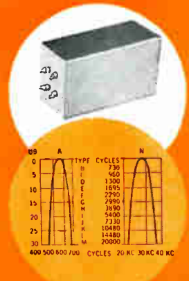
Multi-channel telemetering band pass filters for 400 cycle to 40 KC. Miniaturized units for many applications.
