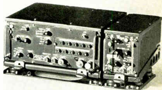
Avco's AN/VRC-12 mobile radio for combat communications
