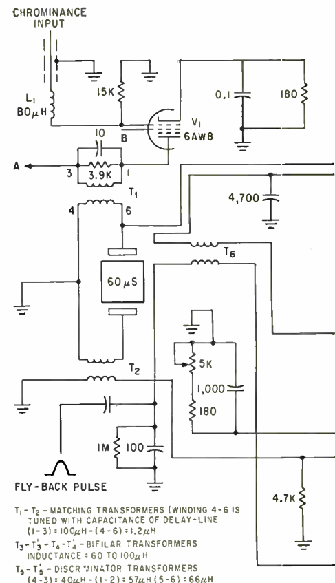
FIG. 3—Chrominance-signal identification
