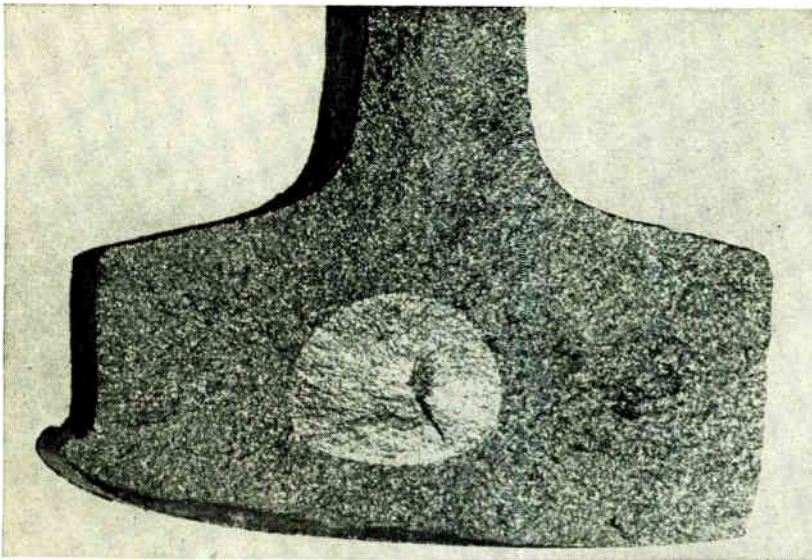
One of the rail defects detected with the pulse amplifiers
