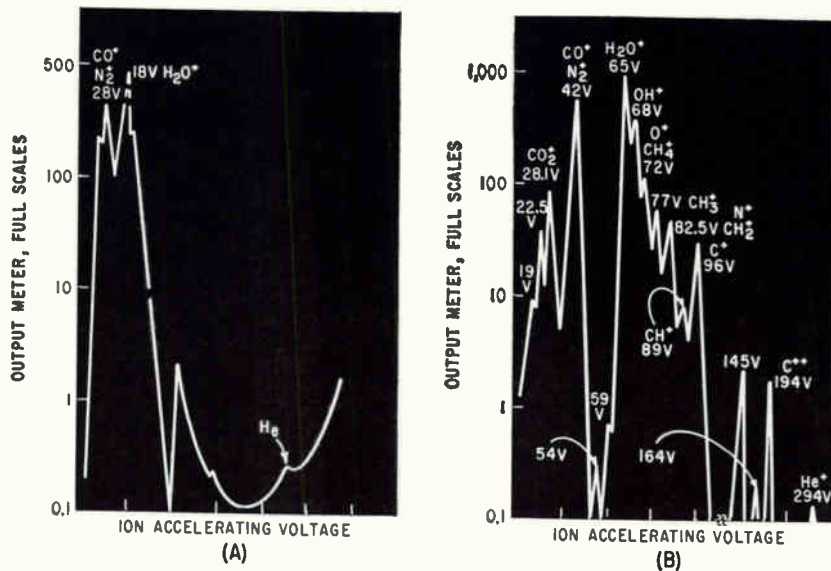
FIG. 4—Resolution obtained by single-stage spectrometer (A) is surpassed by resolution of twin-stage spectrometer (B)
