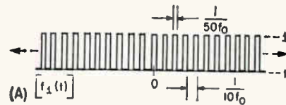
(A) [f_1(t)]
