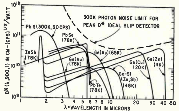
FIG. 1—Spectral responses of nine commercially-available photoconductors are compared with that of ideal background-limited infrared photoconductor
