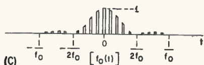
FIG. 3—Radar return from search-lighted target (A); dynamic antenna pattern (B); and return from scanned target for which spectrum is desired (C)
