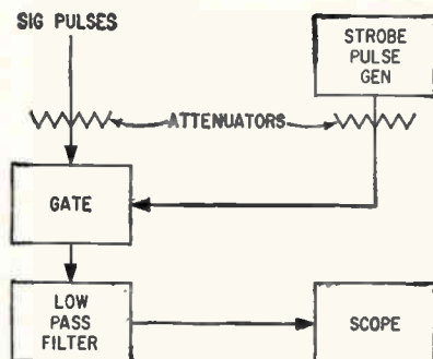
FIG. 1—Basic strobe circuit passes signal amplitudes only when a strobe pulse is applied to gate
