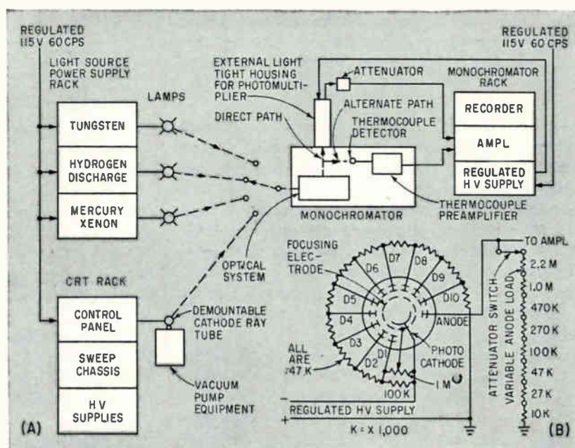
FIG. 1—Fast-acting thermocouple, with a response nearly independent of wavelength, serves as a calibrating standard for amplitude measurements (A). The adjustment between photocathode and the first dynode allows optimum phototube operation (B)
