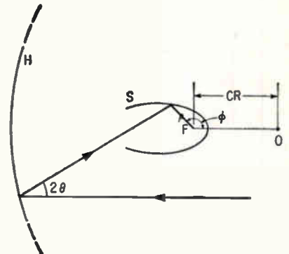
FIG. 1—Parallel incident beam reflected by hemisphere (H) to second reflector (S) comes to point focus (F). Center of hemisphere is (O)
