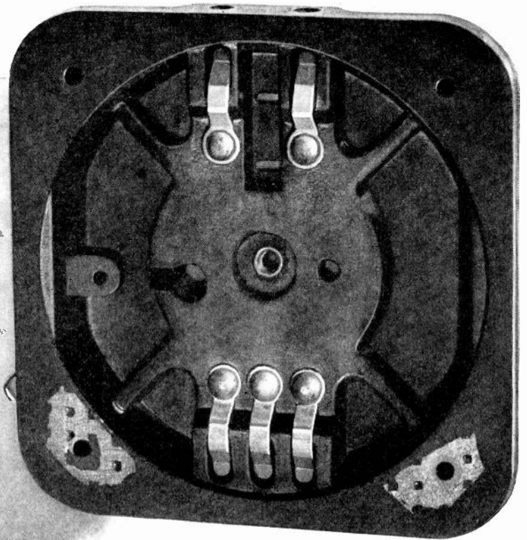
Hardened Metallic Drive Screws overcame difficulties of fastening contacts to this thin molded Bakelite microphone part shown enlarged.
