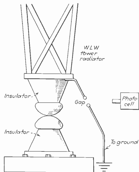
When a flashover takes place across the gap, the photo-cell opens the power cut-off relays
