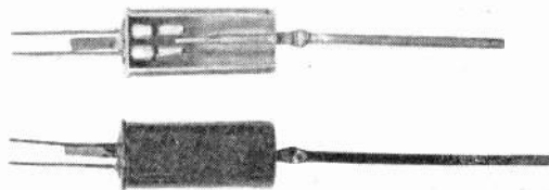
Fig. 5—Vacuum switch. Metal envelope allows mechanical movement of contacts
