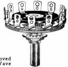
Improved Model "34" Wave Band Switch—has proven its dependability and long life.
