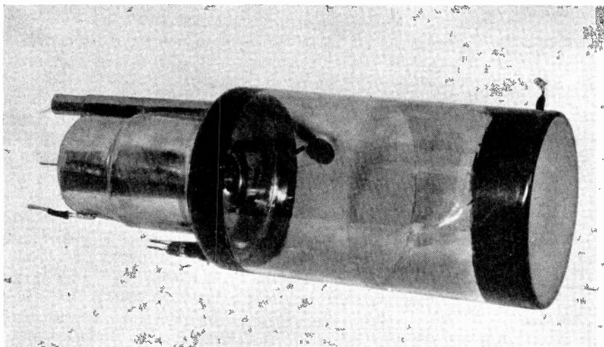
One form of the Farnsworth image dissector. This cathode-ray scanner is capable of televising outdoor scenes by virtue of the electron multiplier (shown at left of tube) which amplifies its output 1000 times
