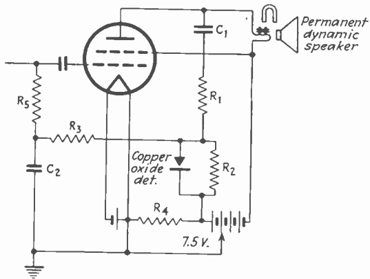
Fig. 1—Circuit of Folks-empfänger receiver. Note copper-oxide rectifier
