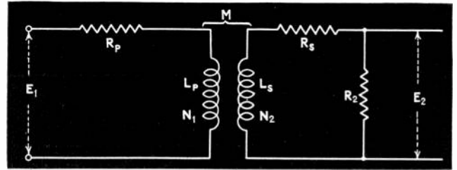
Fig. 1—Reference circuit for calculating inductance of output transformer (equation 7)
