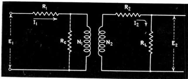
Fig. 2—Reference circuit for estimating core loss, current, and voltage in power transformers
