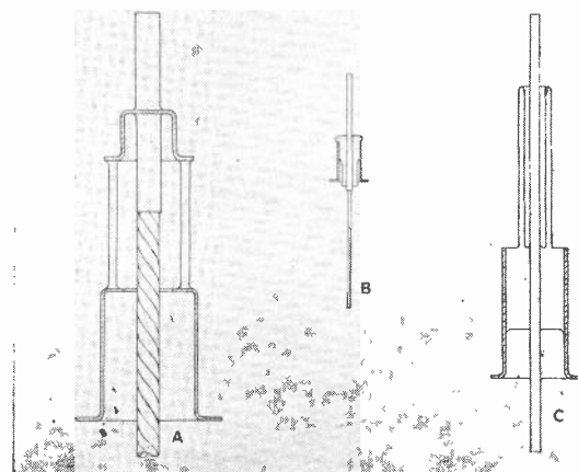
Fig. 1—Cross section of pillar and concentric seals
