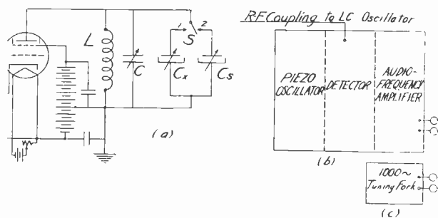
Fig. 1—Diagram showing essential parts used in calibrating condensers
