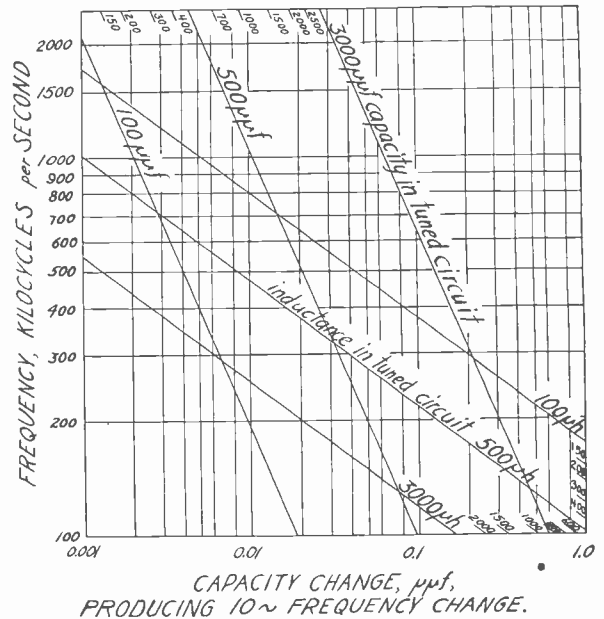
Fig. 3—Chart showing precision obtainable by method described if frequency adjustment is in error by ten cycles per second
