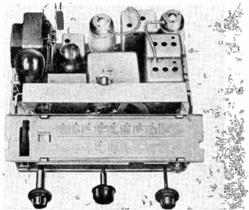
Fig. 3—Chassis of modern 3-tube reflex superheterodyne (A.E.G.)
