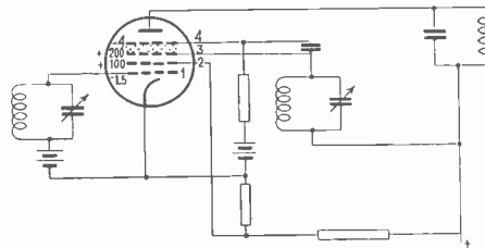
Mixing hexode circuit diagram
