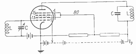
Connections for what the Germans call a "fading" hexode
