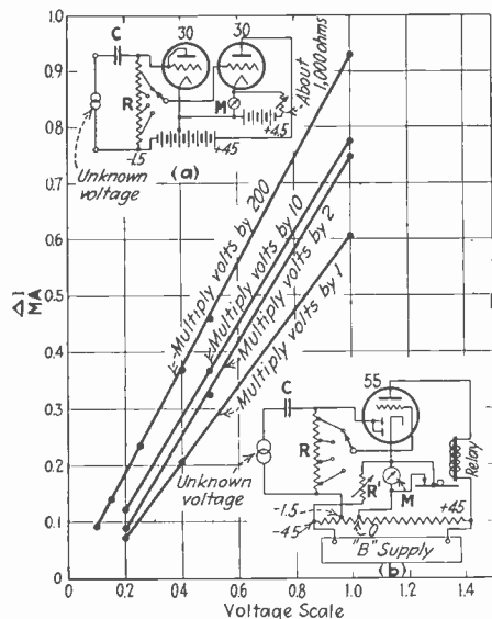
Fig. 1—Circuits and calibration of peak voltmeter
