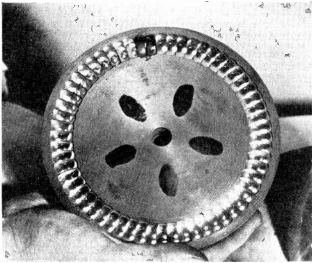
A disc of cast-glass lenses, silvered on the back, reflects the light from the Kerr cell to the viewing screen
