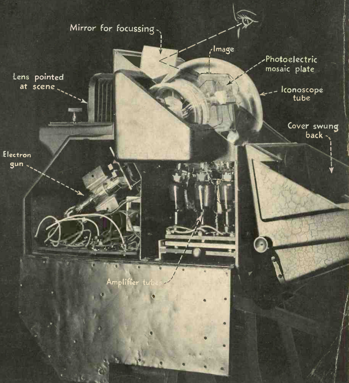
TELEVISION CAMERA
