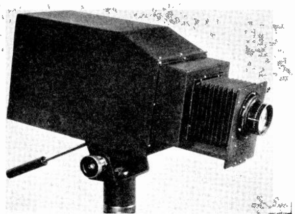
The Farnsworth camera, containing the "image dissector"
