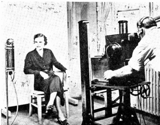
Studio technique, as practiced by engineers of the Philco radio and Television Corporation. The operator has constant visual and aural check on the proceedings
