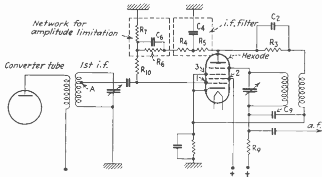
Fig. 4—Three-tube reflex super with amplitude limitation circuit
