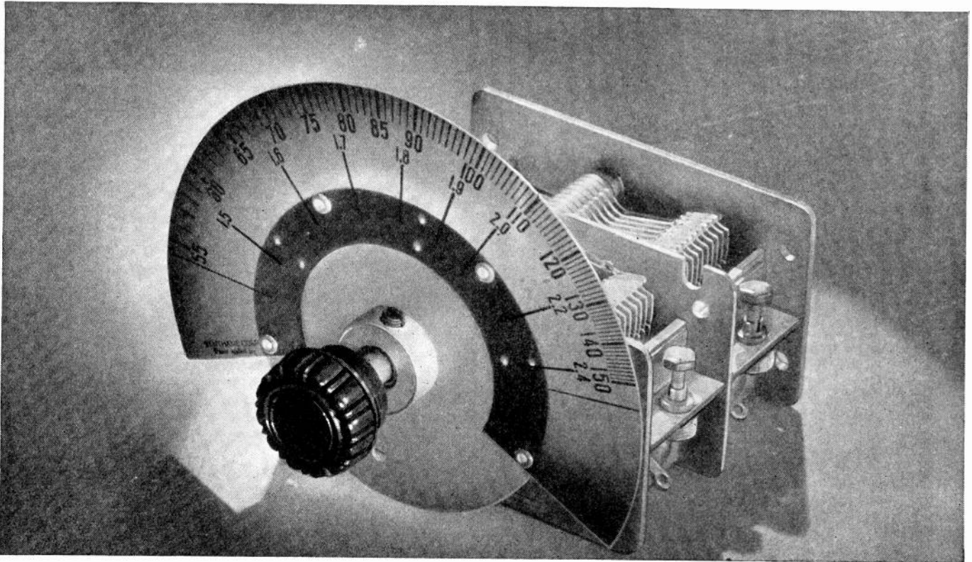
(Above) Philco Condenser with dial of translucent Bakelite Laminated, made by Synthane Corp., Oaks, Va.
