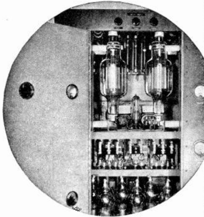
Typical mounting of two Western Electric 279A tubes in a radio telephone transmitter.
