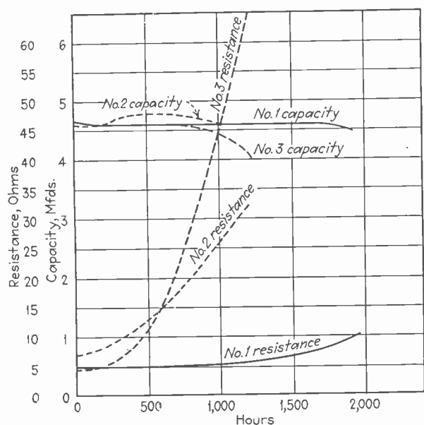
Dependence of condenser life on proper electrolyte
