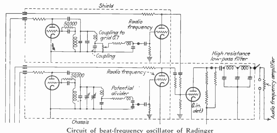
Circuit of beat-frequency oscillator of Radinger
