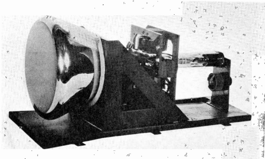
Cathode-ray scanning tube of Zworykin. The scene, focussed upon a mosaic of photocells, charges thousands of condensers whose discharge currents, produced by the cathode-ray beam, are transmitted to the receiver where the scene is re-created
