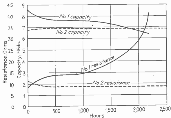
Effect of increasing by 20 per cent plate formation and electrolyte cost (450 volt units)
