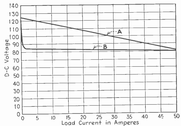
Fig. 2—Regulation curves of a two-element rectifier compared to that of a grid-controlled rectifier
