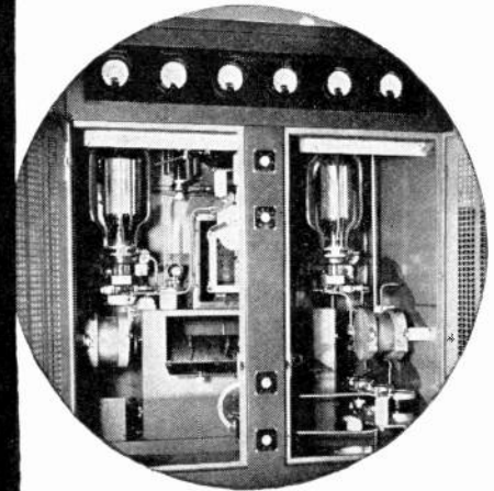
Two Western Electric 279A tubes mounted in the Western Electric 305A transmitter used by the police of the City of New York.
