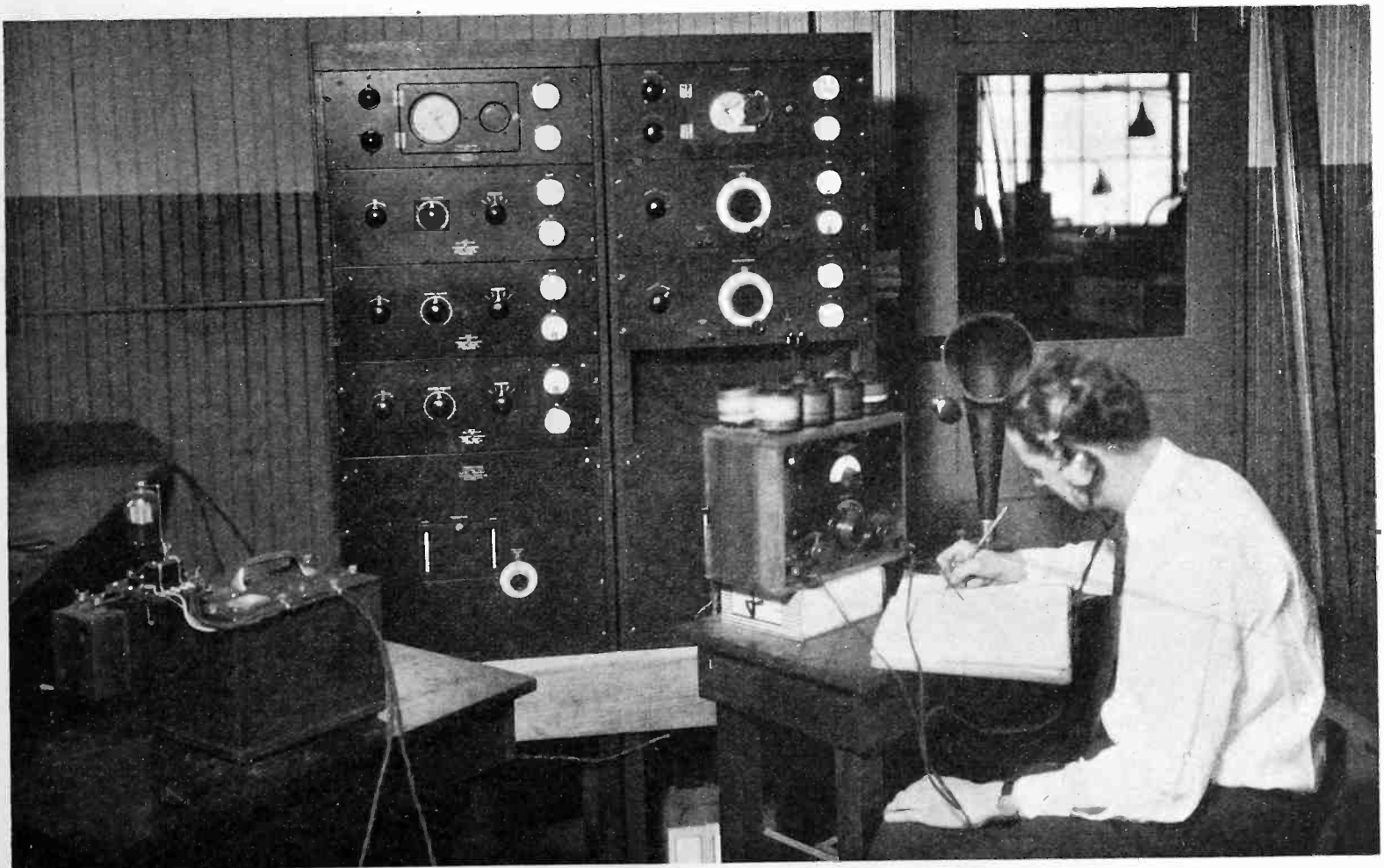
The standard-frequency assembly in use. A heretodyne wavemeter at the left is being calibrated by means of harmonics generated by the apparatus on the panel. The operator is listening in another circuit in which the beats between the two oscillators are reproduced.
