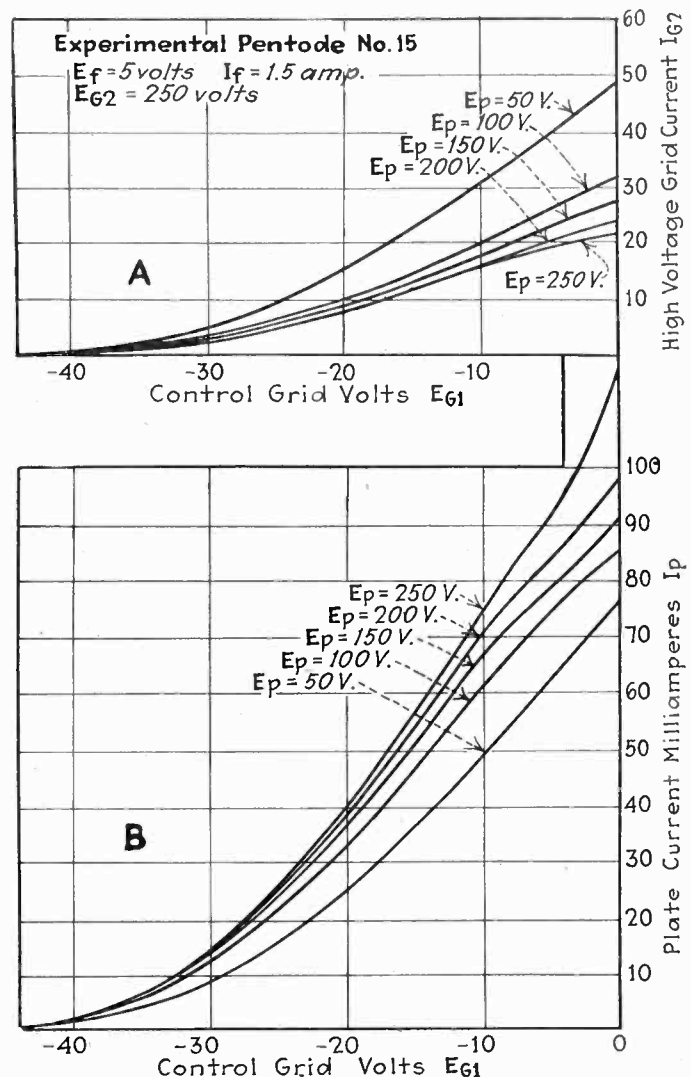
Fig. 2—Static characteristics of power pentode
