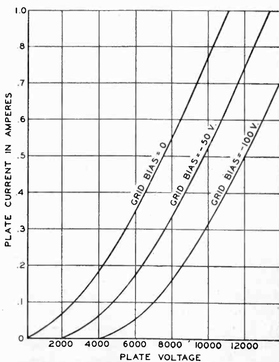
Plate-voltage-to-plate-current characteristics of Western Electric 240-A tube
