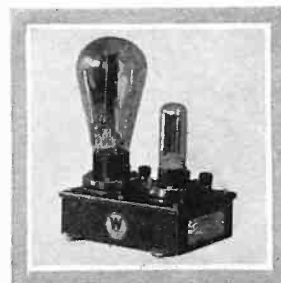
Photo-Electric Cell Amplifier Unit, a simple, low-cost device particularly adapted for experimental work in connection with industrial photoelectric problems
