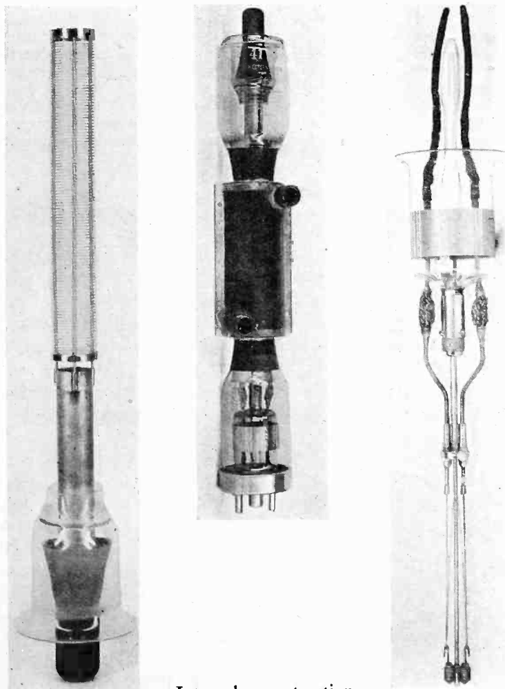
Internal construction and outward appearance of double-ended power tube for Atlantic radio-telephone service
