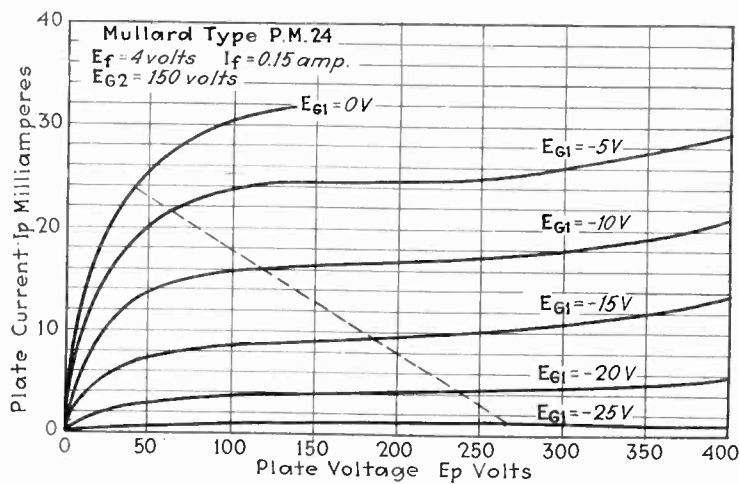
Fig. 4—Static characteristics of a well-known English pentode
