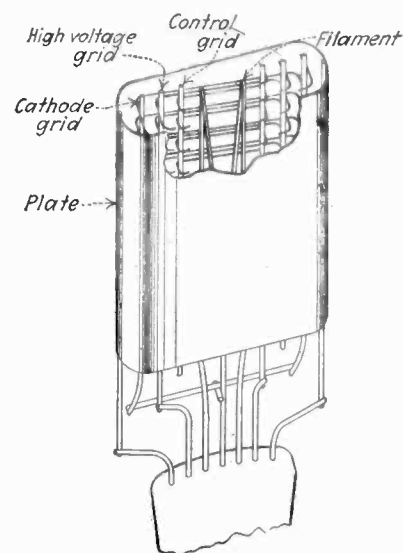
Fig. 1—Internal construction of power pentode
