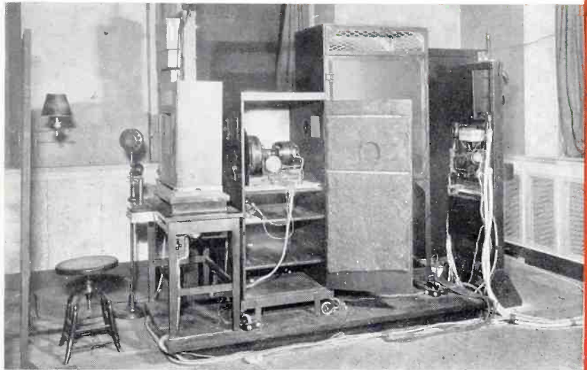
Above —Television Transmitting Apparatus Courtesy Bell Telephone Laboratories
