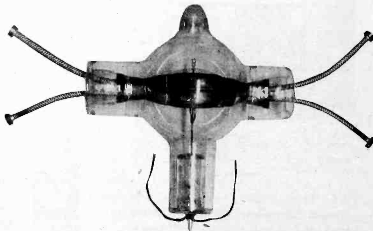
Fig. 2 Water-cooled split-anode magnetron
