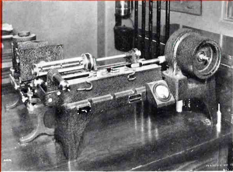
Left—Telephotograph Receiver
