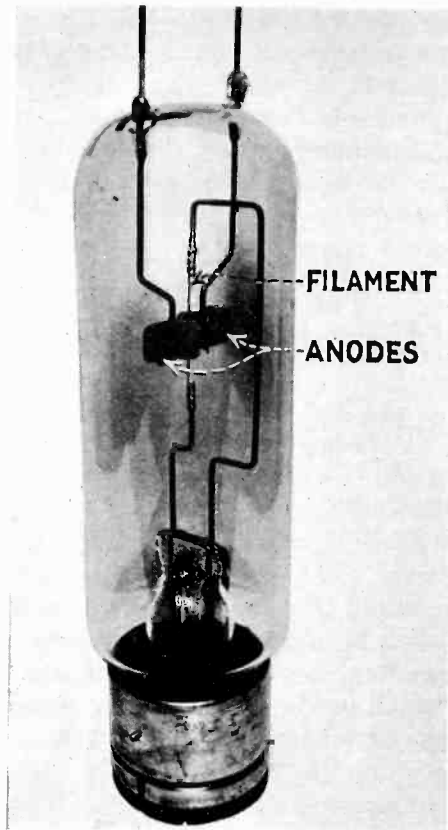
Fig. 1 Small split-anode magnetron
