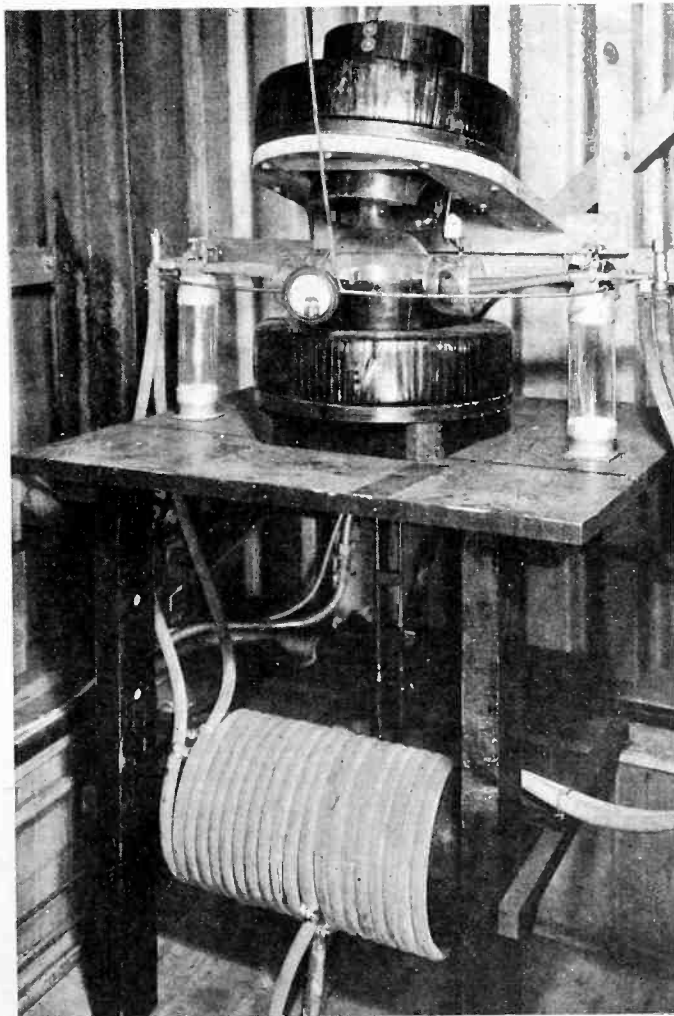
Fig. 4—Water-cooled split-anode magnetron and associated apparatus for production of high-power high-frequency oscillations
