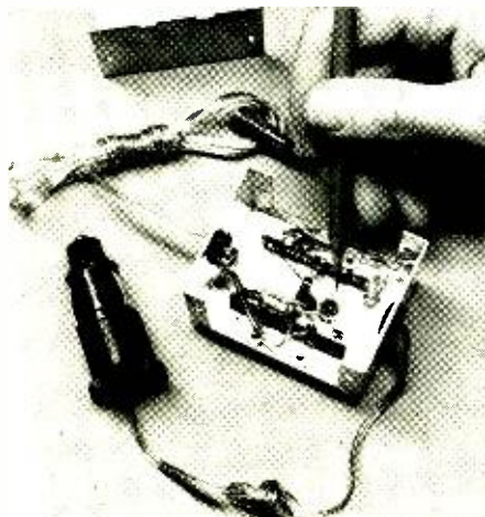
Fig. 3. Model of the converter built by the author. Converter is capable of supplying output currents up to 200 mA. IC is indicated by pencil. Cigarette-lighter plug housing is shown in foreground.
