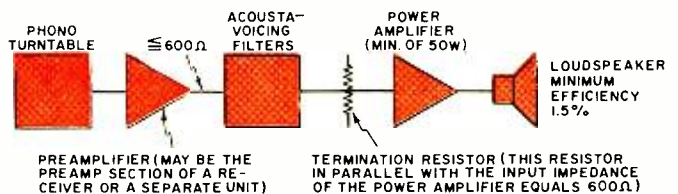
Fig. 6. Installation of equalizing filters in high-fidelity system.
