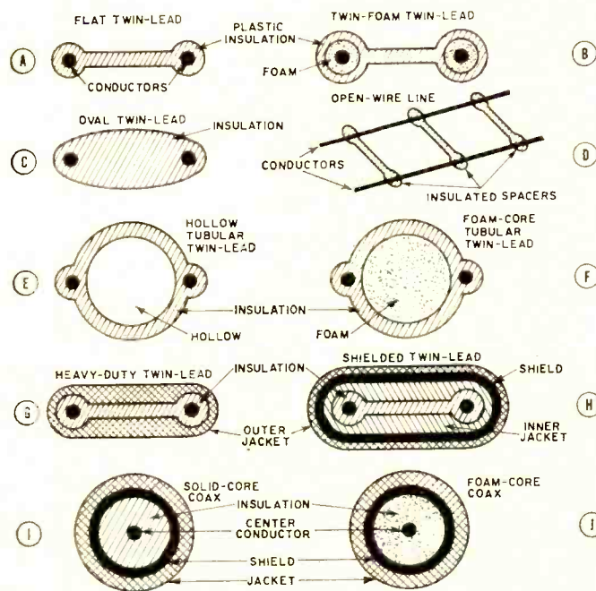
Fig. 3. Cross-sections of various types of lead-in.
