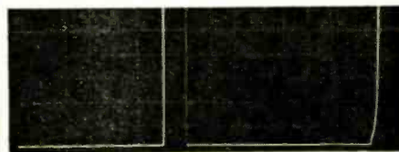
Fig. 1. Base-emitter V-I characteristics of the "p-n-p" 2N3905 (left) and "n-p-n" 2N3904 (right) silicon transistors. In both cases H is 1 V/div., V is 1 mA/div.
