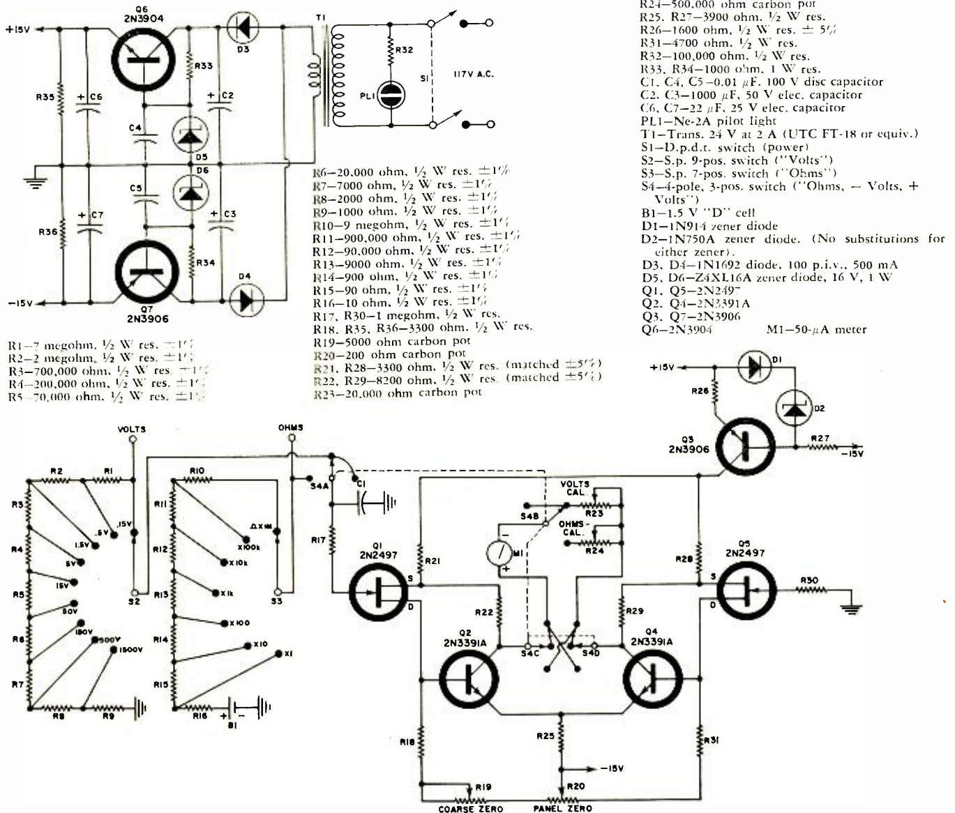
Fig. 3. The complete schematic diagram and parts list for the solid-state volt-ohmmeter and its regulated power supply.
