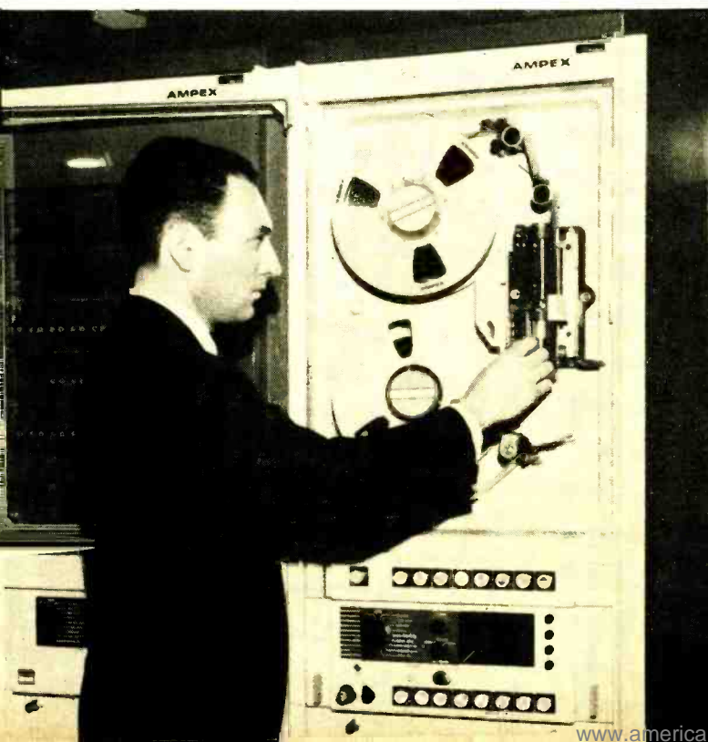
Fig. 1. FAA project engineer adjusting two-channel Ampex F-950 rotary head instrumentation tape recorder used in development of a processing subsystem for radar data to help traffic control personnel better identify aircraft during storms.
