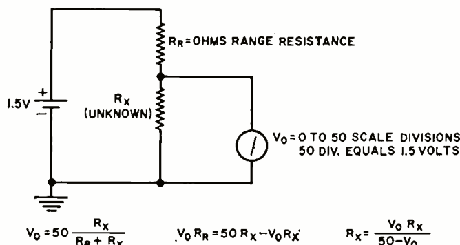
Fig. 2. This schematic shows the ohmmeter's divider feature. The equations included are used to calculate calibration points.
