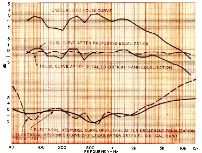
Fig. 5. The response curves of a relatively smooth system in which conventional tone controls can do much to restore overall balance. This type of system is difficult to equalize completely due to close spacing and steep slopes of irregularities.
