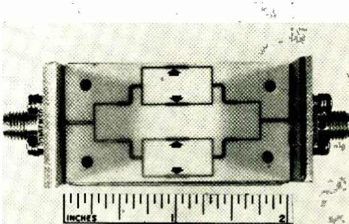
Fig. 5. A 4-to-1 hybrid divider-combiner, which effectively combines four amplifiers (inserted at the arrows) in parallel. These amplifiers may simply be microwave transistors.
