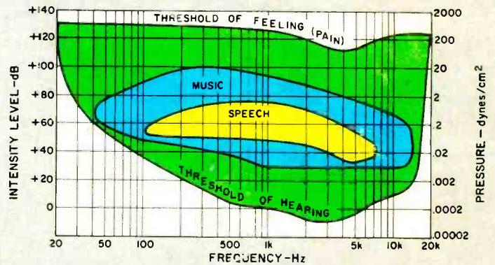
FREQUENCY and VOLUME RANGES. The approximate boundaries of normal hearing based on Fletcher-Munson data. No sound is heard below level indicated by the lower contour. Sound levels that are above the upper contour are felt rather than heard and may be accompanied by a sensation of pain. Also shown are volume levels and the frequency ranges of music as well as of speech.
