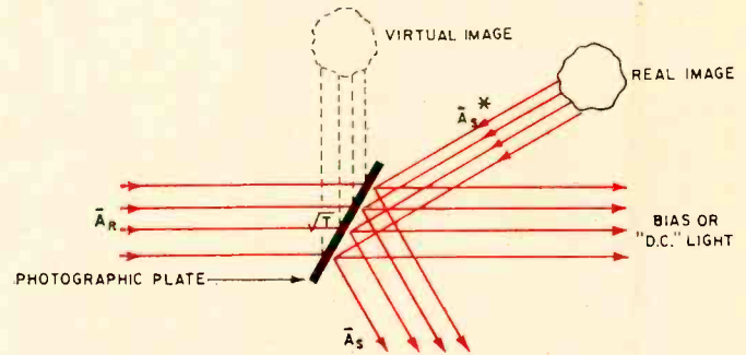
Fig. 2. Developed hologram is illuminated by reference beam. Lenses are not needed to project a real image onto a screen and the naked eye sees the virtual image in three dimensions.
