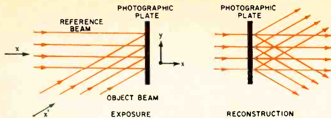
Fig. 4. The original electric field distribution is recreated during the reconstruction process. Here \theta is the angle between object and reference beams at photographic plate surface.
