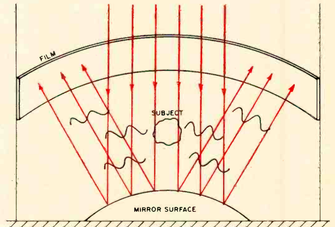
Fig. 3. A 360° hologram can be made by wrapping film around the inside of a cylindrical support in such a way that it picks up light reflected from the subject and curved mirror.
