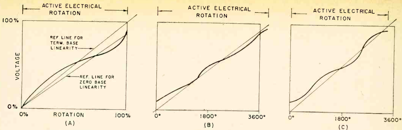
Fig. 3. Although the reference lines of terminal-based potentiometers pass through zero voltage at 0% rotation and maximum voltage at 100% rotation, slope can vary within certain limits as indicated by linearity graphs.
