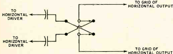
Fig. 11. Polarity-reversal switch for scope horizontal amp.
