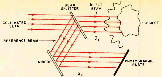
Fig. 1. An experimental setup used to make Fresnel holograms. A beam splitter divides collimated light into the object and reference beams, \bar{A}_s and \bar{A}_r , that serve to compose the picture.
