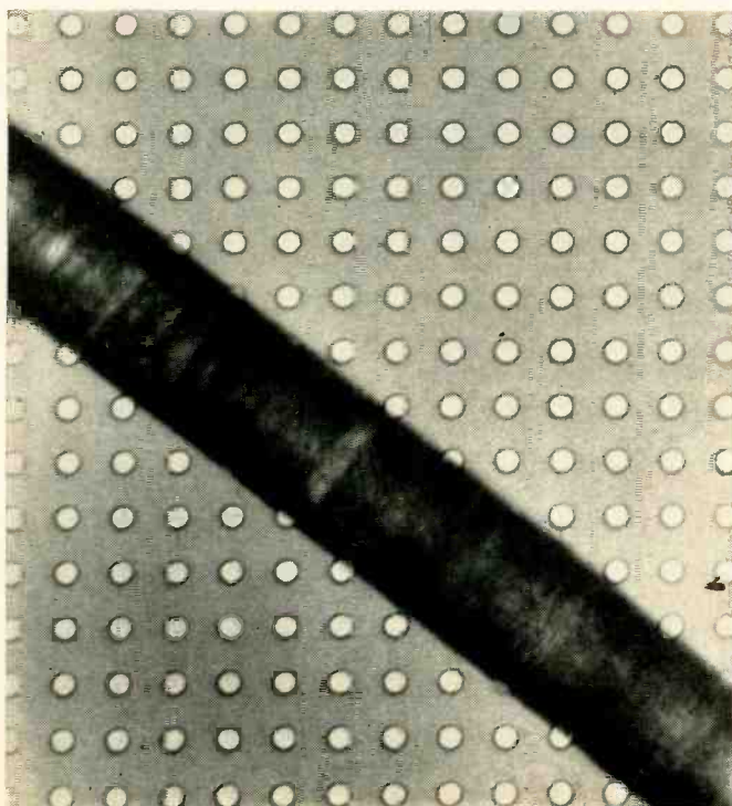
← Here is a magnified portion of target structure of the new camera tube. The entire silicon substrate is about the size of a nickel while the maximum target area measures a half inch on a side. In this area there are about 700,000 silicon photodiodes, each one of which is about 0.3 mil (0.0003 in) in diameter, spaced about 0.8 mil apart. The human hair, shown here for comparison, is about 2 mils thick.
