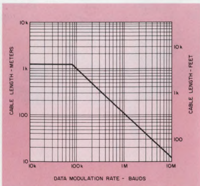
3. Permissible cable length depends on the data modulation rate. The graph is valid for twisted-pair cable, 24 AWG, and a balanced interface.
