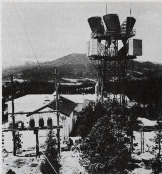
1960—Radio-relay stations like this Western Electric TH microwave system between the Denver-to-Salt-Lake-City route standing atop Buckhorn Mountain (8306 ft) in Colorado, start taking over from cables and lines.
