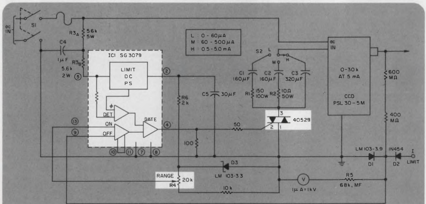
In this power-supply regulator, a triac driven by an SG3079 zero-crossover detector controls the ac line
