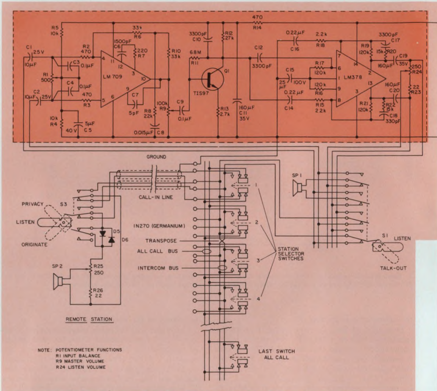
3. A differential input amplifier replaces the transformer for this balanced-line intercom. The entire circuit shown
