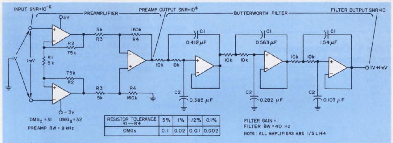
2. A typical data channel contains a high-gain high-CMRR preamplifier and sharp-cutoff low-pass filter.
