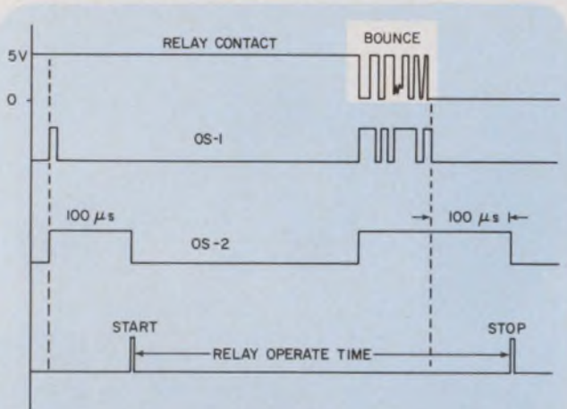
2. The circuit includes the bounce time into the start/stop interval, but the time of OS 2 automatically cancels and isn't included.
