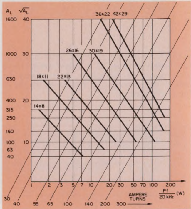
3. Taking the approximated straight line from the Hanna diagram, you can plot a more convenient family of curves for use in practical designs.
