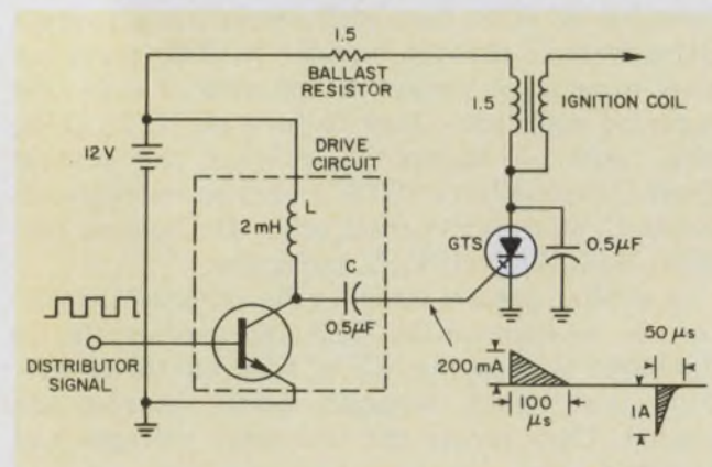
7. Ignition signals from an automobile distributor control the on/off timing of a GTS thyristor. High-voltage developed in the ignition-coil secondary, when the GTS turns off, produces a spark across the gap of a spark plug. The GTS turns on within 100 \mu s and off in about 50 \mu s and needs about 1-A peak to extinguish.
