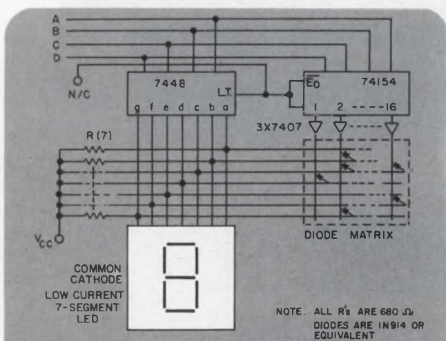
1. Letters and other symbols can be displayed on a 7-segment numerical display, in addition to the usual numbers.
