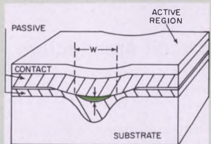
Buried-channel laser structure shows active region (about 10 \mu m wide).
