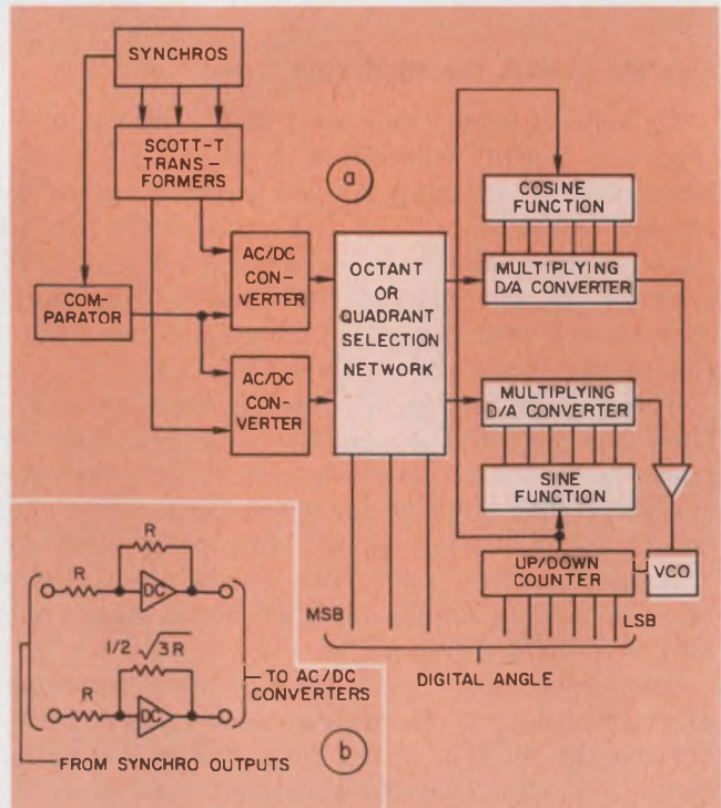
1. Conventional multichannel converters (a) use many linear components. You can replace the Scott-T transformer with an electronic Scott-T converter (b).
